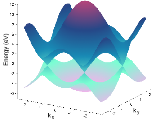
Figure 4: Dispersion relation for graphene.
