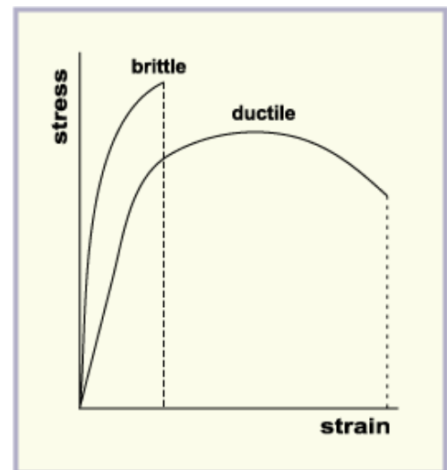
Figure 1. Comparison of stress-strain curves for ductile and brittle materials [3].
