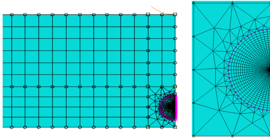
Figure 4. (a) Specimen with mesh. (b) Detail view of mesh surrounding crack tip.
