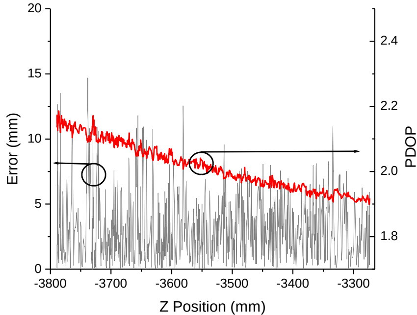
Figure 6-15: 3-D error as tag is moved along the optical rail in the -z direction with the corresponding PDOP shown. No channel effects are included, leading-edge detection is used along with a modulation factor \beta = 5 , a 21-sample MIQR filter, and 5x averaging of the TDOA results. The 1-D ranging error stays almost constant at 1.22 mm while the PDOP and corresponding 3-D error increase as the tag is moved farther along in the -z direction away from the center of the base station geometric configuration.
