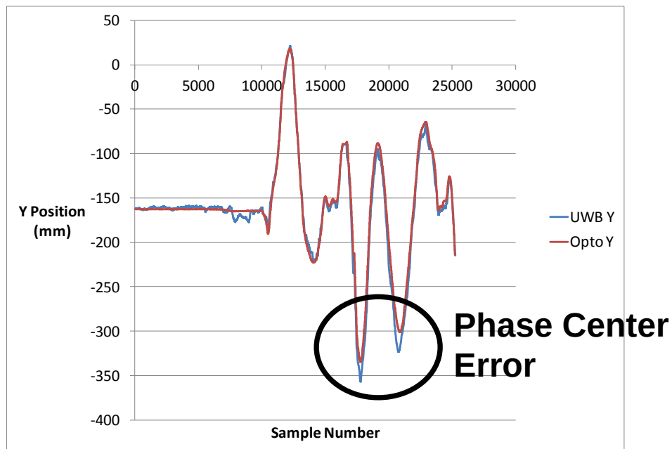
Figure 8-11. Y Position of Tag 10 in a dynamic freeform experiment. The large offsets are indicative of phase center error which ultimately causes these types of scaling errors.
