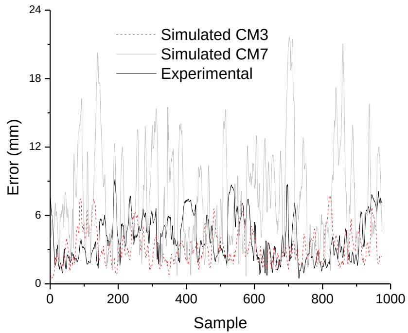
Figure 6-18: Comparison of final 3-D error from optical rail experiment, CM3 simulation, and CM7 simulation over 1000 points along the optical rail.
