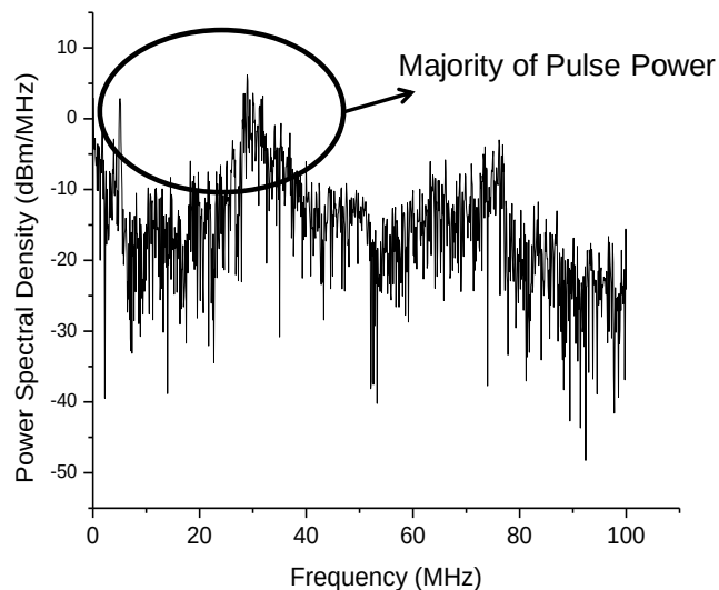
Figure 6-8: Frequency content of simulated time extended UWB pulse including receiver and multipath effects. The majority of the pulse power is contained from 0-30 MHz.
