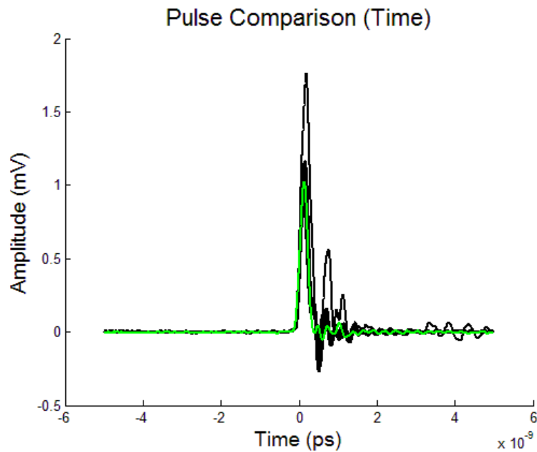
Figure 7-11: Baseband UWB pulses from the 15 tags (in black). A reference pulse from a separate SRD-based pulse generator (green). The pulse amplitude across the 15 tags has some variation, and some of the integrated tags exhibit more ringing than the reference tag. Overall, all of these signals are usable for UWB indoor positioning.
