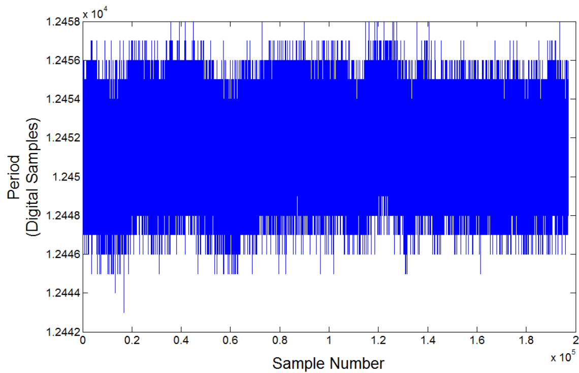
Figure 7-26: Period between successive leading-edges of the UWB pulse train from Tag 2 in digital samples spaced 20 ns apart for almost 200,000 successive UWB pulses.
