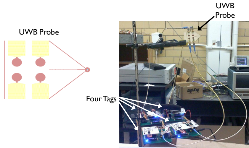
Figure 12-1: Experimental setup showing four tags connected to an ultra-wideband probe containing four monopole antennas in a known geometrical configuration.
