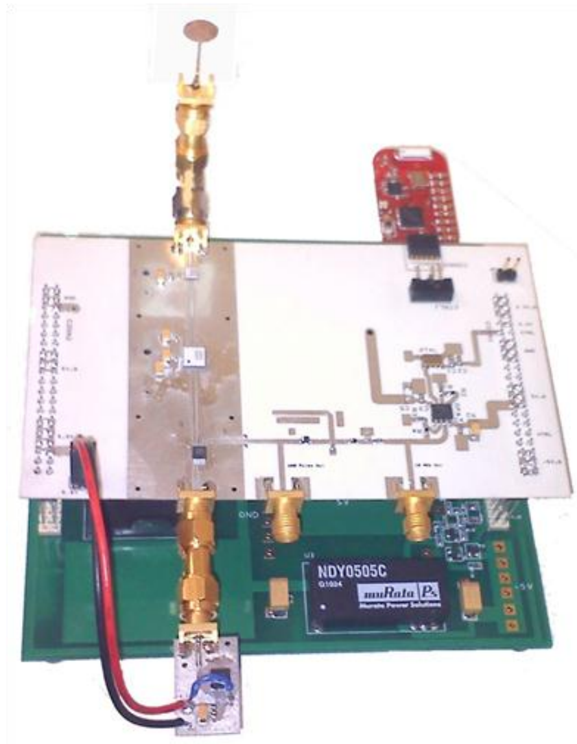
Figure 7-9: Integrated tag including DC power board, RF board, MSP430-EZ2500 microcontroller board, VCO connected via external SMA connector, and monopole UWB antenna.
