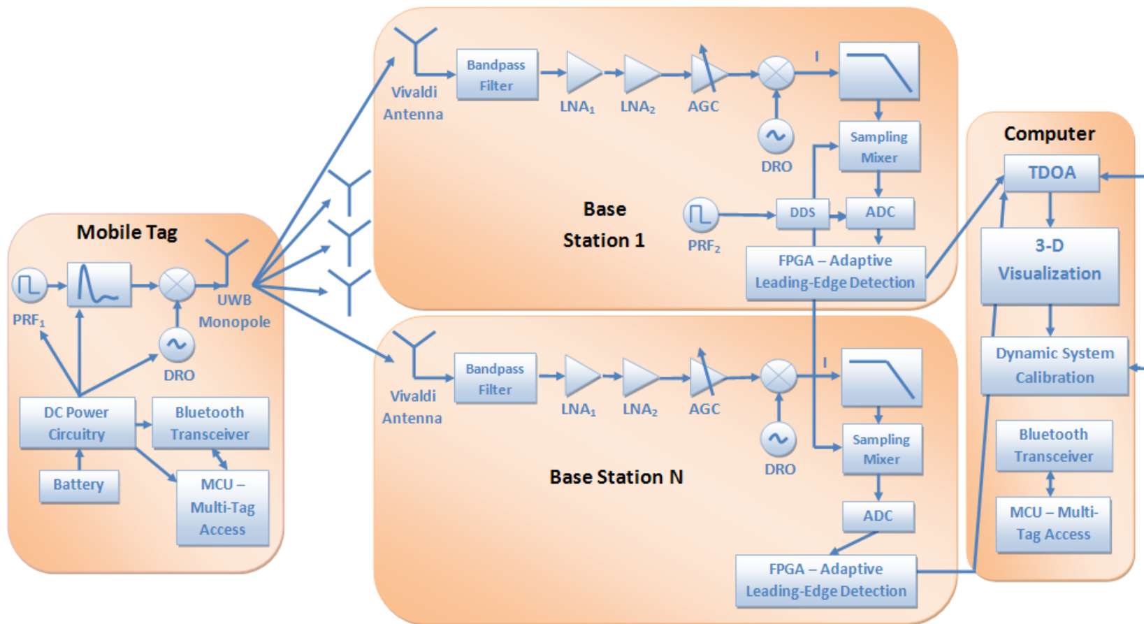
Figure 11-2: Proposed UWB system architecture which incorporates a Bluetooth-based multi-access scheme, dielectric resonator oscillators for reduced phase noise, automatic gain control for increased operating range, a front-end bandpass filter to mitigate IEEE 802.11a/n interferers, adaptive leading-edge detection for system operation in low SNR and NLOS environments, and dynamic system calibration to mitigate adverse effects including jitter, system clock drift (time scaling), and cable length and phase center variation.
