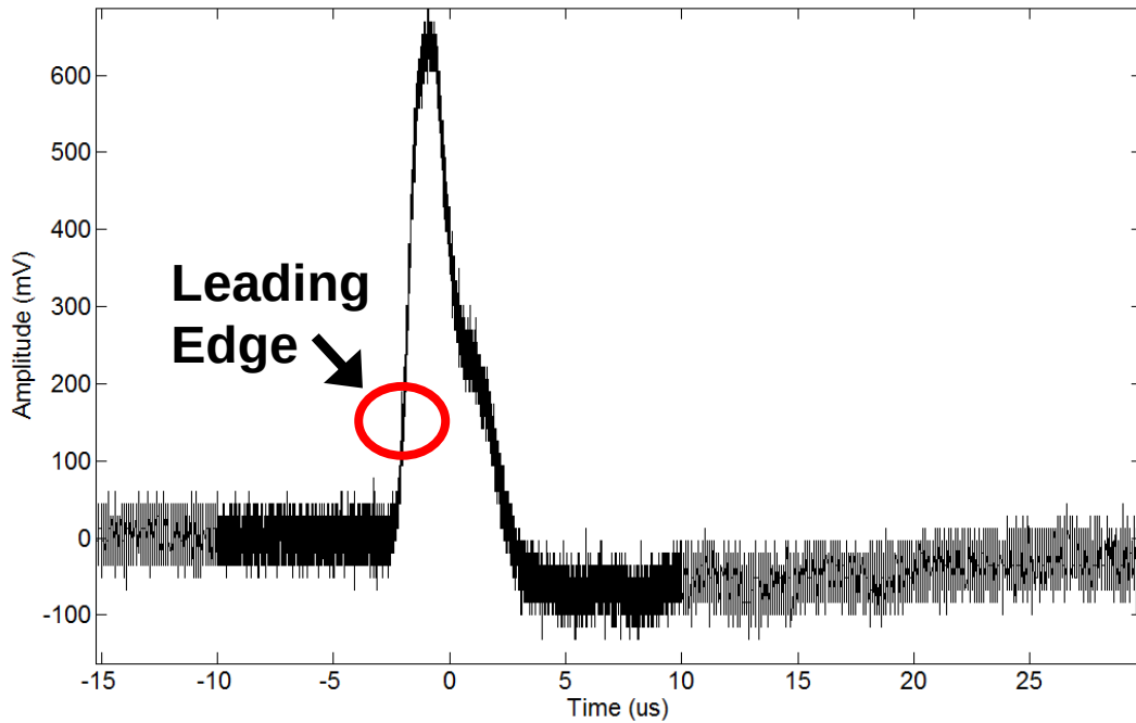
Figure 9-8: UWB pulse before the ADC where the high slew rate leading-edge can be seen and provides a much sharper trigger point for resolution of the time-of-arrival (10-20 ps) when compared to the peak of the UWB pulse (30-300 ps for high SNR signals).
