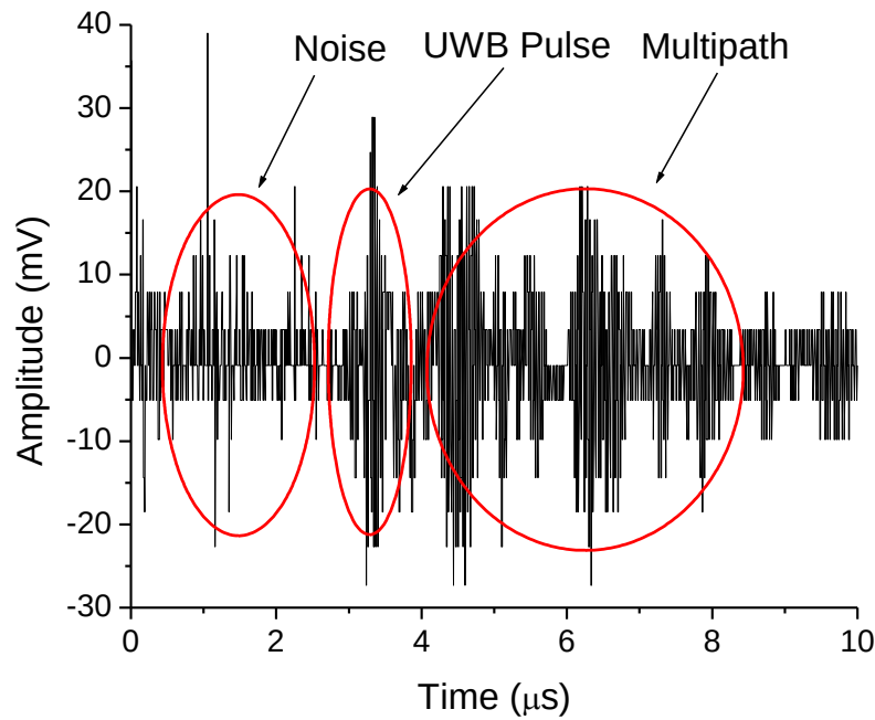
Figure 9-22: Simulated UWB time-extended signal where the Tx-Rx are 3 m apart in an industrial LOS environment defined by the IEEE 802.15.4a channel model and no automatic gain control is used in the UWB receiver creating a weak signal. Electrical noise, multipath interference, and quantization noise are observed. SNR = -2.61dB.
