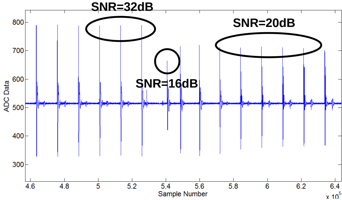
Figure 9-14: Raw UWB signal after the ADC where various UWB pulse peak heights can be seen to illustrate variations in the SNR of the received UWB signal.
