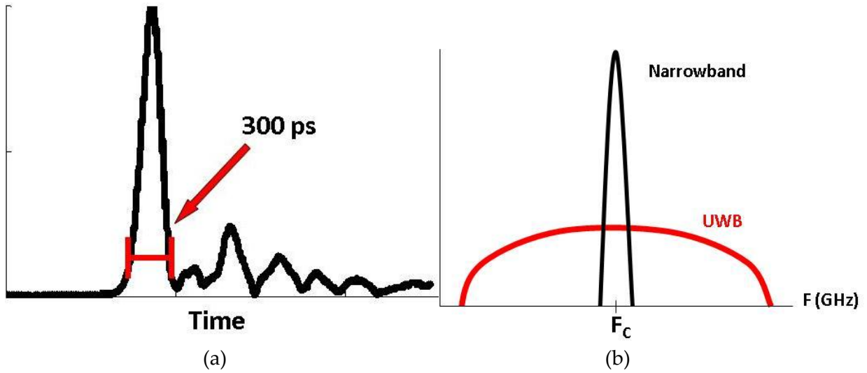
Figure 1-1: Example of an ultra-wideband signal: (a) time-domain baseband 300 ps wide pulse, (b) frequency domain up-converted UWB pulse compared to typical up-converted narrowband signal.
