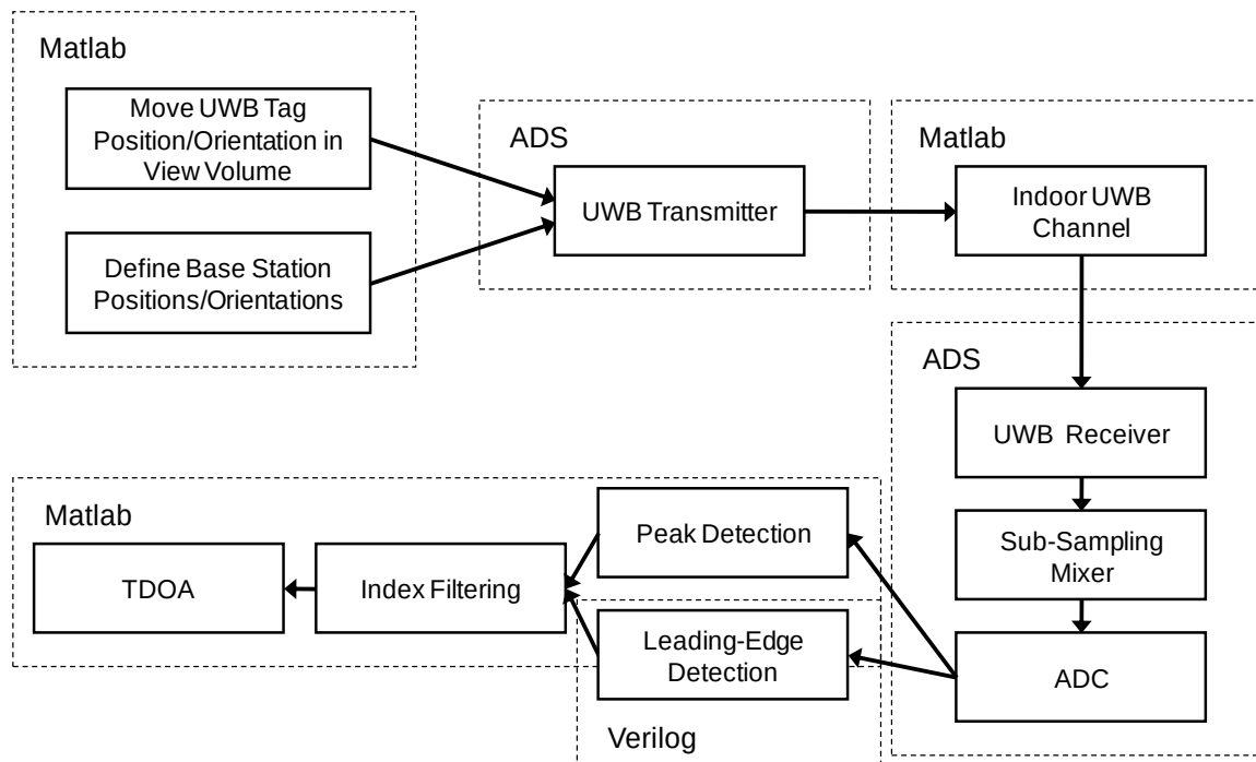
Figure 6-2: Block diagram of overall system simulation outlining the different portions of the system simulated in Matlab, Agilent ADS, and Verilog.
