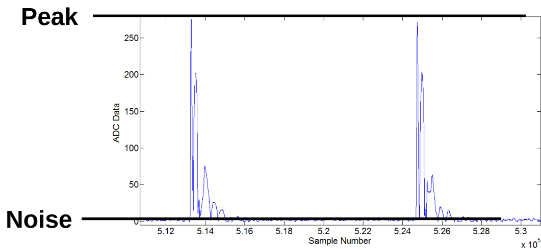
Figure 10-3: Typical received UWB pulse after taking the absolute value of the raw signal and passing it through a 16-sample averaging filter. The amplitude between the peak of the UWB signal and the noise floor is shown to highlight the high SNR's which can typically be achieved when operating with LOS links.
