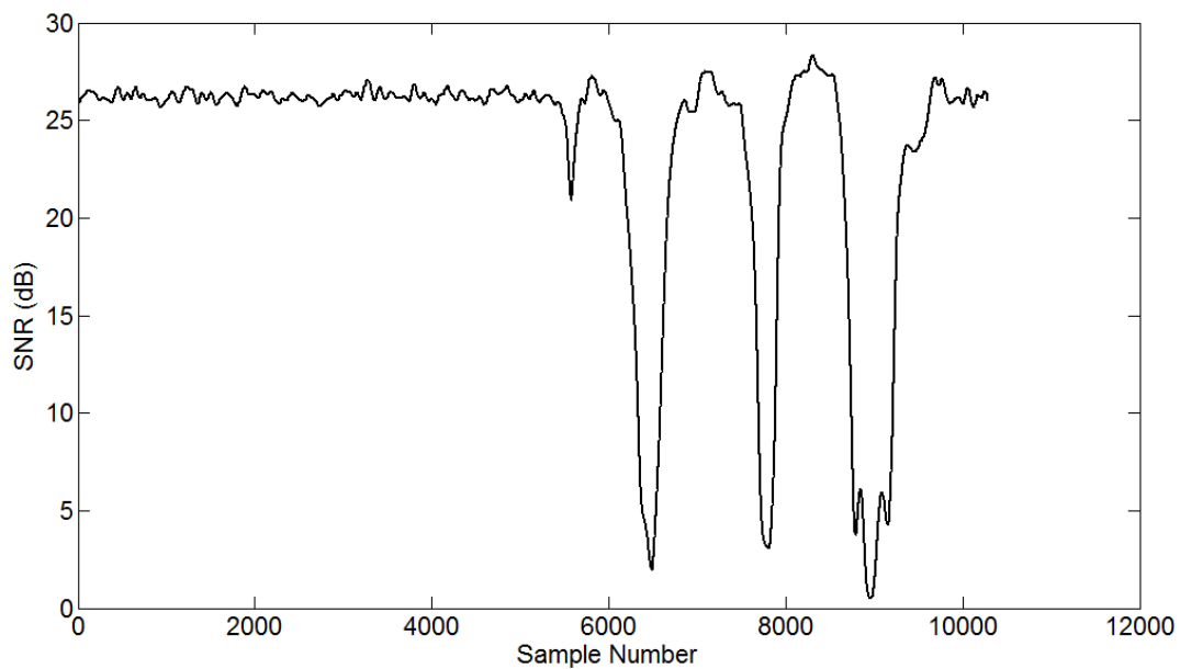
Figure 10-5: The received UWB pulse signal from Figure 10-4 expressed as SNR in dB.
