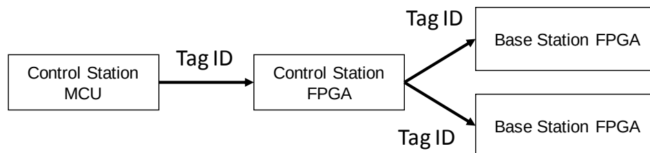
Figure 7-15: The current tag ID is sent from the control station microcontroller to the control station FPGA. From the control station FPGA, the tag ID is sent to all base station FPGAs to synchronize the current tag ID.
