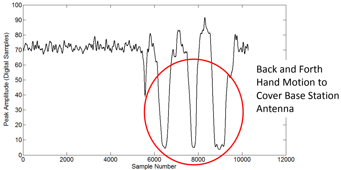
Figure 10-4: Experimental data measuring the peak of the UWB pulses in digital samples. The peak value decreases rapidly as a human hand approaches and almost completely covers the antenna. The quick reduction in link quality is easily measured by measuring the UWB pulse peak values.
