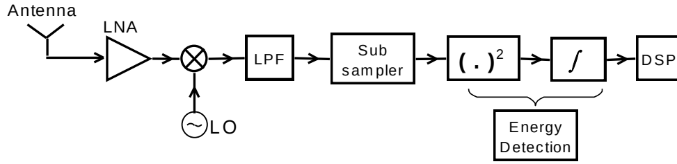
Figure 1-6: UWB receiver architecture which combines the carrier-based and energy detection-based UWB receiver schemes [19].
