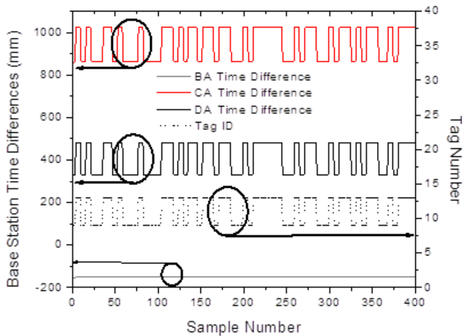
Figure 7-18: Time differences received at the computer where two distinct bands can be seen representing the 3-D positions of tags 9 and 13.
