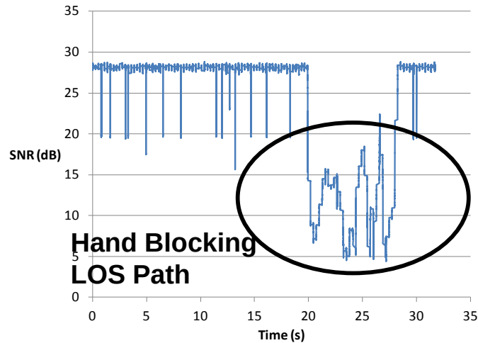
Figure 9-15: The SNR received at a UWB receiver over a 30 s period where hand blocking occurs between 20-30 s. This hand blocking reduces the LOS UWB pulse and consequently the SNR drops from 28 dB to between 6-15 dB.
