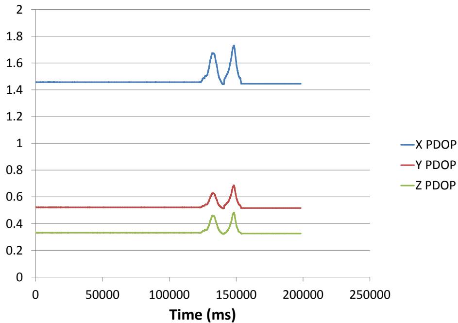
Figure 8-20. PDOP data for the five base station optical rail experiment showing the PDOP in X,Y,Z. The total PDOP is 1.50 ( X=1.45, Y=0.52, Z=0.34 ).
