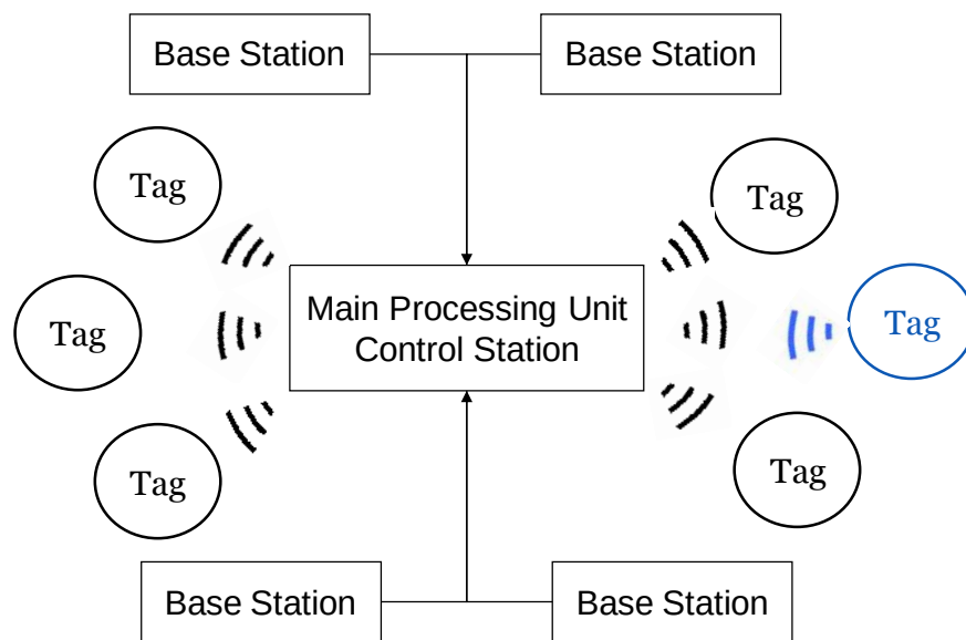
Figure 7-2: Time division multiple access where the main processing unit broadcasts all tag IDs in a round-robin fashion and the base stations localize the tag 3-D positions.
