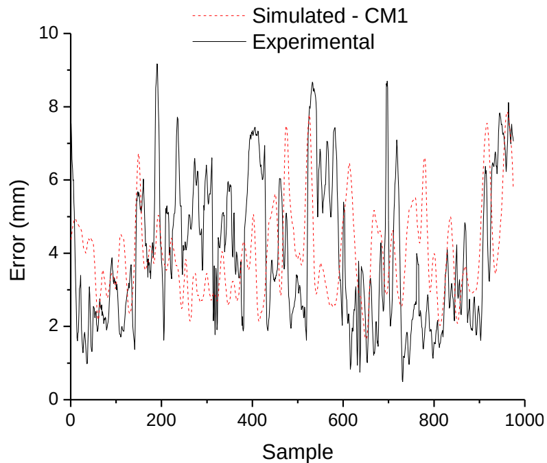
Figure 6-19: Comparison of final 3-D error from optical rail experiment and CM1 simulation.
