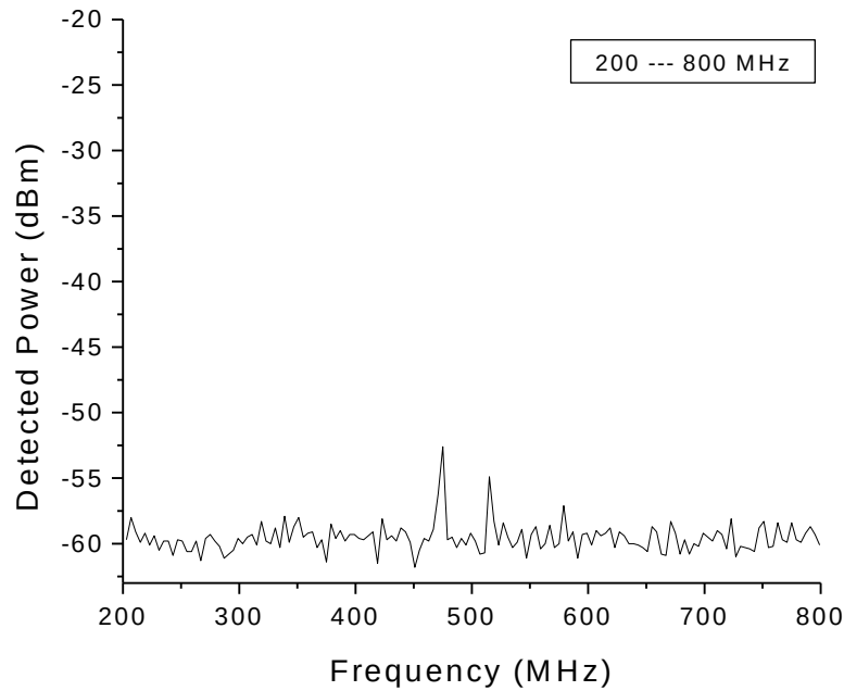
Figure 4-25: Measured EMI over frequency range of 200 – 800 MHz.
