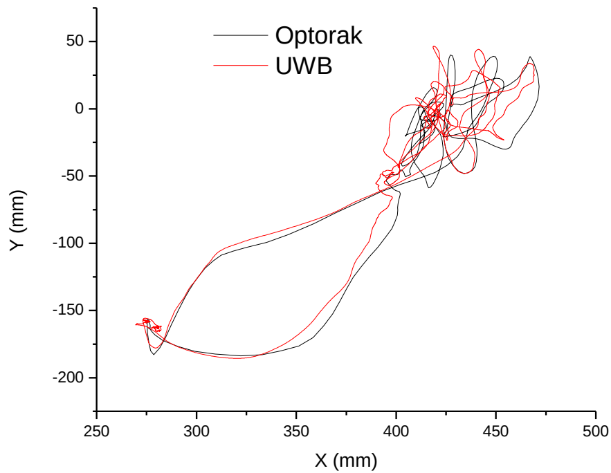
Figure 8-6. X-Y cross section showing optical and UWB data for a dynamic freeform experiment for Tag 10. Good agreement can be seen between the UWB and optical tracking systems, although certain 3-D locations have more error than others.
