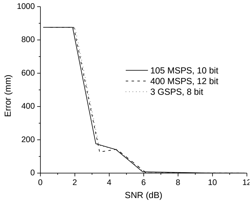
Figure 6-24: Simulated leading-edge detection 1-D error vs. SNR of received UWB pulse for three ADCs.
