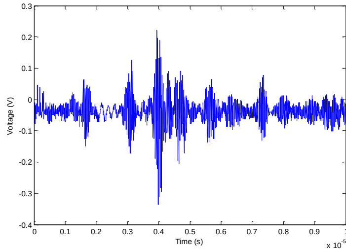
Fig. 10. Received CM3 Commercial LOS signal after passing through the receiver chain depicted in Figures 8 and 9.
