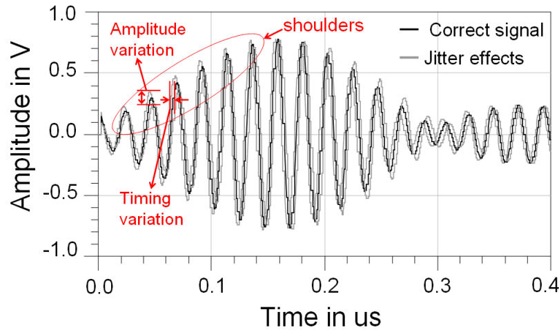
Figure 5-5: The “shoulder effect” in static scenario: the received single channel sub-sampled signal modulated by the equivalent offset carrier frequency [19].
