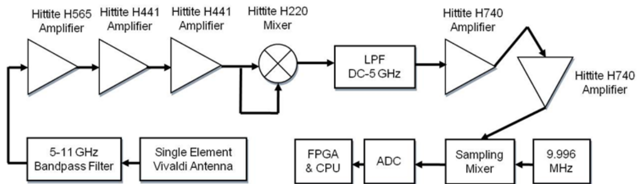
Figure 7-13: Block diagram of the UWB receiver where a single element Vivaldi antenna is connected to a 5-11 GHz band-pass filter, goes through three stages of amplification followed by a squaring mixer, then is low-pass filtered, goes through two stages of baseband amplification, and is sub-sampled to be 2500 times larger in the time domain. The signal is then converted to digital and processed on a FPGA before being fed to a C++ application on a computer via a serial connection [219].
