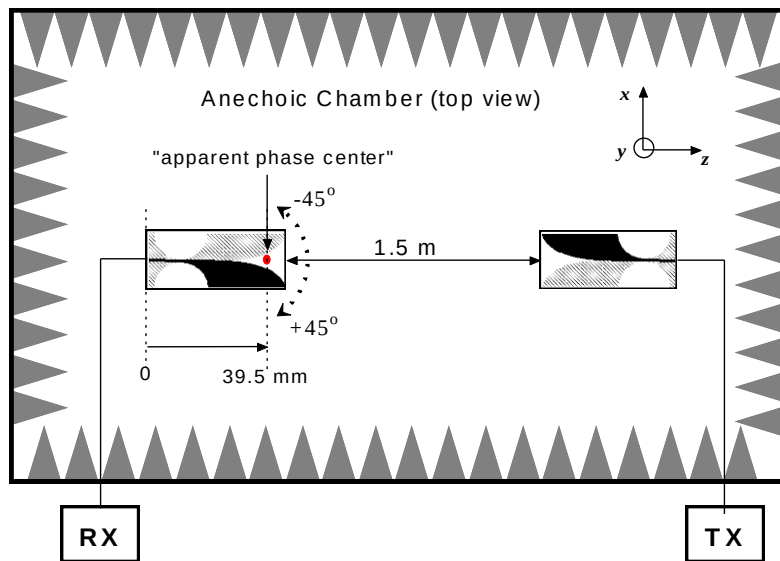
Figure 5-7: Experimental setup of Vivaldi antennas in an anechoic chamber used to measure Vivaldi antenna directivity-dependent phase center variation [18].
