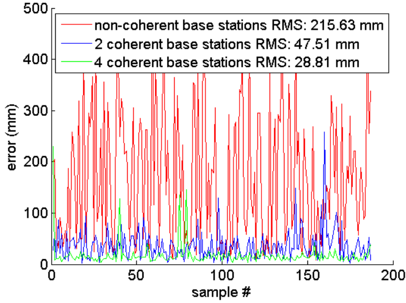
Figure 5-2: Raw data captured using wired transmitter and receiver clocks while changing between coherent and non-coherent LOs at each of the four base stations [93].
