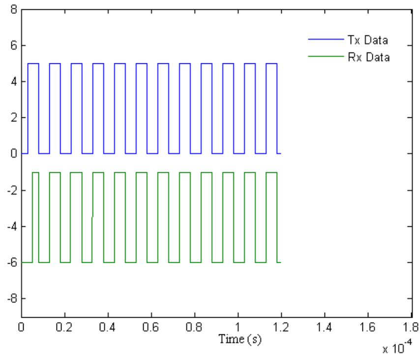
Figure 4-7: Original data stream and recovered data stream after passing through Tx/Rx.
