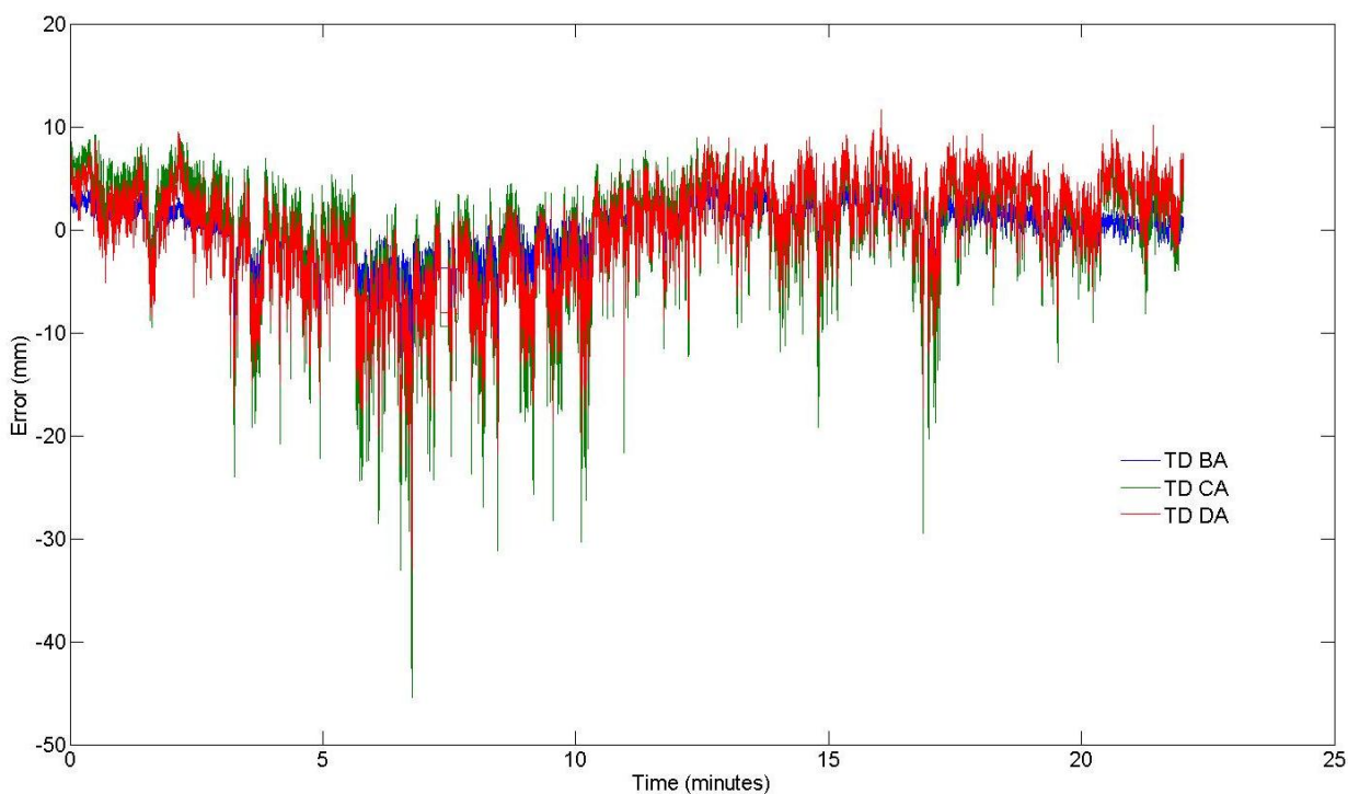
Figure 7-22: Measured receiver clock jitter and drift over a 23 minute interval caused by the 9.996 MHz signal used by the sub-sampling mixer to sub-sample the incoming UWB pulses. The clock jitter and drift can cause up to 30-40 mm of error in each measured range difference. This can cause 3-D positioning errors of 30 mm or more.
