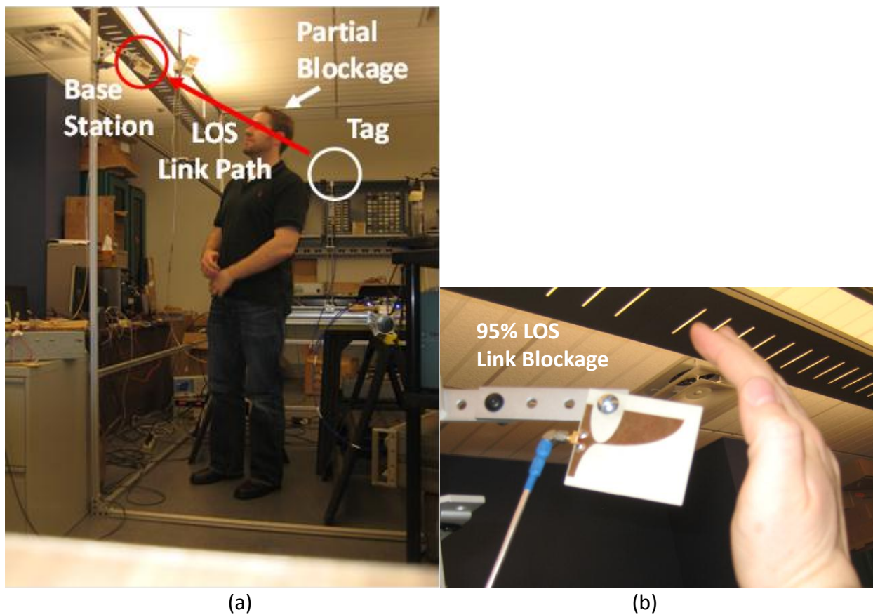
Figure 10-1: Experimental setup where partial blockage is introduced in the LOS link path: (a) 30-40% blockage, (b) 95% blockage.
