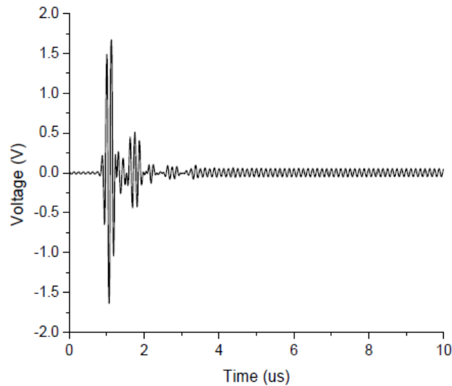
Fig. 5. Simulated UWB pulse after upconversion from LO_1 and amplification.
