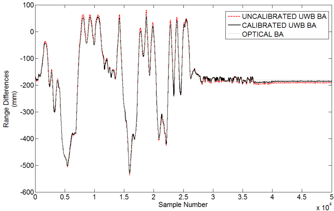
Figure 7-29: Raw range difference data for base station B minus base station A (BA) for both the optical and ultra-wideband positioning systems as the tag is moved around the view volume. Both uncalibrated and calibrated UWB range difference curves are shown. The calibrated UWB range differences better fit the optical BA range differences.
