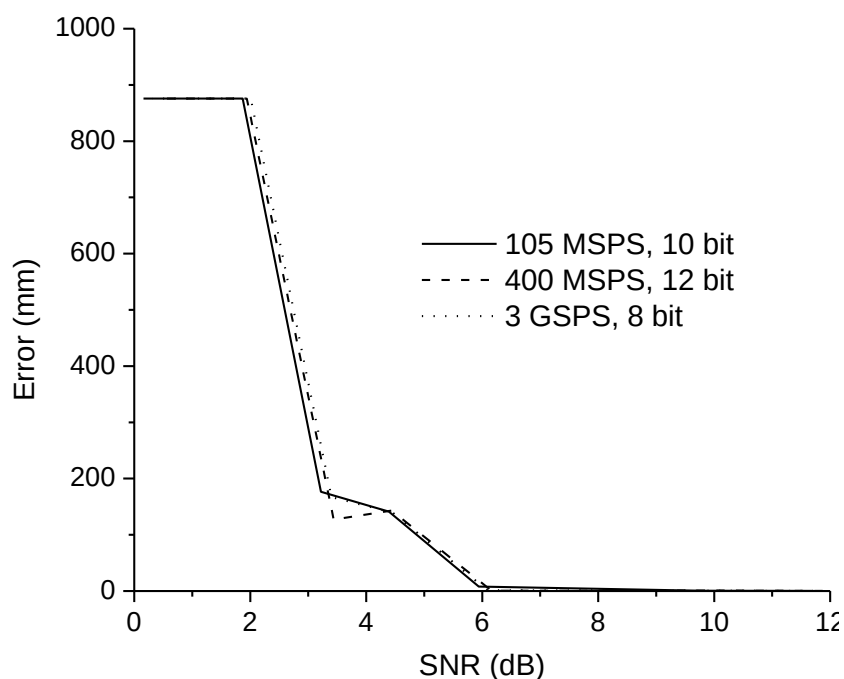
Figure 9-17: Simulated leading-edge detection 1-D error vs. SNR of received UWB pulse for three ADCs.
