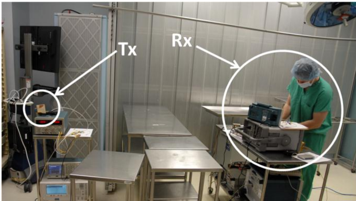
Figure 4-16: Experimental setup in the operating room during non-live scenario.
