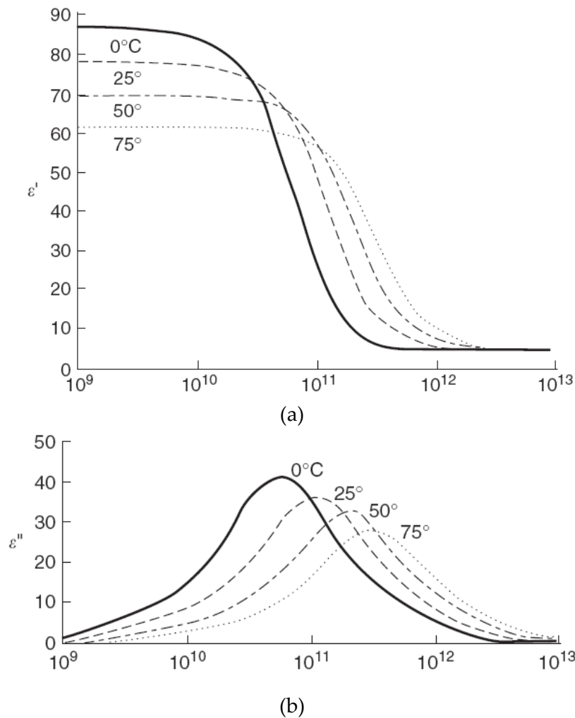
Figure 2-5: Effects of temperature on complex permittivity of water: (a) \epsilon' , (b) \epsilon'' [78].
