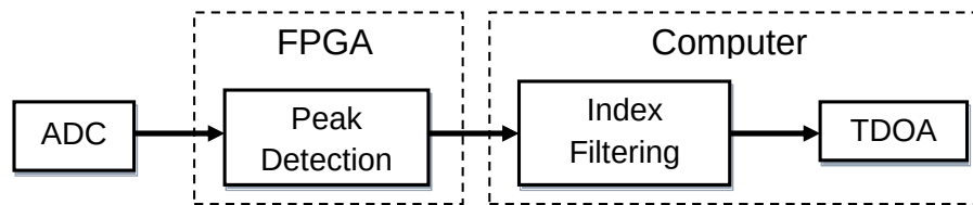
Figure 6-7: Block diagram of digital backend at the UWB receiver.
