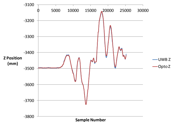
Figure 8-12. Z position of Tag 10 where the other error sources (geometric dilution of precision and phase center biasing) do not occur to large extent.
