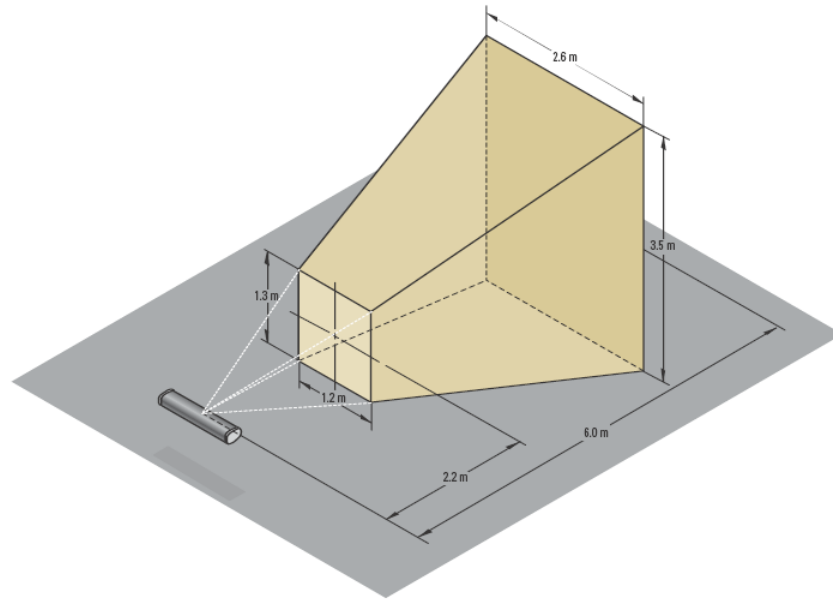
Figure 3-2: NDI Optotrak Certus view volume with 3.8 m in the z-direction and an in-plane area of 2.6 \times 3.5 \text{ m}^2 at a z distance of 6 m [99].
