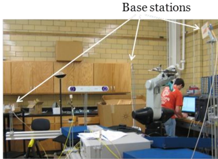
Figure 5-10: 3-D localization experiments with four base stations deployed.
