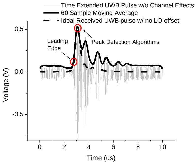
Figure 6-9: Simulated UWB time extended pulse for ideal case with LO\_offset = 3\text{MHz} . Channel effects (e.g. pathloss, multipath interference) are not included to provide an ideal received signal. The system architecture in Figure 6-3 is used to capture the non-ideal performance of various system components. In the ideal case, both the use of peak detection and leading-edge detection algorithms at the FPGA result in accurately detecting the UWB pulse. The ideal case includes use of an ideal channel. PRF_1 and PRF_2 are not coherent.
