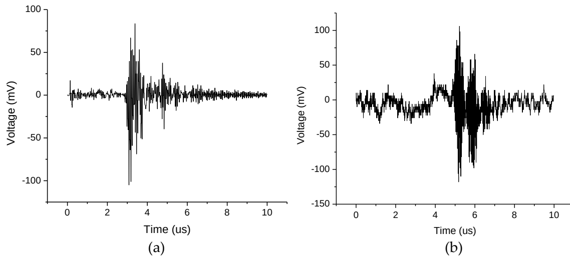
Figure 6-6: Time extended UWB pulse obtained at the UWB receiver after passing through the sampling mixer including indoor channel effects and non-linearities from the UWB transmitter: (a) simulated, (b) experimental.
