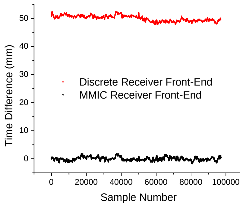
Figure 7-45. Time difference static data for two discrete front-end receivers versus two MMIC receivers in millimeters after applying a 300 sample averaging window.
