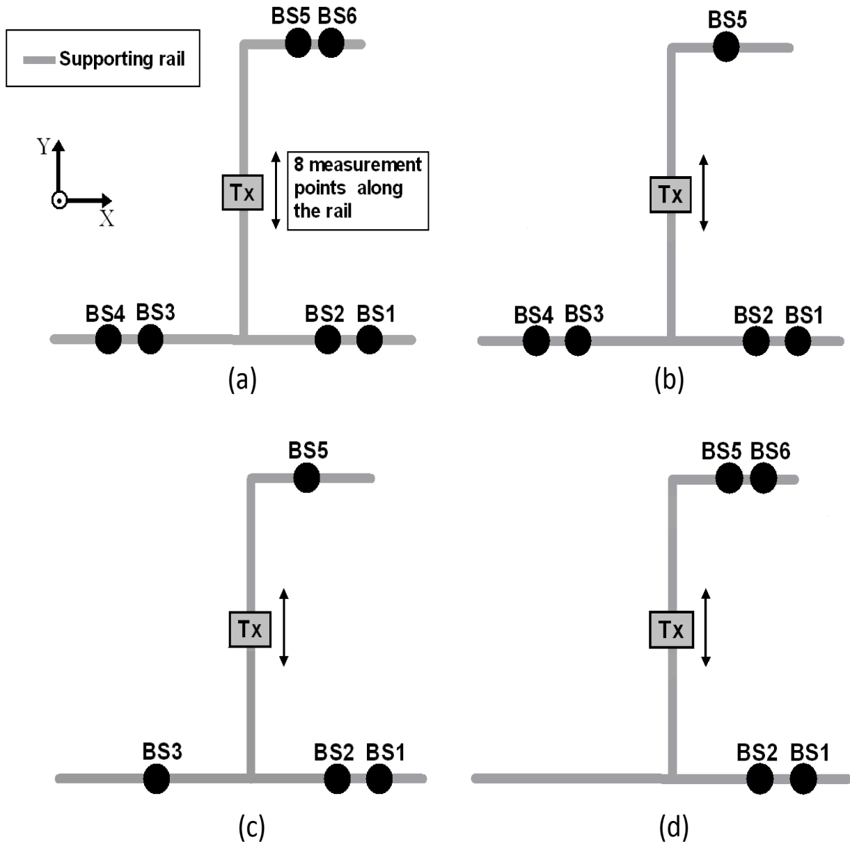
Figure 6-20: 3-D synchronized localization experiments: (a) 6 base stations. (b) 5 base stations. (c) 4 base stations with low PDOP. (d) 4 base stations with poor coverage in x -direction resulting in high PDOP [18].
