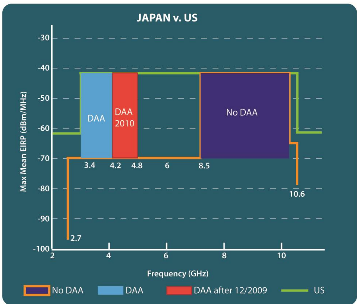
Figure 2-2: Comparison of allocated UWB bands between 3-11 GHz in the U.S. versus Japan.
