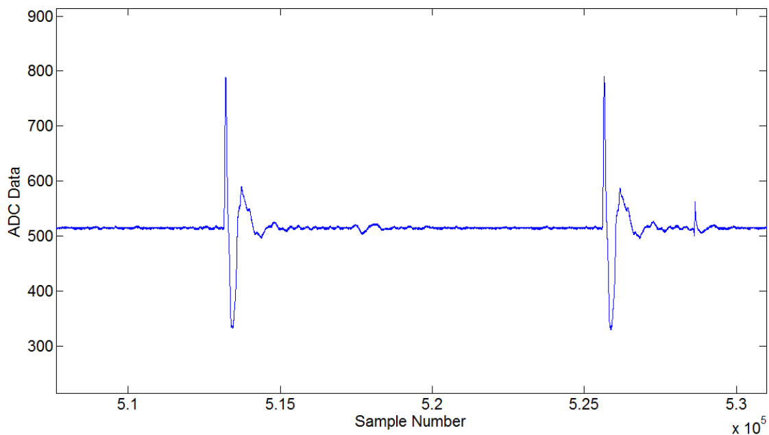
Figure 9-2: Raw received UWB pulse using a 2500x expansion factor after analog-to-digital conversion. A slight ringing is introduced by the high pass filter on the ADC which can be observed immediately after the initial UWB pulse. The original shape of the UWB pulse before analog-to-digital conversion is shown in Figure 9-1.
