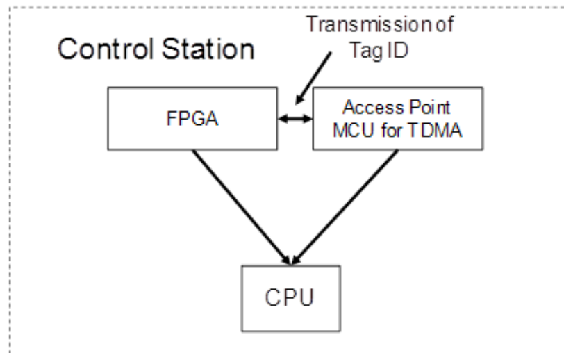
Figure 7-3: Control station architecture where Access Point MCU sends tag IDs to the FPGA for synchronous tagging of the TDOA data for TDMA approach.
