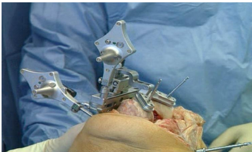
Figure 3-10: Example of a CAS system used in a TKR where optical trackers are attached to the femoral cutting guide and also to the femur itself. Stryker Knee Trac System (imageless).
