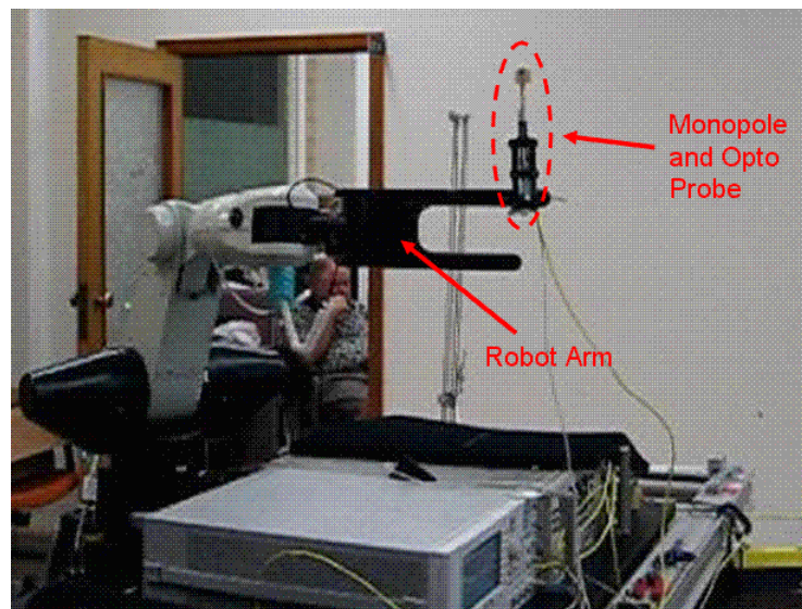
Figure 5-12: Experimental setup of robot tracking using the first generation UWB positioning system.
