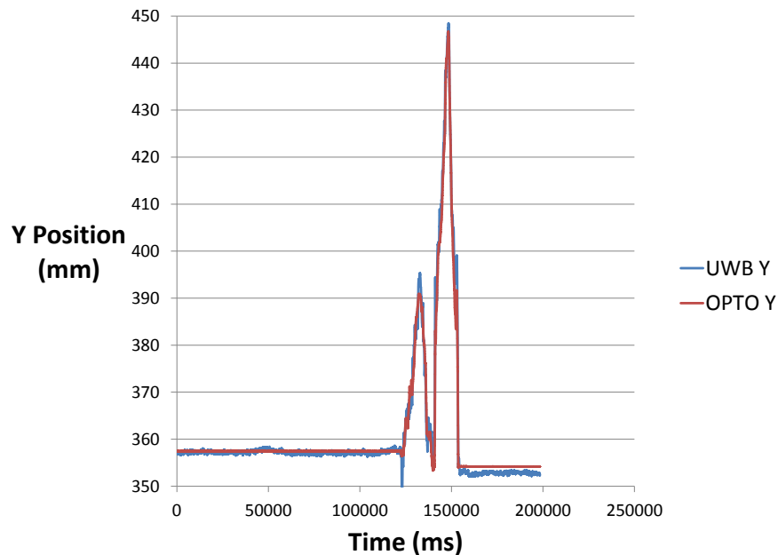
Figure 8-16. Y position values for both the UWB and optical tracking systems for an optical rail experiment where Tag 13 is dynamically moved along the optical rail. The RMSE in the Y dimension is 0.93 mm.
