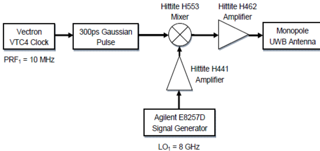
Fig. 2. Block diagram of the UWB transmitter where a 10 MHz clock triggers a step recovery diode pulse generator. The baseband pulse is then upconverted by a low phase noise LO ( LO_1 ) and amplified by a low noise amplifier. The signal is transmitted via an omnidirectional monopole antenna.
