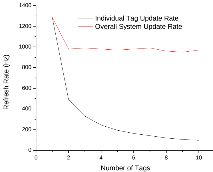
Figure 8-3. System and individual tag refresh rate versus the number of tags for up to 10 tags. The overall update rate with a single tag is around 1300 Hz. Only 1000 Hz total update rates can be achieved for multi-tag tracking since around 20% of the data is lost during the tag switching process.
