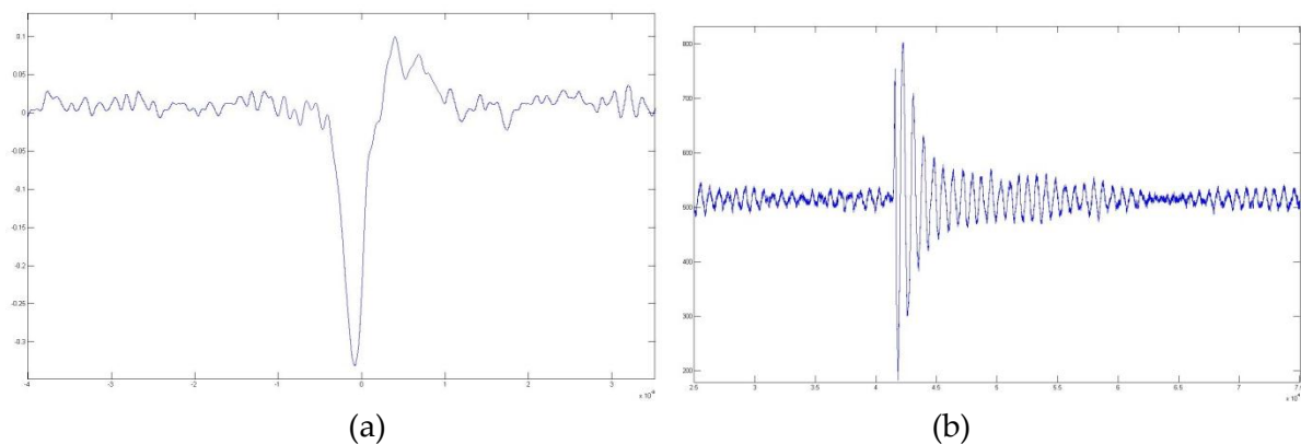
Figure 9-4: (a) 3 \mu s UWB pulse at a 10,000 expansion factor before analog-to-digital conversion, (b) 3 \mu s UWB pulse at a 10,000 expansion factor after analog-to-digital conversion where a large amount of ringing is evident which is caused by the RF transformer at the differential input of the analog-to-digital converter.
