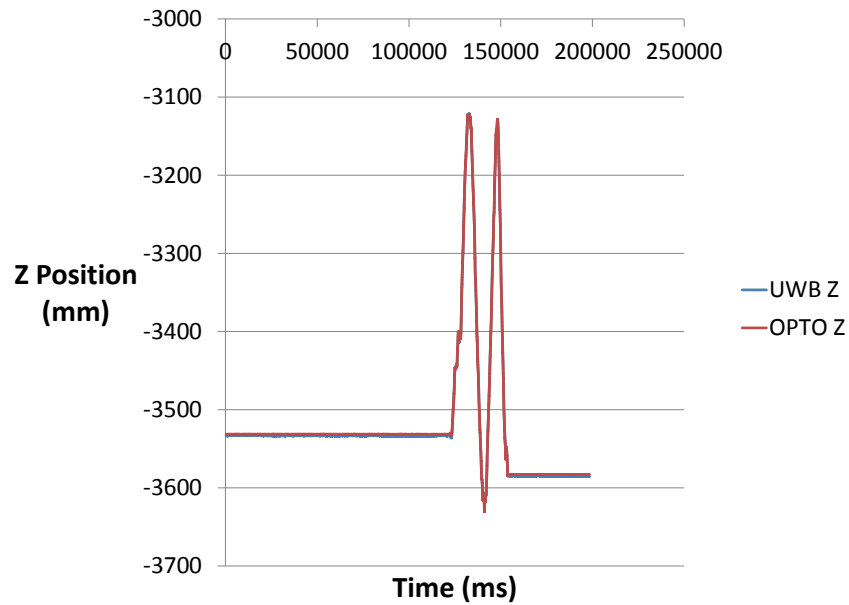
Figure 8-17. Z position values for both the UWB and optical tracking systems for an optical rail experiment where Tag 13 is dynamically moved along the optical rail. The RMSE in the Z dimension is 1.85 mm.
