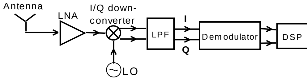
Figure 1-4: Carrier-based non-coherent UWB receiver architecture [19].
