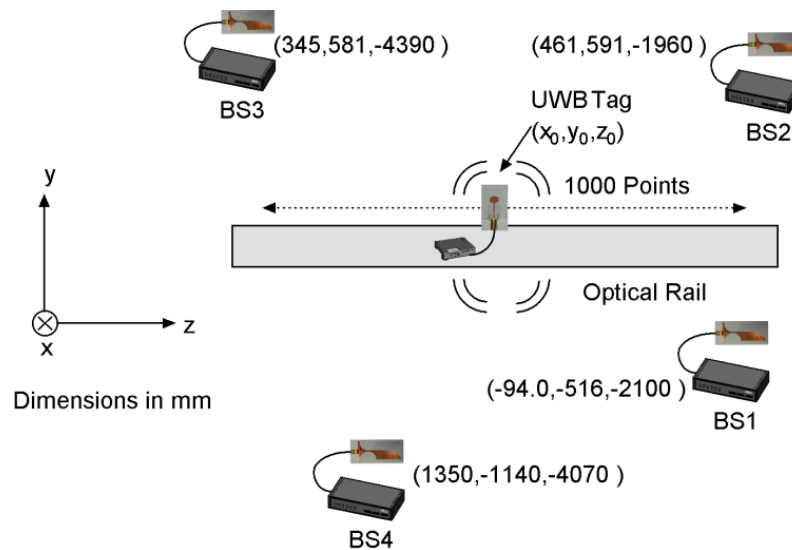
Fig. 11. Optical rail experimental setup where 1000 (or really 975) points are obtained as the tag is moved along the rail. For all 4BS Matlab driver files, this is the experimental setup used.
