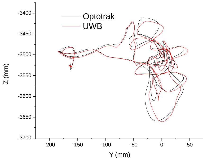
Figure 8-7. Y-Z cross section showing optical and UWB data for a dynamic freeform experiment for Tag 10. Good agreement can be seen between the UWB and optical tracking systems.
