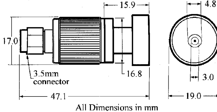
Figure 2-6: Agilent 85070D coaxial probe [84].
