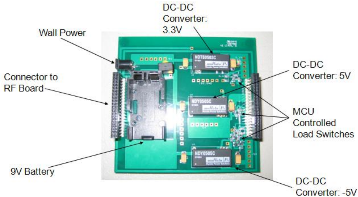
Figure 7-8: DC power board which includes wall power or power via a 9V battery. Connectors are used to directly connect the RF board shown in Figure 7-7. DC-DC converters are used to supply the RF board with +5V, -5V, and +3.3V. Load switches allow the DC power to the tag to be turned on and off and are controlled by the tag MCU. This provides the underlying time division multiple access functionality.
