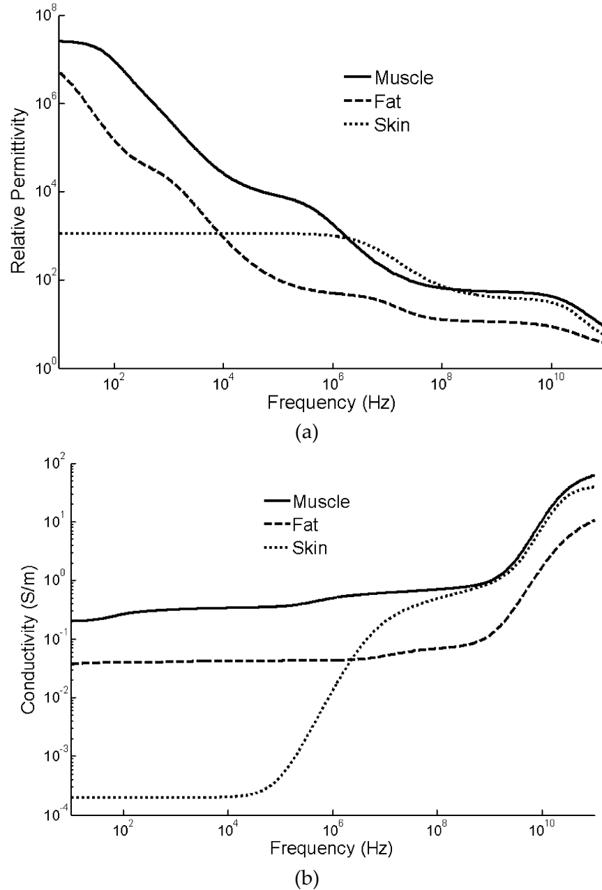
Figure 2-3: Electrical properties of human muscle, fat, and skin at 37°C. (a) relative permittivity, (b) conductivity.
