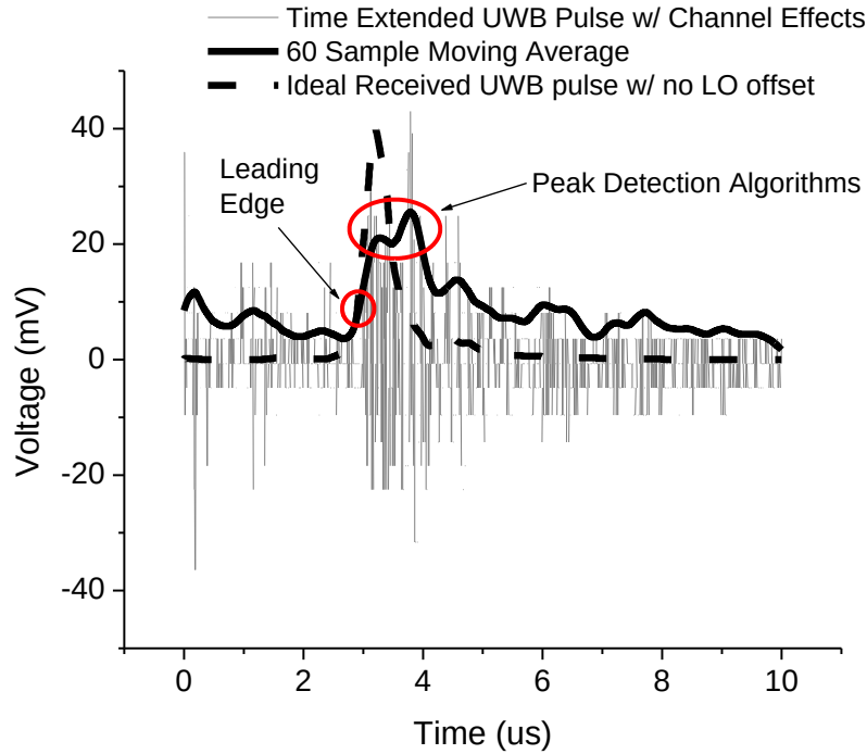
Figure 6-10: Simulated UWB time extended pulse with LO\_offset = 3\text{MHz} . IEEE 802.15.4a industrial LOS channel (CM7) effects (e.g. pathloss, multipath interference) are included to provide a realistic received signal. The system architecture in Figure 6-3 is used to capture the non-ideal performance of various system components. PRF_1 and PRF_2 are not coherent. With a smaller SNR and the addition of multipath interference and significant pathloss, a large variation in the detected peak is observed which results in gross 1-D ranging errors of up to 30 cm. The leading edge still provides accurate 1-D ranging even in this harsh environment.
