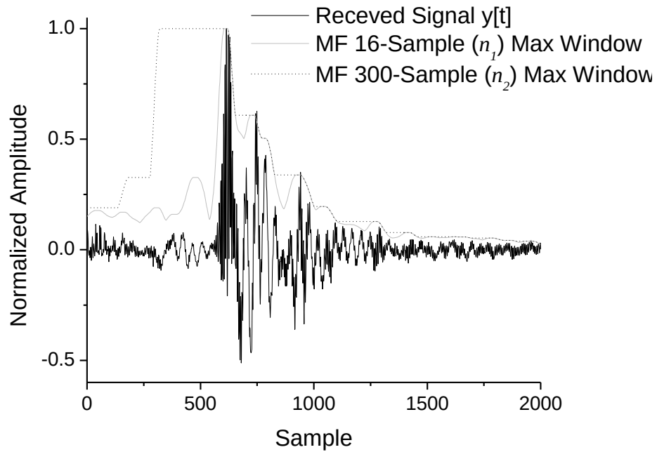
Figure 9-26: Simulated UWB received signal using the UWB IEEE 802.15.4a residential LOS channel with Tx-Rx distance of 2 m. The SNR of y[t] is 17.7dB. After applying a MF, the SNR drops to 14.4dB.
