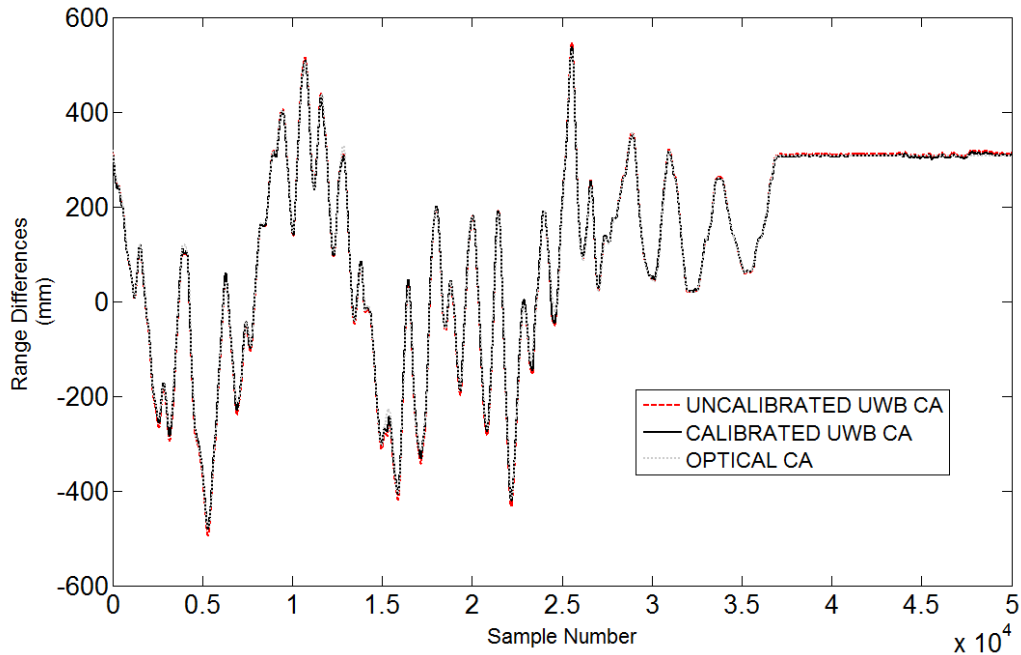
Figure 7-31: Raw range difference data for base station C minus base station A (CA) for both the optical and ultra-wideband positioning systems as the tag is moved around the view volume. The calibrated UWB range differences better fit the optical CA range differences.
