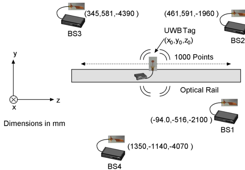
Figure 6-12: Optical rail experimental setup where four base stations are positioned at distinct 3-D locations and the UWB tag is moved along an optical rail while 1000 3-D points are taken in real-time, utilizing the UWB transmitter and receiver architectures in Figure 6-3.
