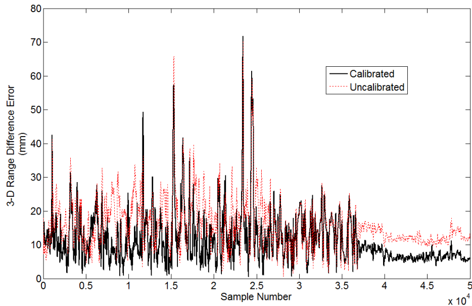
Figure 7-35: The 3-D range difference error (defined in (7-8)) for all 50,000 calibration points before and after the dynamic calibration (applying H ). The dynamic calibration provides a 26% reduction in RMS 3-D range difference error (reduced from 13.9 mm to 10.3 mm).
