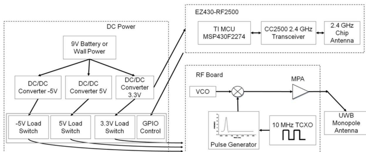
Figure 7-6: Block diagram of integrated UWB tag including the RF board containing the UWB pulse generator, VCO, mixer, and amplifier. A separate DC power board contains the DC-DC converters and load switches used to switch on and off the power to the RF board to implement the TDMA scheme.
