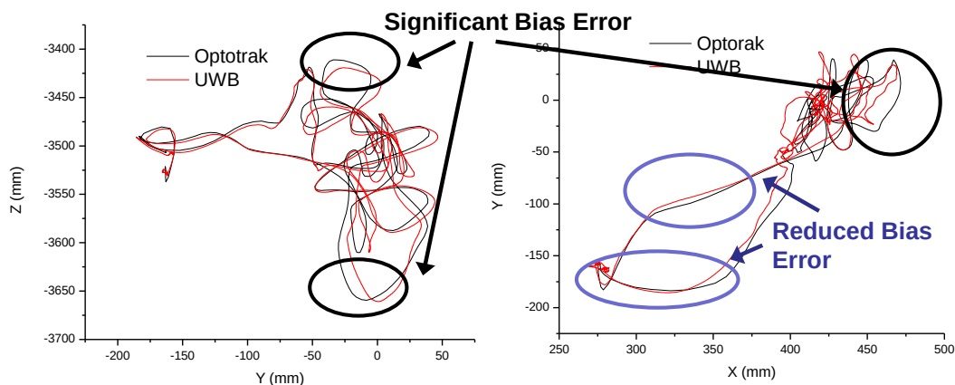
Figure 8-13. X,Y,Z cross sections with focus on significant bias error locations versus reduced bias error locations. This variation in bias error is most likely caused by dynamic base station phase center variation.
