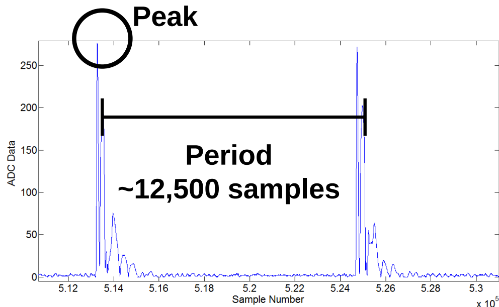
Figure 9-6: Absolute value of the received UWB pulse. The peak can easily be located by using a search window which is a substantial size of the UWB pulse period of around 12,500 digital samples. A window size of 5/8 of the period is used which equates to 7812 samples.
