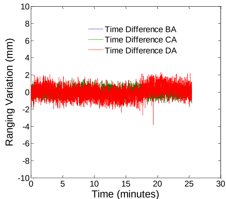
Figure 7-24: Measured receiver clock jitter and drift for a 2 nd tag using the 1 st tag as a static tag to calculate and remove the receiver clock jitter and drift. A nice Gaussian white noise is observed while the jitter and drift effects outlined in Figure 7-22 and Figure 7-23 are removed.
