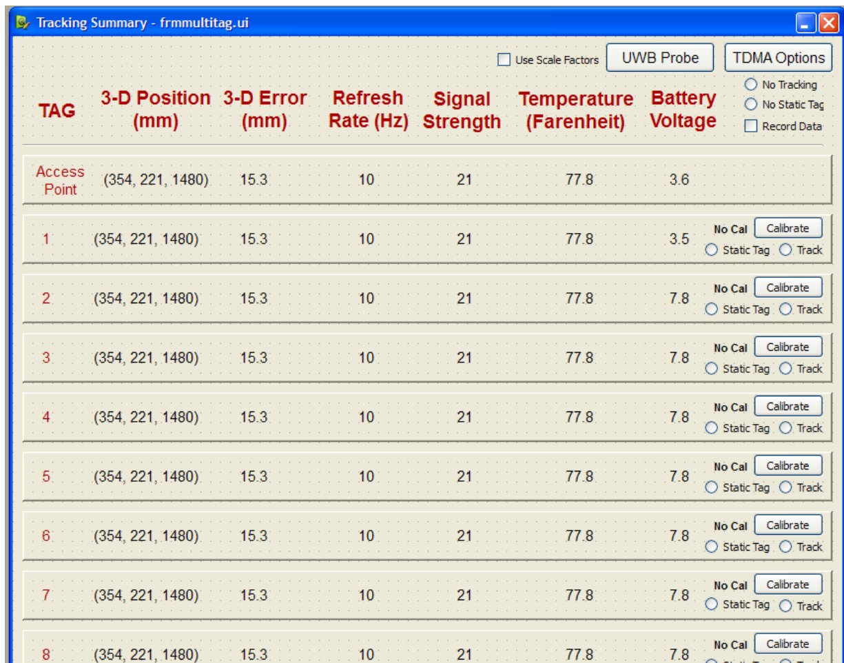
Figure 7-19: C++ software application for displaying and collecting multi-tag data. This includes information for each tag such as 3-D position, 3-D error (if being tracked by an optical tracker), refresh rate (Hz), signal strength (from 2.4 GHz MCU), temperature (from MCU), and battery voltage. Each tag can be calibrated separately. Each tag can be tracked by an optical probe. A static tag is used to filter out receiver clock jitter and drift.
