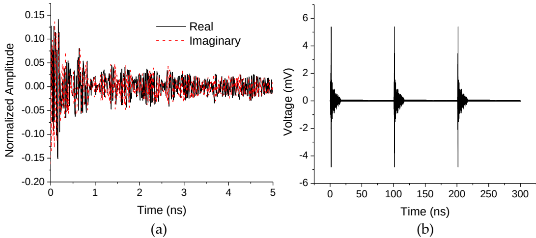
Figure 6-5: Simulated (a) complex impulse response using the IEEE 802.15.4a industrial LOS channel model, (b) pulse train with PRF_1 = 10\text{ MHz} where the transmitted signal x(t) is convolved with the channel impulse response h(t) and pathloss effects are incorporated for Tx-Rx distance of 2.5 m [178].
