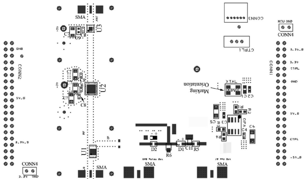
Top Layer Silk and Mask Layers
