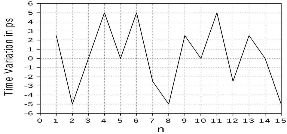
Figure 5-4: Time variation of the pulse peak position acquired over n sample points [18].
