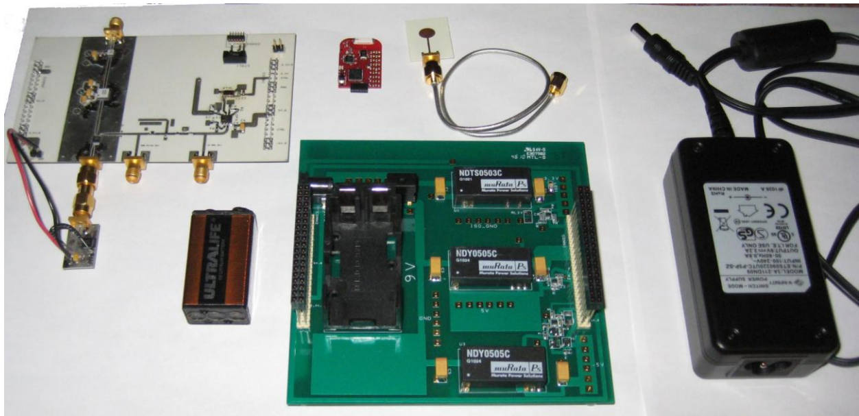
Figure 7-10: Integrated tag components including DC power board, RF board, MSP430-EZ2500 microcontroller board, VCO connected via external SMA connector, monopole UWB antenna, 9V battery, and 9V AC/DC power converter.
