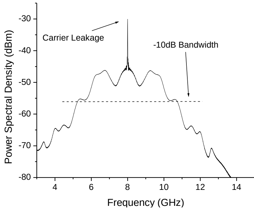
Figure 4-28: Power spectral density of simulated UWB signal showing -10 dB bandwidth from 5.4-10.6 GHz which bypasses interfering signals observed below 3 GHz. This spectrum contains the IEEE 802.11a WLAN band (5.15-5.875 GHz) as outlined in Section 4.4.
