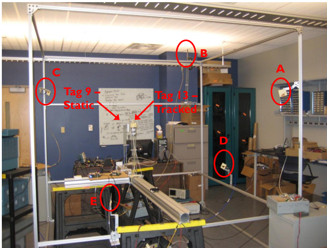
Figure 8-14. Experimental setup where dynamic (Tag 13) and static (Tag 9) tags are positioned on an optical rail. Five base stations are positioned around the tags (A,B,C,D,E) in a geometrical setup with low PDOP.
