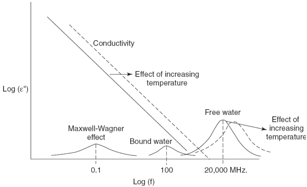
Figure 2-4: Water and temperature effects on the loss factor [78].
