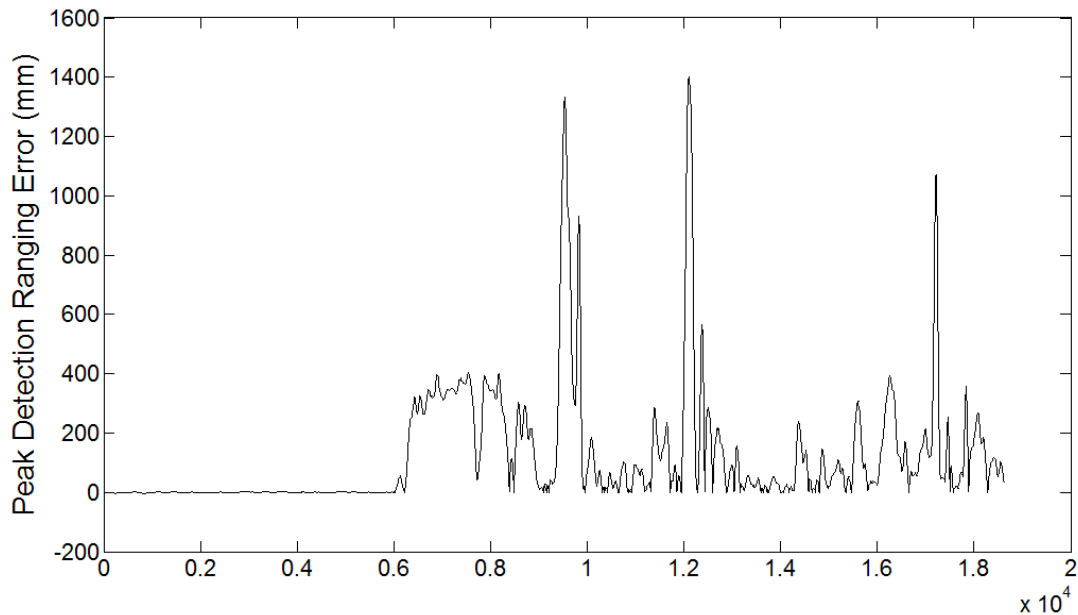
Figure 10-10: Peak detection ranging error for the poor SNR scenario outlined in Figure 10-9.
