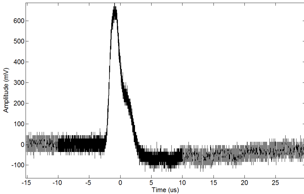
Figure 9-1: Raw received UWB pulse using a 2500x expansion factor before analog-to-digital conversion. No ringing is observed in the UWB pulse when compared to Figure 9-2.
