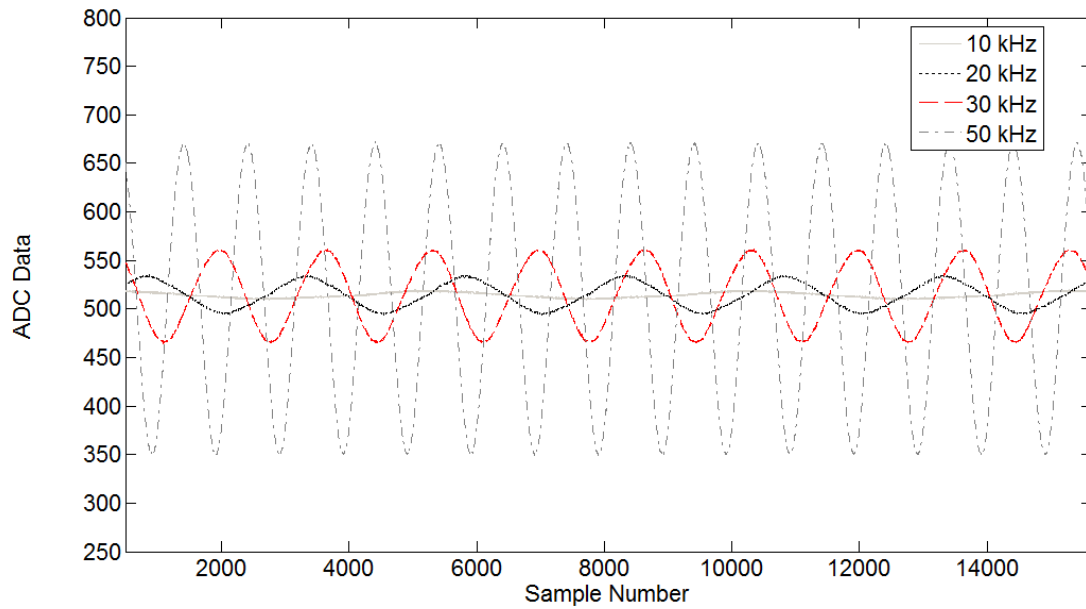
Figure 9-3: Output sine wave signals for input sine waves of 500 mVpp with frequencies of 10 kHz, 20 kHz, 30 kHz, and 50 kHz. The signals attenuate significantly when comparing 50 kHz to 10 kHz. This is the saturation effect of the RF transformer which effectively limits the input signal to a frequency bandwidth of 50 kHz and above (a high pass filter with a 50 kHz cutoff).
