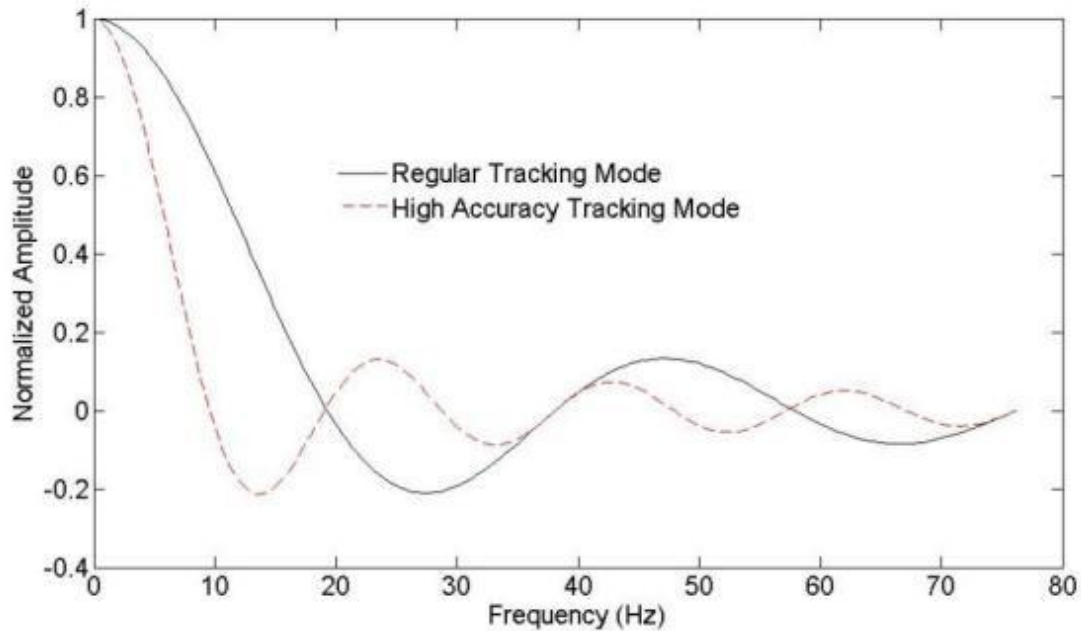
Figure 8-1. Two different sized averaging filters are applied to the 3-D UWB dynamic positioning data. The regular tracking mode detects frequencies in the 3-D motion of up to 15 Hz while the high accuracy tracking mode provides better accuracy but at the expense of detecting only 8 Hz of 3-D motion.
