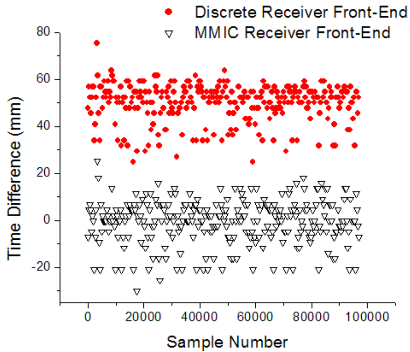
Figure 7-44. Raw time difference static data for two discrete front-end receivers versus two MMIC receivers in millimeters with MMIC data offset to zero for illustration.
