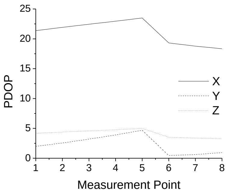
Figure 6-22: Comparison of PDOP in the x,y,z dimensions for simulating the experiment outlined in Figure 6-20d. The PDOP in the x-dimension is much greater than y,z. Also, the PDOP in the z-dimension is consistently greater than y.
