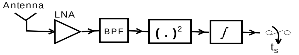
Figure 1-3: Energy detection-based UWB receiver architecture [19].
