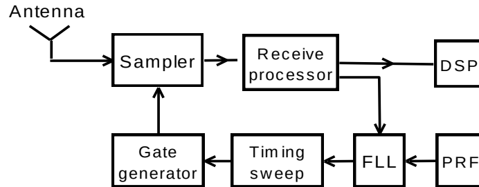
Figure 1-5: Non-coherent UWB receiver architecture using frequency locked loop [19].
