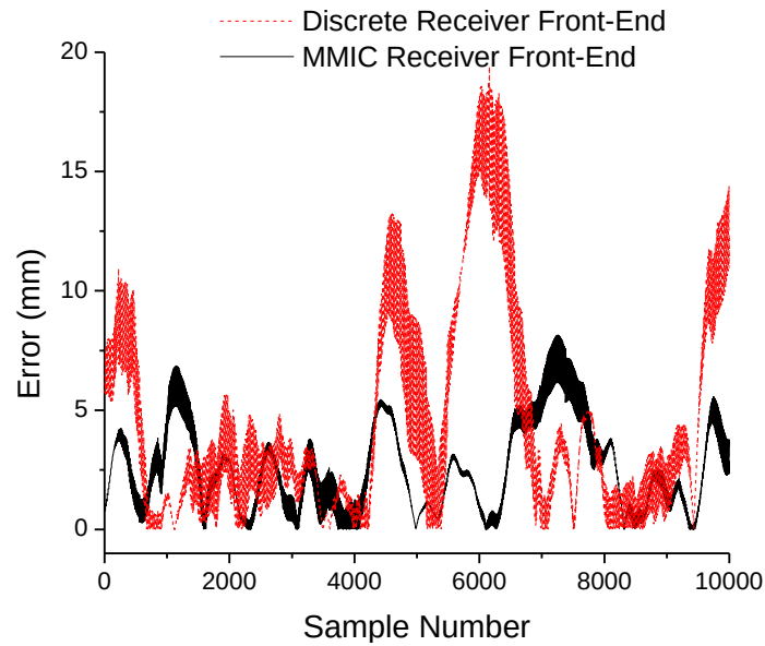
Figure 7-48. Ranging errors in the dynamic time differences shown in Figure 7-47 when comparing the UWB time difference data to the optical (ground truth) time difference data.
