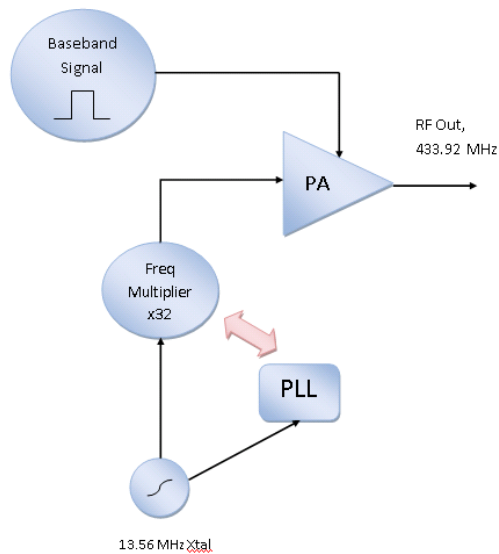
Figure 2-11: Standard ASK transmitter architecture where a digital signal modulates the RF carrier operating at 315 MHz or 433 MHz.
