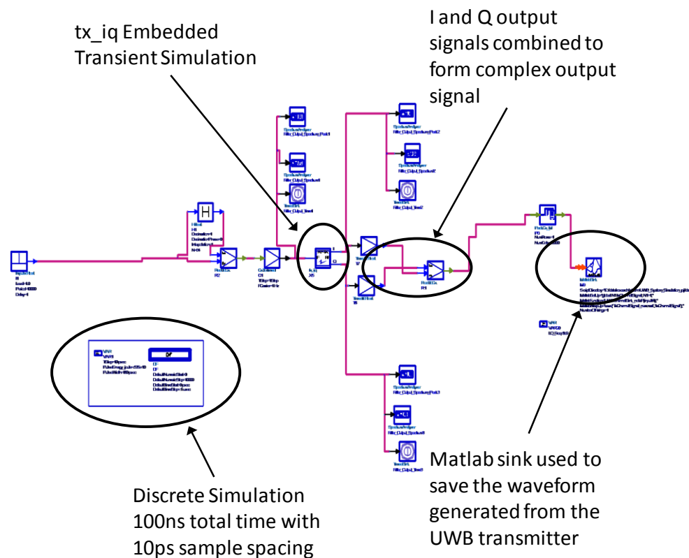
Fig. 4. Overview of transmitter_UWB_channel_RF_PG discrete time simulation which embeds the tx_iq transient simulation and formats the I and Q output signals into a complex waveform passed to a Matlab sink for processing and saving as a MAT file.
