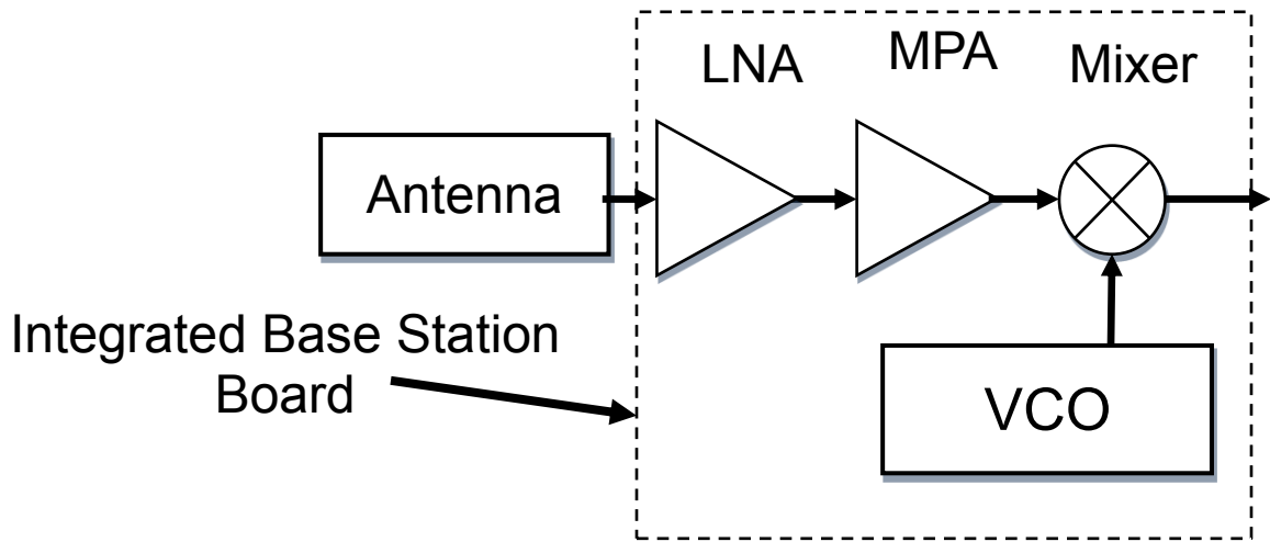
Figure 11-3: Current integrated base station where commercially available chips are used.
