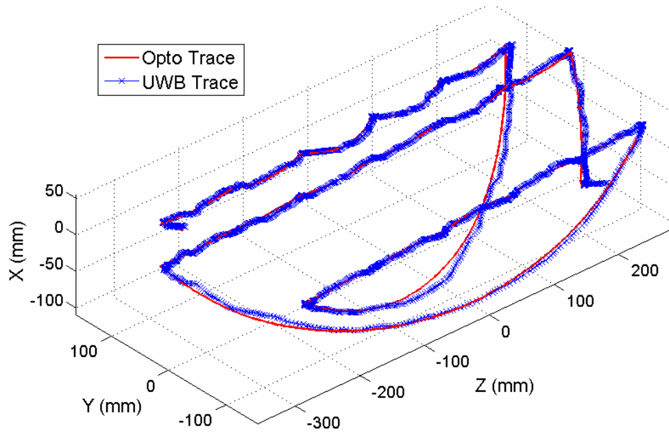
Figure 5-13: 3-D dynamic robot tracking. UWB trace compared to Optotrak trace [19].
