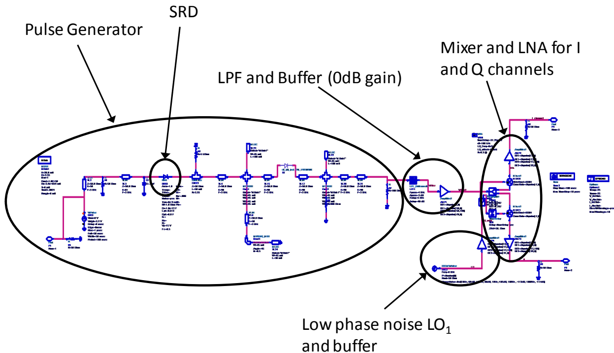
Fig. 3. Overview of tx_iq transient simulation which simulates the UWB transmitter including pulse generator, LO_1 , mixer, and LNA.
