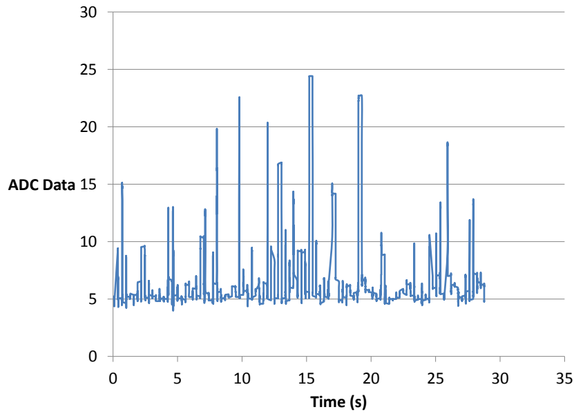
Figure 9-13: A typical noise signal measured over a time period of 30 s. Values fluctuate from 5-25 as measured by the 10-bit ADC.
