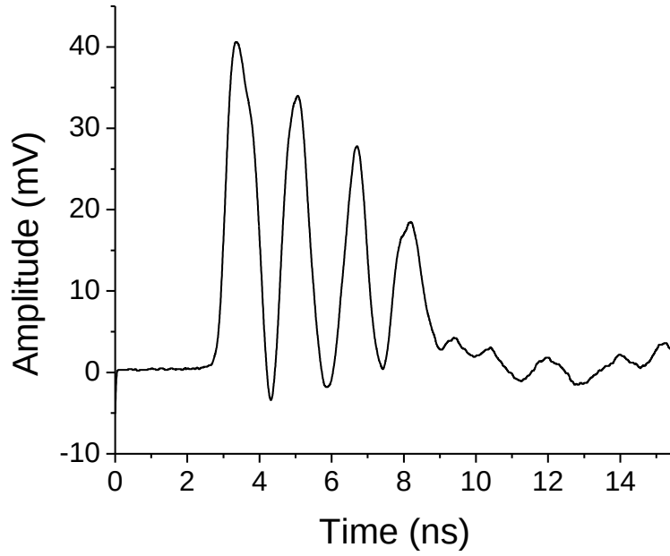
Figure 4-20: Experimental received time domain signal with noticeable multipath interference caused by metal tables and walls in the operating room.
