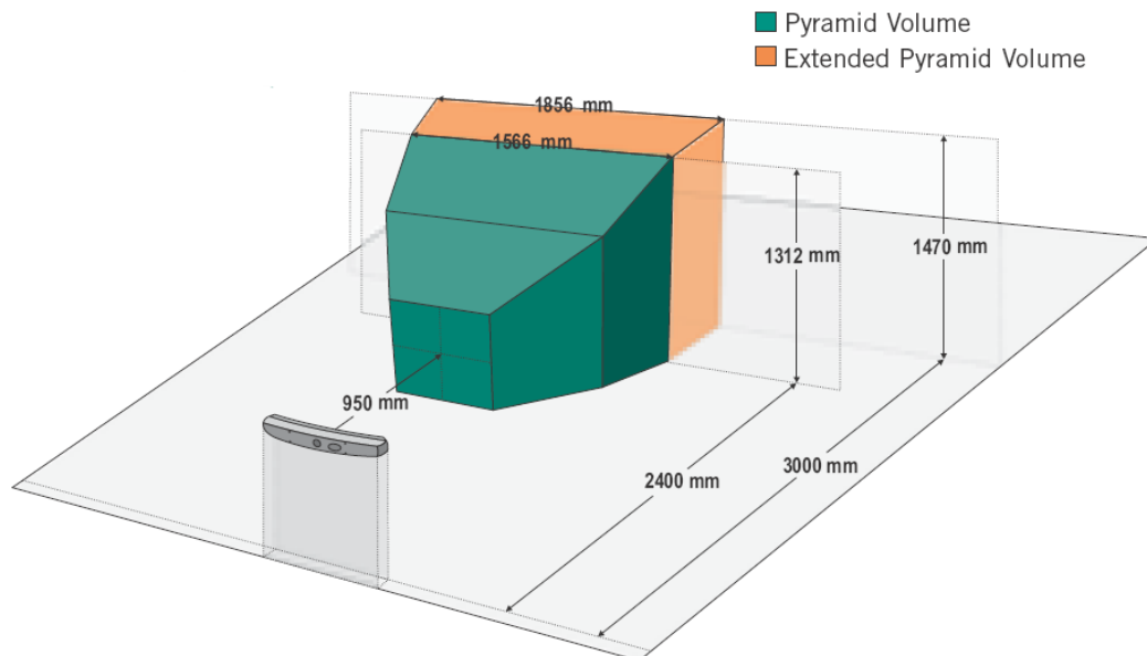
Figure 3-3: NDI Polaris Spectra view volume with 2.050 m in the z-direction and an in-plane area of 1.856 \times 1.470 \text{ m}^2 at a z distance of 3.000 m [98].
