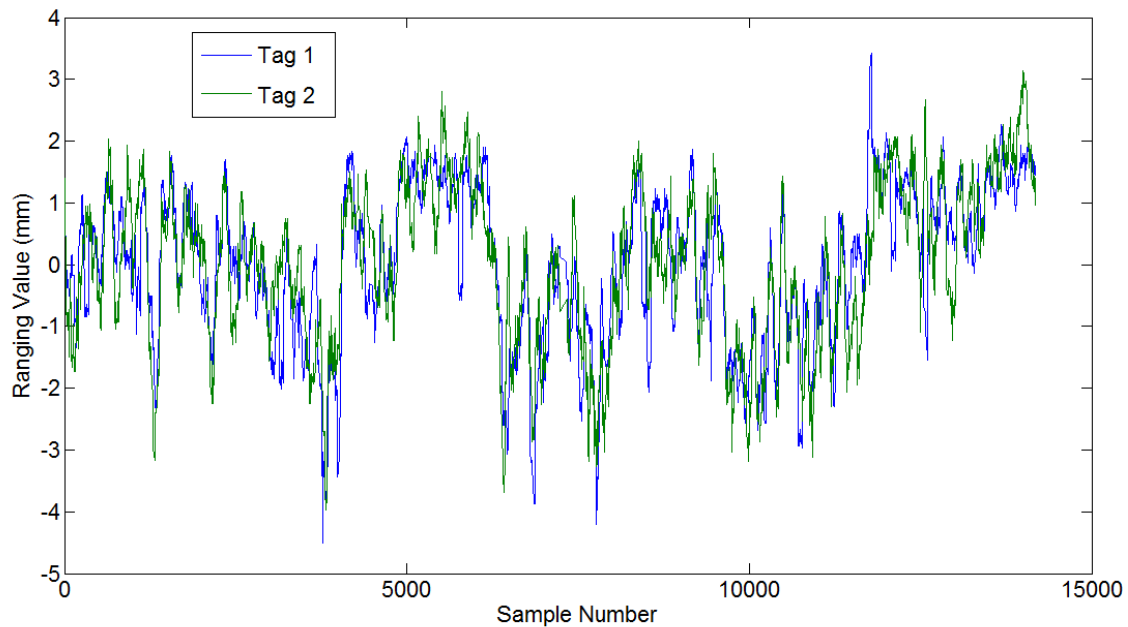
Figure 7-23: Received signal over 15000 samples (20-30 seconds) for one range difference for two different tags in static locations. The jitter and drift observed in the two signals correlates well, indicating that the main source of clock jitter and drift is from the UWB receivers and is therefore similar across all tags.
