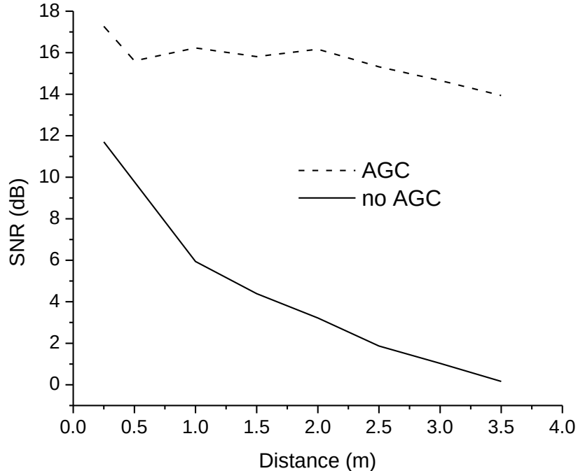
Figure 6-23: SNR of received UWB pulse vs. distance between transmitter and receiver with and without automatic gain control.
