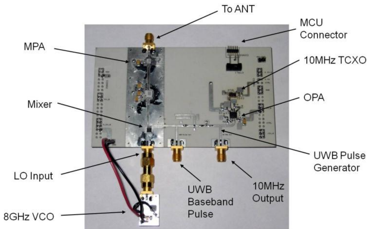
Figure 7-7: Integrated tag RF board including 10 MHz clock, high slew rate op amp, step recovery diode pulse generator, mixer, VCO, and medium power amplifier. A 6-pin connector is used to connect the MCU board to the RF board.
