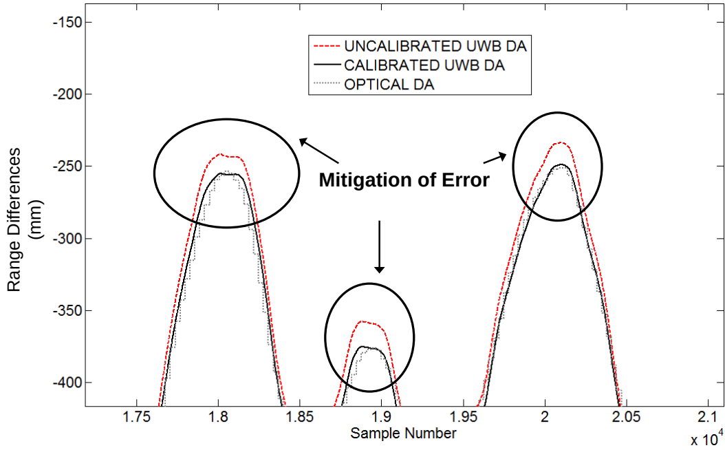
Figure 7-34: A zoomed-in view of the raw range difference data for base station D minus base station A (DA) for both the optical and ultra-wideband positioning systems as the tag is moved around the view volume. The calibrated UWB range differences have a 6.3% scale reduction which provides a noticeably better fit to the optical range difference data, especially at the extremities of the view volume.
