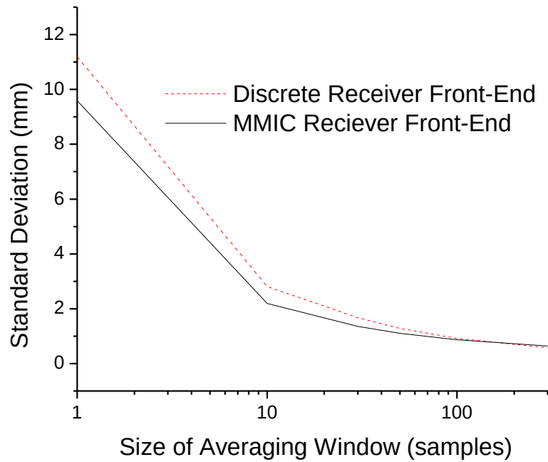
Figure 7-46. Standard deviation of static time differences comparing two discrete receiver front-ends to two MMIC receiver front-ends with a variable averaging window size.
