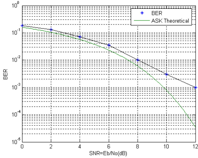
Figure 4-8: Theoretical and simulated BER of the ASK system.
