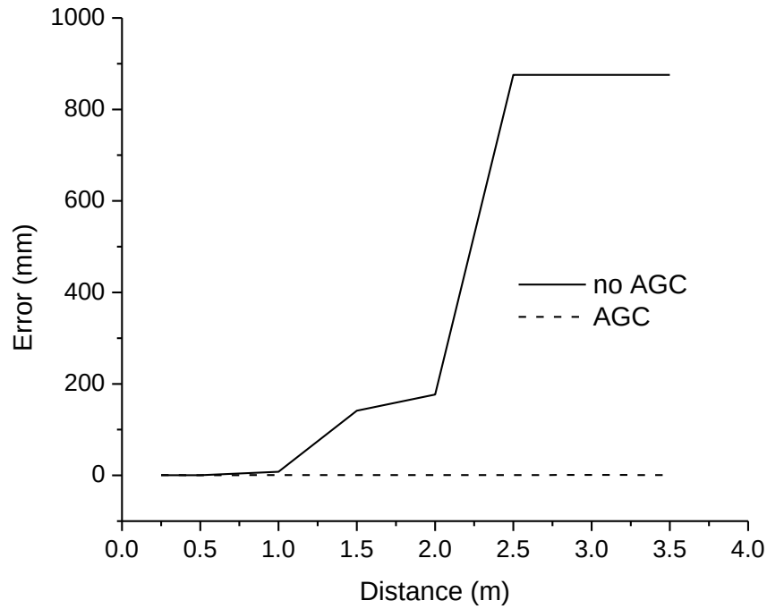
Figure 6-26: Simulated leading-edge detection 1-D error vs. distance between transmitter and receiver in the industrial LOS channel with and without automatic gain control.
