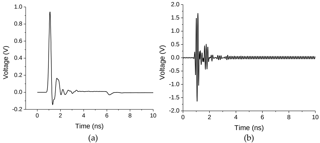
Figure 6-4: Simulated (a) baseband Gaussian pulse generated from a SRD, (b) modulated UWB pulse after passing through the transmitter chain outlined in Figure 6-3 including the monopole UWB antenna, denoted x(t) .
