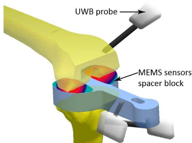
Figure 3-19: Illustration of the MEMS spacer block integrated with the UWB positioning system for 3-D real-time tracking. UWB probes are rigidly fixed to the femur and tibia to track the bones in real-time. A UWB probe is also rigidly attached to the spacer block to track it in real-time.
