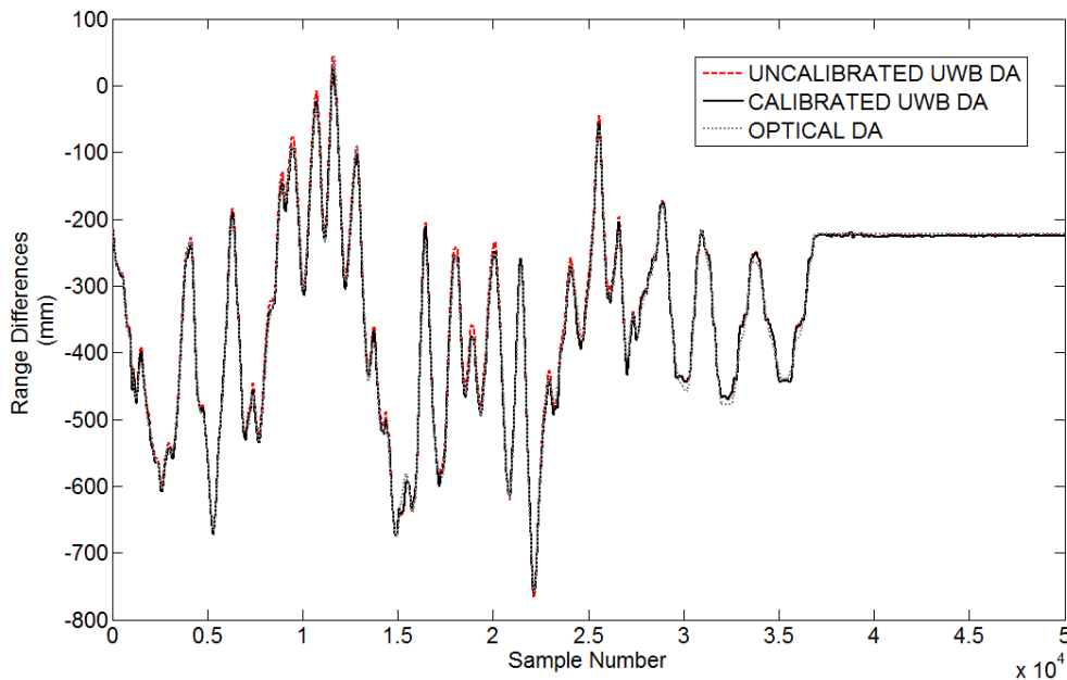
Figure 7-33: Raw range difference data for base station D minus base station A (DA) for both the optical and ultra-wideband positioning systems as the tag is moved around the view volume. The calibrated UWB range differences better fit the optical DA range differences.
