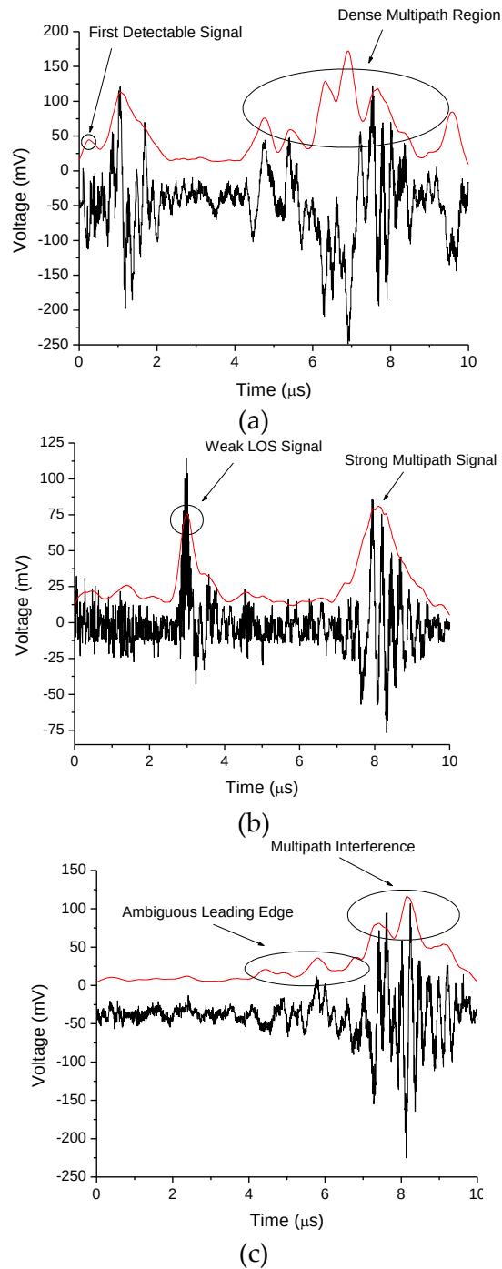
Figure 6-17: Examples of received signals. (a) CM8 received signal highlighting the need to detect the first signal above the noise floor instead of trying to resolve the arrival of the peak in the dense multipath region. (b) CM4 received signal highlighting the weaker LOS signal which still provides accurate ranging compared to the strong multipath signal. (c) CM2 received signal where the leading edge is distorted. Since the multipath signals can be resolved, iterative peak subtraction or a matched filter provides the best performance.
