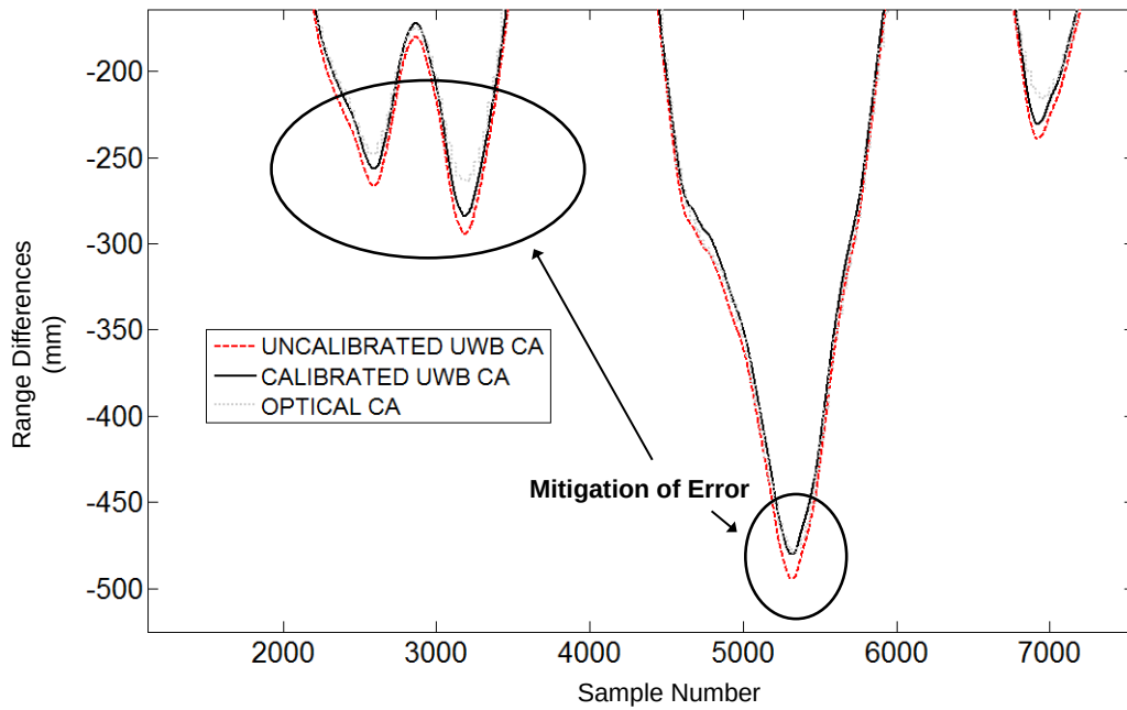
Figure 7-32: A zoomed-in view of the raw range difference data for base station C minus base station A (CA) for both the optical and ultra-wideband positioning systems as the tag is moved around the view volume. The calibrated UWB range differences have a 2.8% scale reduction which provides a noticeably better fit to the optical range difference data, especially at the extremities of the view volume.
