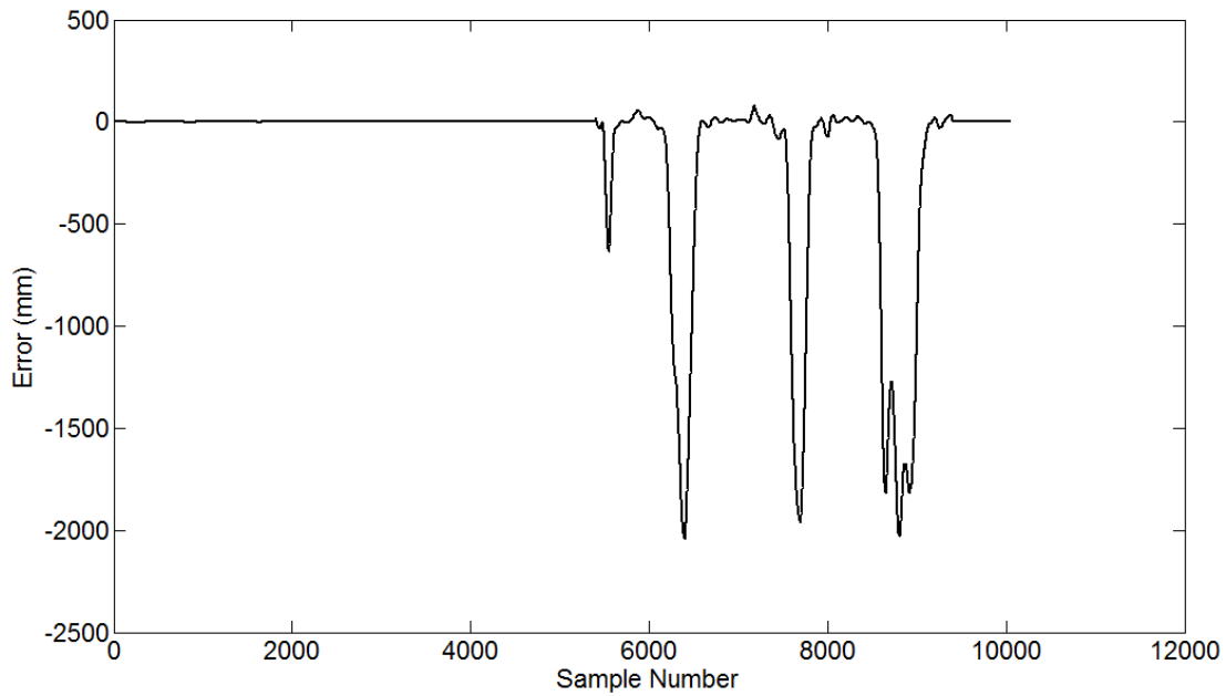
Figure 10-6: Range difference corresponding to the UWB base station where the NLOS blockage occurred. Extremely large ranging errors are observed on the order of two meters.
