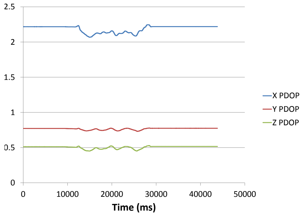
Figure 8-19. PDOP data for a four base station optical rail experiment showing the PDOP in X,Y,Z. The total PDOP is 2.40 ( X=2.22, Y=0.77, Z=0.50 ).
