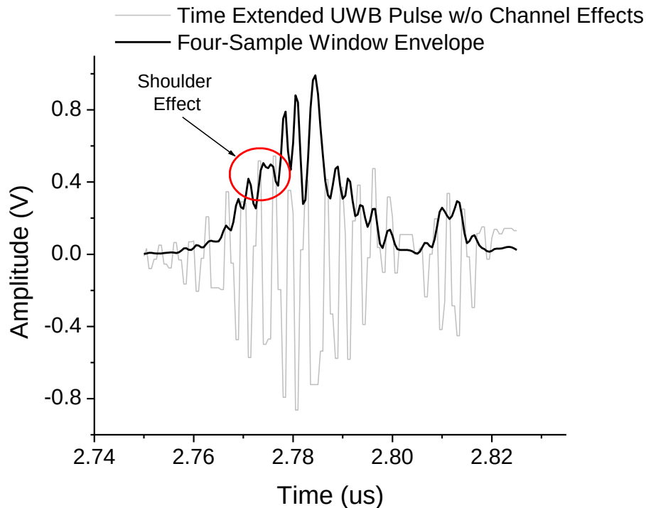
Figure 6-11: Simulated UWB time extended pulse with LO\_offset = 3\text{MHz} . A zoomed-in portion of Figure 6-9 is shown to highlight the shoulder effects caused by carrier leakage in the time extended received signal.
