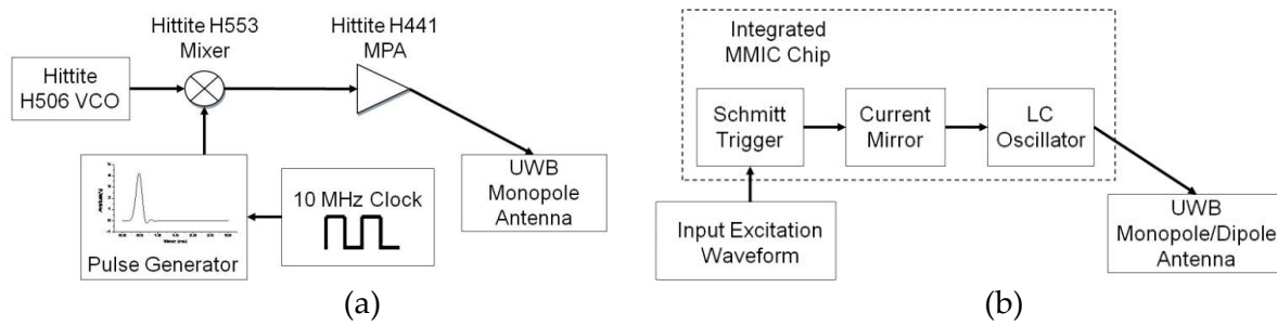
Figure 7-39. Block diagram of UWB transmitter front-ends: (a) discrete, (b) integrated into a MMIC chip [221].
