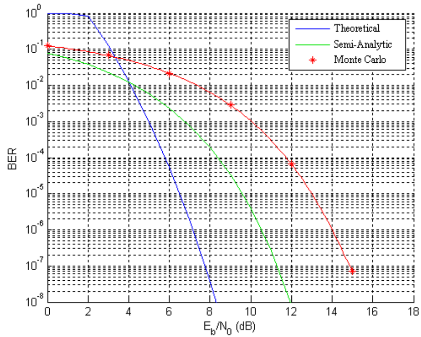
Figure 4-9: Comparison of theoretical, semi-analytic, and Monte Carlo methods for computing the BER of the 433 MHz ASK system.
