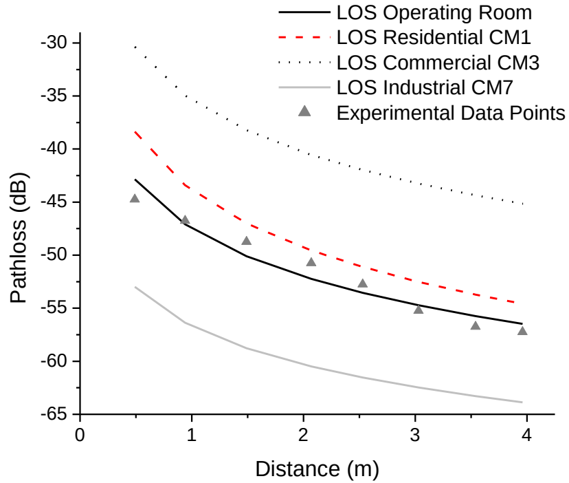
Figure 4-18: Comparison of pathloss for IEEE 802.15.4a LOS channels. The pathloss for the OR environment is most similar to residential LOS [141].
