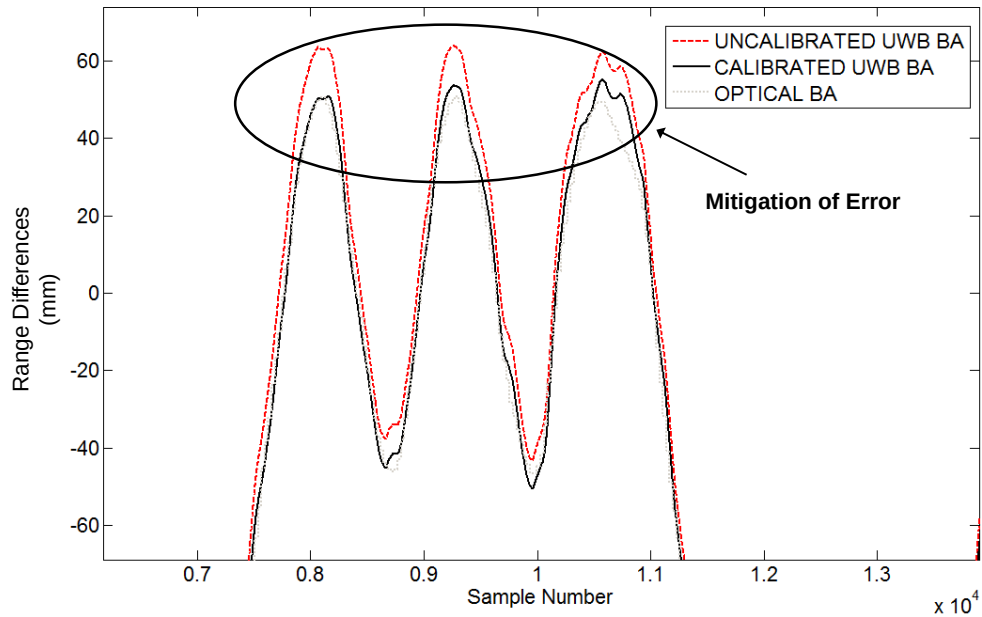
Figure 7-30: A zoomed-in view of the raw range difference data for base station B minus base station A (BA) for both the optical and ultra-wideband positioning systems as the tag is moved around the view volume. The calibrated UWB range differences have a 5.8% scale reduction which provides a noticeably better fit to the optical range difference data, especially at the extremities of the view volume.
