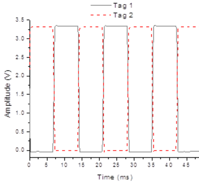
Figure 7-16: MCU control signals for tags 1 and 2 over a 50 ms time period broken into 7 ms transmitting intervals for each tag.
