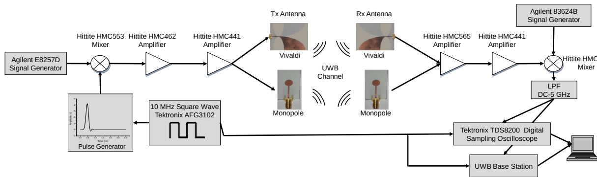
Figure 4-12: Experimental setup to collect time domain data in the operating room with the UWB localization system.
