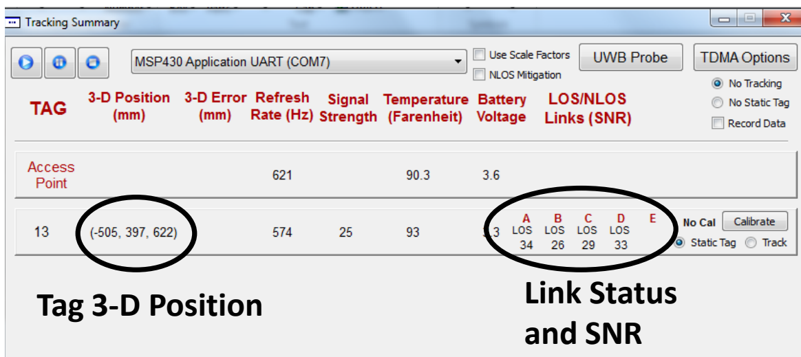
Figure 10-2: Software application where 3-D tag position and base station link status (LOS versus NLOS) and base station SNR are displayed and output to a CSV file in real-time.
