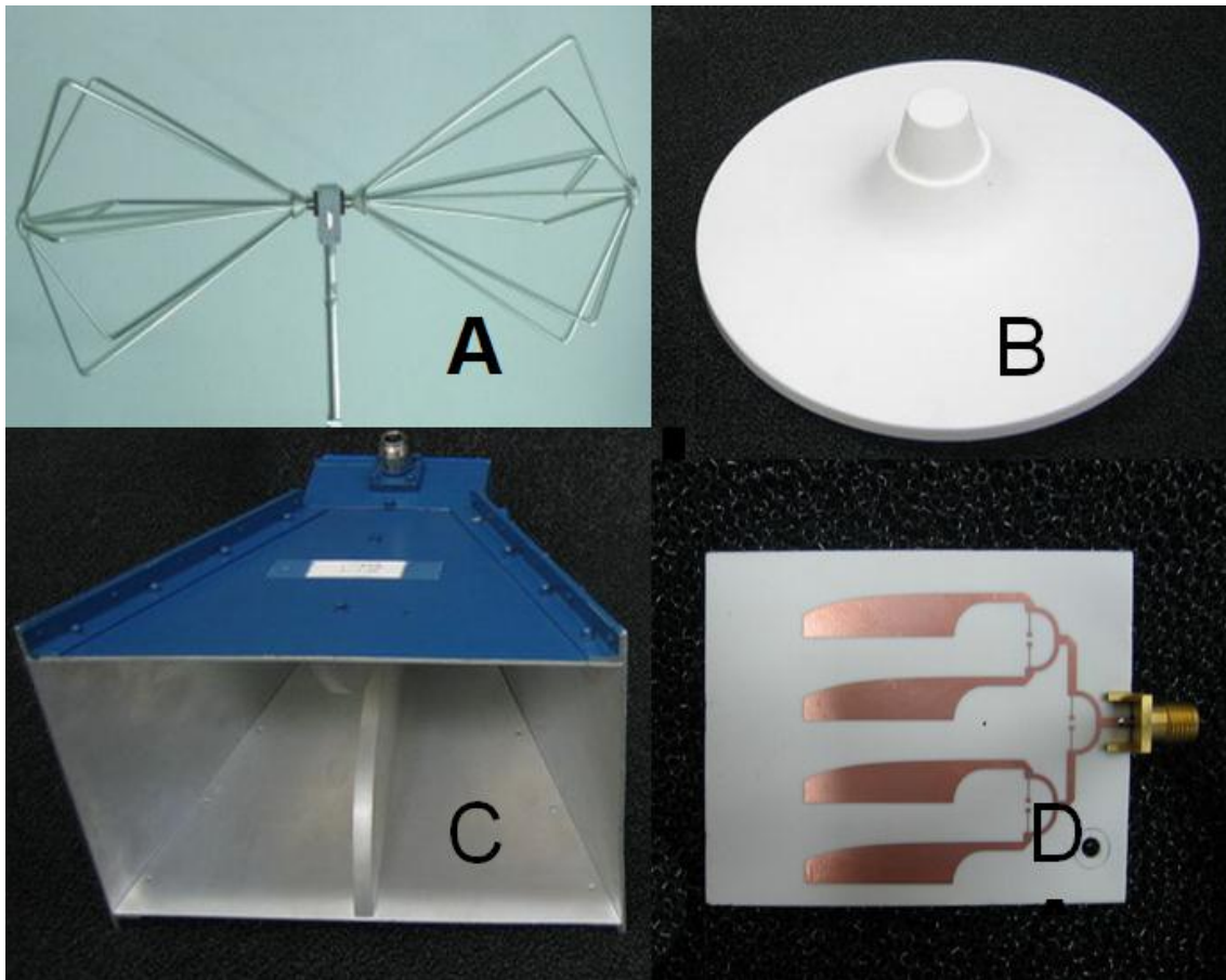
Figure 4-24: Antennas used in OR measurements: a) biconical, b) multiband disc, c) broadband TEM horn, d) 4-element Vivaldi array.
