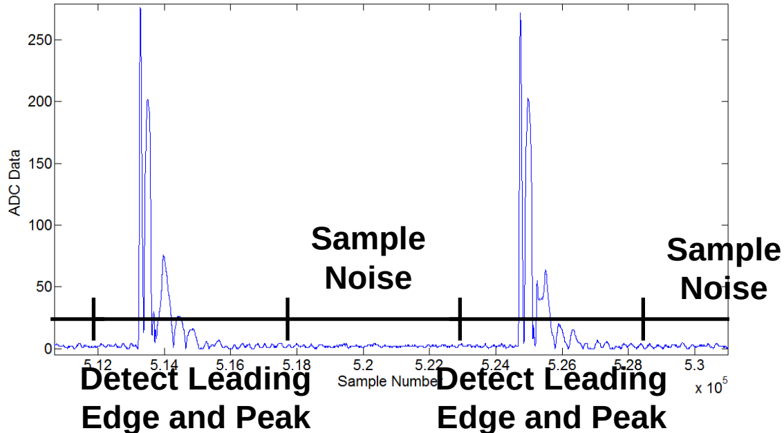
Figure 9-12: Received UWB pulse peak triggering process where a window is first allocated for peak and leading-edge detection followed by a separate time window allocated for noise sampling and estimation.
