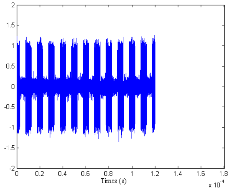
Figure 4-4: ASK signal at transmitter with the addition of AWGN.
