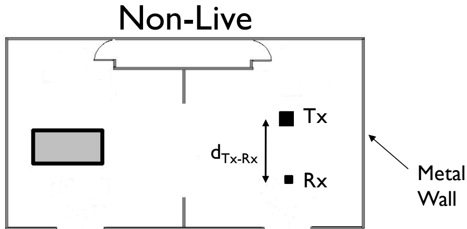
Figure 4-15: Layout of dual operating room without surgery taking place where medical equipment, glass walls, and the patient table have been removed. The Tx and Rx were placed in the surgical area and moved from 0.5-4 m apart.
