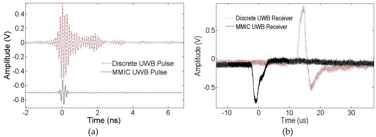
Figure 7-43. Experimental signals: (a) transmitted UWB pulse, (b) received UWB pulse after subsampling.
