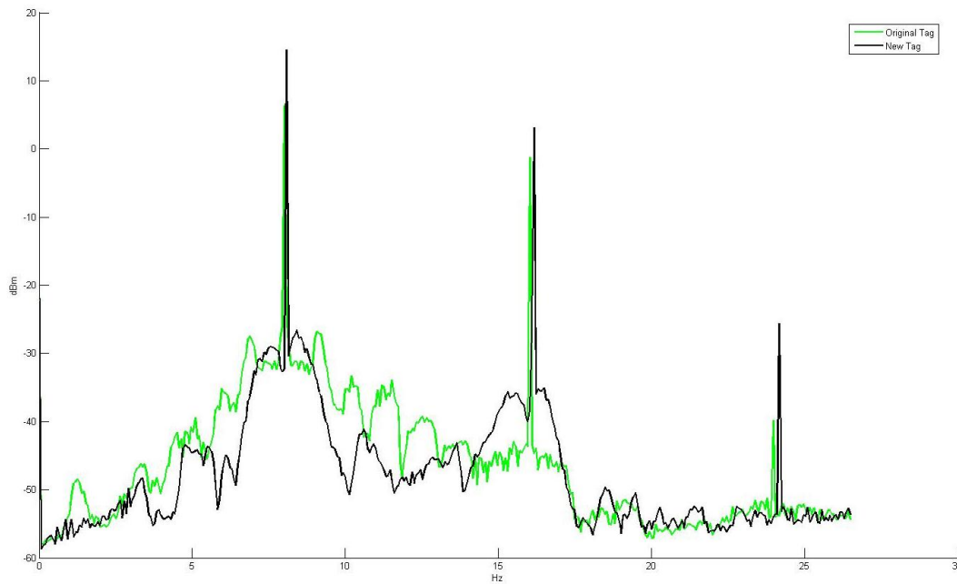
Figure 7-12: Upconverted UWB pulse in the frequency domain: integrated tag (black), discrete tag (green).
