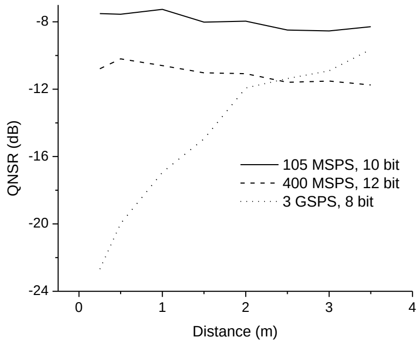
Figure 6-25: QNSR of received UWB pulse vs. distance between transmitter and receiver for three ADCs without AGC: 105 MSPS, 400 MSPS, and 3 GSPS.
