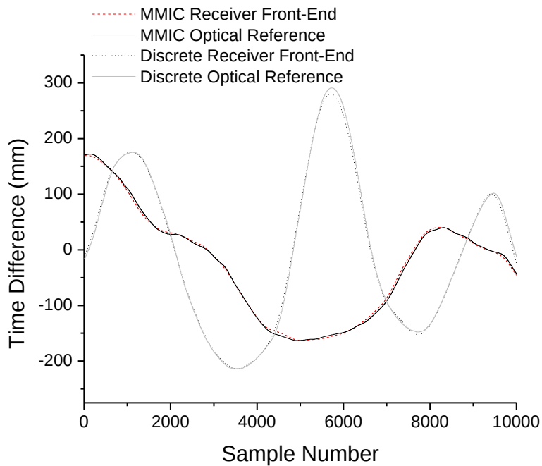
Figure 7-47. Dynamic time differences in millimeters as the tag is moved freely in the view volume comparing two discrete and two MMIC receiver front-ends. An optical tracking system provides 3-D real-time reference data.
