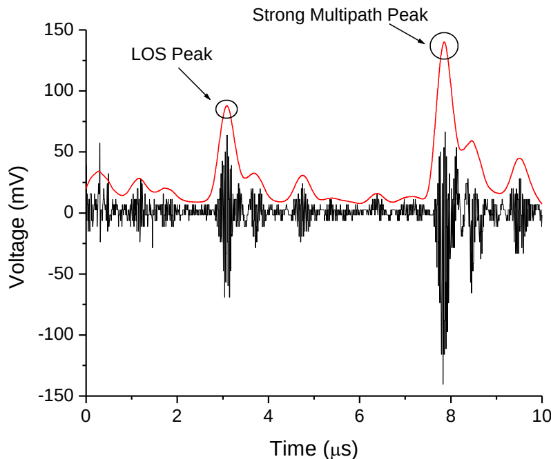
Figure 6-16: Simulated CM3 signal obtained at the UWB receiver for Tx-Rx distance of 1 m after time extension from the sampling mixer and conversion to digital. The LOS peak is highlighted as well as a strong multipath peak which arrives 4 \mu s after the LOS peak and causes a 1-D ranging error of 1.2 m using matched filter, iterative peak subtraction, and signal strength peak detection algorithms.
