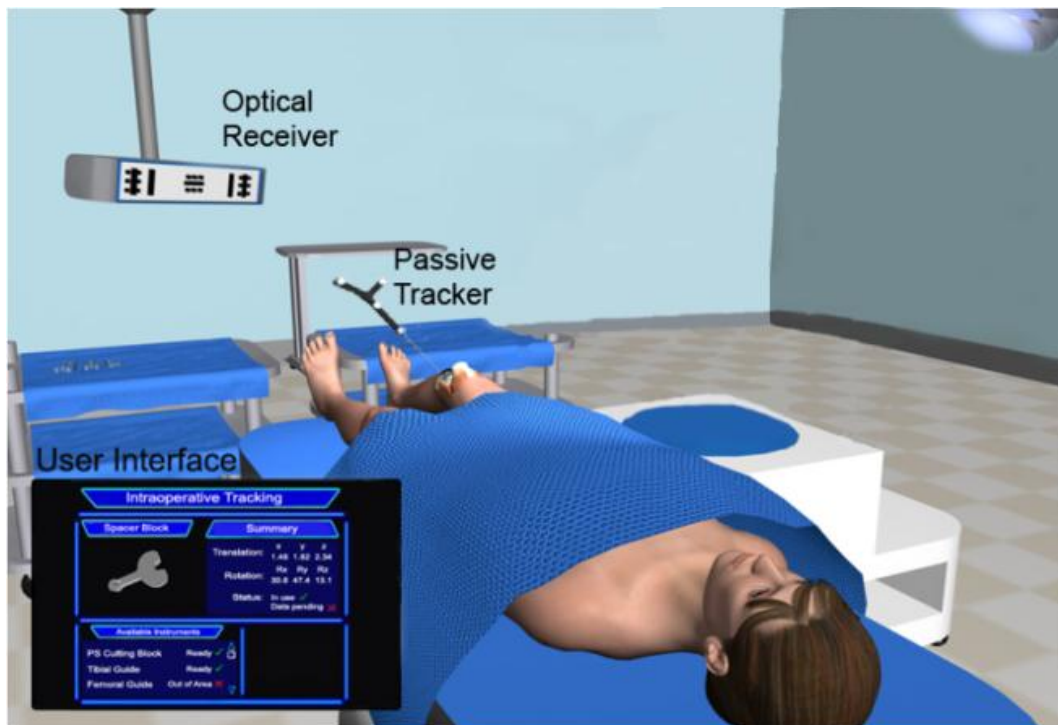
Figure 3-7: CAS system where optical tracking is utilized to assist in a TKR.
