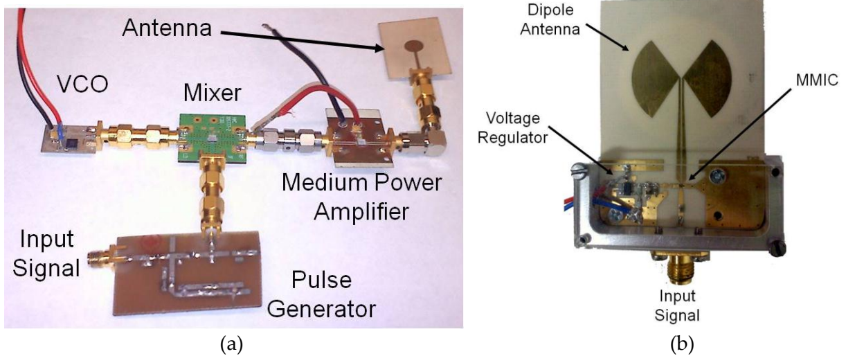
Figure 7-40. UWB transmitter front-ends: (a) discrete, (b) integrated into a MMIC chip [221].
