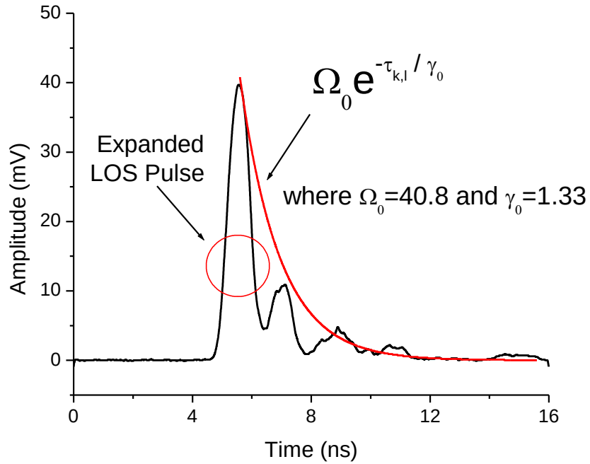
Figure 4-21: Example received signal in the time domain for a Tx-Rx distance of 1.49 m highlighting the distortion (seen as expansion) in the LOS pulse due to a dense cluster of multipath rays. The overlaid exponential is fit using \gamma_0 as outlined in Table 4-2 to show the intra-cluster decay of the LOS cluster.
