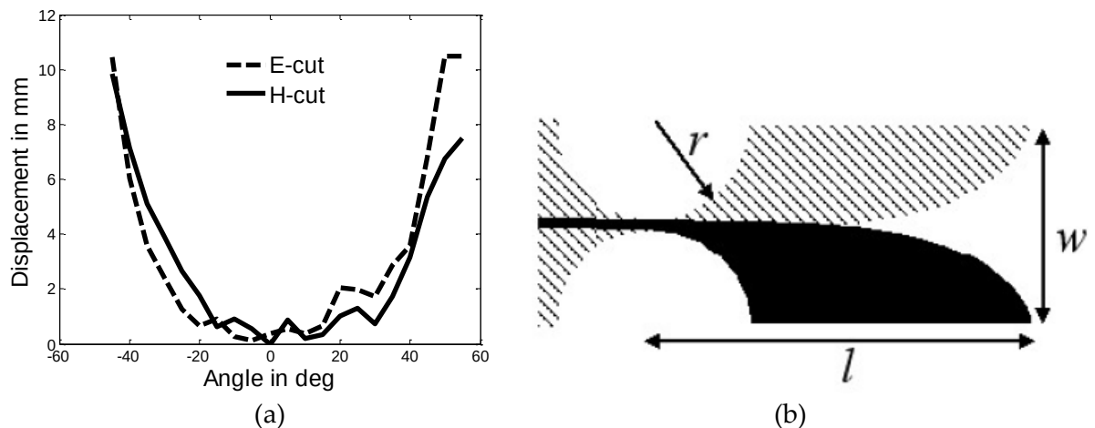
Figure 11-1: (a) Experimentally measured phase center variation of single element Vivaldi antenna in receiving an up-converted UWB pulse (5.4-10.6 GHz bandwidth), (b) single element Vivaldi antenna.
