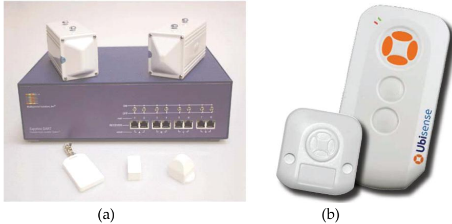
Figure 1-2: Commercial indoor UWB localization systems (a) Zebra Technologies Corporation, (b) UbiSense.
