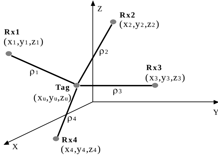
Figure 5-9: Calculation of tag position based on TDOA approach.
