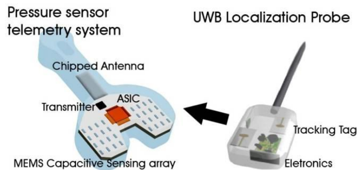
Figure 3-18: Illustration of a smart surgical tool. The spacer block, with embedded pressure sensing-telemetry system, is tracked in 3-D by an UWB localization probe.
