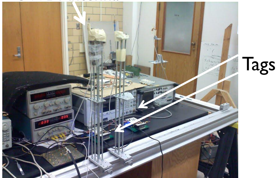
Figure 8-4. Experimental setup for optical rail experiments where one tag serves as the static tag while the other tag is moved along the optical rail with an infrared 6 DOF probe rigidly attached to it.
