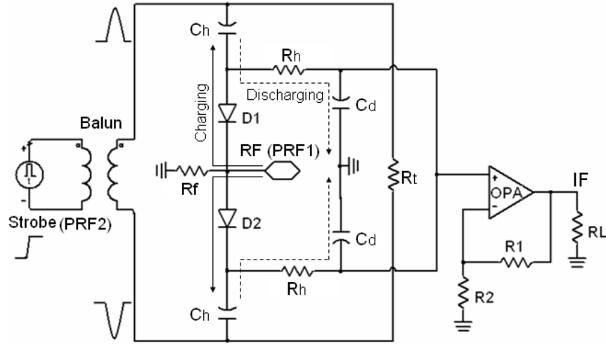
Figure 5-3: Schematic of the sampling mixer highlighting the broadband balun and balanced topology [38].
