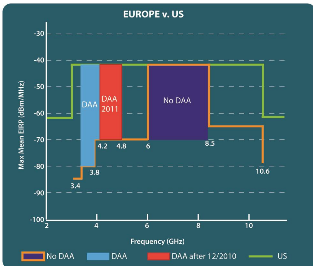
Figure 2-1: Comparison of allocated UWB bands between 3-11 GHz in the U.S. versus Europe.
