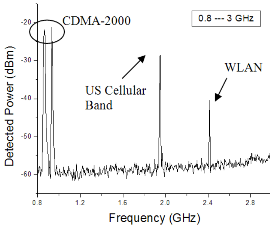
Figure 4-26: Measured EMI over frequency range of 800 MHz – 3 GHz.
