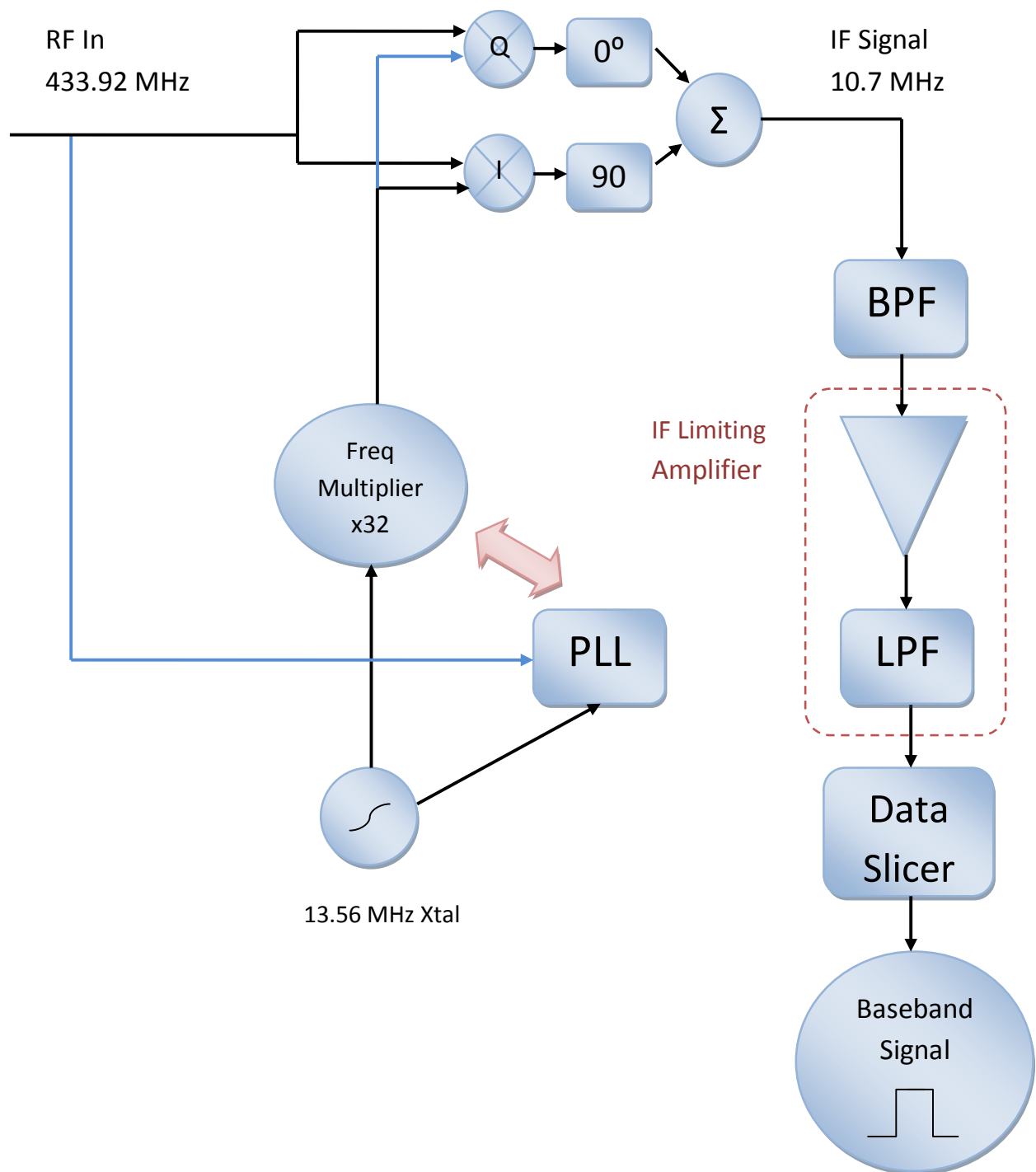
Figure 4-2: Block diagram of the MAX1473 ASK receiver.
