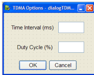
Figure 7-20: Time division multiple access parameters can be configured in the software and distributed to all tags via the 2.4 GHz communication link. This includes time interval (per tag, one time slice) and duty cycle which it is turned on within that time interval as a percentage.
