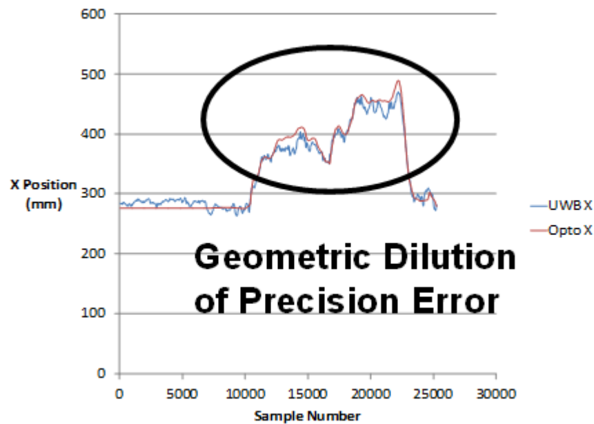
Figure 8-10. X position of Tag 10 in a dynamic freeform experiment where increased error and instability caused by a high geometric dilution of precision in the X direction can be seen.
