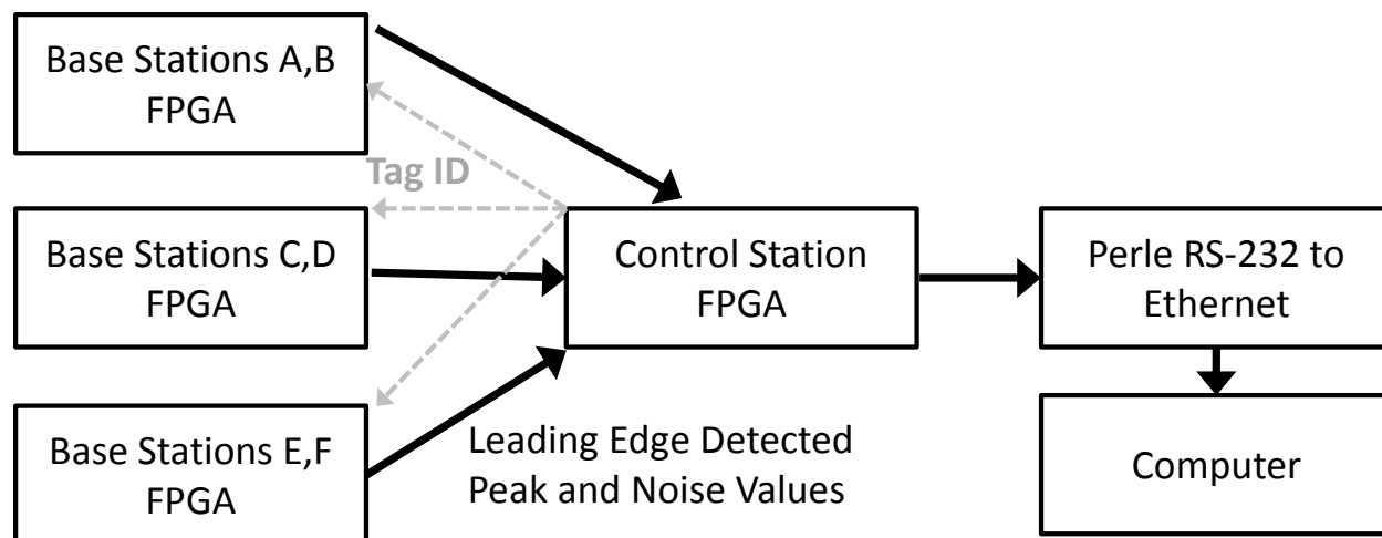
Figure 9-18: Block diagram of complete digital processing system which includes three 2-channel base station FPGAs which communicate with the control station FPGA when a leading-edge is detected for either channel. The data is transmitted from the control station FPGA through a Perle RS-232 to Ethernet converter to the computer.
