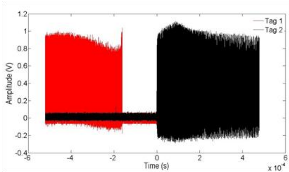
Figure 7-17: Baseband UWB pulse trains for tags 1 and 2 where a 160 \mu s latency occurs between turning off and on tags 1 and 2. Obtained by an 8 GHz real-time sampling oscilloscope.
