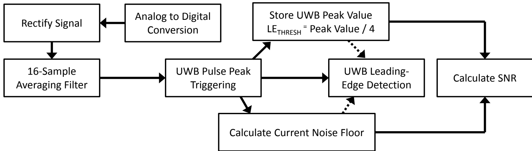
Figure 9-11: Leading-edge detection algorithm implemented on the base station FPGA which uses a rectified signal which undergoes a 16-sample averaging filter. This signal is used in triggering the algorithm off of the UWB pulse peak. The peak value is used to set the leading-edge detection threshold. The noise floor is calculated as discussed in Section 9.4. Finally, the peak and noise values are used to calculate the UWB SNR.
