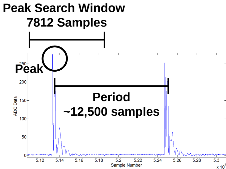
Figure 9-7: Absolute value of the received UWB pulse. The peak search window is 7812 samples or 5/8^{\text{th}} of the overall UWB pulse period of 12,500 samples.
