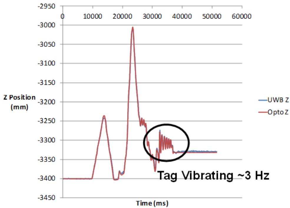
Figure 8-2. 3-D dynamic experiment where UWB and optical systems are calibrated together. A 3 Hz vibration of the tag as it is placed back on the optical rail is detected by both the UWB and optical tracking systems. These results are for Tag 13.
