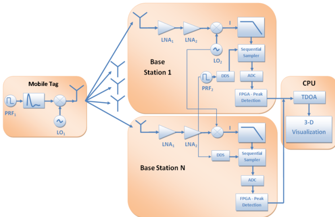
Figure 5-1: System architecture of UWB positioning system which includes a carrier-based transmitted signal at the tag and LO down-conversion and leading-edge detection at the UWB receiver.
