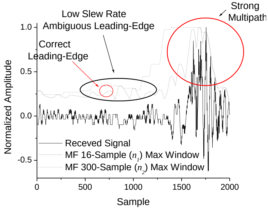
Figure 9-21: Simulated UWB received signal using the UWB IEEE 802.15.4a residential NLOS channel. The low slew rate of the NLOS leading-edge is highlighted as well as the strong multipath interference which arrives almost 1000 samples after the original weak LOS signal.
