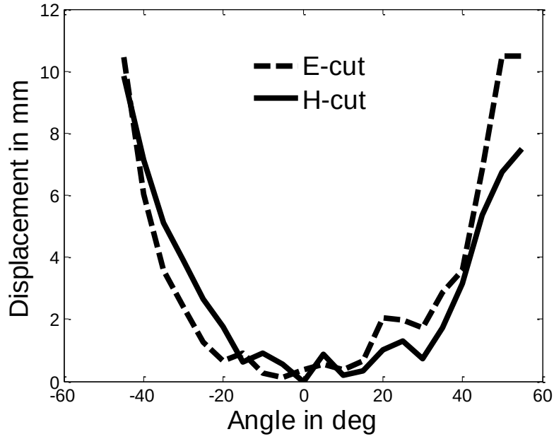
Figure 5-8: Measured Vivaldi phase center error versus angle for E-cut and H-cut.
