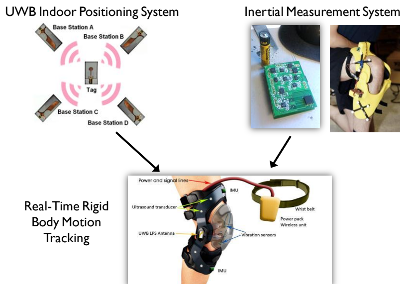
Figure 12-2: Integration of the ultra-wideband positioning system and inertial measurement systems for highly accurate real-time 3-D tracking of rigid bodies for applications such as real-time tracking of the tibia and femur.
