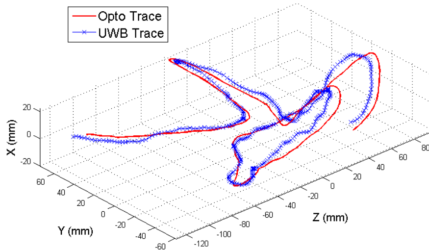
Figure 5-11: 3-D dynamic random mode with energy detection. UWB trace is compared to Optotrak trace [19].
