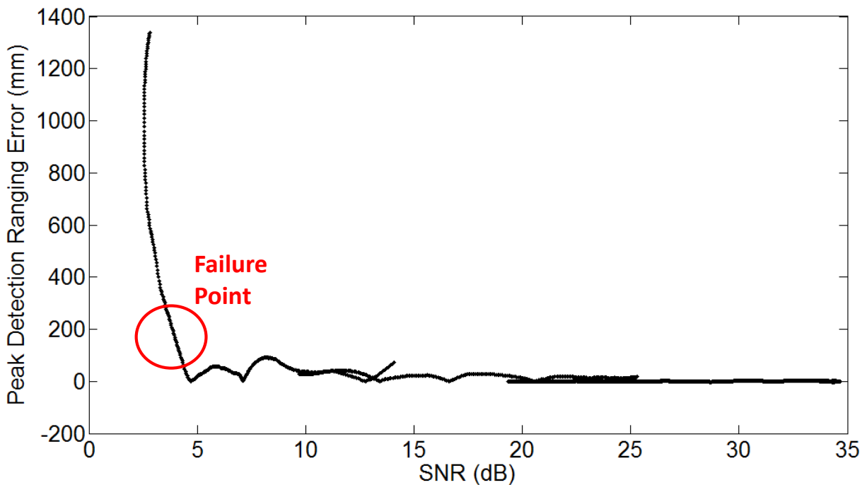
Figure 10-11: Peak detection algorithm ranging error for one base station versus SNR from the experimental results outlined in Figure 10-9 and Figure 10-10. The peak detection algorithm fails when the SNR reaches 4-5 dB. This is a 6-7 dB improvement over the leading-edge detection algorithm as shown in Figure 10-7.
