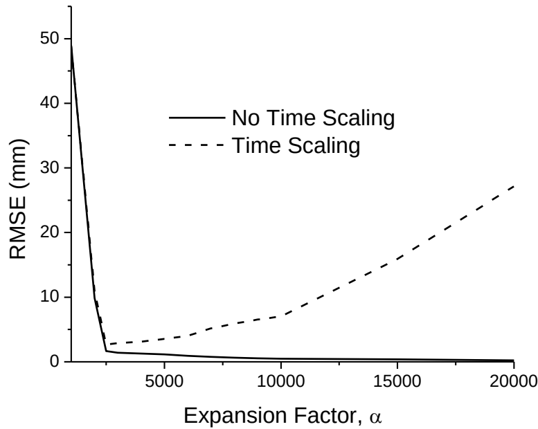
Figure 6-13: Average 3-D RMSE obtained by simulating the optical rail experiment with no channel effects incorporating leading-edge detection, a modulation factor \beta = 5 , a 21-sample MIQR filter, and 5x averaging of the TDOA results. The effects of time scaling increase proportionally with the expansion factor and cause a trade-off between mitigating jitter/AWGN effects and mitigating time scaling effects. \alpha = 2500 is considered the optimal expansion factor for minimizing the combined effects of jitter, AWGN, and time scaling.
