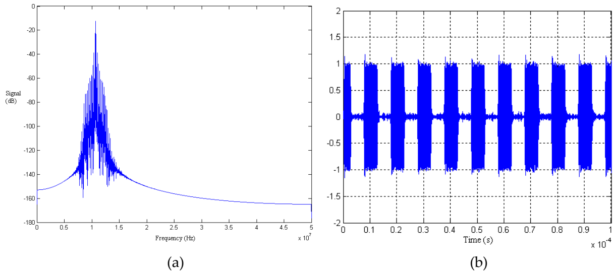
Figure 4-6: (a) Frequency spectrum in dB of ASK signal after BPF, (b) Corresponding signal in time domain.
