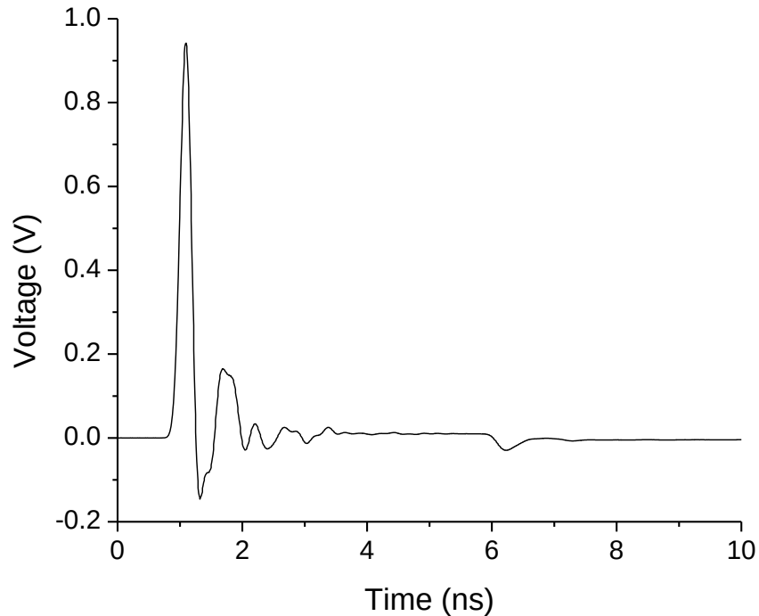
Figure 9-20: Simulated baseband UWB Gaussian pulse used as a template signal for the matched filter outlined in Step 1.
