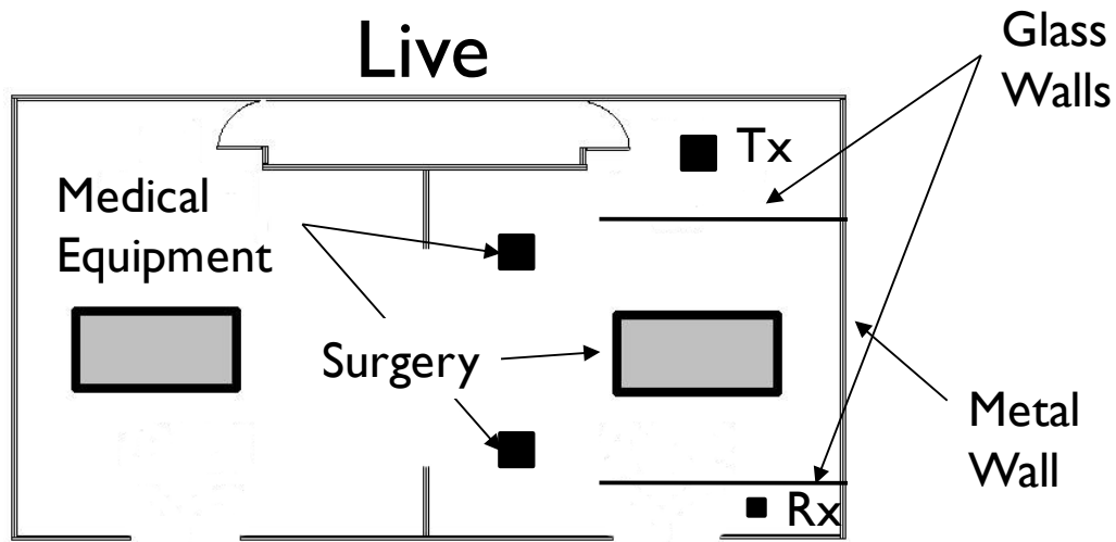
Figure 4-14: Layout of dual operating room during surgery outlining the patient table, glass walls, medical equipment, doors, and walls. The Tx and Rx were positioned 4 m apart across the surgery.
