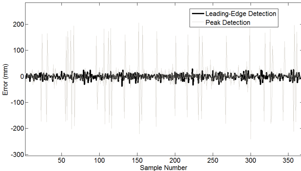
Figure 9-9: Variation in millimeters for a tag in a static location comparing raw output data from the peak and leading-edge detection algorithms. The leading-edge detection algorithm has a standard deviation of 11.1 mm compared to a standard deviation of 76.5 mm for peak detection.
