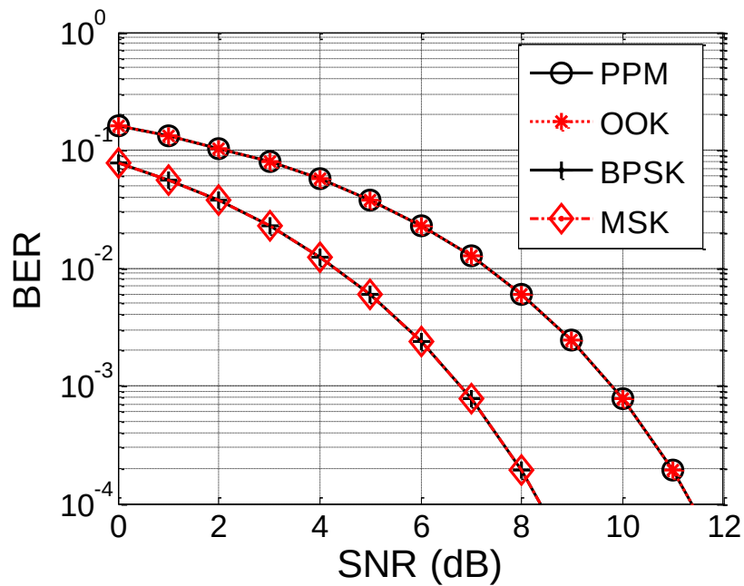
Figure 7-1: Comparison of theoretical bit-error-rates for UWB modulation schemes (PPM, OOK, BPSK) and narrowband 2.4 GHz MSK in AWGN channel.
