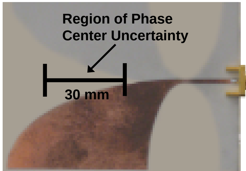
Figure 7-37: A roughly 30 mm range of uncertainty is introduced in measuring the UWB base station Vivaldi phase centers. This can translate into 10-60 mm of systematic error in the BA, CA, and DA range differences when comparing optical and UWB range difference data.
