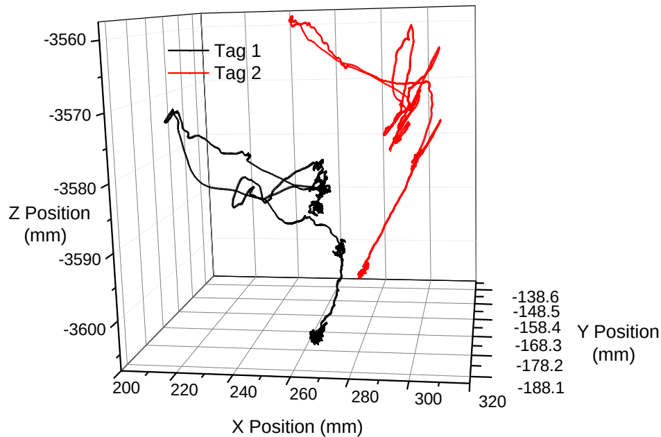
Figure 8-9. X,Y,Z plot of the 3-D position of two separate tags as they are moved dynamically while attached to the same rigid body. Accuracy was not measured but is estimated at 6-7 mm 3-D RMSE.
