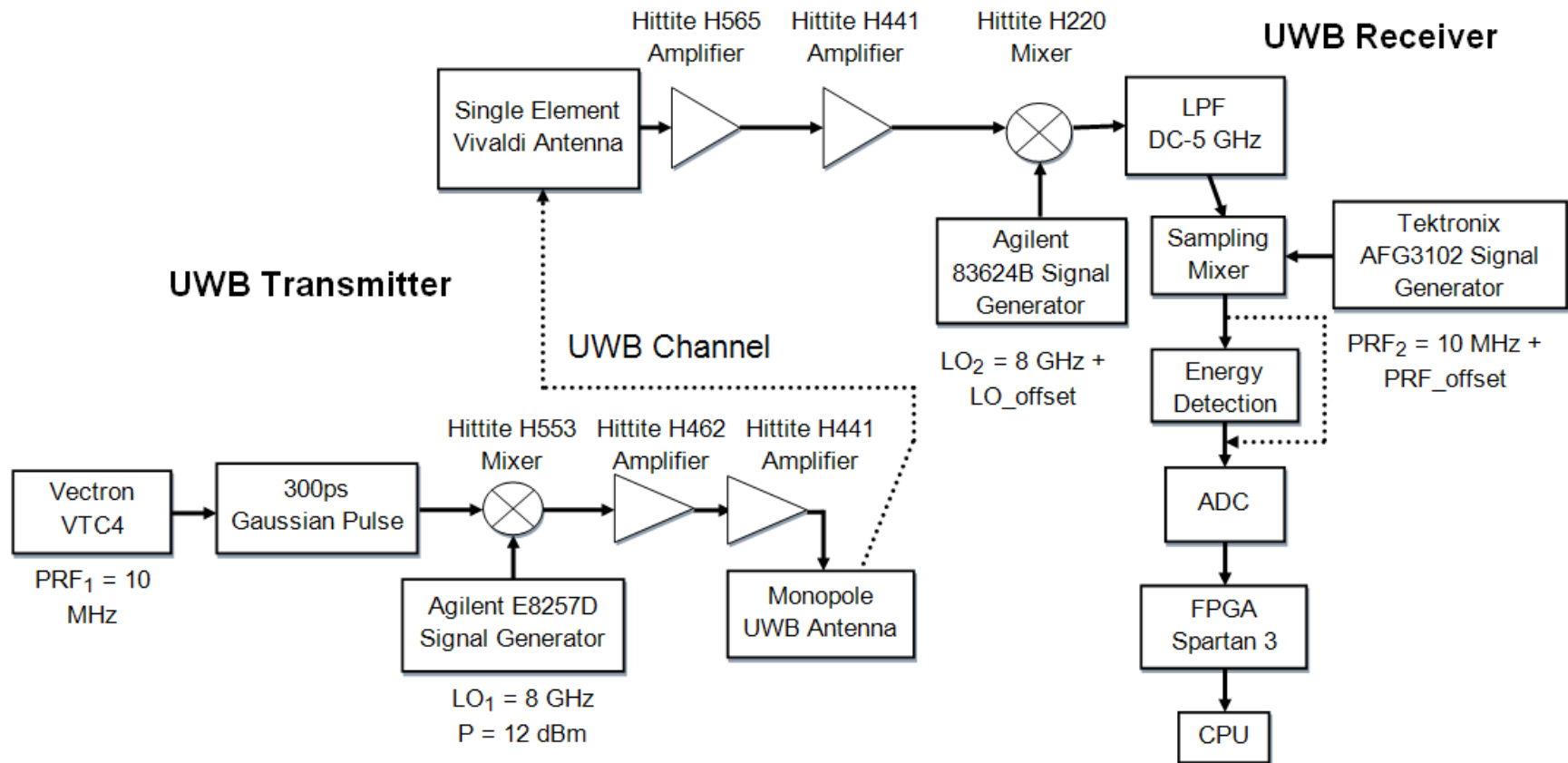
Figure 6-3: Block diagram of UWB transmitter and receiver architectures including the UWB channel.
