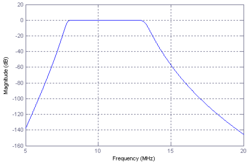
Figure 4-5: Frequency response of bandpass filter.
