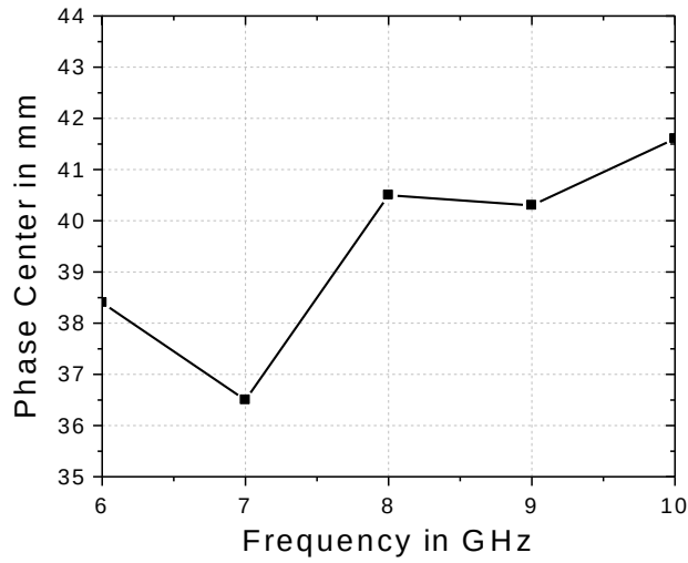
Figure 5-6: Simulation of broadside Vivaldi phase center location versus frequency [18].
