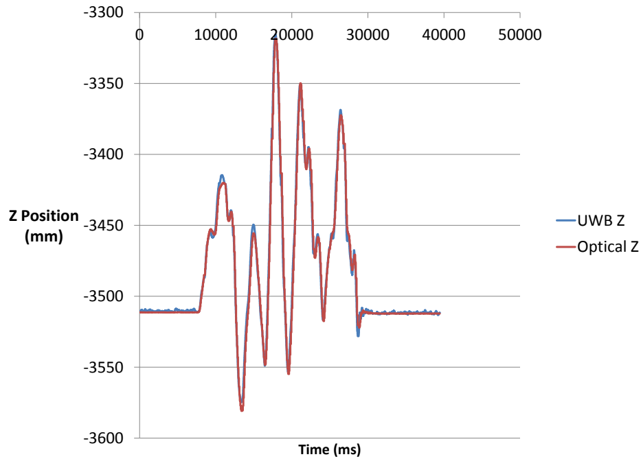
Figure 8-5. Typical optical rail experiment where the majority of 3-D motion is along the Z axis. The optical tracking system and UWB positioning system track together with around 6-8 mm of 3-D dynamic error. These results are for Tag 8.
