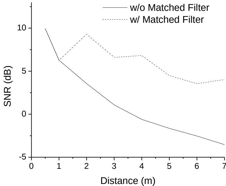
Figure 9-25: SNR versus Tx-Rx distance for standard leading-edge algorithm versus adaptive leading-edge algorithm. The UWB channel environment is the IEEE 802.15.4a industrial LOS channel. On average the addition of a MF increases the SNR by 5.82dB in low SNR conditions (when original signal y[t] has SNR below 6dB).
