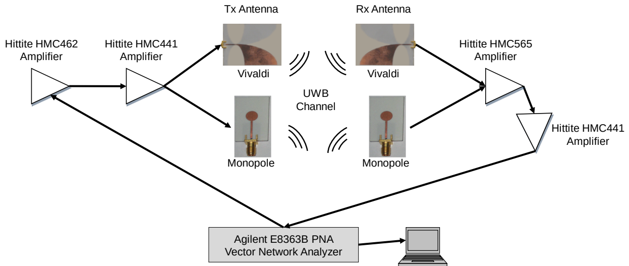
Figure 4-13: Experimental setup to collect frequency domain data in the operating room for characterization of the 3.1-10.6 GHz UWB band.
