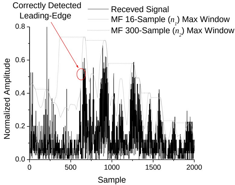
Figure 9-24: Simulated UWB received signal from Figure 9-22 where the adaptive leading-edge algorithm is run with \alpha = 2 , n_1 = 16 , n_2 = 300 , and the template shown in Figure 9-20. Since the new SNR = 4.11dB after applying a matched filter, the adaptive algorithm has no problem locating the correct UWB leading-edge (sample 595).
