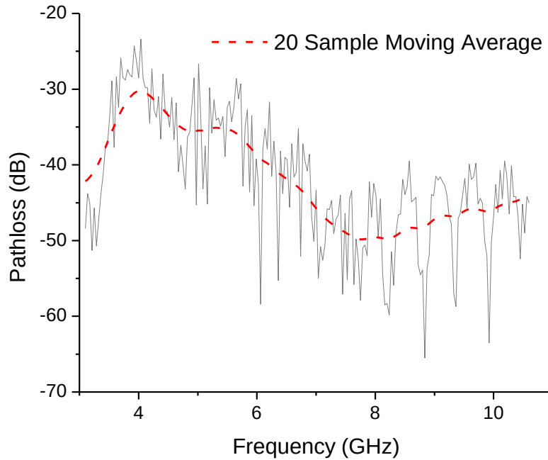
Figure 4-19: Pathloss obtained with the Tx and Rx placed 0.49 m apart where effects from the transmitting (monopole) and receiving (Vivaldi) antennas have been removed. The frequency dependence, \kappa in Table 4-2, can clearly be seen as well as small scale fading effects.
