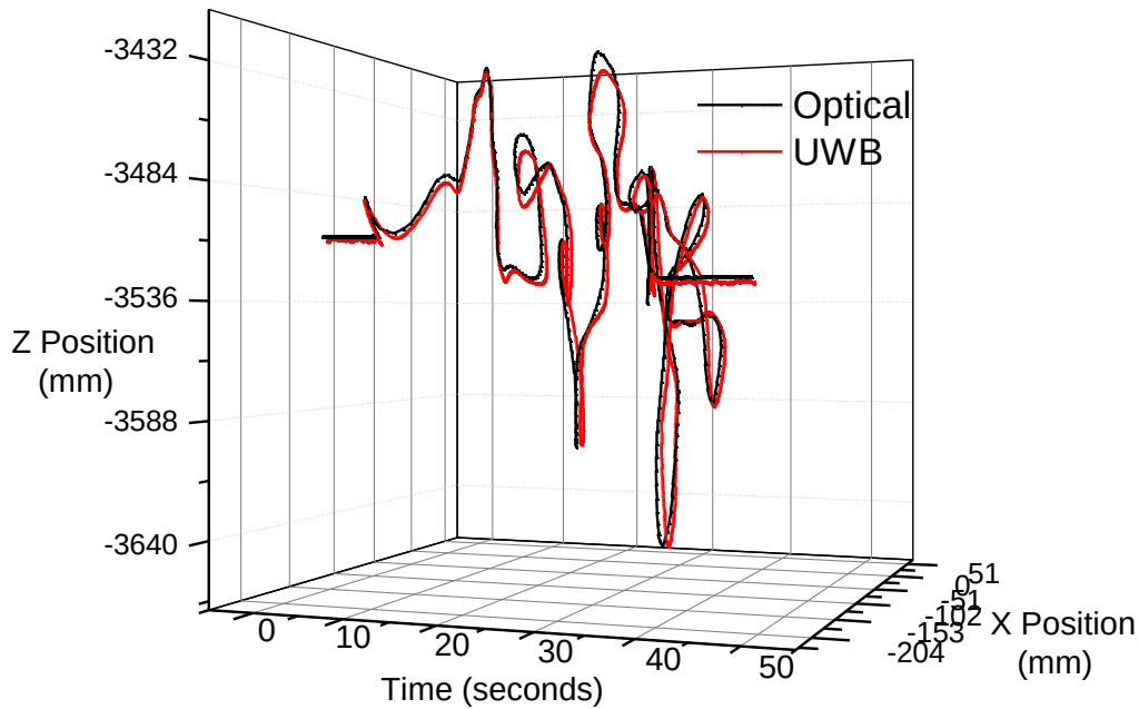
Figure 8-8. X-Z cross section with time also displayed for Tag 10 to show the real-time tracking of the UWB positioning system by the optical tracking system.
