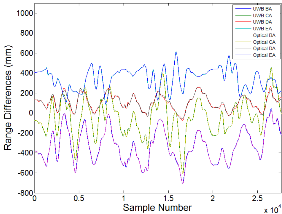
Figure 8-18. Five base station calibration data where the optical and UWB range differences BA, CA, DA, and EA are calibrated together via a homogeneous transformation matrix.
