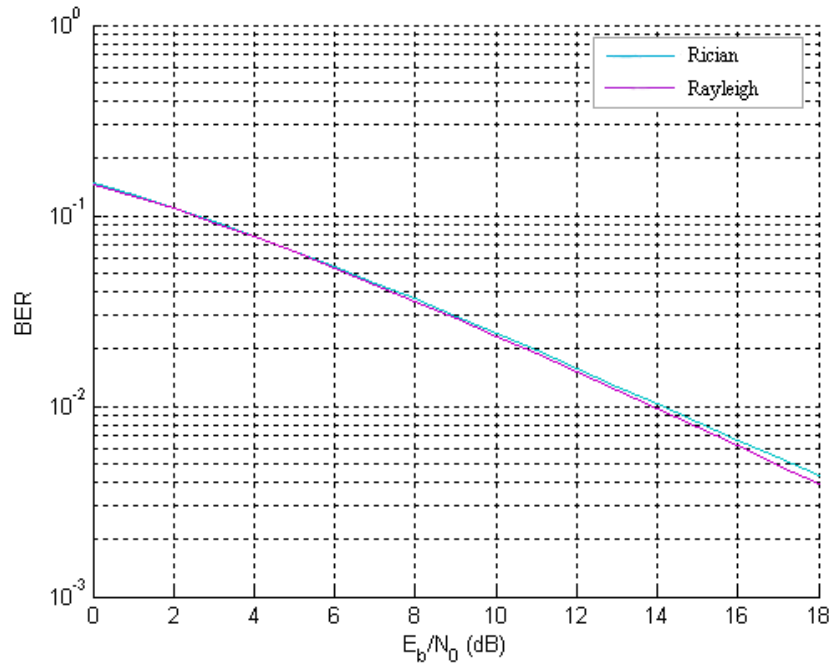
Figure 4-10: Theoretical performance of the ASK in fading Rayleigh and Rician channels.
