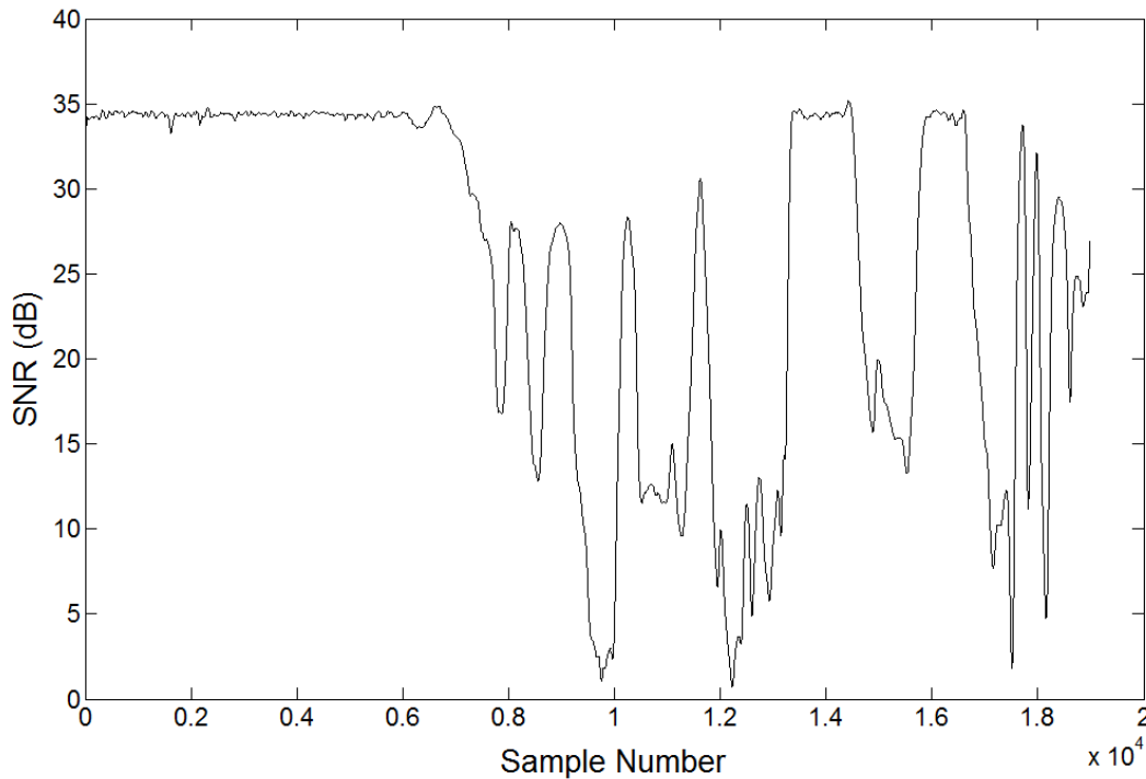
Figure 10-9: SNR for an experiment where a tag is left in a static location and extreme LOS blockage is introduced.
