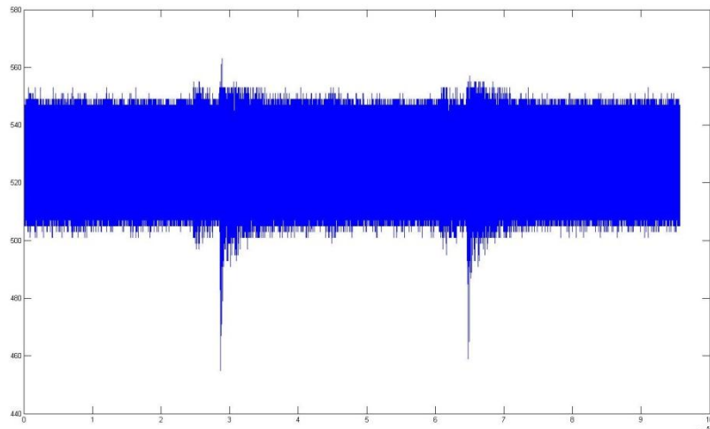
Figure 9-5: 30 \mu s UWB pulse at a 100,000 expansion factor after analog-to-digital conversion where the UWB pulse has been almost completely attenuated by the ADC input RF transformer.
