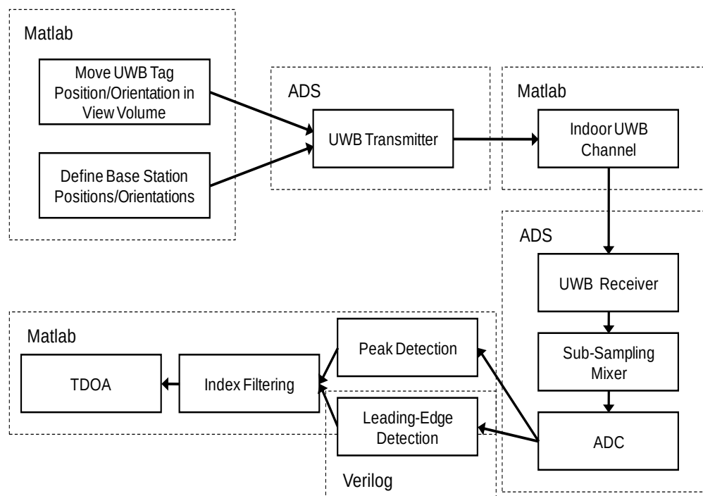
Fig. 1. Block diagram of overall system simulation framework outlining the various portions of the system simulated in Matlab, Agilent ADS, and Verilog.
