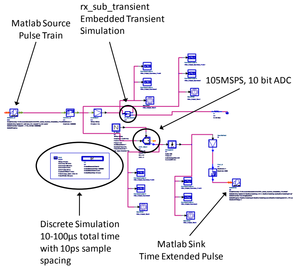
Fig. 9. Overview of receiverQ discrete time simulation which embeds the rx_sub_transient transient simulation. The UWB pulse train is read from the Matlab source. The subsampling takes place in the rx_sub_transient block. The pulse then goes through the ADC and finally the time extended, digital pulse is saved via the Matlab sink.
