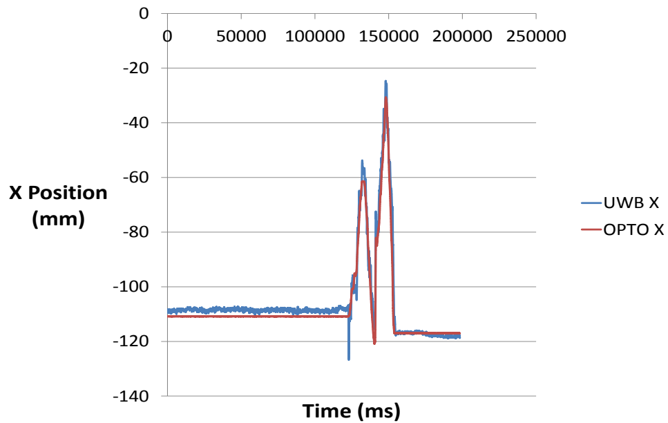
Figure 8-15. X position values for both the UWB and optical tracking systems for an optical rail experiment where Tag 13 is dynamically moved along the optical rail. The RMSE in the X dimension is 2.52 mm.
