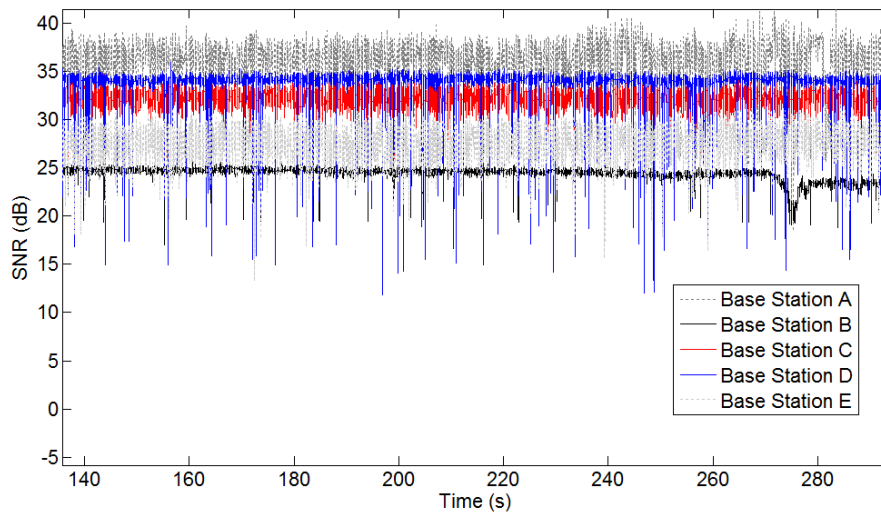
Figure 9-16: The SNR for five base stations (A, B, C, D, E) for a static scenario where the tag is kept in a static location. The SNRs of the base stations vary between 25-38 dB but illustrate a strong UWB link between the tag and the five base stations.
