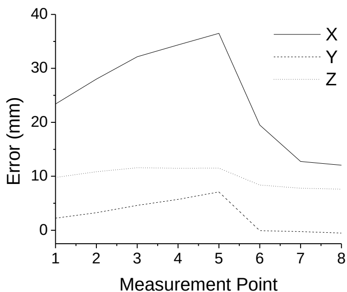
Figure 6-21: Comparison of x,y,z error for all points in simulating the multi-base station experiment outlined in Figure 6-20d using leading-edge detection. Substantially larger errors are observed in x; z also has higher error than y.
