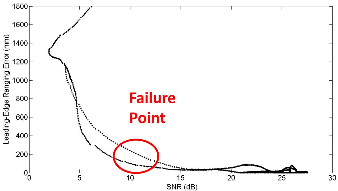
Figure 10-7: Leading-edge algorithm ranging error for one base station versus SNR from the experimental results outlined in Figure 10-5 and Figure 10-6. The leading-edge detection algorithm fails around when the SNR reaches 10-12 dB. At this signal level, the leading-edge ( 1/4^{\text{th}} peak amplitude) will often drop below the noise floor, resulting in large ranging errors (1000 mm or greater).
