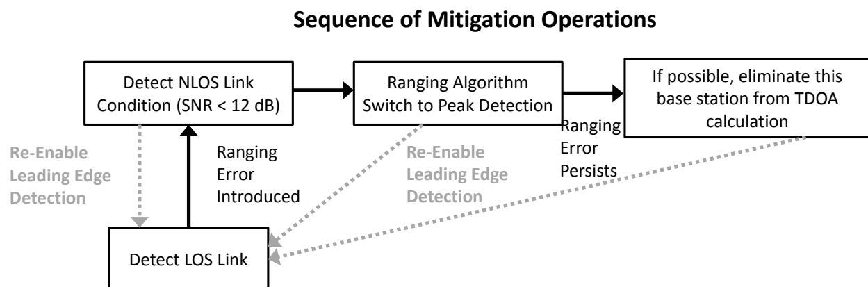
Figure 10-8: Block diagram of NLOS detection and mitigation steps including a return to a LOS link.
