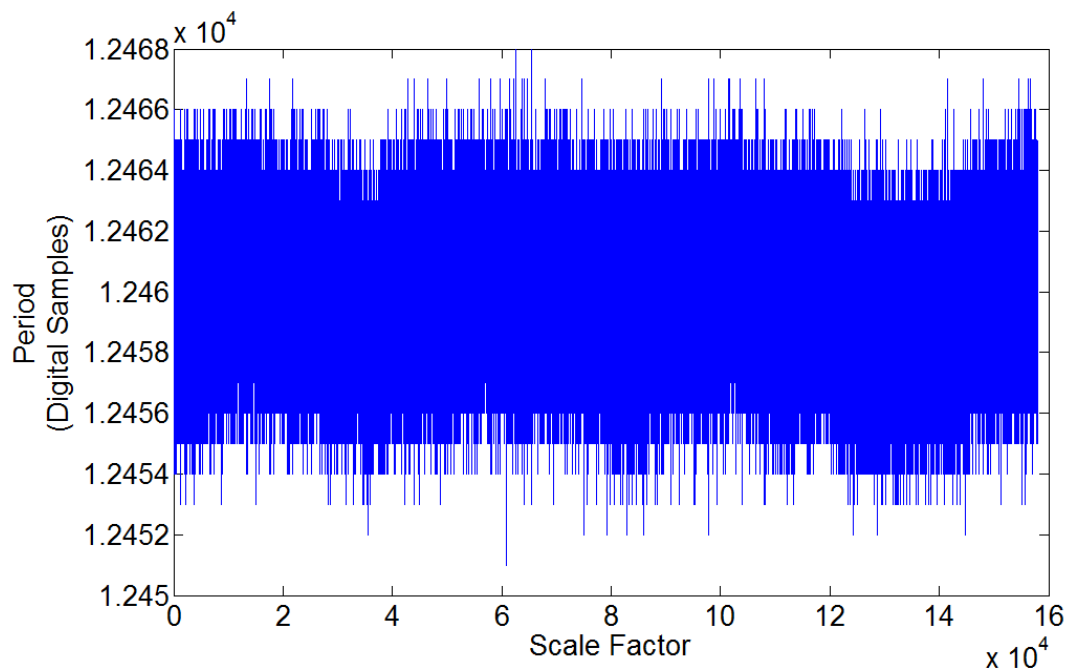
Figure 7-27: Period between successive leading-edges of the UWB pulse train from Tag 9 in digital samples spaced 20 ns apart for almost 160,000 successive UWB pulses.
