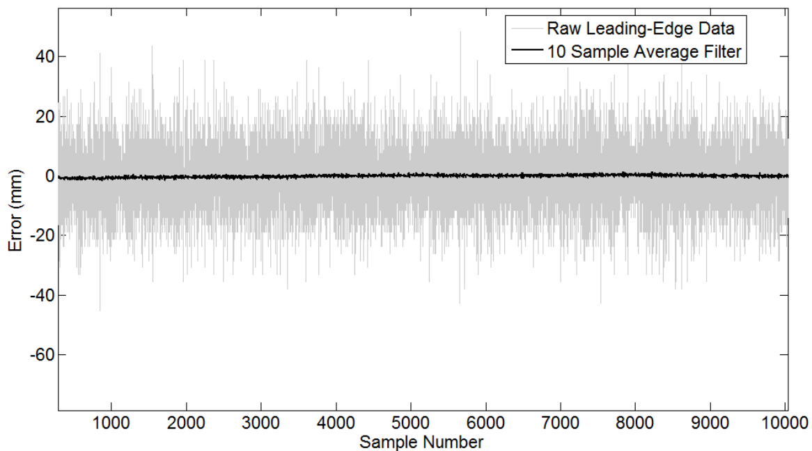
Figure 9-10: Variation in millimeters for a tag in a static location for 10,000 consecutive UWB pulse leading-edge calculations. The raw leading-edge detection data has a standard deviation of 11.1 mm while the application of a 10-sample averaging filter reduces the standard deviation to 0.60 mm. The leading-edge detection data is Gaussian and is easily filtered.
