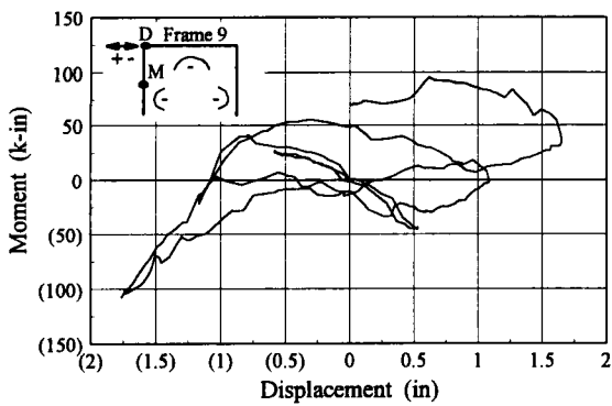
Bare Frame 9 Moment-Displacement Hysteresis
