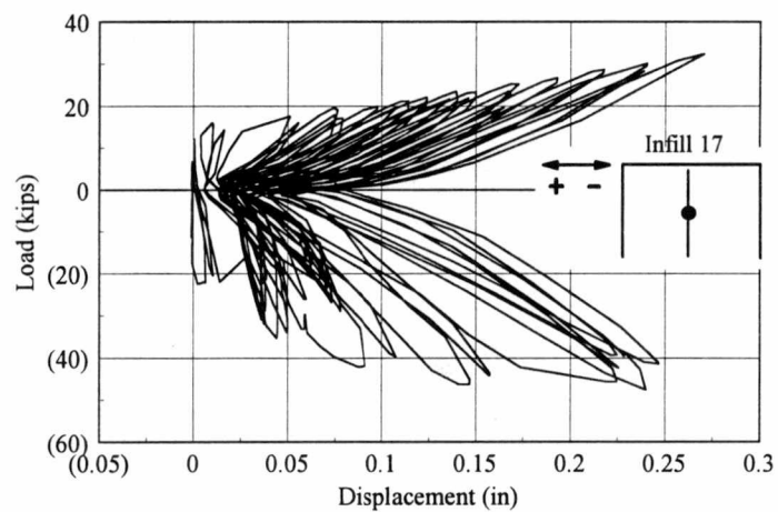
Figure 5.6 Specimen 17 Panel Vertical Hysteresis
