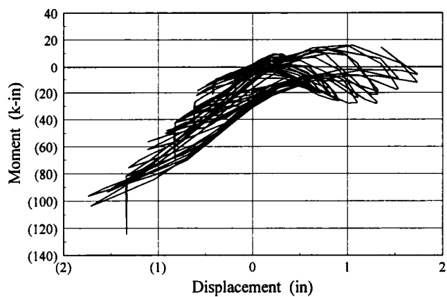
Figure 7.32 Specimen 23 Moments Near Left Column Midheight
