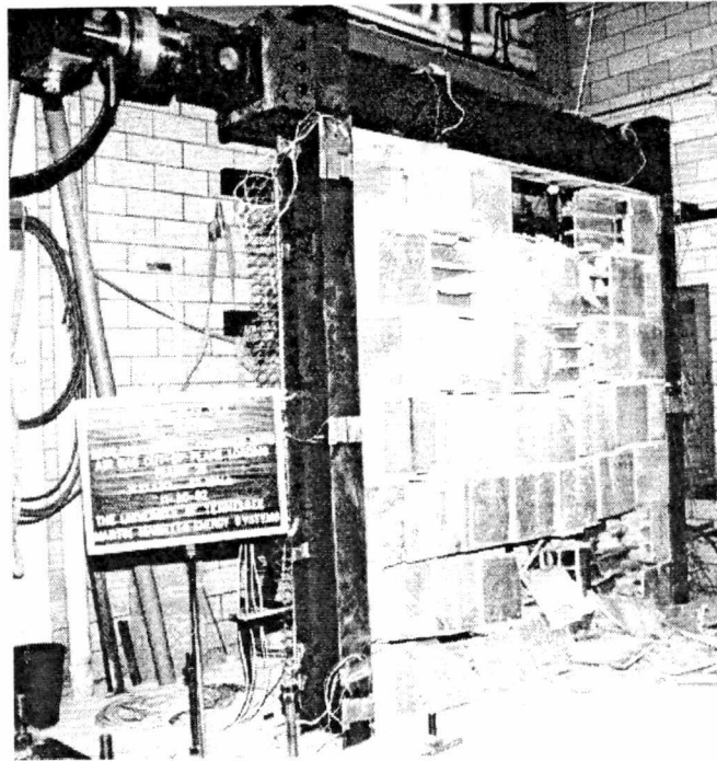
Figure 7.27 Specimen 23 After Testing
