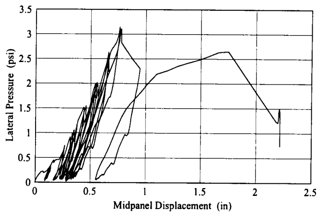
Figure 7.12 Specimen 19 Uniform Lateral Loading
