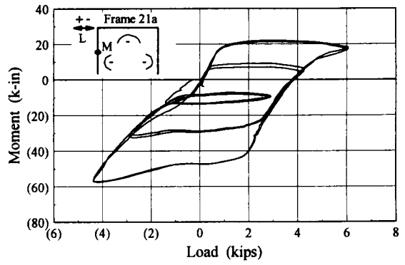
Bare Frame 21a Moment-Load Hysteresis
