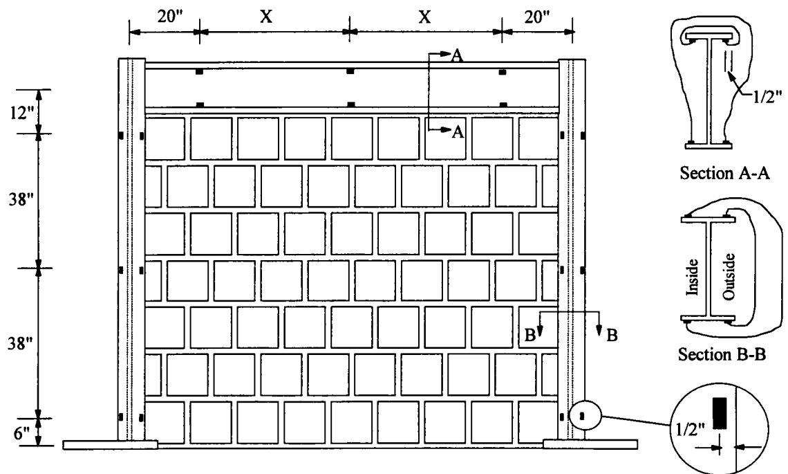
Figure 3.7 Frame Strain Gage Measurements
