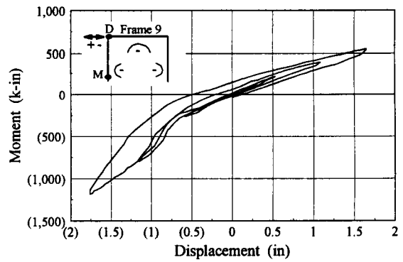
Bare Frame 9 Moment-Displacement Hysteresis
