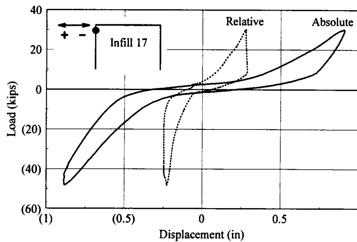
Figure 5.9 Comparison of Relative and Absolute Displacement
