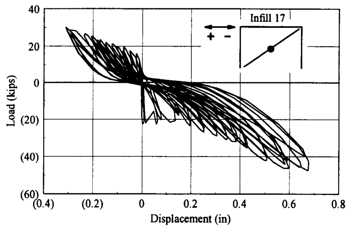
Figure 5.4 Specimen 17 Panel Diagonal Hysteresis 2
