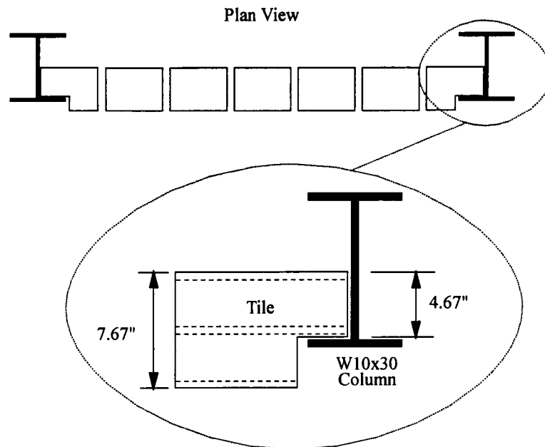
Figure 3.10 Specimen 7 Offset Panel Detail
