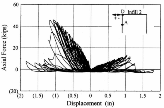
Infilled Frame 2 Axial Force-Displacement Hysteresis
