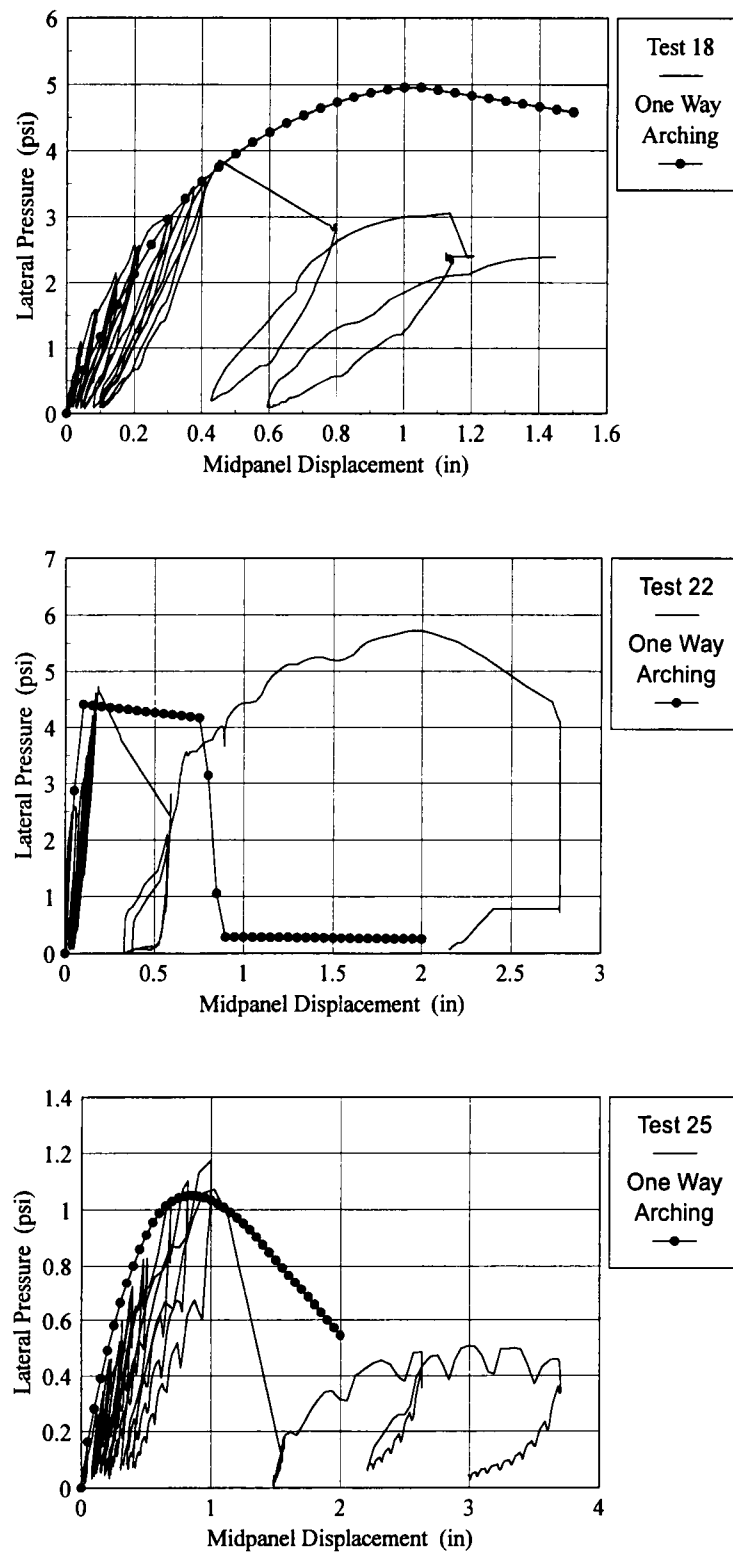
Figure 6.13 Comparison of Lateral Load Tests With Dawe and Seah (1989b)
