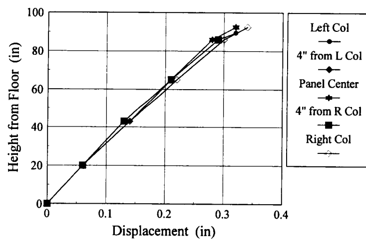
Figure 7.8 Specimen 13 Displaced Shape at Peak Beam Curvature Drift Load (49.4 kips)
