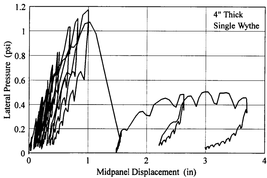
Figure 6.5 Specimen 25 Pressure Versus Displacement
