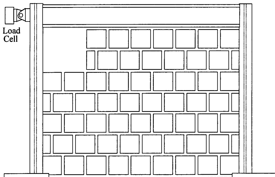
Figure 3.13 Specimen 24 Corner Opening
