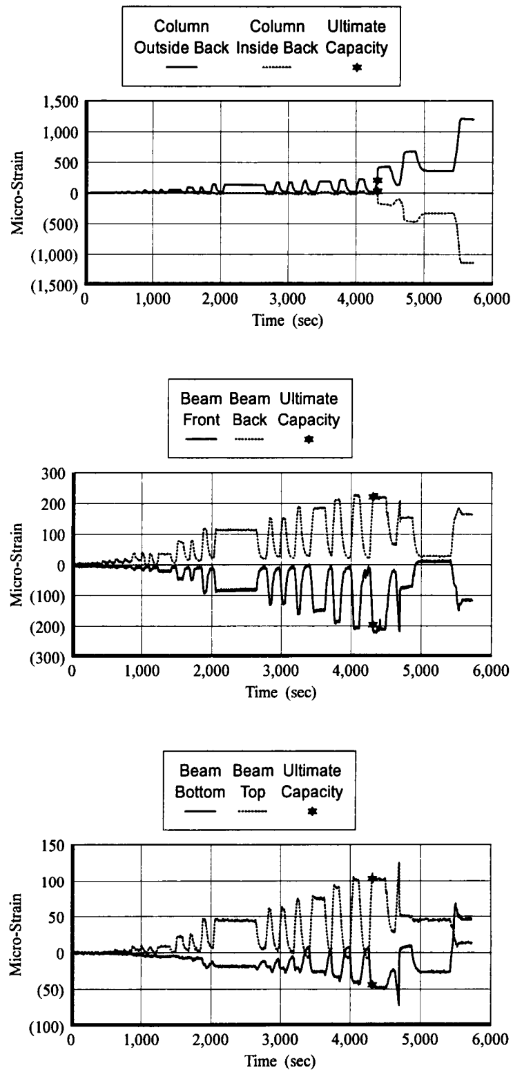
Figure 6.11 Infilled Frame 18 Strain Time History Relationships
