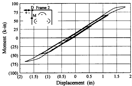
Bare Frame 2 Moment-Displacement Hysteresis
