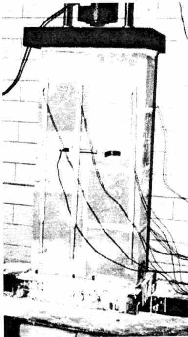
Figure 4.7 Prism Testing (Cores Parallel to Load)
