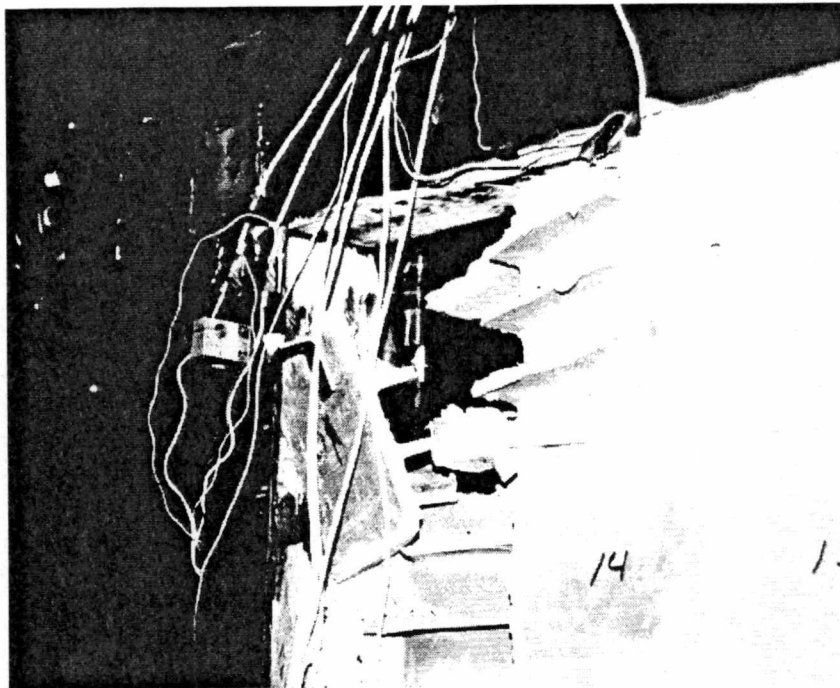
Figure 5.11 Infill 17 Corner Crushing Failure
