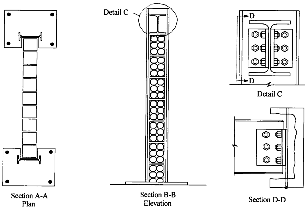
Figure 3.2 Single Wythe Panel Construction Details
