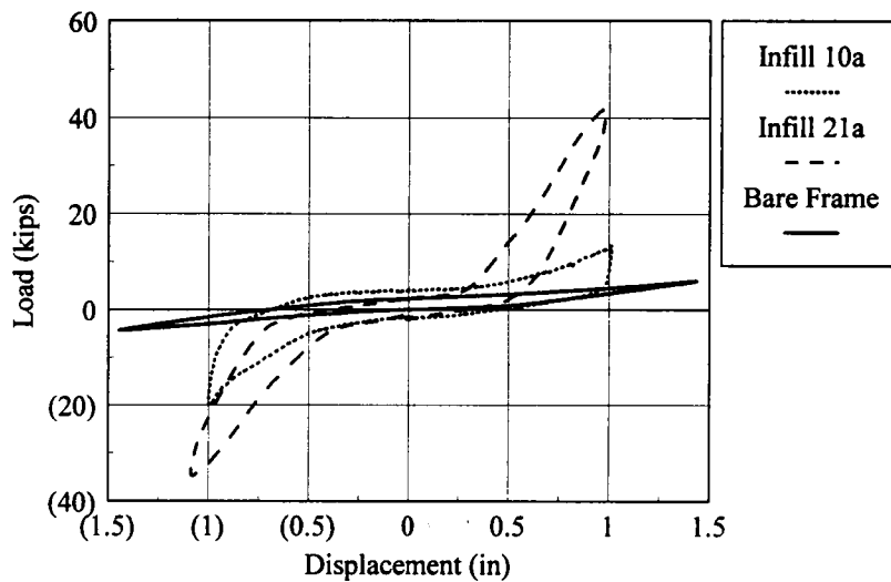
Figure 5.15 Comparison of Infill 10a and 21a With Bare Frame
