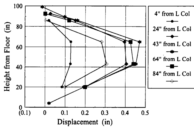
Figure 6.7 Specimen 18 Displaced Shape at Ultimate Capacity (3.9 psi)
