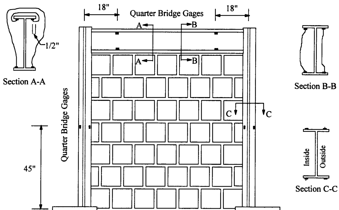
Figure 3.19 Air Bag Test Strain Gage Locations
