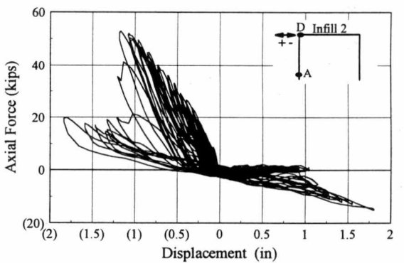
Infilled Frame 2 Axial Force-Displacement Hysteresis
