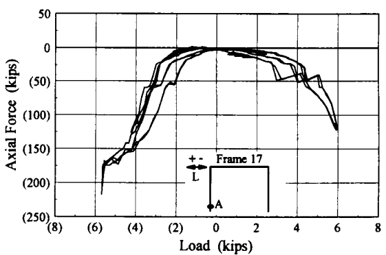
Bare Frame 17 Axial Force-Load Hysteresis
