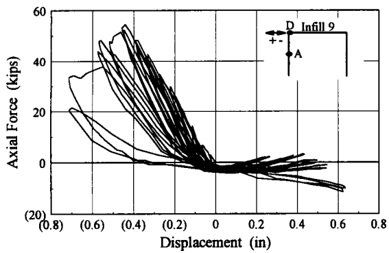
Infilled Frame 9 Axial Force-Displacement Hysteresis
