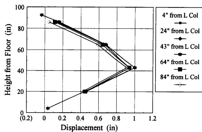
Figure 6.8 Specimen 25 Displaced Shape at Ultimate Capacity (1.2 psi)
