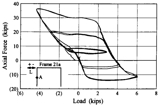
Bare Frame 21a Axial Force-Load Hysteresis
