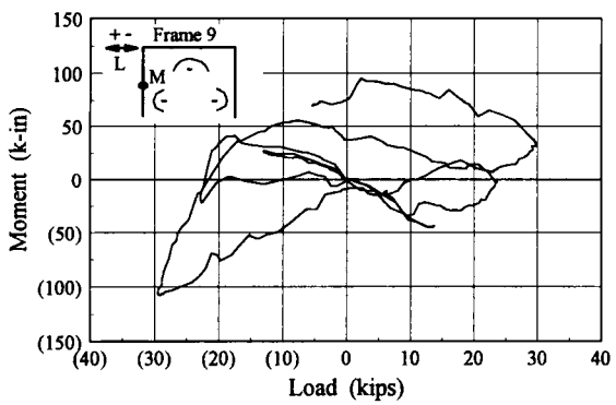
Bare Frame 9 Moment-Load Hysteresis
