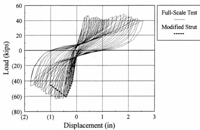
Figure 5.23 Henderson et al. (1993) Strut Analysis With Added Stiffness
