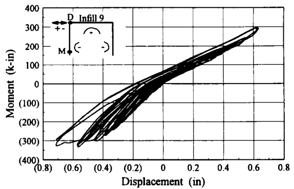
Infilled Frame 9 Moment-Displacement Hysteresis
