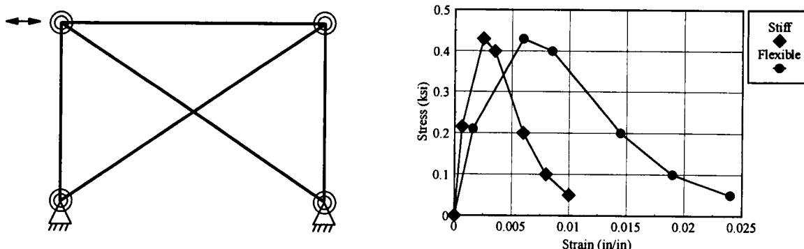
Figure 5.18 Nonlinear Compressive Strut Properties
