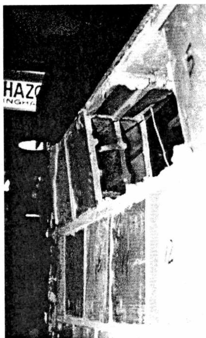
Figure 6.6 Failure Mechanism of Top and Bottom Course Tiles
