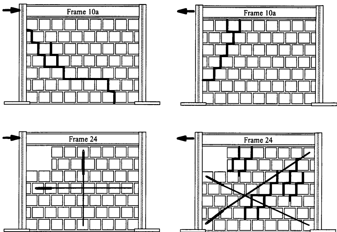
Figure 5.16 Infill 10a and 24 Crack Patterns
