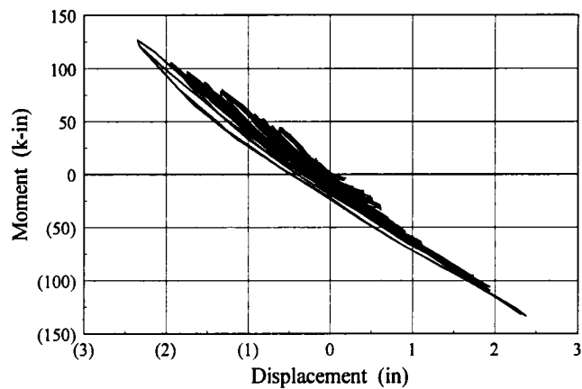
Figure 7.30 Specimen 23 Moments Near Right Column Base
