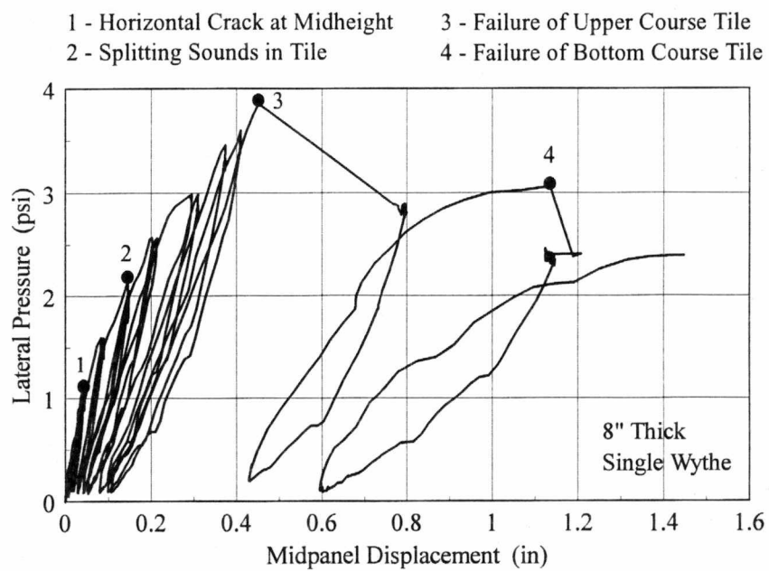
Figure 6.3 Specimen 18 Pressure Versus Displacement
