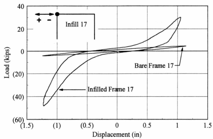
Figure 5.7 Comparison of Infilled Frame and Bare Frame
