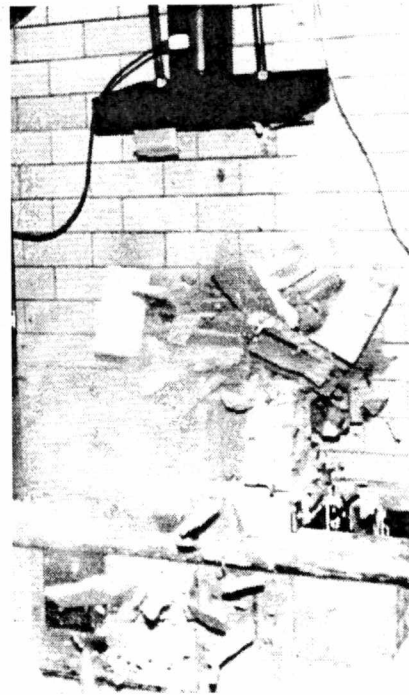
Figure 4.6 Prism Testing (Cores Normal to Load)
