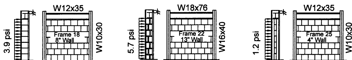
Figure 3.14 Summary of Uniform Lateral Load Testing Specimens and Ultimate Capacities
