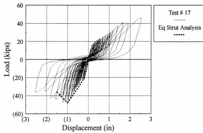
Figure 5.21 Infilied Frame 17 Piecewise Linear Strut Analysis
