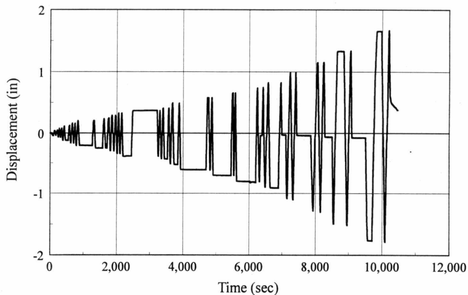
Figure 3.5 Typical In-Plane Displacement Time History
