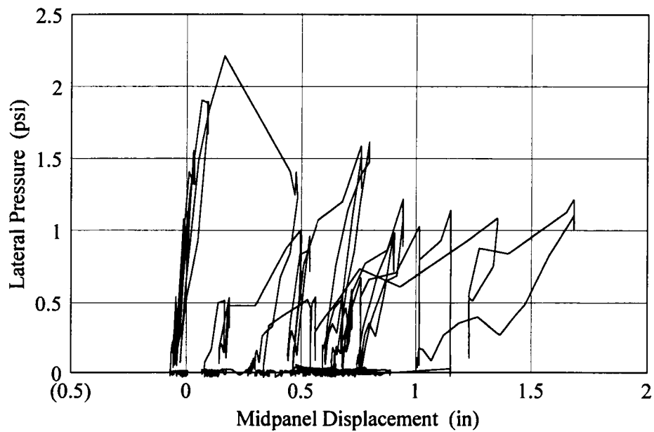
Figure 7.29 Specimen 23 Uniform Lateral Load Hysteresis
