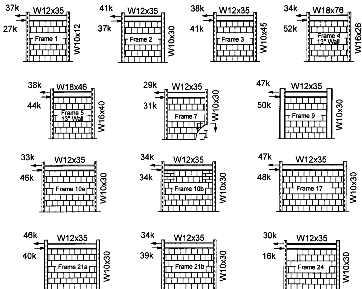
Figure 3.9 Summary of In-Plane Testing Specimens and Ultimate Capacities
