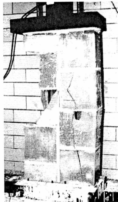
Figure 4.7 Prism Testing (Cores Parallel to Load)
