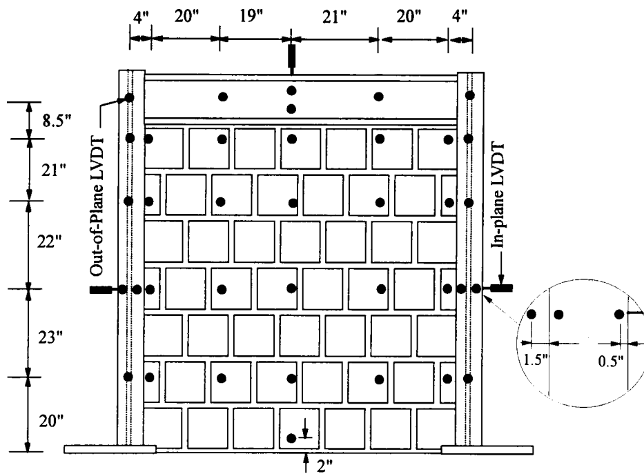
Figure 3.18 Air Bag Test Displacement Measurements
