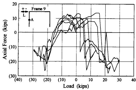
Bare Frame 9 Axial Force-Load Hysteresis
