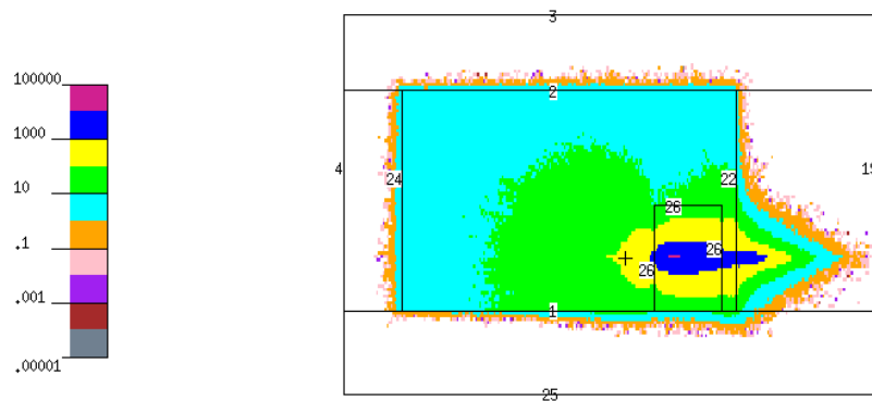
Figure 15: YZ View of Flux Map [particles/cm 2 /sec] with Beehive
