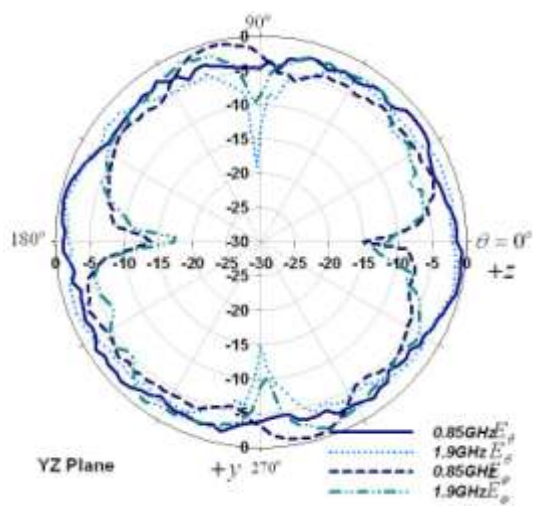
Figure 5.28 State1 YZ plane
