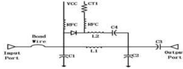
Figure 4.3 A reconfigurable output matching network structure with switchable inductors [25]
