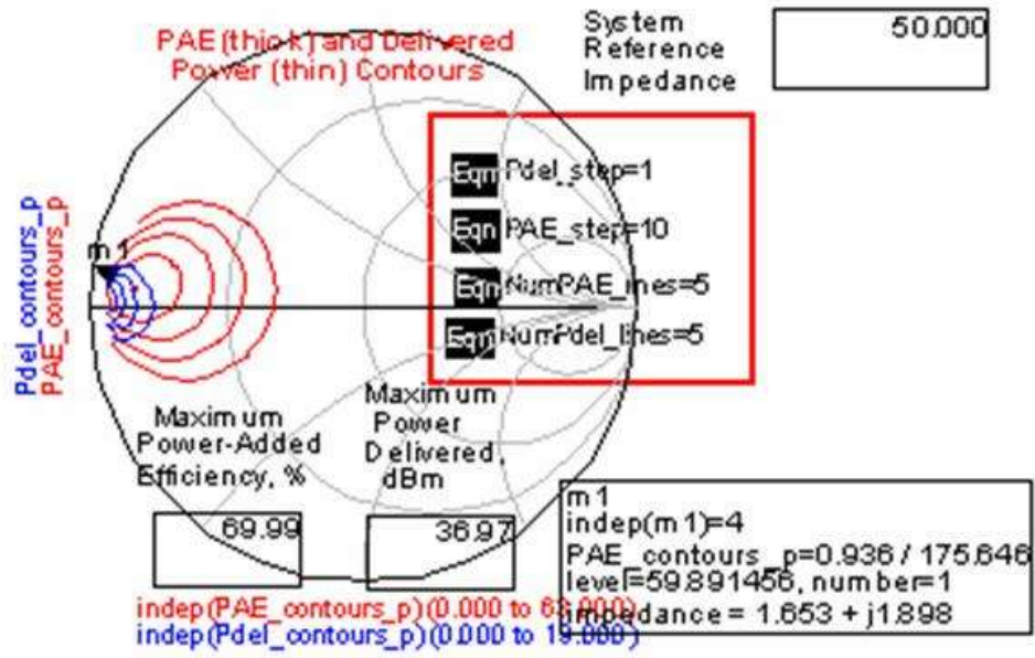
Figure 4.21 Load pull simulation result for LB
