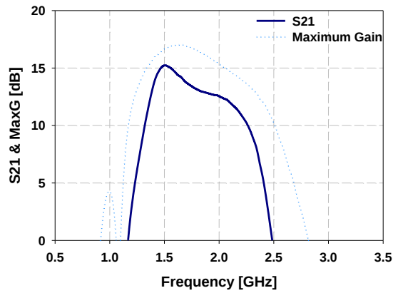
Figure 4.37 Maximum Gain and S21
