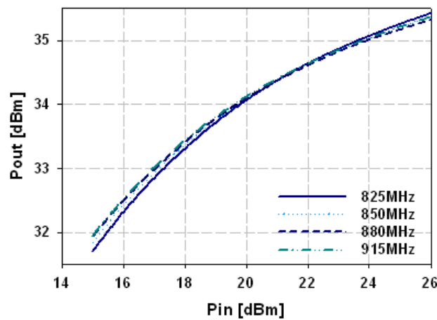
Figure 4.30 Pout vs. Pin, where a 17.5 dB input power is required to achieve a 33 dBm output power over the frequency range of interest
