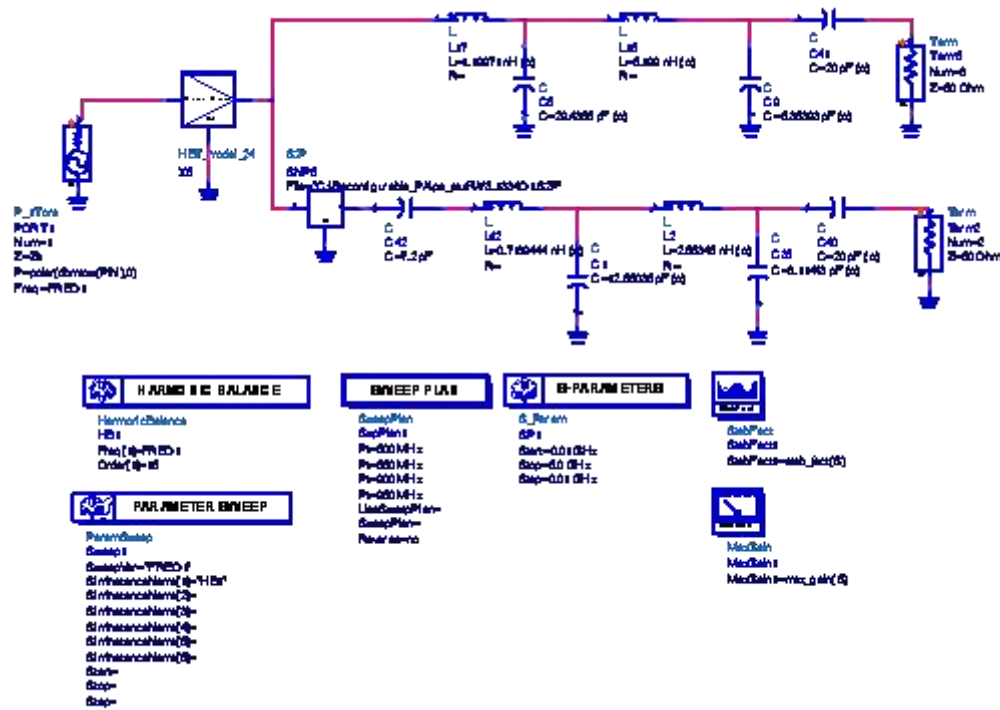
Figure 4.29 Bench setup for the Harmonic Balance and S-parameter simulation. (S-parameters of the MEMS switch provided by Radant has been used in the simulation [33])
