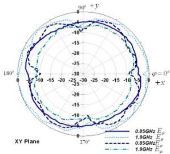
Figure 5.27 State1 XY plane
