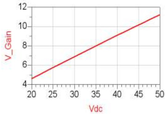
Figure 4.15 Drain voltage vs Voltage gain [29]
