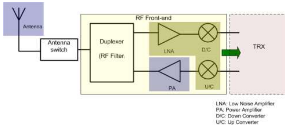
Figure 2.1 A RF transceiver configuration example [7]
