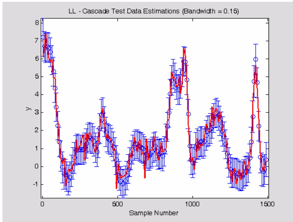
Figure 5.3.19: LL median result estimation and analytic prediction intervals Representative result for LL model (Bandwidth = 0.15) showing every 10 th estimate and the corresponding analytic prediction intervals. This model exhibited the median value of the 100 Mean Absolute Error results for the Bandwidth=0.15 models. LL – Local Linear Regression.
