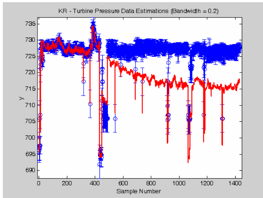
Figure 5.5.18: KR median result estimation and analytic prediction intervals.
