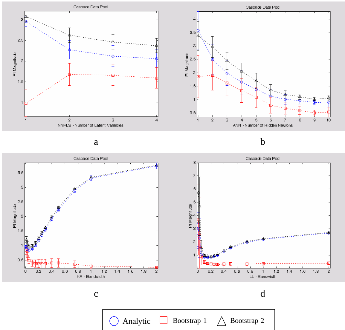
Figure 5.3.3: PI Magnitude Results for Cascade Data Pool.
