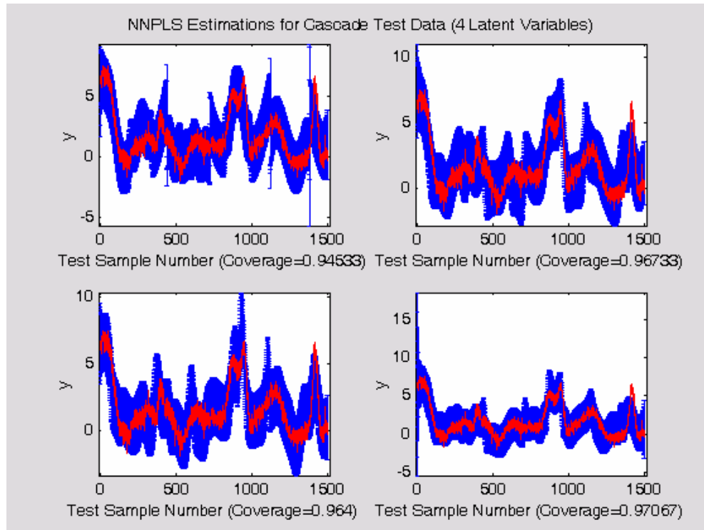
Figure 5.3.12: NNPLS cascade test data estimations and analytic prediction intervals. Test estimations and their corresponding analytic prediction intervals. These 4 results were selected at random from the 100 models. The coverage values for each are shown along the x-axis. NNPLS – Neural Network Partial Least Squares.
