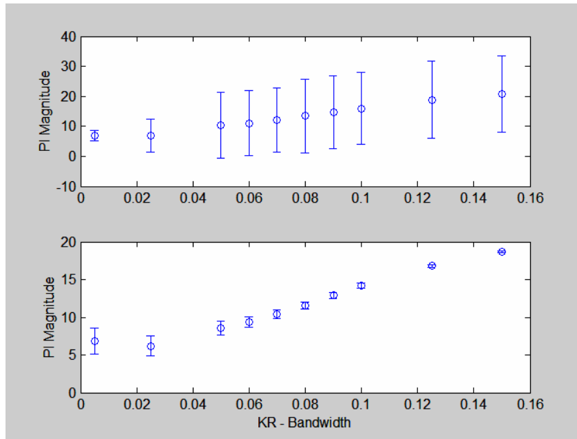
Figure 5.4.18: Original and modified bootstrap prediction intervals for KR models of the feedwater flow rate data pool.
