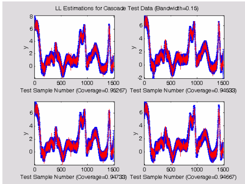
Figure 5.3.15: LL cascade test estimations and analytic prediction intervals.
