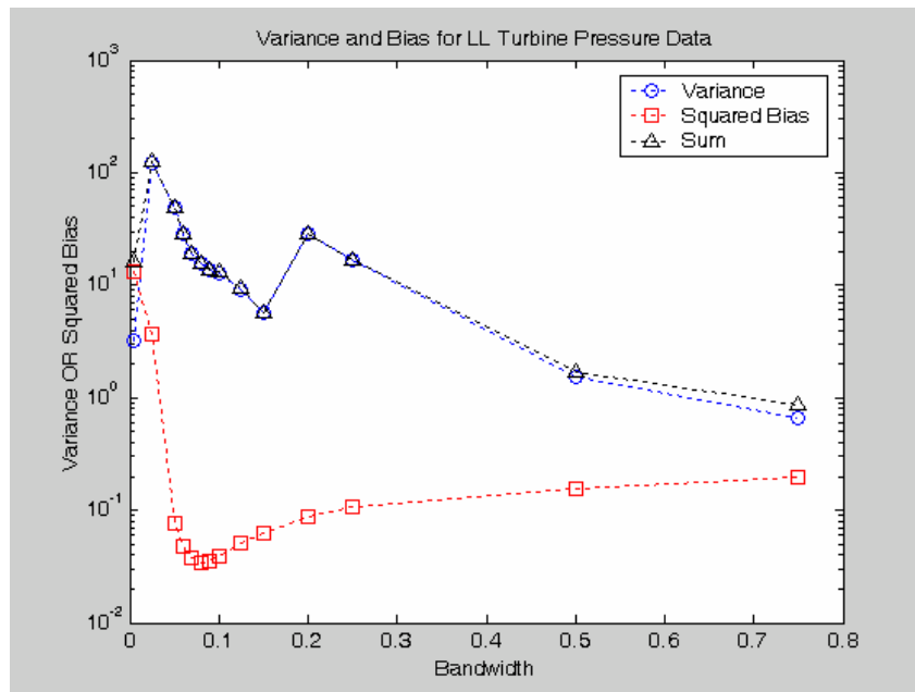
Figure 5.5.23: Combined variance of training and validation data vs. squared bias of data pool for LL models of turbine pressure data.
