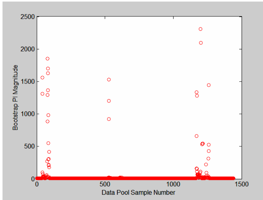
Figure 5.4.31: Bootstrap prediction intervals for LL models of feedwater flow rate data pool, bandwidth = 0.08.
