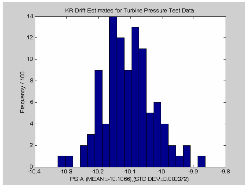
Figure 5.5.19: Distribution of drift estimate from KR models (bandwidth = 0.2). Drift estimates obtained from the 100 KR models via computing the MAE over test samples 600 to 1430. All 100 models provided \leq 5\% coverage in the region of drift.
