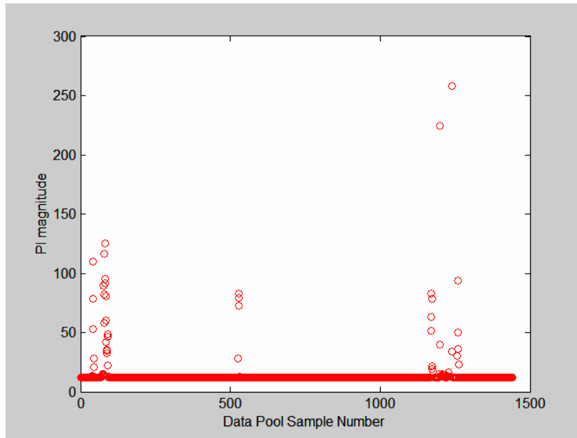
Figure 5.4.16: Bootstrap prediction intervals for KR models of the feedwater flow rate data pool, bandwidth = 0.025.
