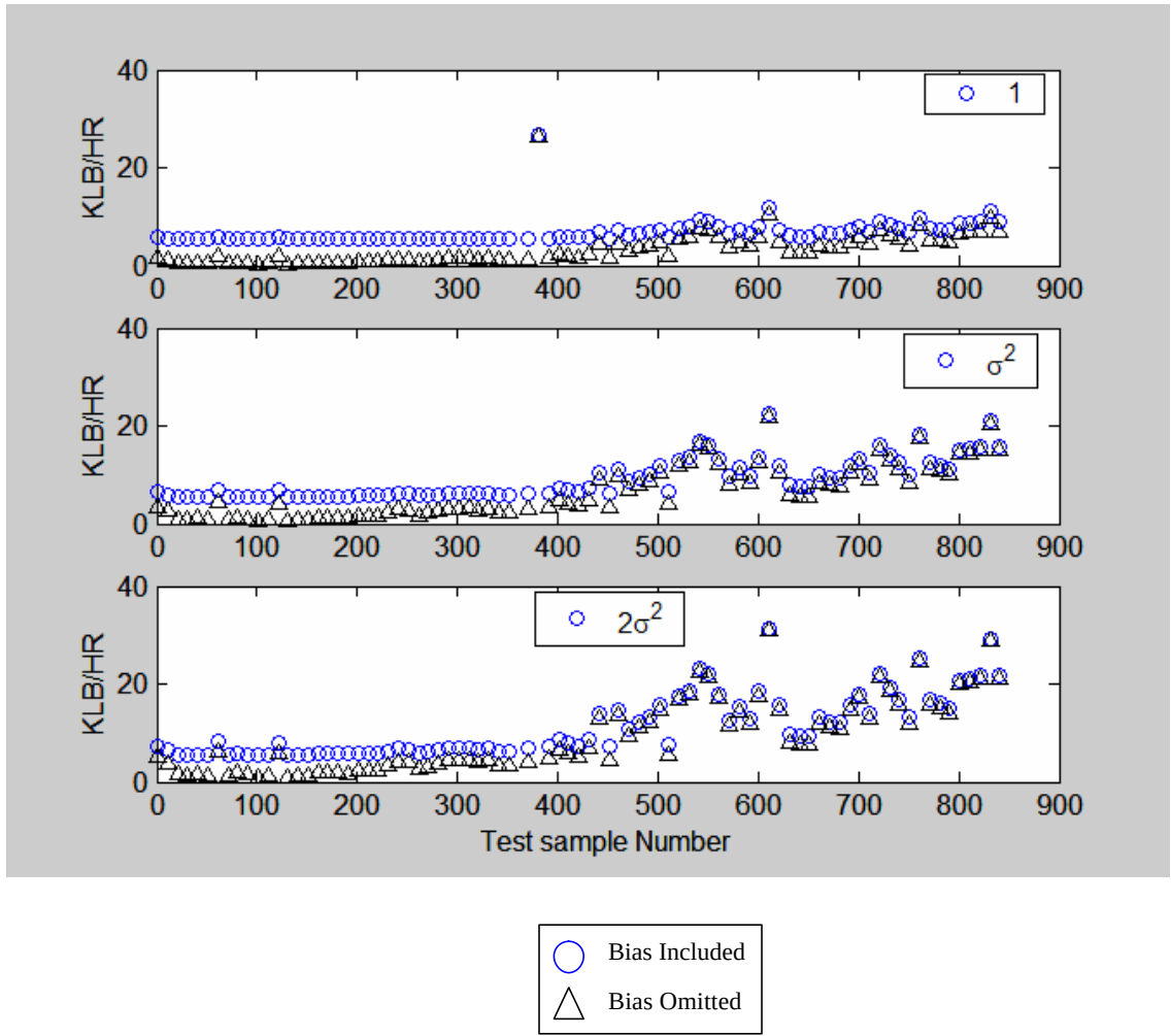
Figure 5.4.40: Analytic prediction interval magnitudes, of feedwater test data LL models, for various conditional variance estimates.
