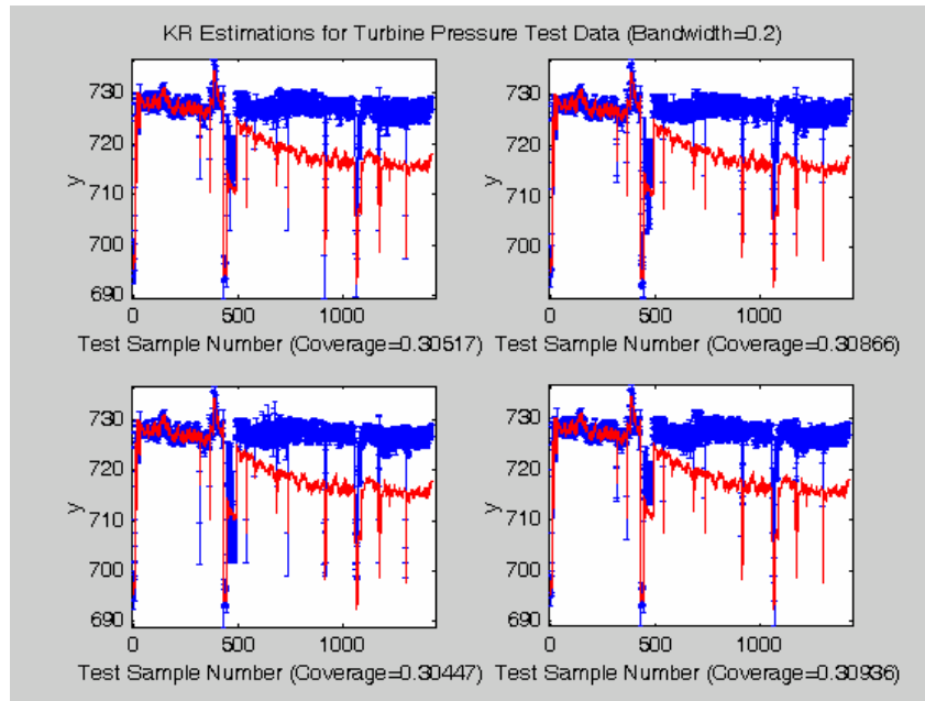
Figure 5.5.17: KR test estimations and their corresponding analytic prediction intervals. These 4 results were selected at random from the 100 available 0.2 bandwidth KR models. The coverage value for each case is indicated on the x-axis.
