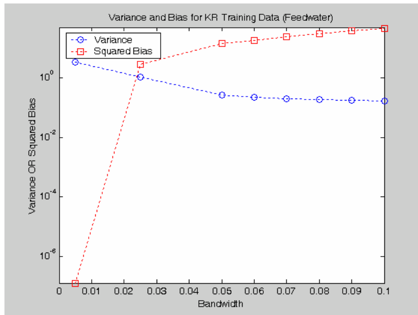
Figure 5.4.21: Variance / squared bias plot for KR models of feedwater flow rate training data.
