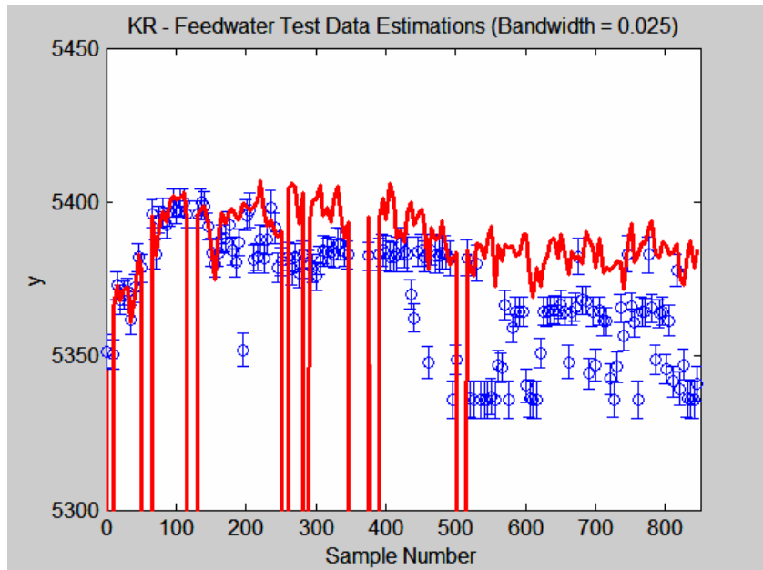
Figure 5.4.26: KR median result estimation and analytic prediction intervals. Representative results for KR model of bandwidth=0.025 showing every 5 th estimate and the corresponding analytic prediction intervals. This model exhibited the median value of the 100 Mean Absolute Error results for the KR models with a bandwidth of 0.025.
