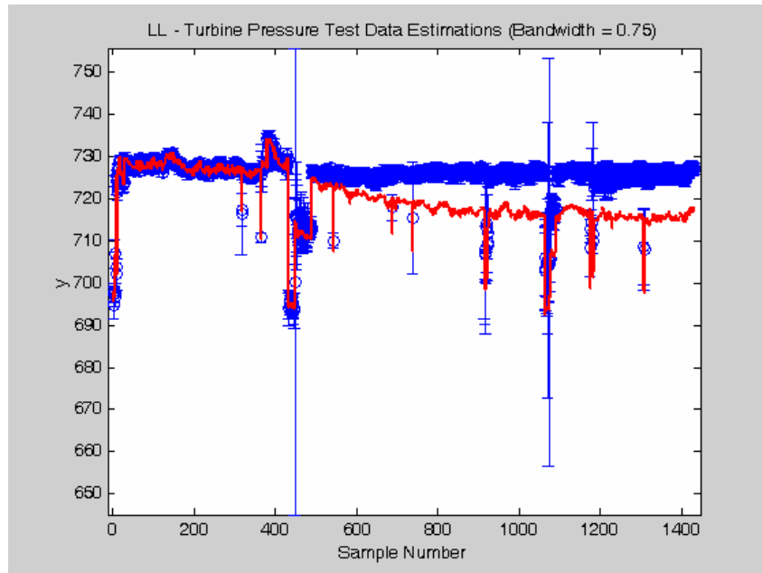
Figure 5.5.25: LL median result estimation and analytic prediction intervals.
