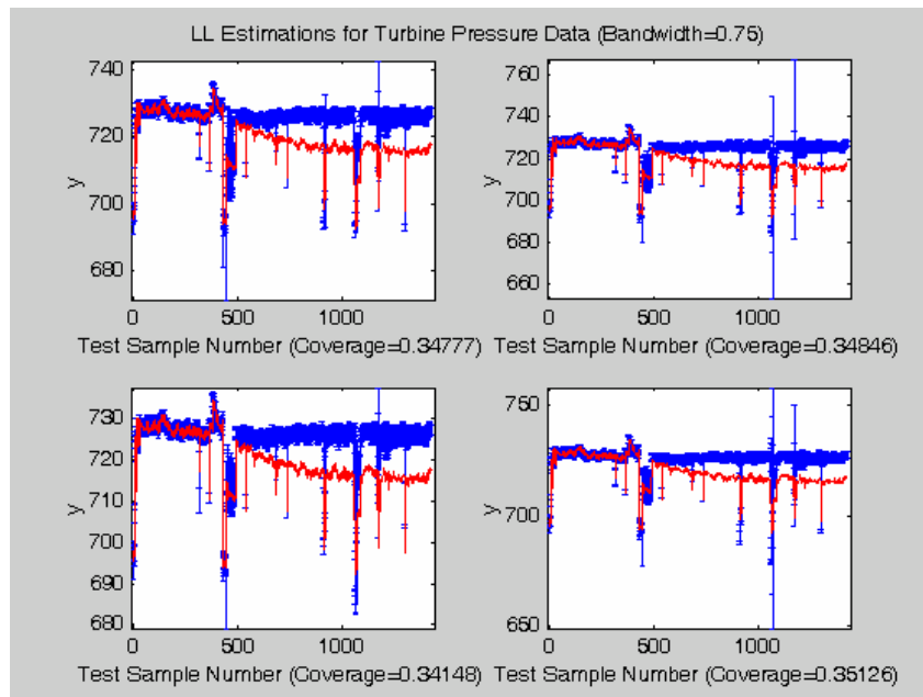
Figure 5.5.24: LL test estimations and their corresponding analytic prediction intervals. These 4 results were selected at random from the 100 available 0.75 bandwidth LL models. The coverage value for each case is indicated on the x-axis.
