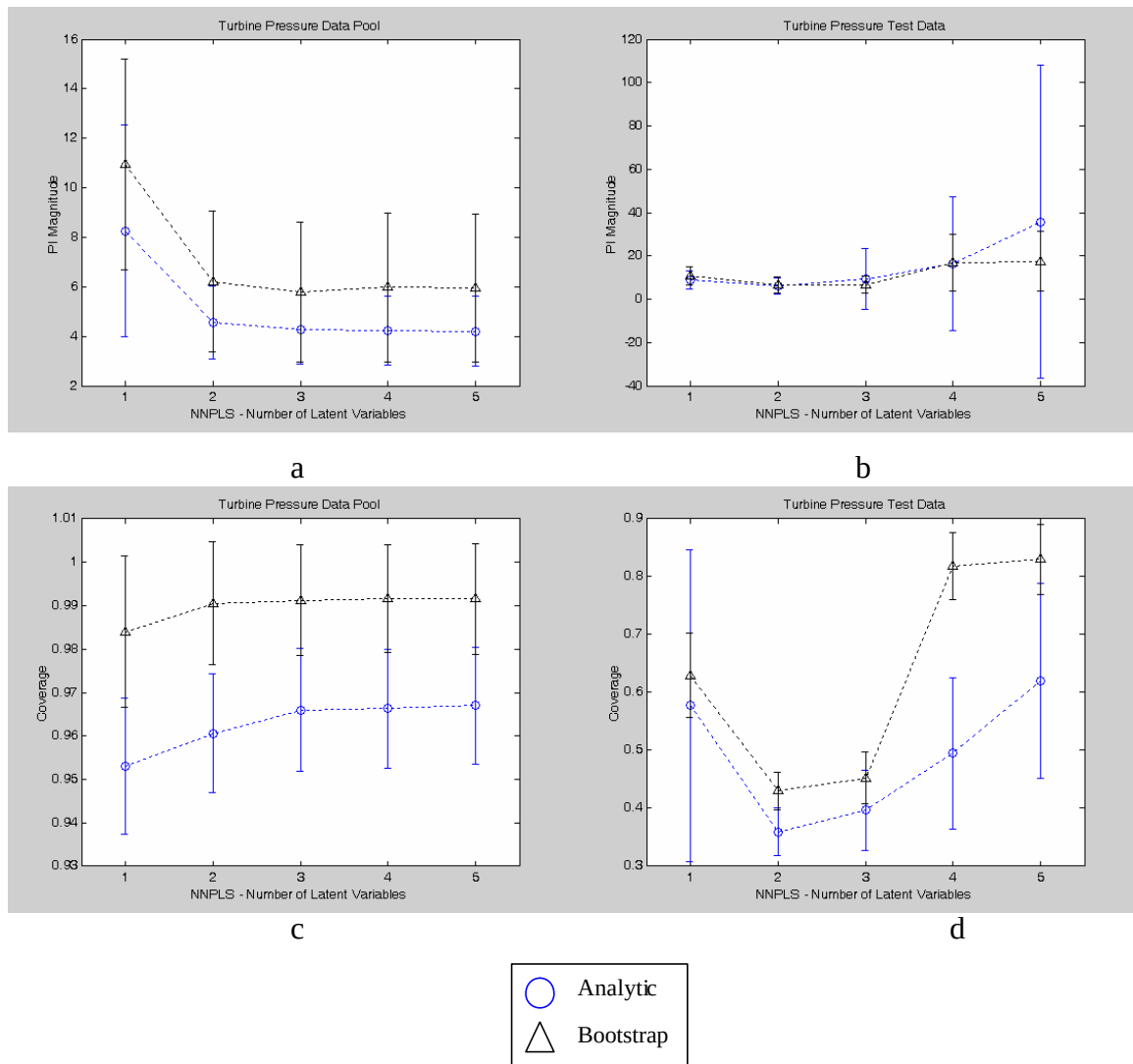
Figure 5.5.2: PI magnitude and coverage results for NNPLS models of turbine pressure data pool. The bands represent the 1s variation in the results over the 100 iterations.
