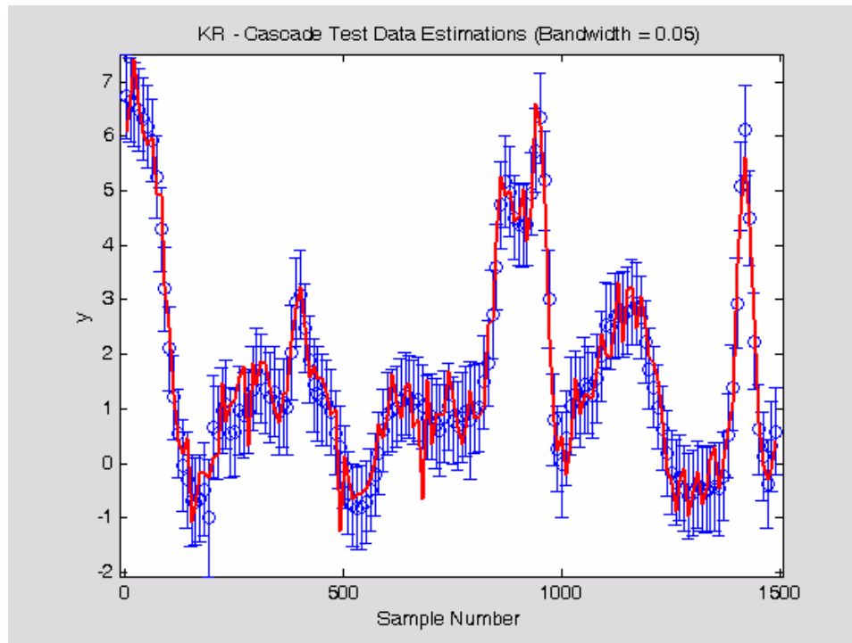
Figure 5.3.18: KR median result estimation and analytic prediction intervals Representative result for KR model (Bandwidth = 0.05) showing every 10 th estimate and the corresponding analytic prediction intervals. This model exhibited the median value of the 100 Mean Absolute Error results for the Bandwidth=0.05 models. KR – Kernel Regression.
