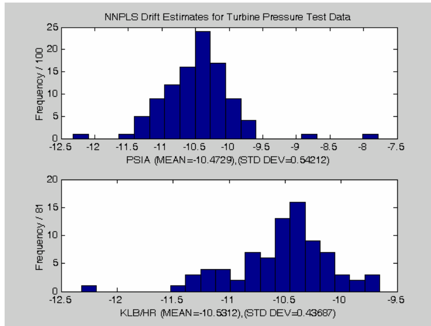
Figure 5.5.7: Distribution of drift estimate for 2 latent variable NNPLS models. Drift estimates obtained from the 100 NNPLS models via computing the MAE over test samples 600 to 1430. The upper subplot shows all results, while the lower subplot excludes any results for which coverage was greater than 5%.
