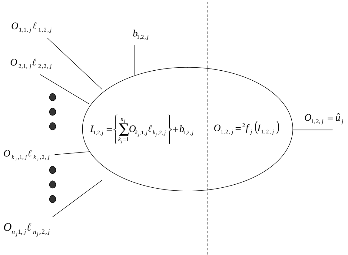
Figure 4.7.3: NNPLS output layer neuron
