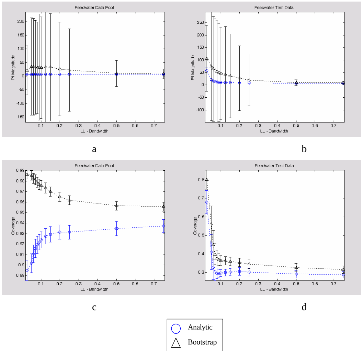
Figure 5.4.30: Prediction interval magnitude and coverage results for LL models of feedwater data pool. The bands represent the 1\sigma variation in the results over the 100 iterations.
