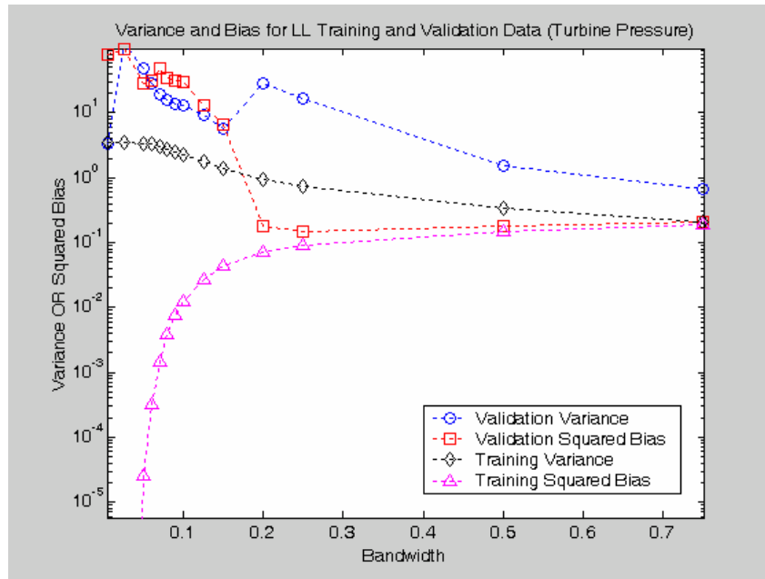
Figure 5.5.22: Variance / squared bias plots for LL models of turbine pressure training and validation data.
