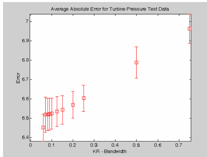
Figure 5.5.14: Mean absolute error results for KR models of turbine pressure data. The bands represent the 1s variation in the results over the 100 iterations.
