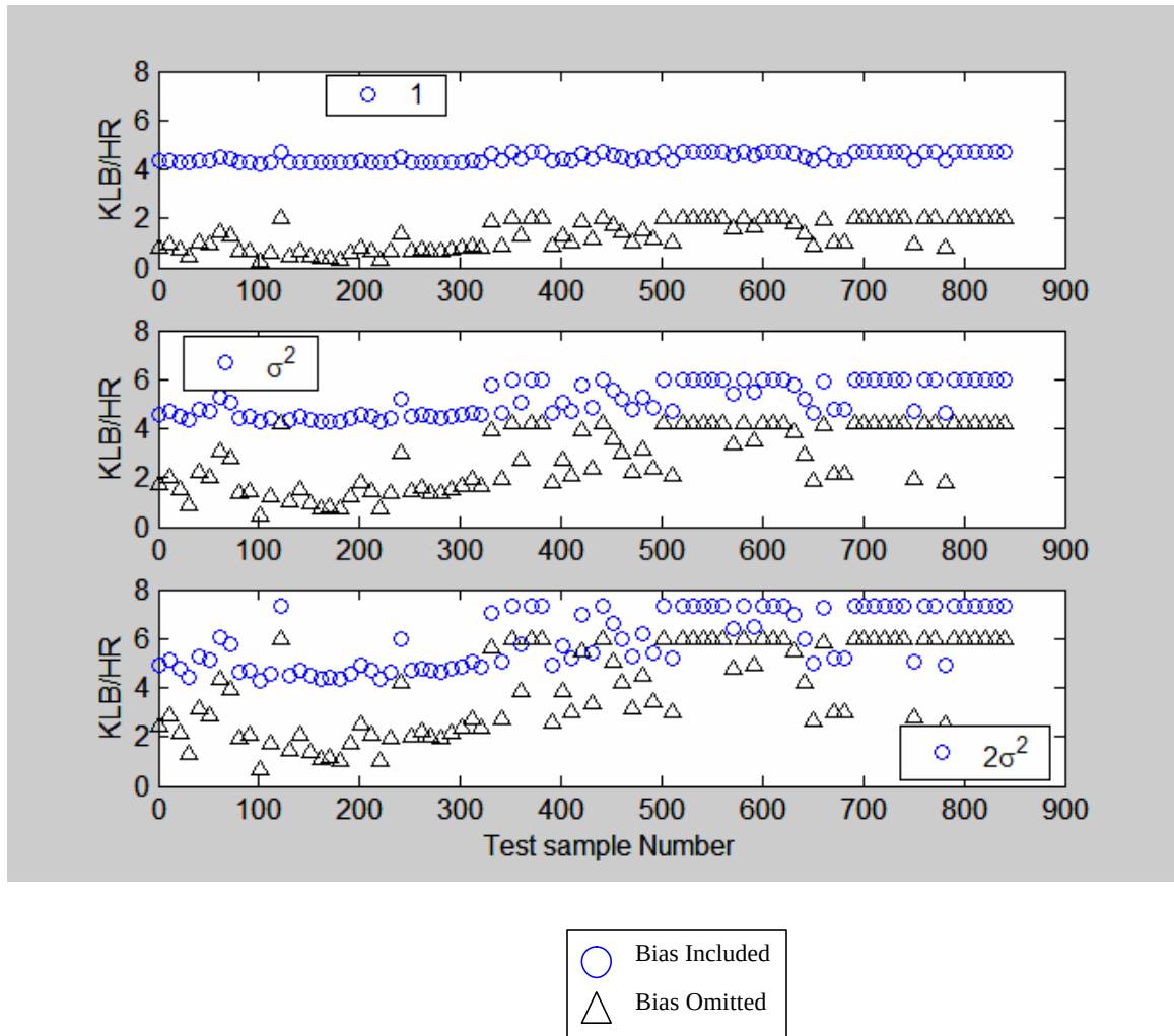
Figure 5.4.28: Analytic prediction interval magnitudes, of feedwater test data KR models, for various conditional variance estimates.
