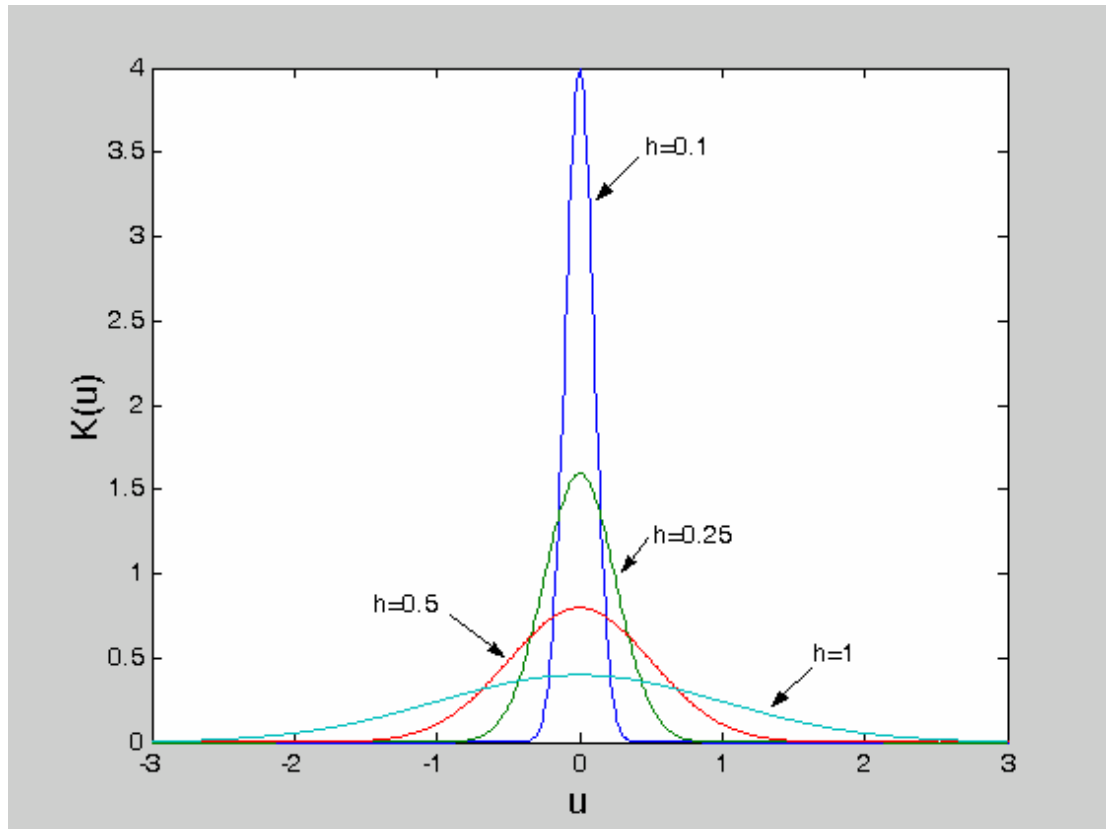
Figure 3.8.1: Gaussian kernel function for various bandwidth parameters.
