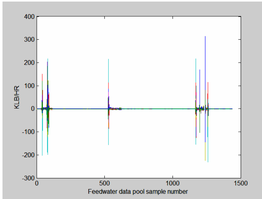
Figure 5.4.15: Deviation of estimates from the 100 KR models of the feedwater flow data pool with respect to the mean estimate for each observation.
