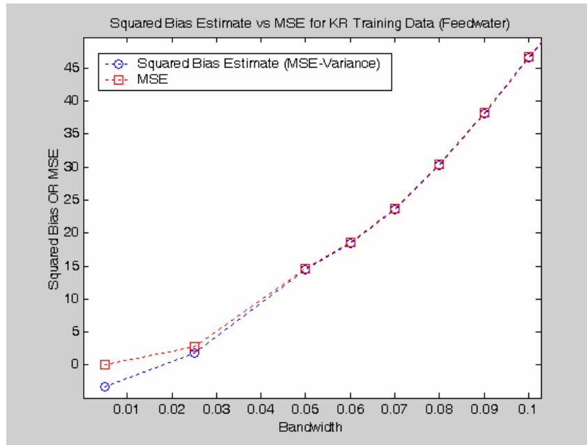
Figure 5.4.22: Comparison of feedwater flow rate data MSE and MSE-Variance.
