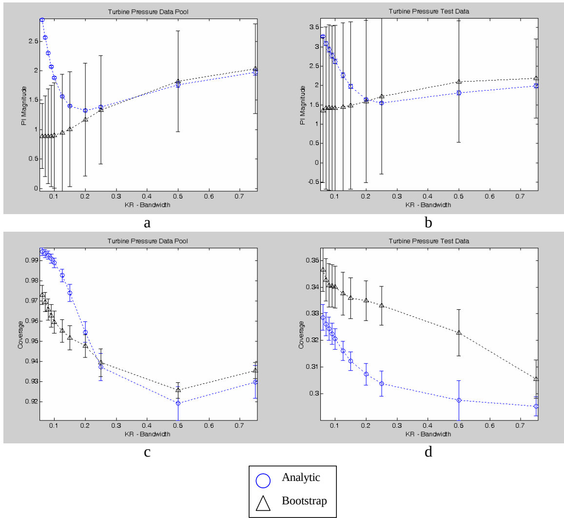
Figure 5.5.13: PI magnitude and coverage results for KR models of turbine pressure data pool. The bands represent the 1\sigma variation in the results over the 100 iterations.
