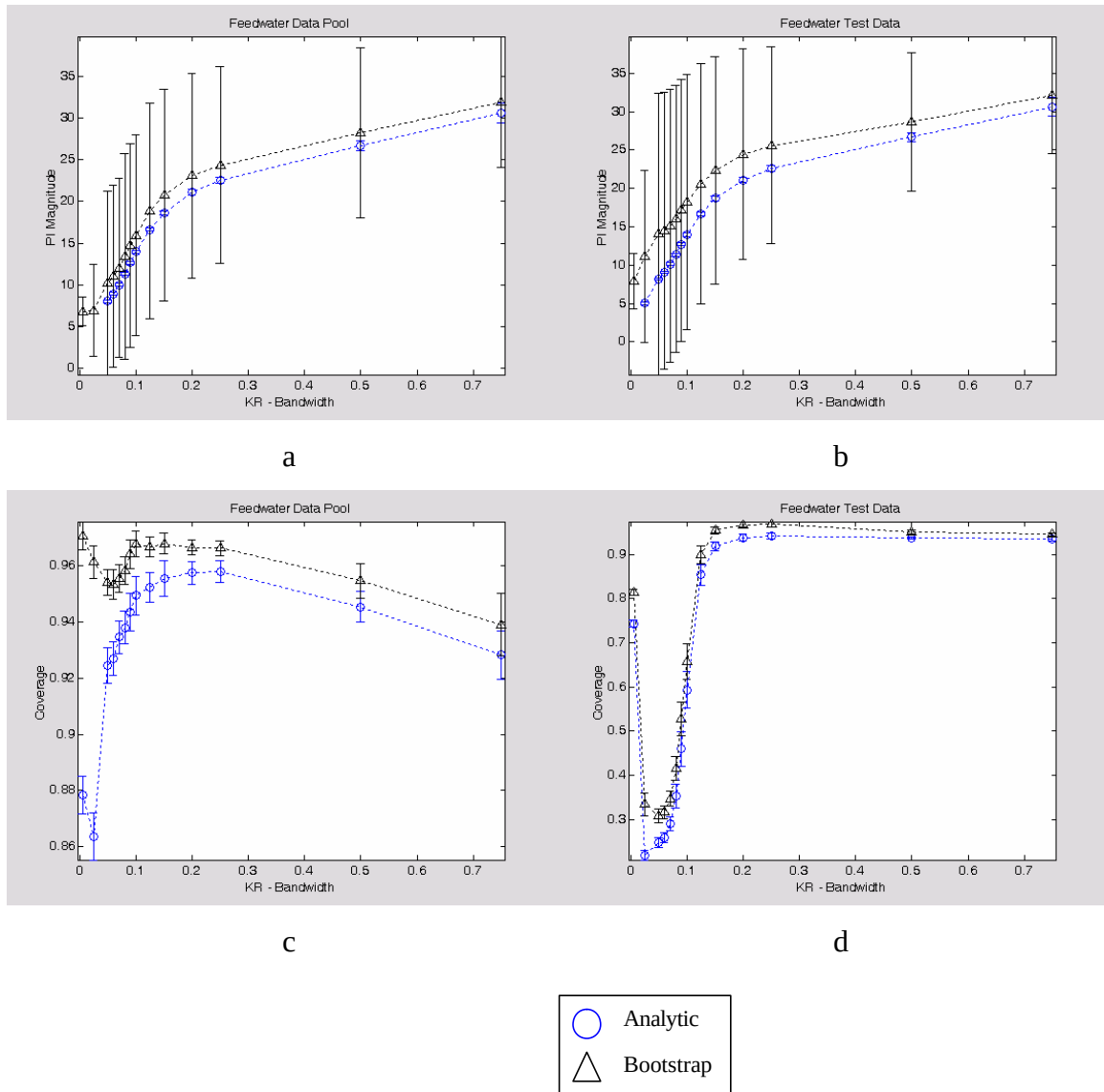
Figure 5.4.14: PI magnitude and coverage results for KR models of feedwater data pool. The bands represent the 1 \sigma variation in the results over the 100 iterations.
