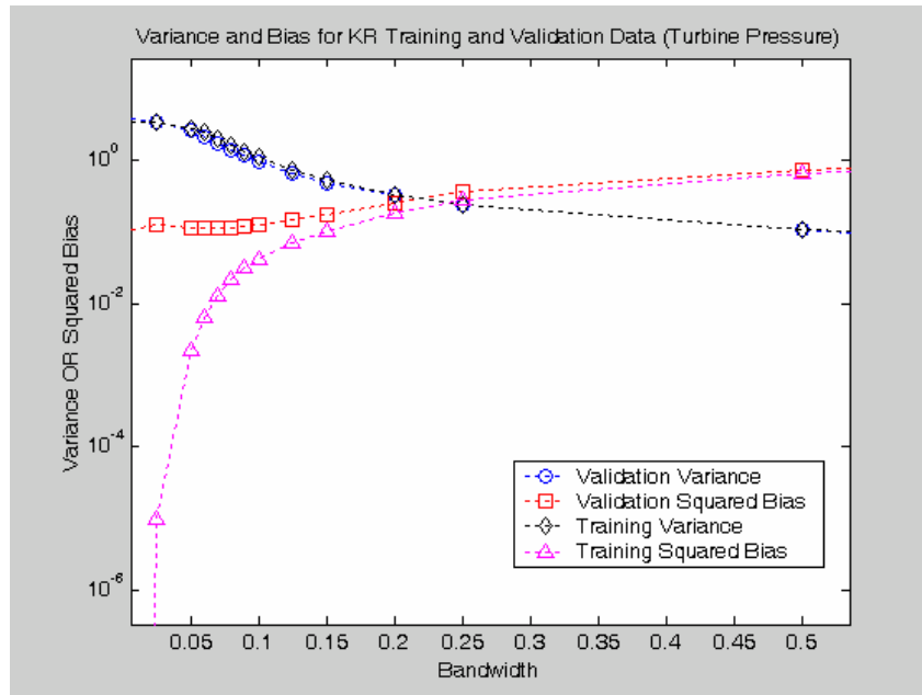
Figure 5.5.15: Variance / squared bias plots for KR models of turbine pressure training and validation data.
