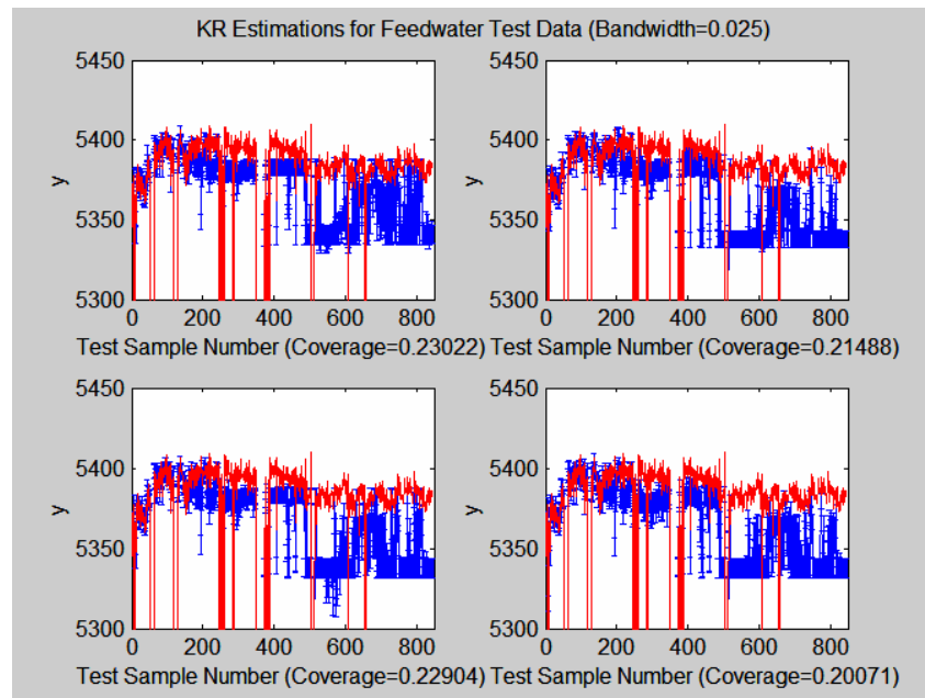
Figure 5.4.25: Test estimations and their corresponding analytic prediction intervals. These 4 results were selected at random from the 100 available KR models with bandwidth 0.025. The coverage value for each case is indicated on the x-axis.
