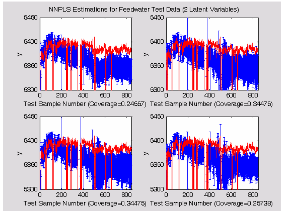
Figure 5.4.4: Test estimations and their corresponding analytic prediction intervals. These 4 results were selected at random from the 100 available 2 latent variable NNPLS models. The coverage value for each case is indicated on the x-axis.
