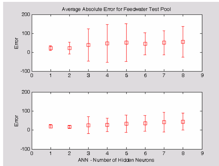
Figure 5.4.10: Mean absolute error results for ANN models of feedwater flow rate data. The bands represent the 1s variation in the results. The upper subplots provide the results for all 100 models and the lower subplots provide the result for the reduced set of models. (a) – data pool, (b) - test data
