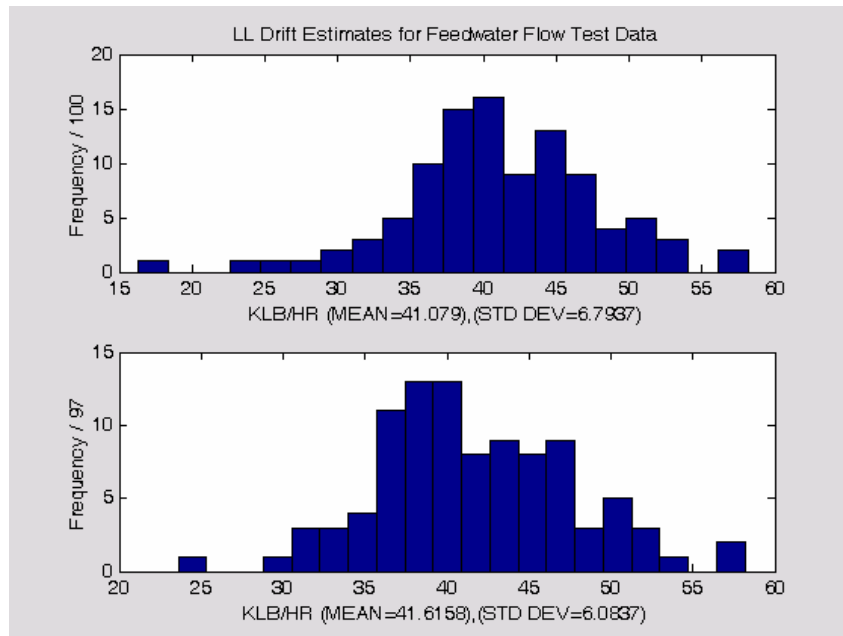
Figure 5.4.41: Distribution of drift estimate for LL models of bandwidth 0.08. Drift estimates obtained from the 100 LL models via computing the MAE over test samples 700 to 847. The upper subplot shows all results, while the lower subplot excludes any results for which coverage was greater than 5%.
