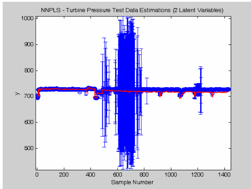
Figure 5.5.5: NNPLS median result estimation and analytic prediction intervals. Representative result of NNPLS 2 latent variable models. This model exhibited the median value of the 100 Mean Absolute Error results for the 2 latent variable models.
