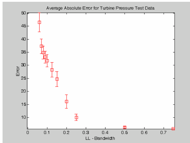
Figure 5.5.21: Mean absolute error results for LL models of turbine pressure data. The bands represent the 1s variation in the results over the 100 iterations.
