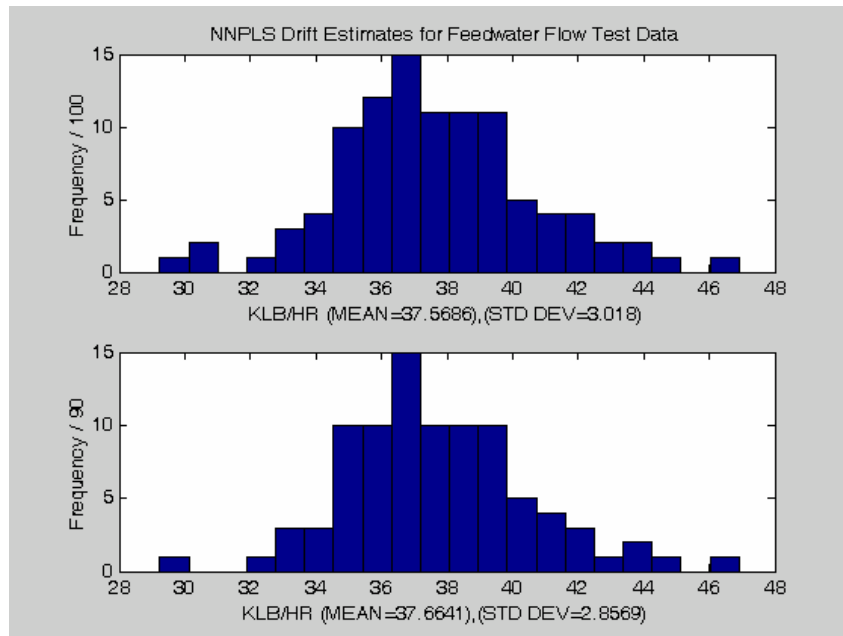
Figure 5.4.6: Distribution of drift estimate for 2 latent variable NNPLS models. Drift estimates obtained from the 100 NNPLS models via computing the MAE over test samples 700 to 847. The upper subplot shows all results, while the lower subplot excludes any results for which coverage was greater than 5%.
