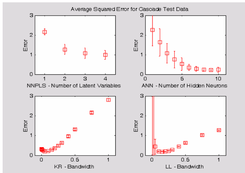
Figure 5.3.8: Error Results for Cascade Test Data.
