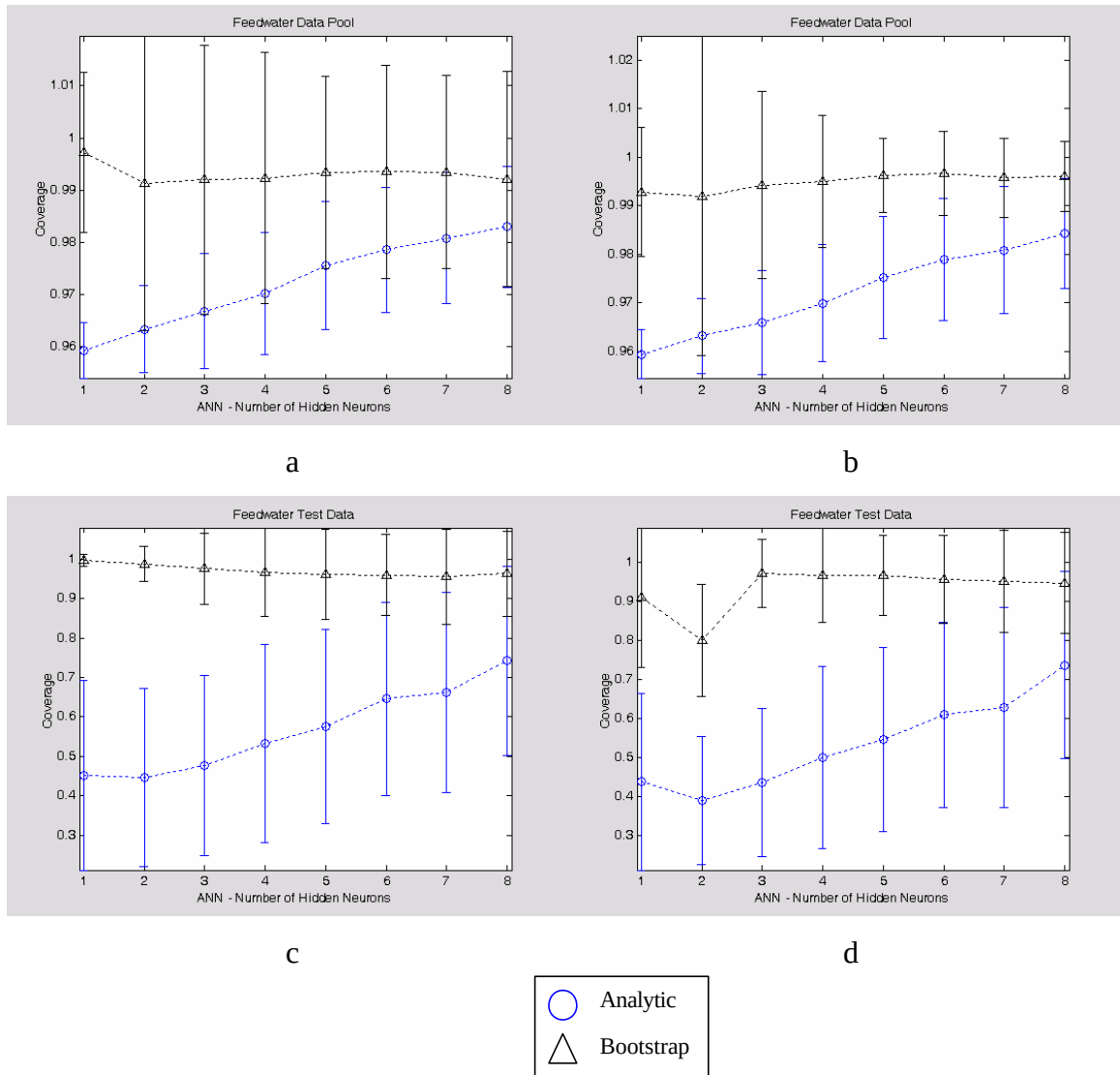
Figure 5.4.9: Coverage values for ANN models of feedwater data pool and test data. The bands represent the 1s variation in the results over the 100 iterations. (a) and (c) provide results for all 100 iterations and (b) and (d) provide results for a reduced set of models as explained below.
