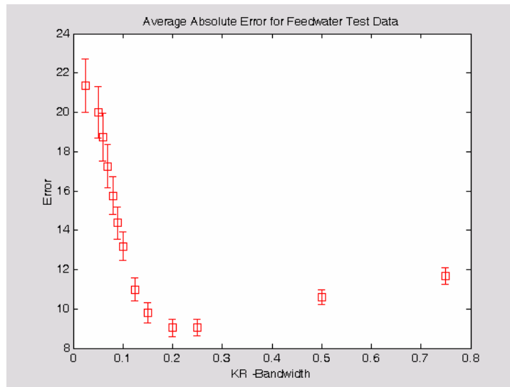
Figure 5.4.20: Mean absolute error results for KR models of feedwater flow rate data. The bands represent the 1-sigma variation in the results over the 100 iterations. (a) – data pool, (b) – test data.
