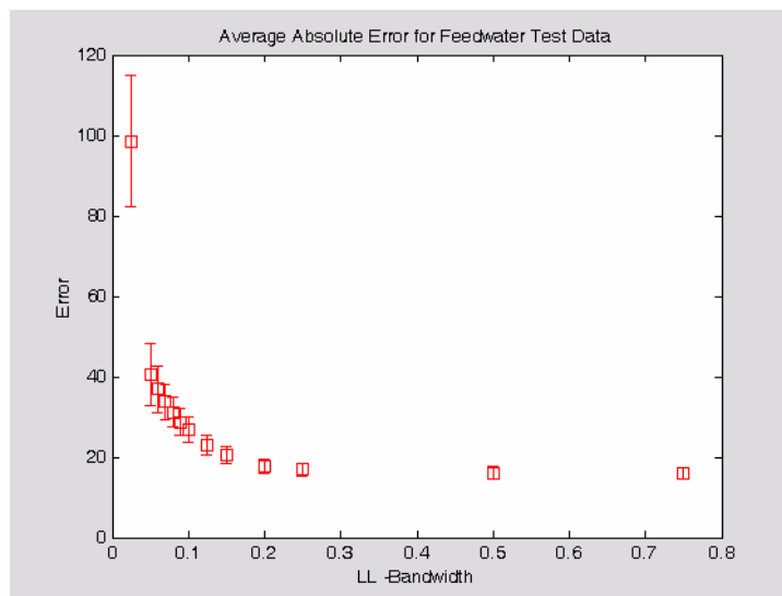
Figure 5.4.35: Mean absolute error results for LL models of feedwater flow rate data.
