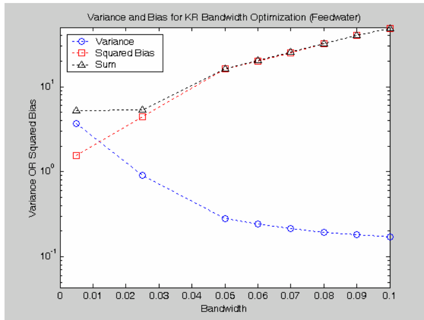
Figure 5.4.24: Combined variance of training and validation data vs. squared bias of data pool for KR models of feedwater flow rate data.
