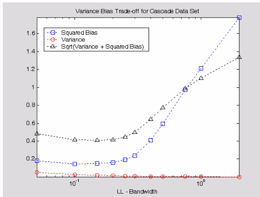
Figure 5.3.9: Bias and Variance plots for cascade data.
