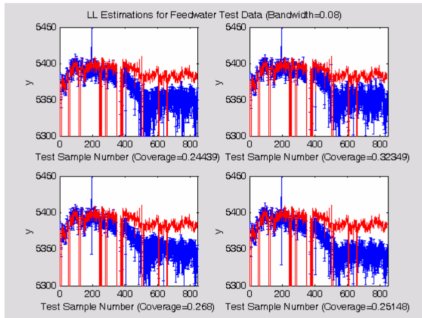
Figure 5.4.38: Test estimations and their corresponding analytic prediction intervals. These 4 results were selected at random from the 100 available LL models with bandwidth 0.08. The coverage value for each case is indicated on the x-axis.
