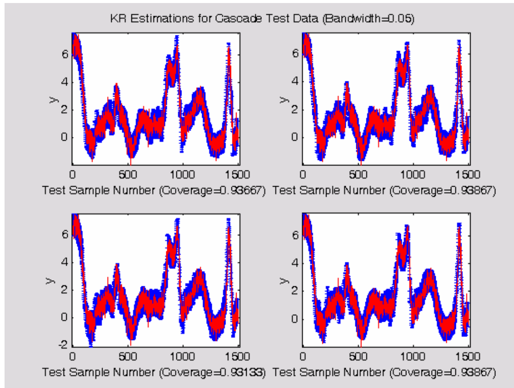
Figure 5.3.14: KR cascade test data estimations and analytic prediction intervals.
