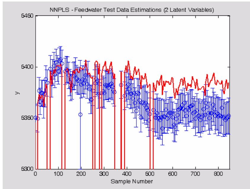
Figure 5.4.5: NNPLS median result estimation and analytic prediction intervals. Representative result for NNPLS 2 latent variable model showing every 5 th estimate and the corresponding analytic prediction intervals. This model exhibited the median value of the 100 Mean Absolute Error results for the 2 latent variable models.
