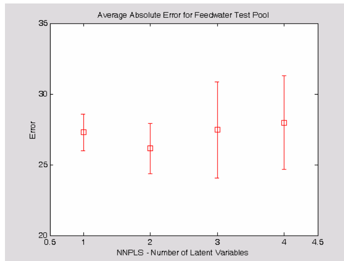
Figure 5.4.3: Mean absolute error results for NNPLS models of feedwater flow rate data pool (a) and test data (b).
