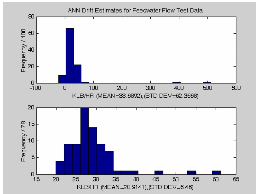
Figure 5.4.13: Distribution of drift estimate for 2 hidden neuron ANN models. Drift estimates obtained from the 100 ANN models via computing the MAE over test samples 700 to 847. The upper subplot shows all results, while the lower subplot excludes any results for which coverage was greater than 5%.
