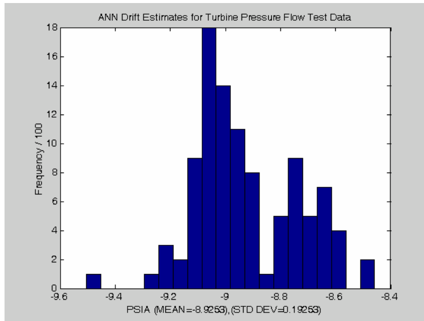
Figure 5.5.12: Distribution of drift estimate from 2 hidden neuron ANN models. Drift estimates obtained from the 100 ANN models via computing the MAE over test samples 600 to 1430. All 100 models provided \leq 5\% coverage in the region of drift.
