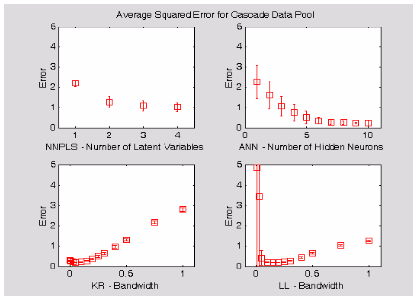
Figure 5.3.7: Error Results for Cascade Data Pool.
