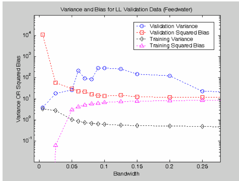
Figure 5.4.36: Variance / squared bias plots for LL models of feedwater flow rate training data and validation data.
