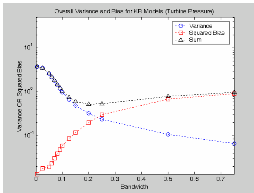
Figure 5.5.16: Combined variance of training and validation data vs. squared bias of data pool for KR models of turbine pressure data.
