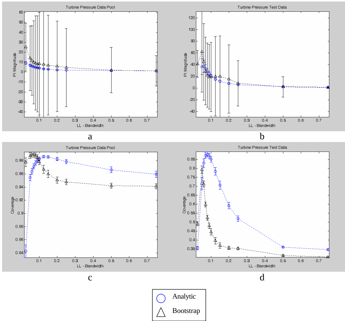
Figure 5.5.20: PI magnitude and coverage results for LL models of turbine pressure data pool. The bands represent the 1s variation in the results over the 100 iterations.
