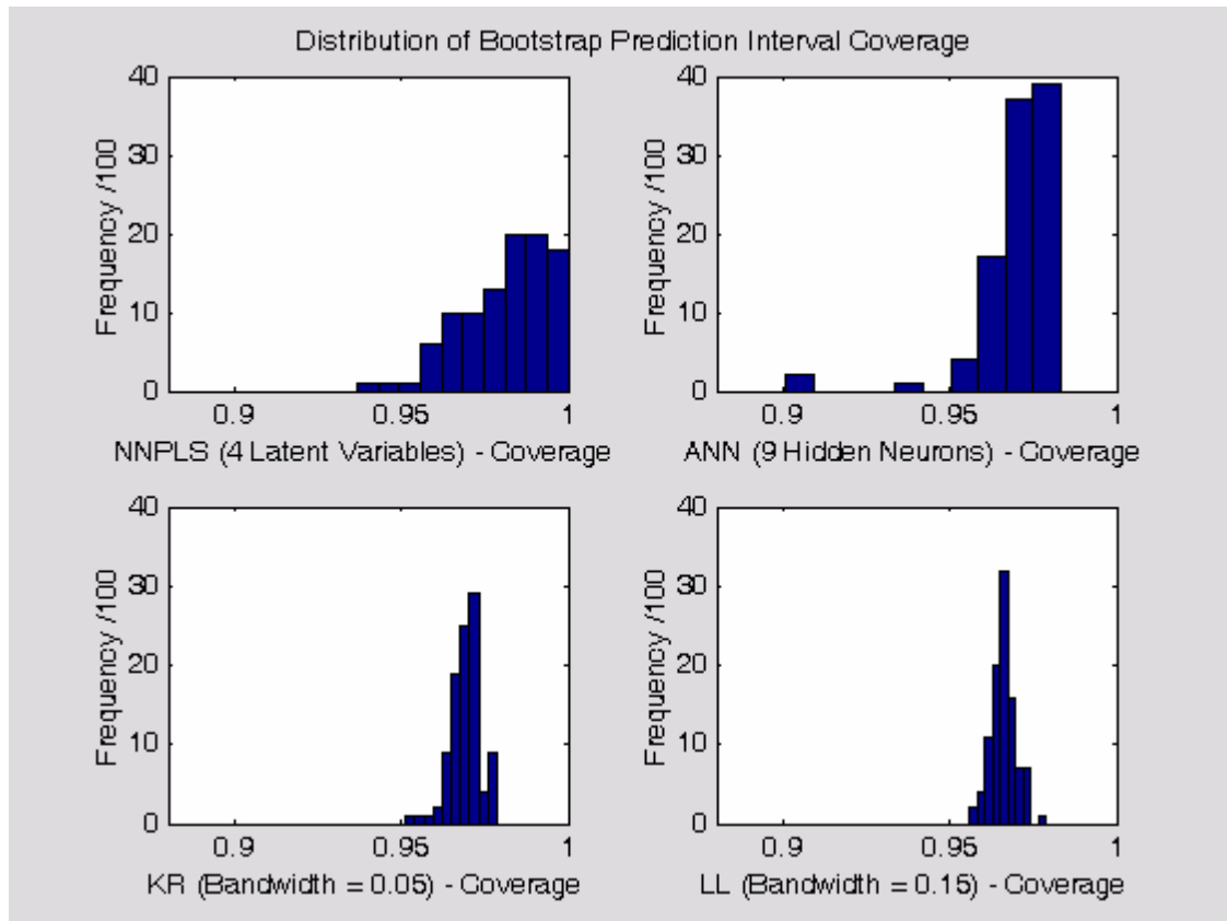
Figure 5.3.11: Bootstrap prediction interval coverage values for cascade test data set. The plot shows the distributions of the coverage values for the bootstrap prediction intervals over 100 iterations. These coverage values are with respect to the Cascade Test Data, and were based on the coverage of the bootstrap prediction intervals using the squared error bias estimate. NNPLS – Neural Network Partial Least Squares, ANN – Artificial Neural Network, KR – Kernel Regression, LL – Local Linear Regression.
