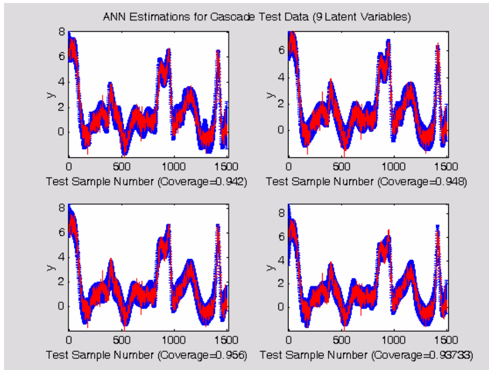
Figure 5.3.13: ANN cascade test data estimations and analytic prediction intervals.
