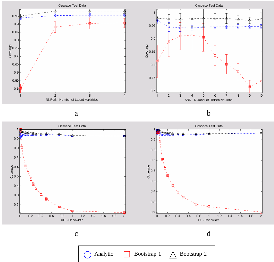
Figure 5.3.6: Coverage Results for Cascade Test Data.
