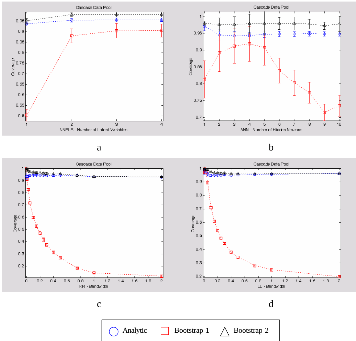
Figure 5.3.5: Coverage Results for Cascade Data Pool.
