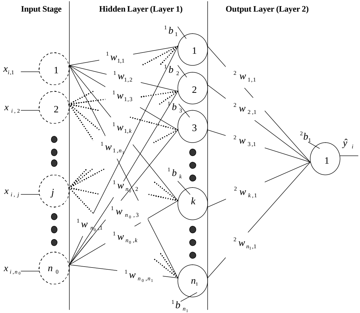
Figure 4.6.1: Schematic of an inferential ANN
