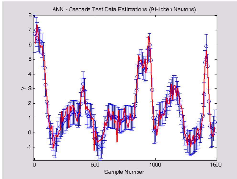
Figure 5.3.17: ANN median result estimation and analytic prediction intervals Representative result for ANN 9 hidden neuron model showing every 10 th estimate and the corresponding analytic prediction intervals. This model exhibited the median value of the 100 Mean Absolute Error results for the 9 hidden neuron models. ANN – Artificial Neural Network.
