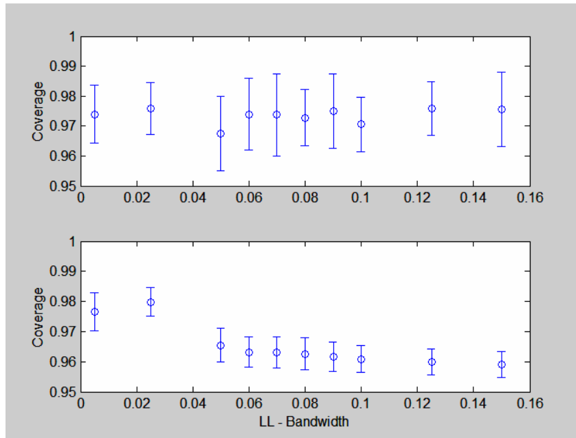
Figure 5.4.34: Original and modified bootstrap prediction interval coverage values for LL models of feedwater flow rate data pool.
