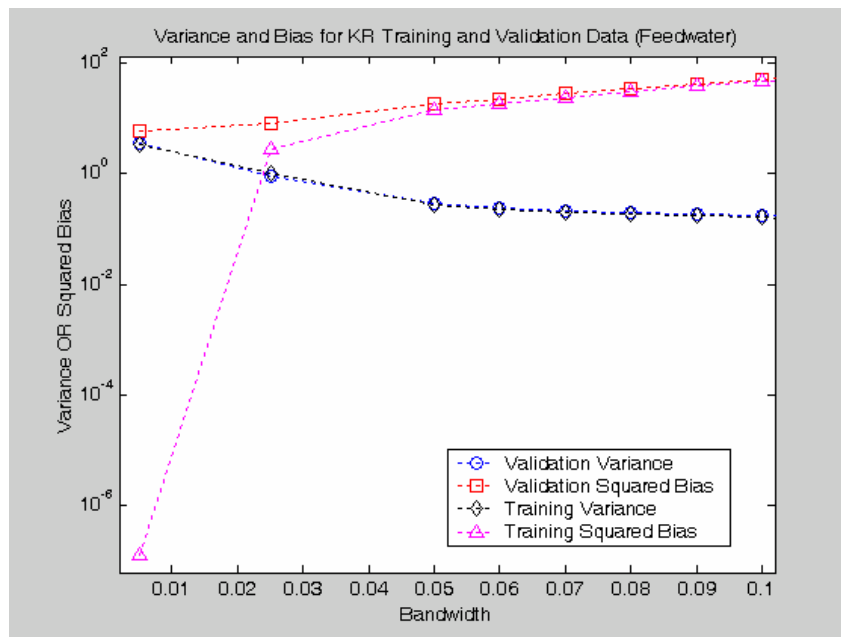
Figure 5.4.23: Variance / squared bias plots for KR models of feedwater flow rate training data and validation data.
