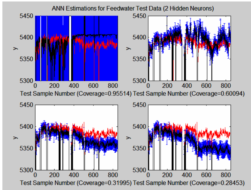
Figure 5.4.11: Test estimations and their corresponding analytic prediction intervals. These 4 results were selected at random from the 100 available 2 hidden neuron ANN models. The coverage value for each case is indicated on the x-axis.
