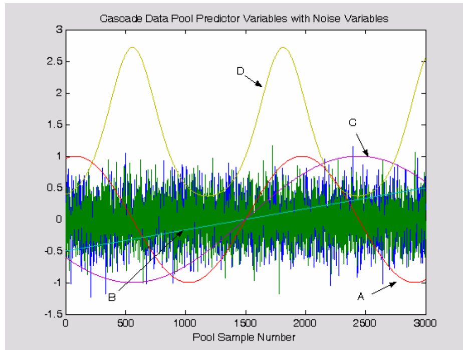
Figure 5.3.20: Cascade Data Pool predictor variables with 2 additional noise variables.
