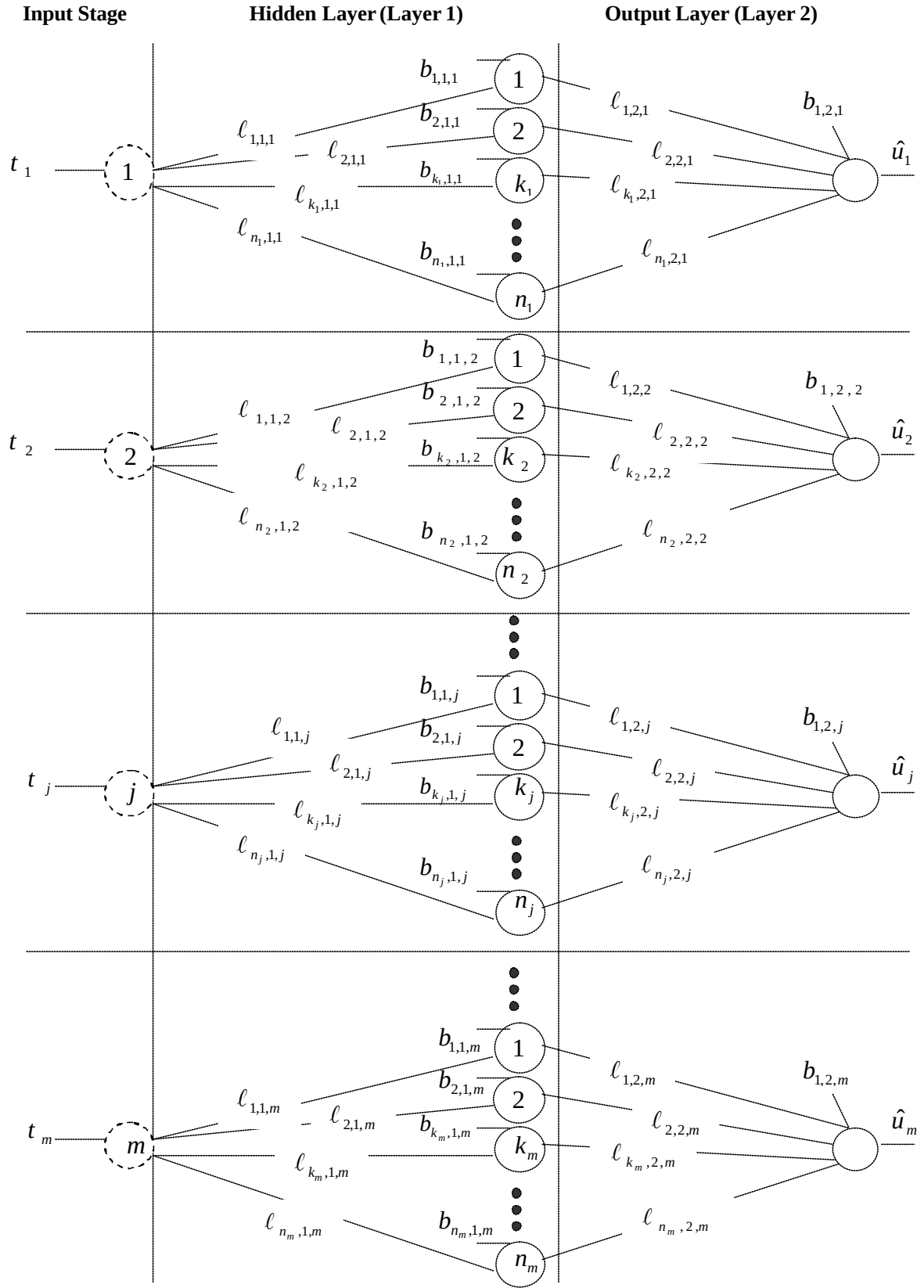
Figure 4.7.2: Schematic of the inner relationships of the NNPLS-1 model
