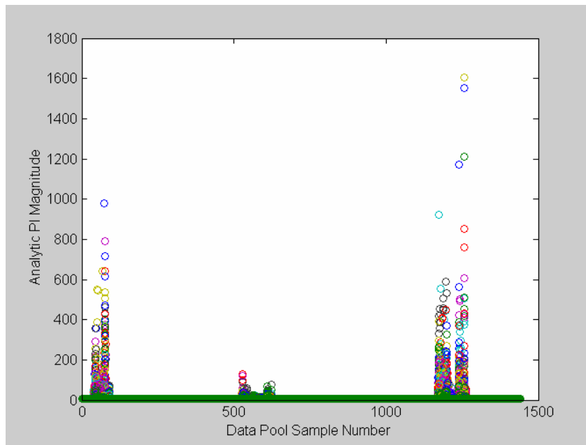
Figure 5.4.32: Analytic prediction intervals for all 100 LL models of feedwater flow rate data pool, bandwidth = 0.08.
