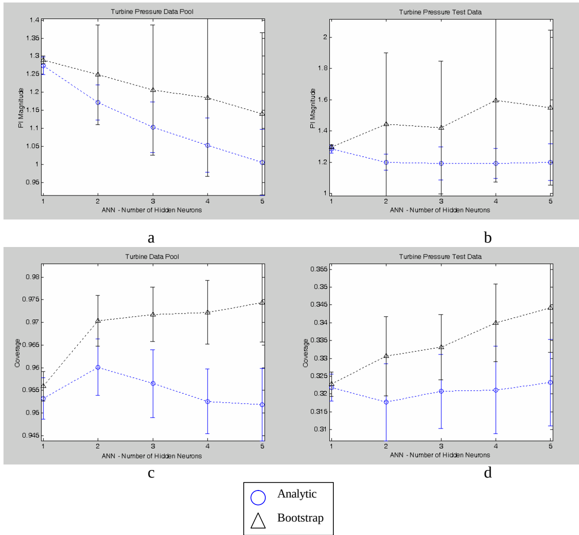
Figure 5.5.8: PI magnitude and coverage results for ANN models of turbine pressure data pool. The bands represent the 1s variation in the results over the 100 iterations.
