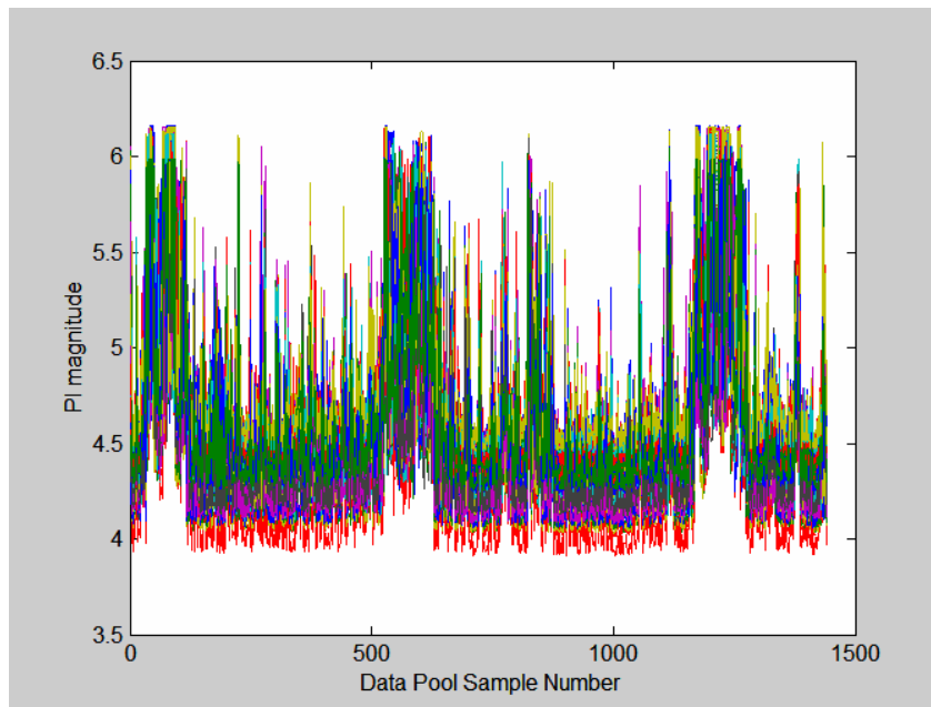
Figure 5.4.17: Analytic prediction intervals for all 100 KR models of feedwater flow rate data pool, bandwidth = 0.025.
