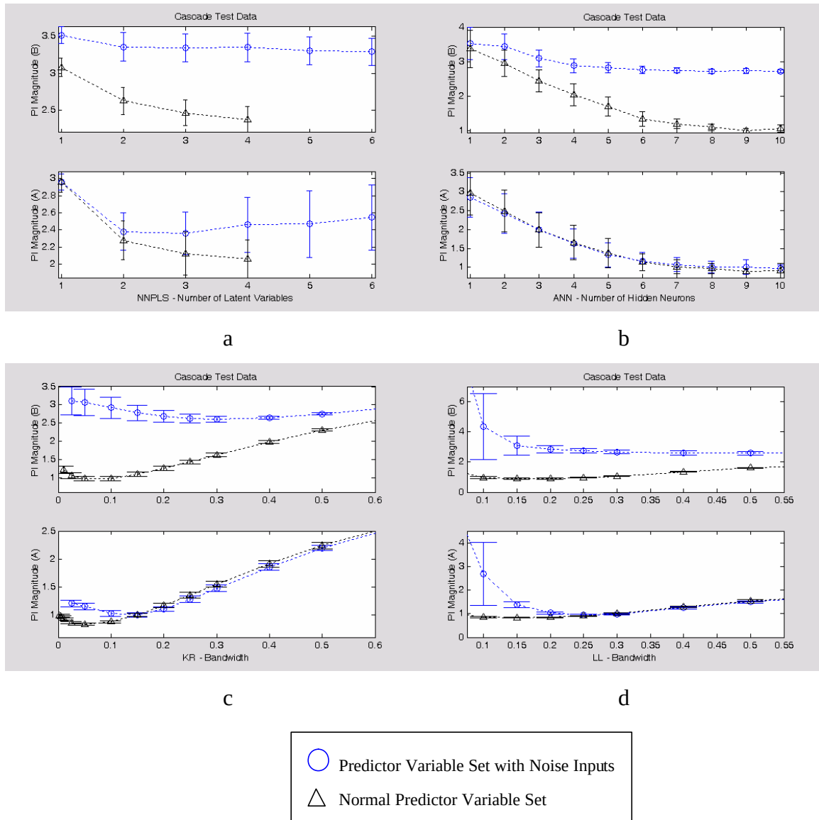
Figure 5.3.21: Comparison of PI magnitude results for Cascade Test Data Pool for normal set of predictors and the augmented set that included 2 normal random variables. The models used are specified along the x-axis. The bands represent the 1s variation in the results over the 100 iterations. The upper subplot of each plot contains the results based on the analytic prediction interval methods, indicated by an (A) on the y-axis. The lower subplot of each plot contains the results based on the bootstrap prediction intervals utilizing the squared error bias estimate (For more information, see section 4.10), and is indicated by a (B) on the y-axis. NNPLS – Neural Network Partial Least Squares, ANN – Artificial Neural Network, KR – Kernel Regression, LL – Local Linear Regression.
