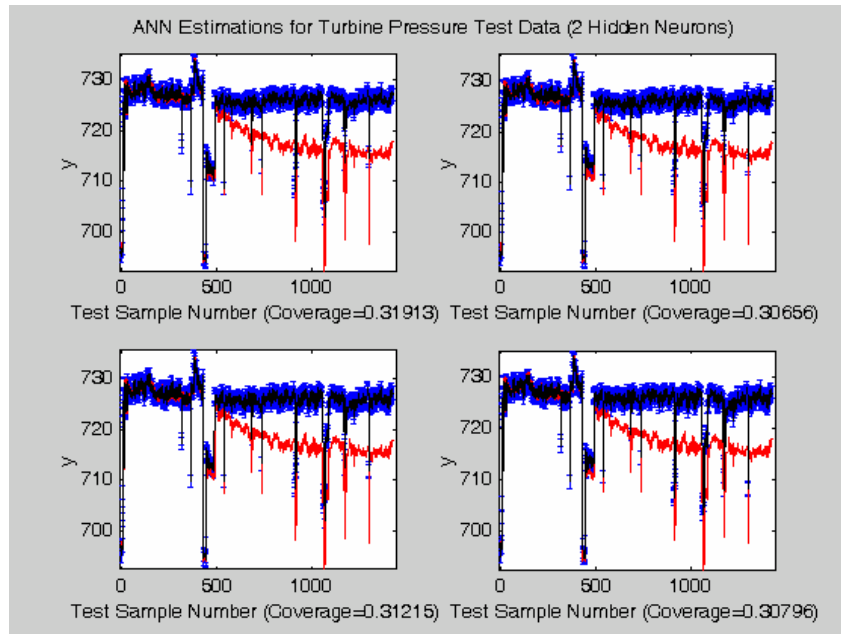
Figure 5.5.10: ANN test estimations and their corresponding analytic prediction intervals. These 4 results were selected at random from the 100 available 2 hidden neuron ANN models. The coverage value for each case is indicated on the x-axis.
