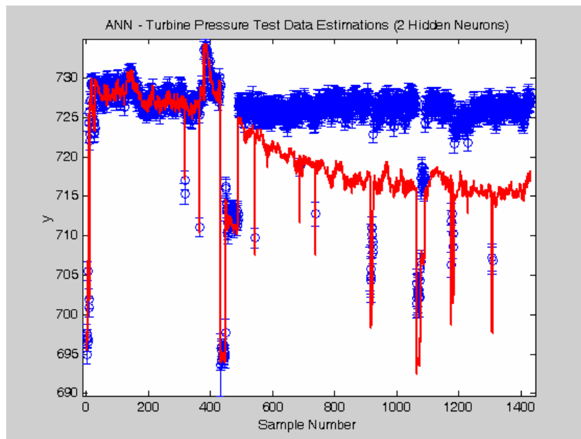
Figure 5.5.11: ANN median result estimation and analytic prediction intervals. Representative result of 2 hidden neuron ANN models. This model exhibited the median value of the 100 Mean Absolute Error results for the 2 hidden neuron models.
