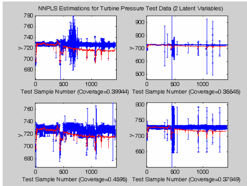
Figure 5.5.4: NNPLS test estimations and their corresponding analytic prediction intervals.
