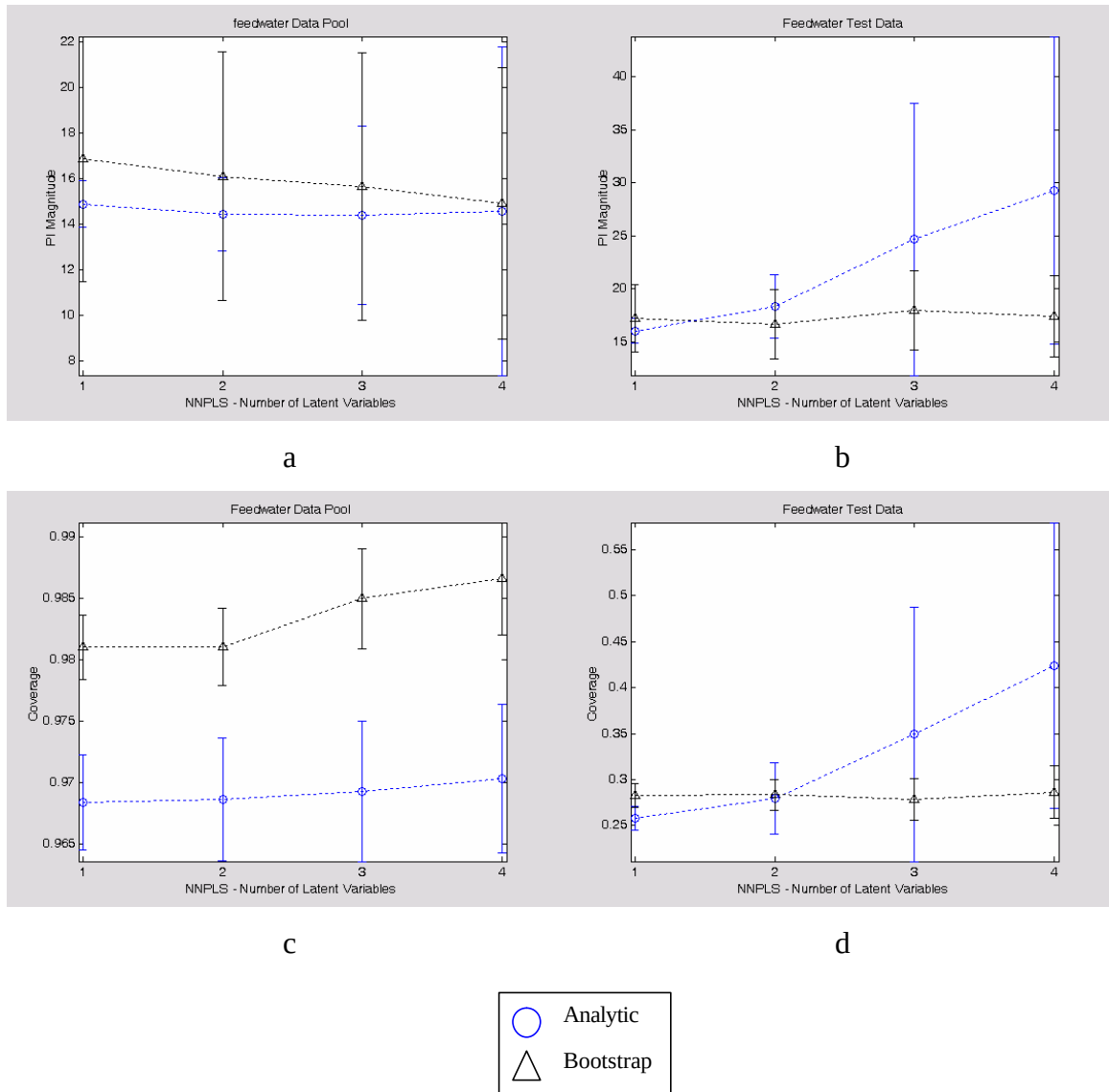
Figure 5.4.2: PI magnitude and coverage results for NNPLS models of feedwater data pool. The bands represent the 1s variation in the results over the 100 iterations.
