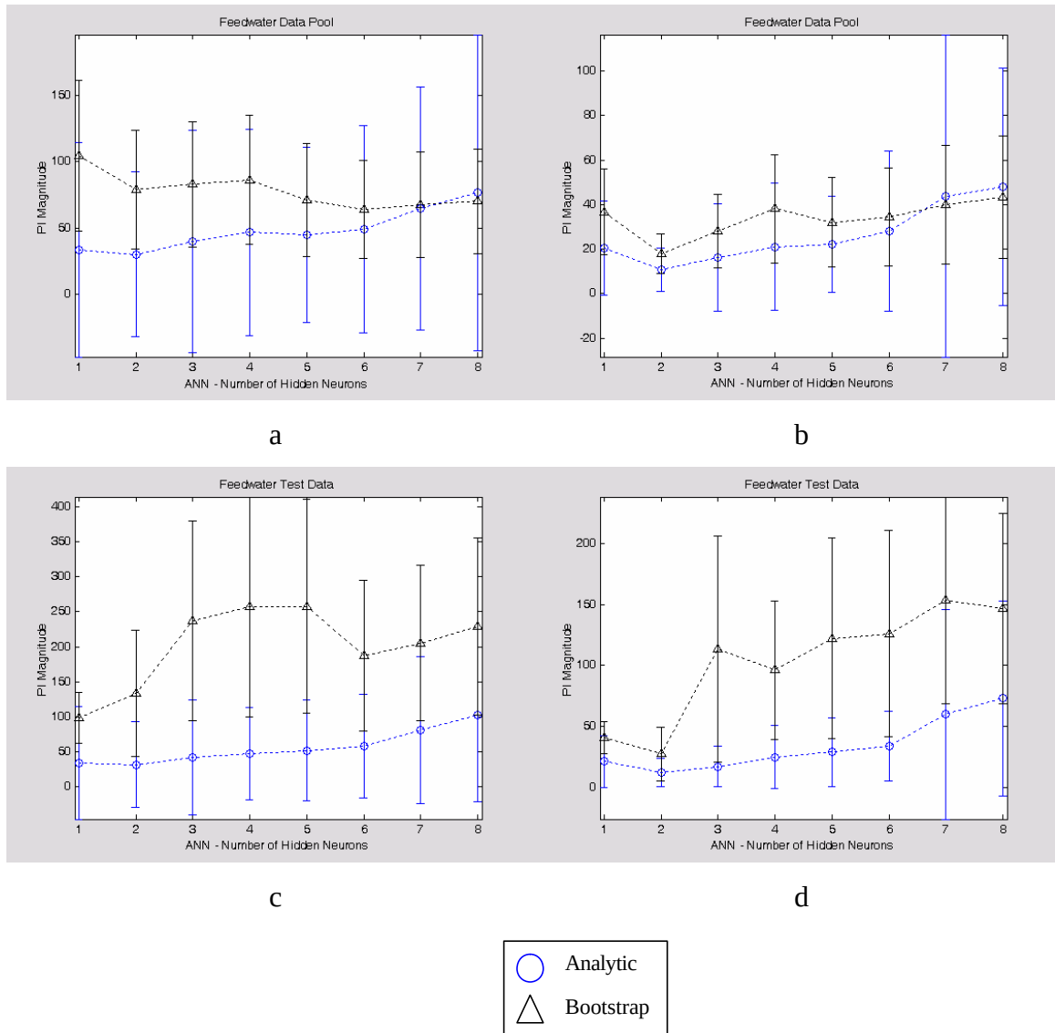
Figure 5.4.7: PI magnitude results for ANN models of feedwater data pool and test data. The bands represent the 1s variation in the results over the 100 iterations. (a) and (c) provide results for all 100 iterations and (b) and (d) provide results for a reduced set of models as explained below.
