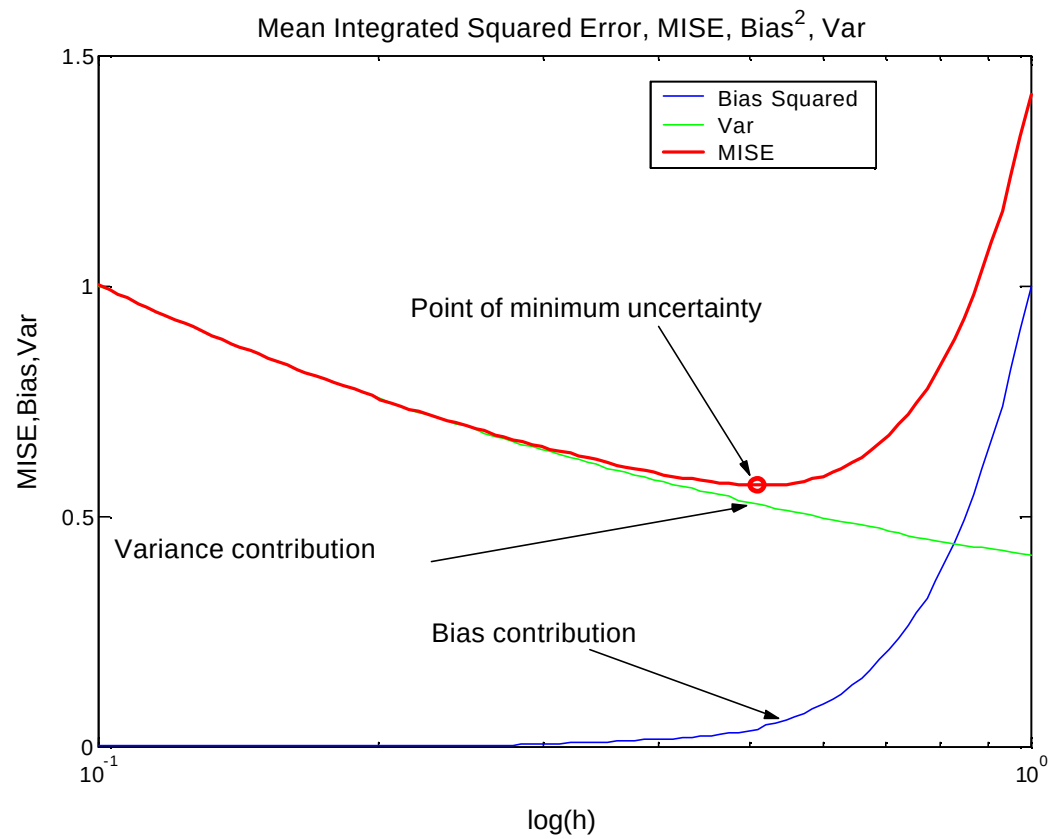
Figure 4.9.1: Nonparametric regression bias / variance trade-off.
