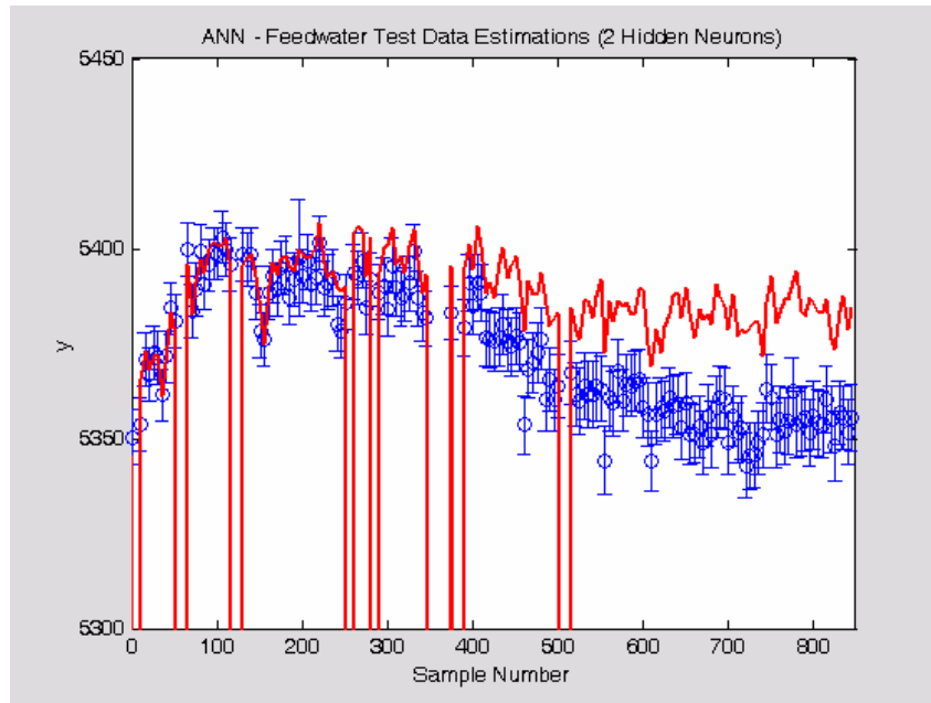
Figure 5.4.12: ANN median result estimation and analytic prediction intervals. Representative results for 2 hidden neuron ANN model showing every 5 th estimate and the corresponding analytic prediction intervals. This model exhibited the median value of the 100 Mean Absolute Error results for the 2 hidden neuron models.
