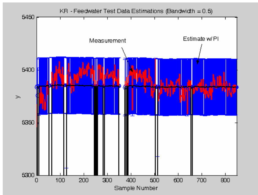
Figure 5.4.27: Example of an over-regularized fit of a KR model to the feedwater flow rate test data (bandwidth=0.5).
