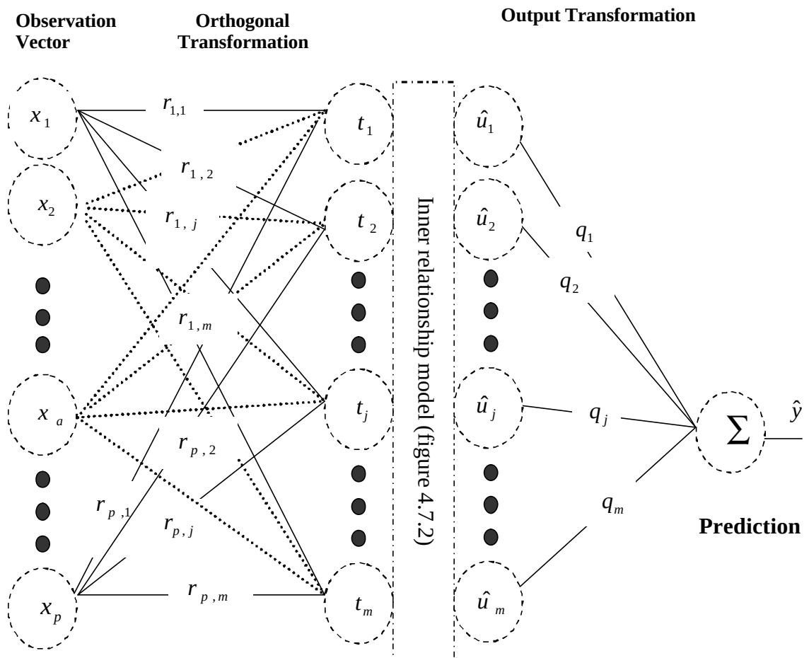
Figure 4.7.1: Schematic of the outer relationships of an inferential NNPLS model.
