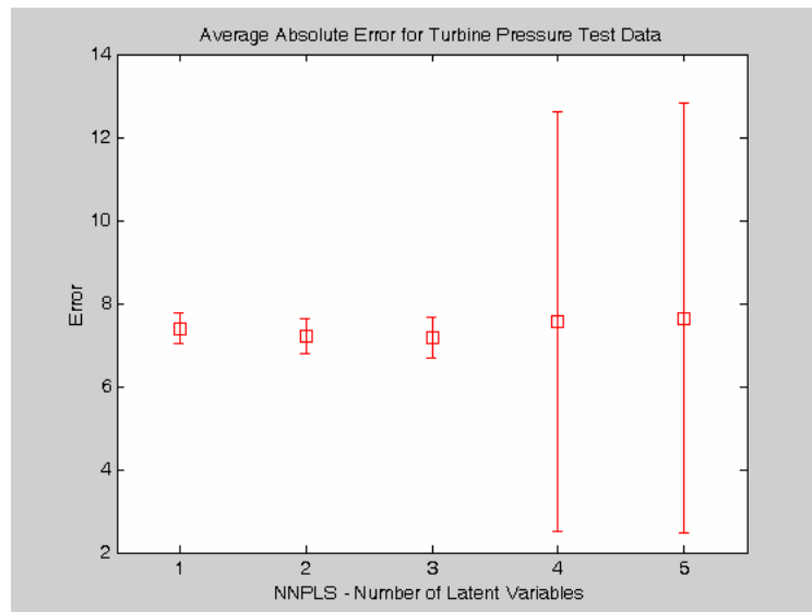
Figure 5.5.3: Mean absolute error results for NNPLS models of turbine pressure data. The bands represent the 1σ variation in the results over the 100 iterations. (a) – data pool, (b) – test data
