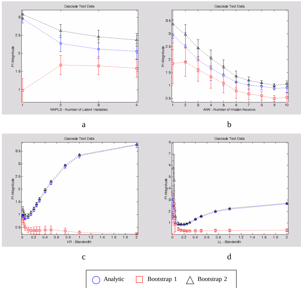
Figure 5.3.4: PI Magnitude Results for Cascade Test Data.
