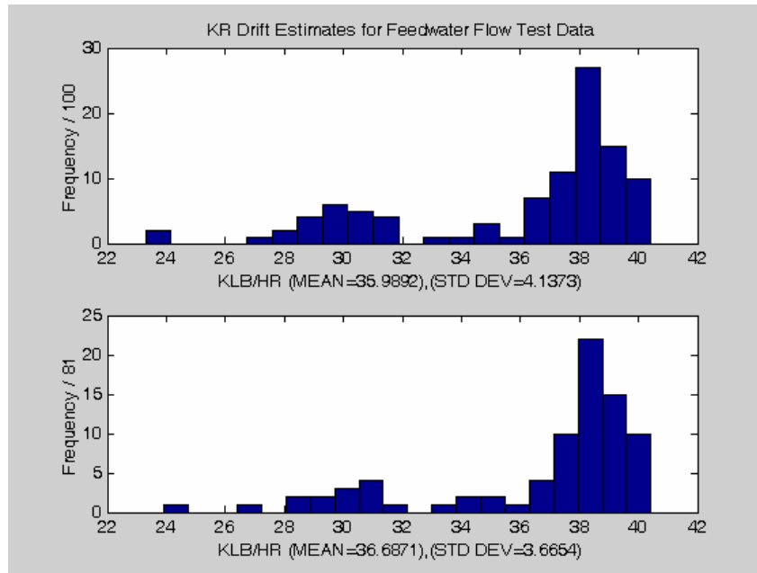
Figure 5.4.29: Distribution of drift estimate for KR models of bandwidth 0.025. Drift estimates obtained from the 100 KR models via computing the MAE over test samples 700 to 847. The upper subplot shows all results, while the lower subplot excludes any results for which coverage was greater than 5%.
