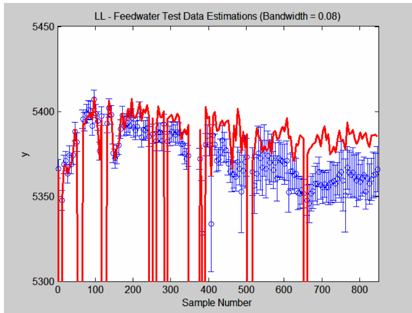
Figure 5.4.39: LL median result estimation and analytic prediction intervals. Representative results for LL model of bandwidth=0.08 showing every 5 th estimate and the corresponding analytic prediction intervals. This model exhibited the median value of the 100 Mean Absolute Error results for the LL models with a bandwidth of 0.08
