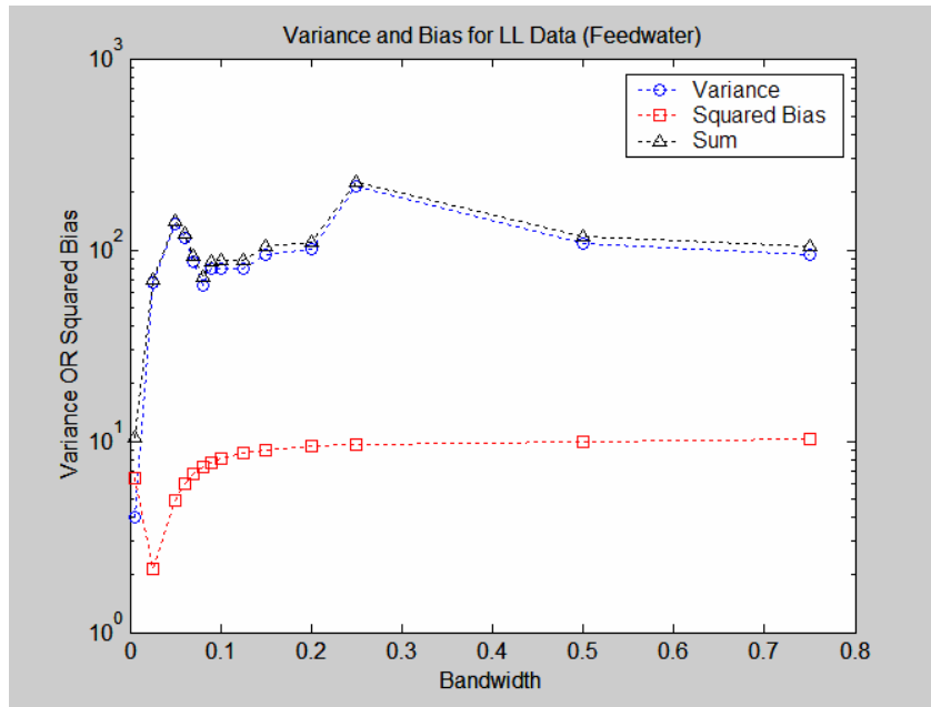
Figure 5.4.37: Combined variance of training and validation data vs. squared bias of data pool for LL models of feedwater flow rate data.
