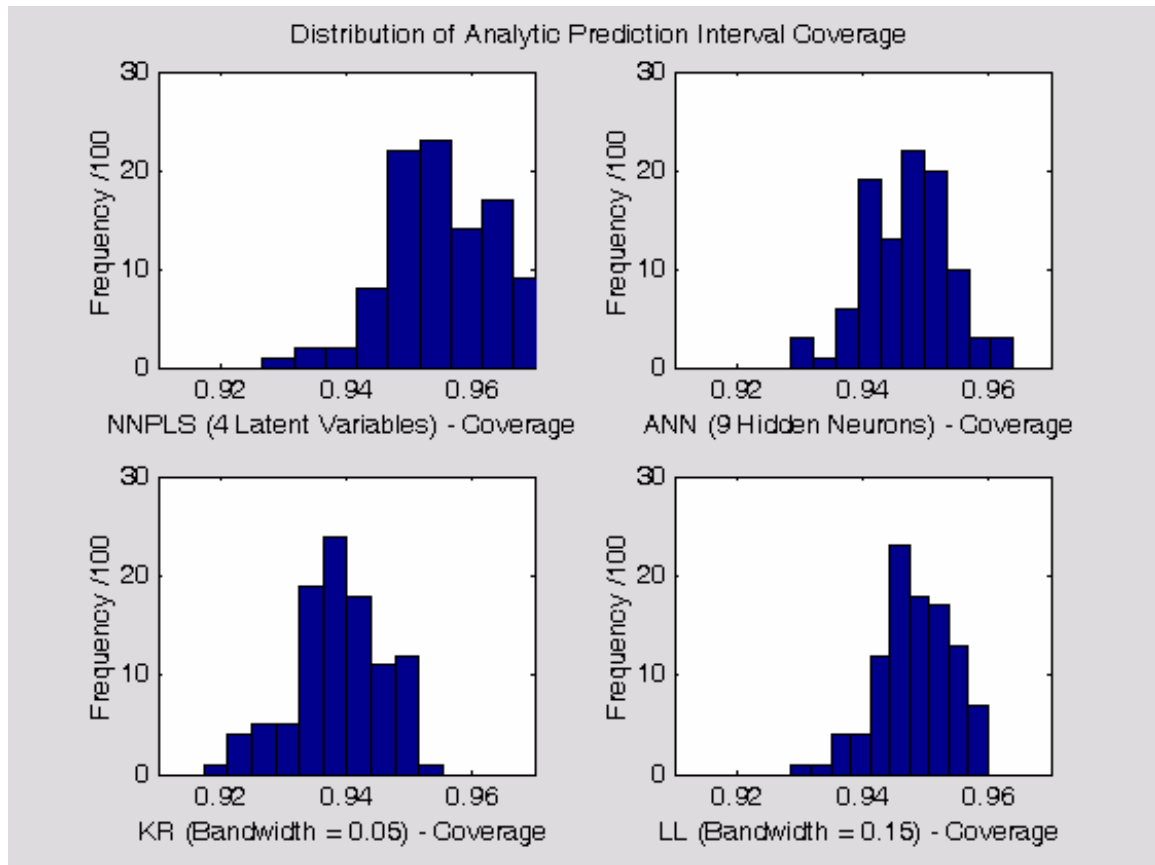
Figure 5.3.10: Analytic prediction interval coverage values for cascade test data set.
