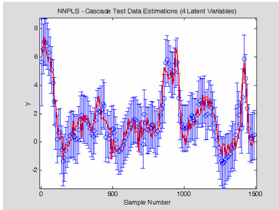
Figure 5.3.16: NNPLS median result estimation and analytic prediction intervals. Representative result for NNPLS 4 latent variable model showing every 10 th estimate and the corresponding analytic prediction intervals. This model exhibited the median value of the 100 Mean Absolute Error results for the 4 latent variable models. NNPLS – Neural Network Partial Least Squares.
