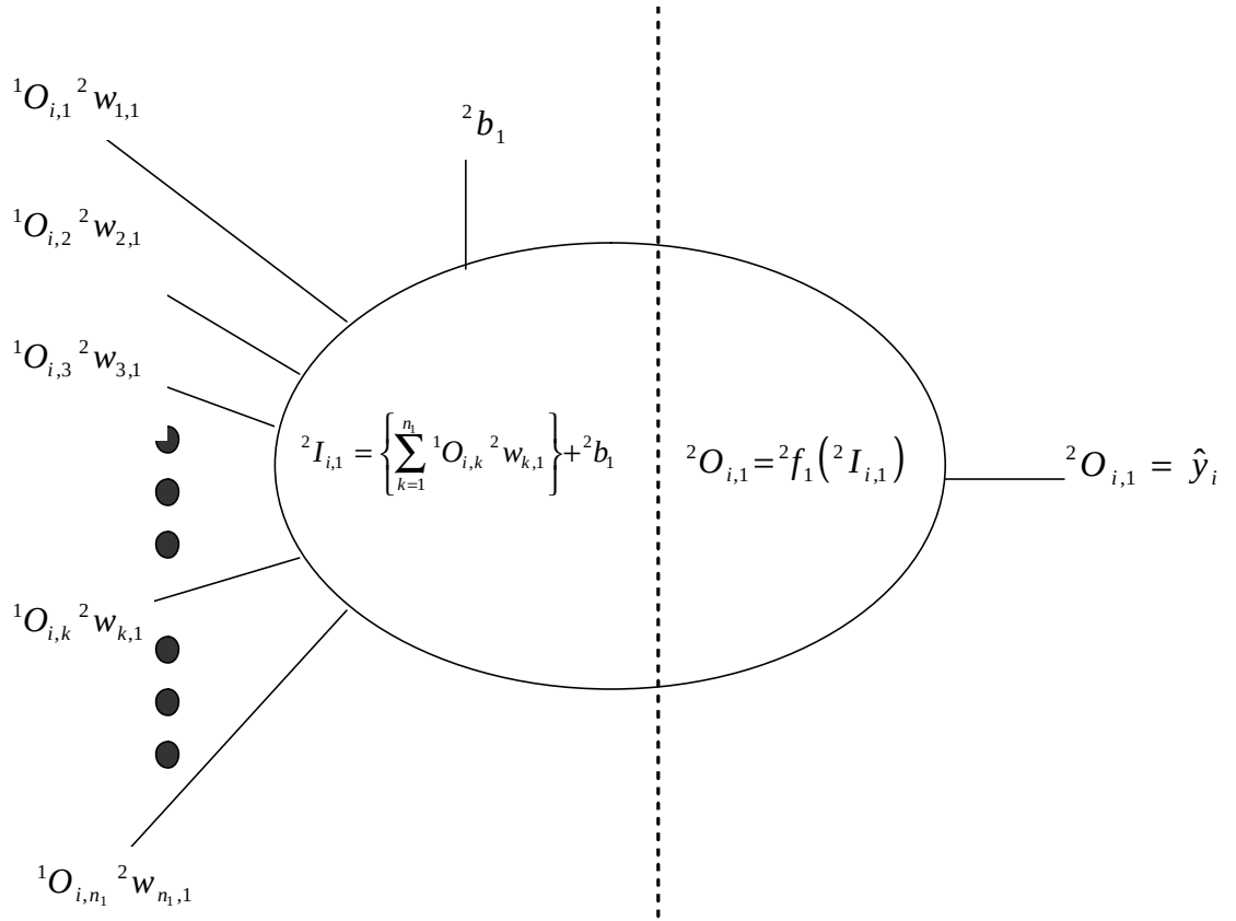
Figure 4.6.2: IANN output layer neuron
