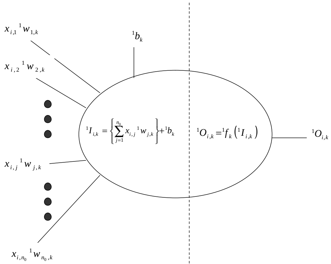
Figure 4.6.3: IANN hidden layer neuron
