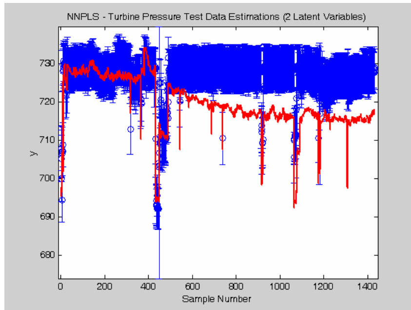
Figure 5.5.6: 2 latent variable NNPLS model with good behavior for turbine pressure test data.
