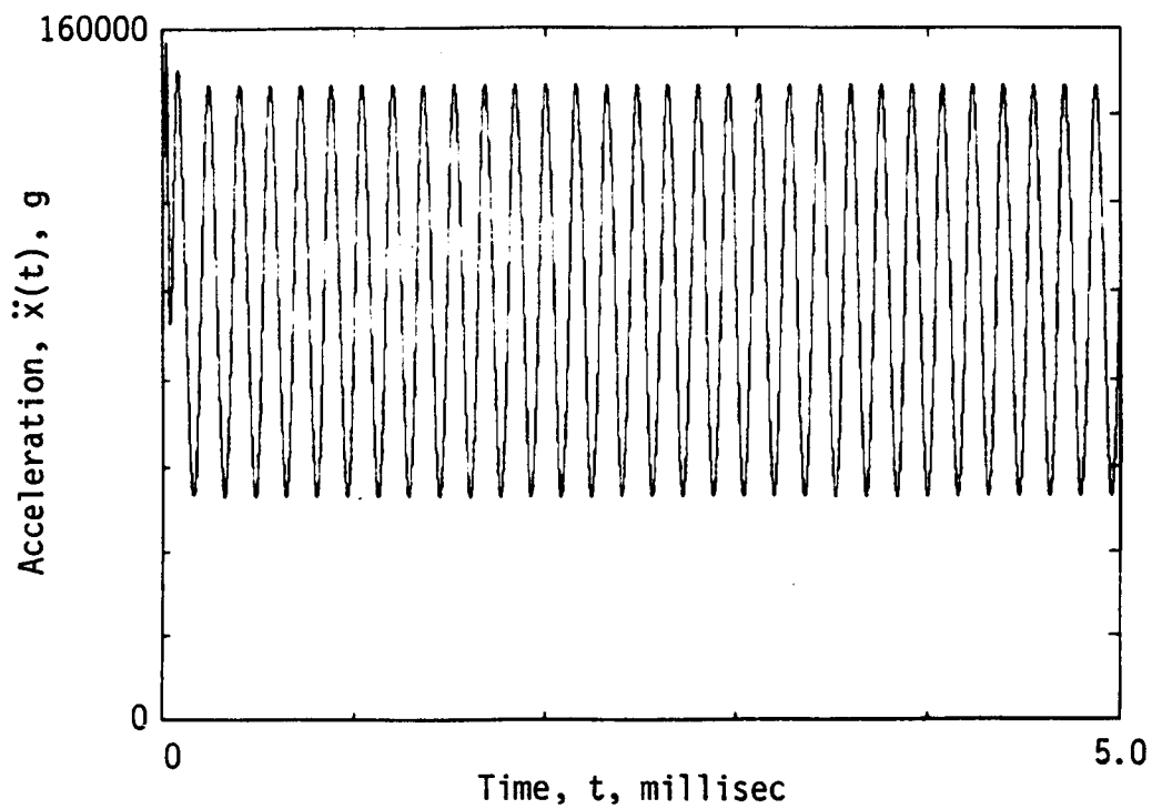
Figure 16. TXHARS Results With Perfect 24 GHz Signal
