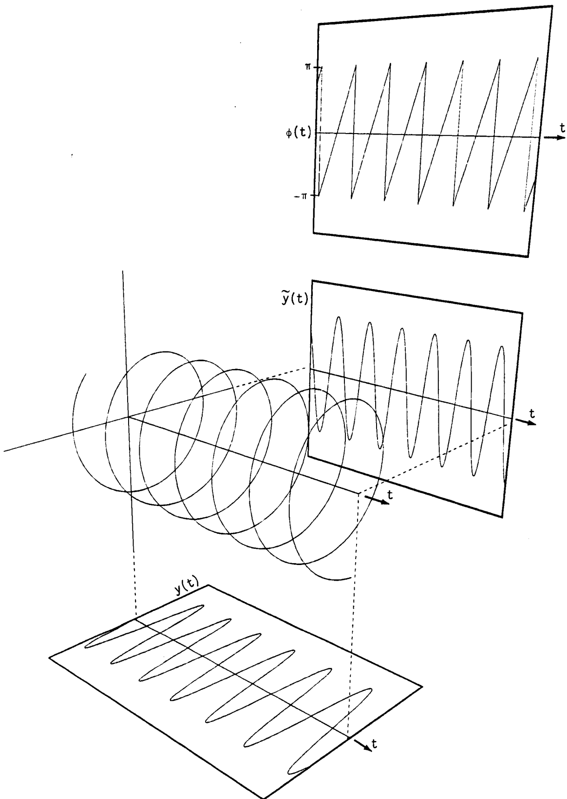
Figure 4. Analytic Signal
