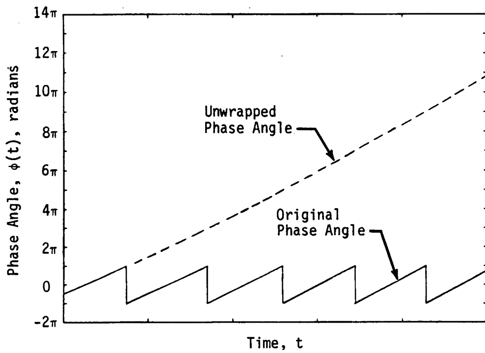
Figure 8. Phase Angle Unwrapping
