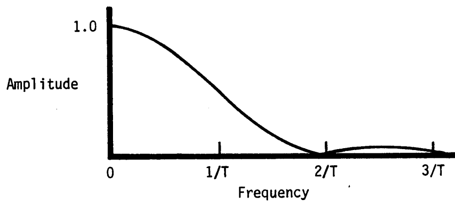
Figure 6. Low-Pass Nature of Hanning Window
