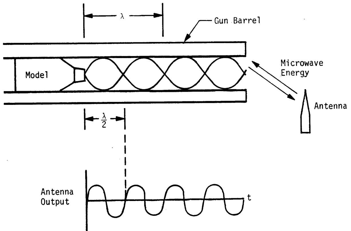
Figure 3. Doppler Radar in the Gun Barrel
