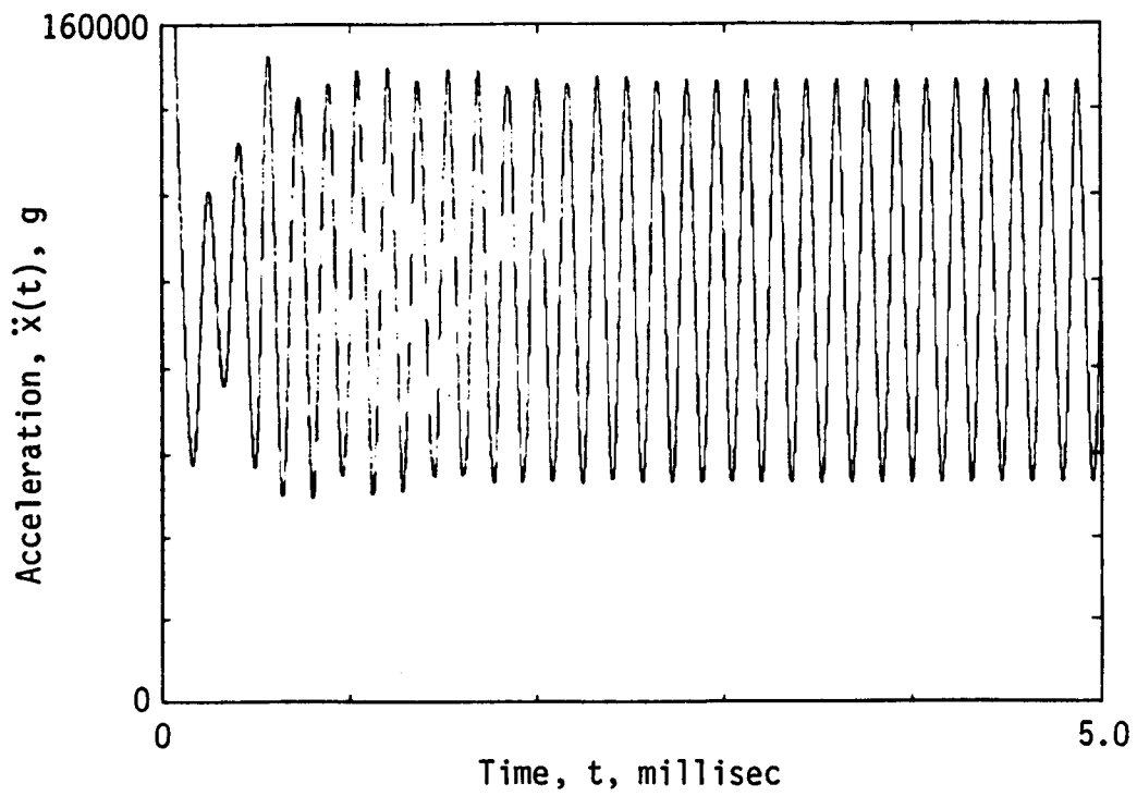
Figure 15. TXHARS Results With Perfect 3.6 GHz Signal
