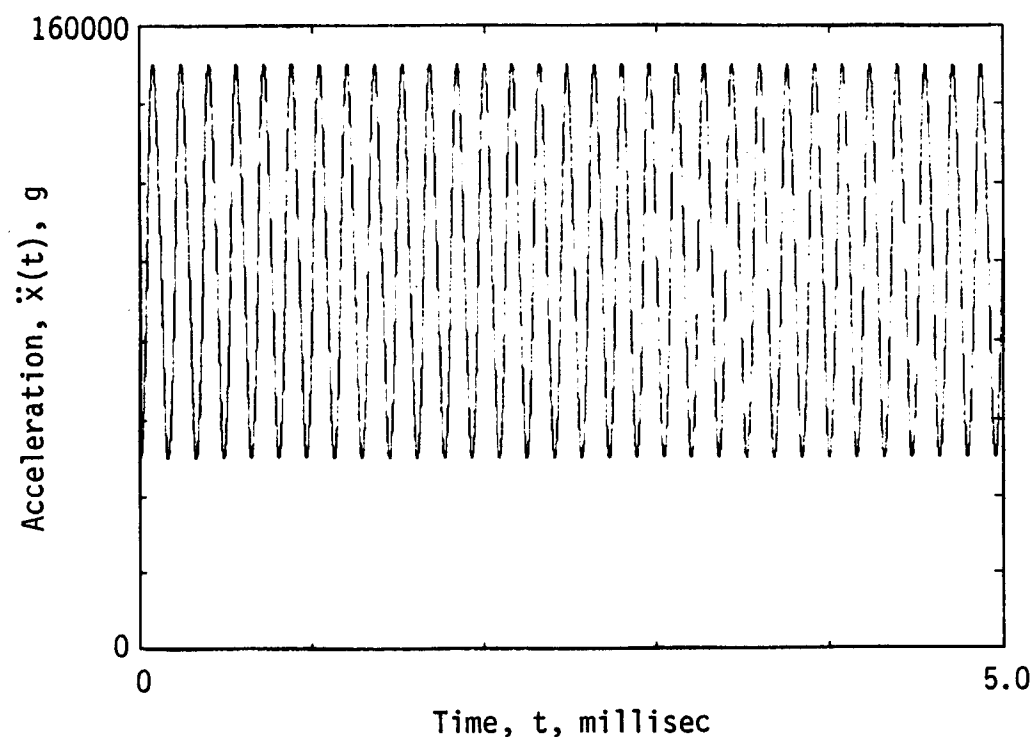
Figure 14. Theoretical Trajectory for Simulated Signals
