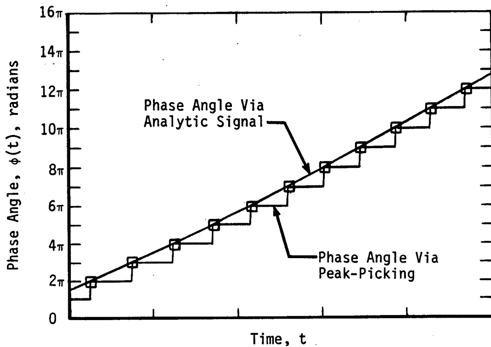
Figure 5. Analytic Signal and Peak Picking Methods
