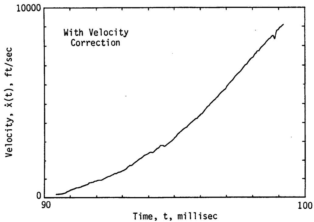
Figure 13. Effectiveness of Velocity Correction Algorithm
