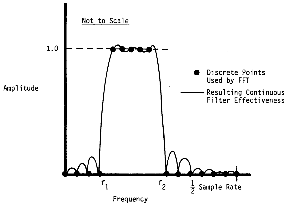
Figure 7. Box Car Filter
