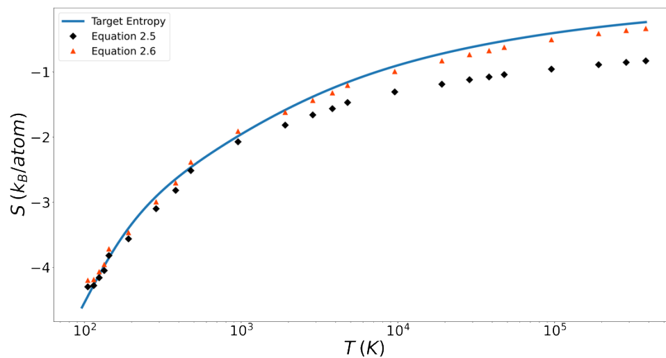
Figure 4-1. Liquid Lennard-Jones argon entropy.
