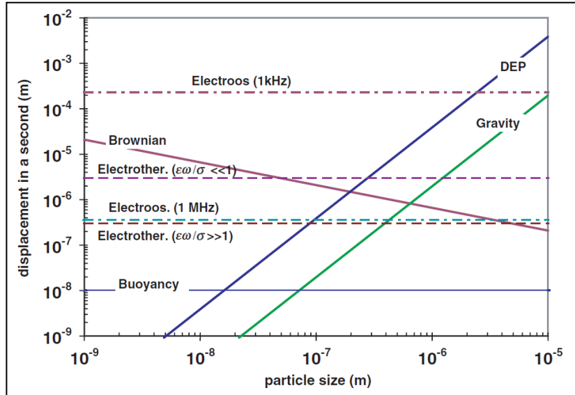
Figure 3-8. Particle displacement influenced by various forces in 1 second versus particle radius ( V=5 volt, r=25 \mu\text{m} , \sigma=0.01 S/m) [12].
