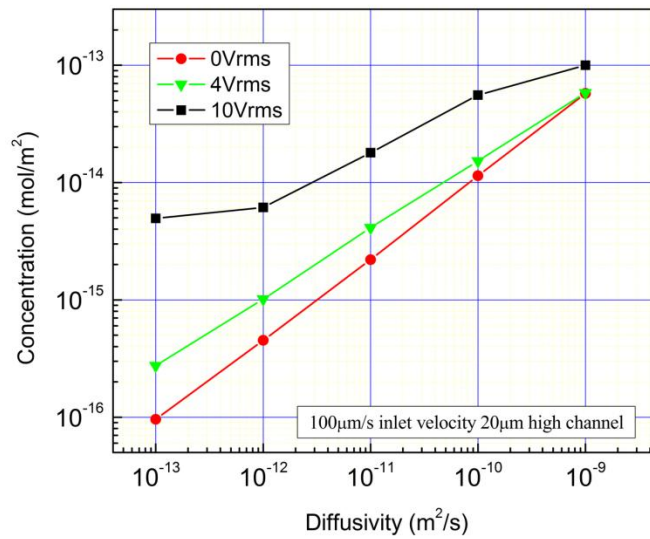
Figure 4-7. ACET concentration effect with molecular diffusivity change. Calculation assumes 100 \mu m/s inlet velocity and 20 \mu m channel height.
