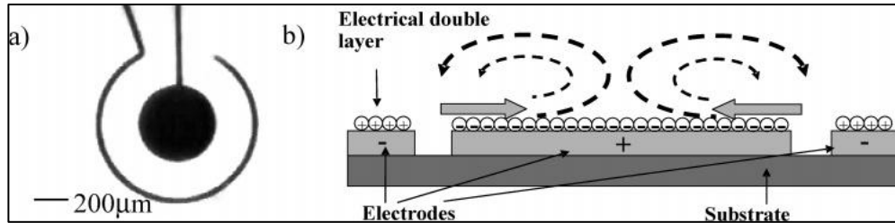
Figure 2-5. (a) Electrode design of the ac electroosmotic processor (top view). (b) Schematic (side view) illustrating electrode polarization and formation of ac electroosmotic flow. Solid arrows represent the ac electroosmotic force and dotted lines indicate the flow pattern [37].
