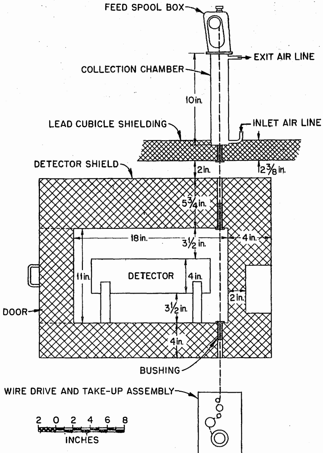
Fig. 4. The ORR Fission Gas Detector
