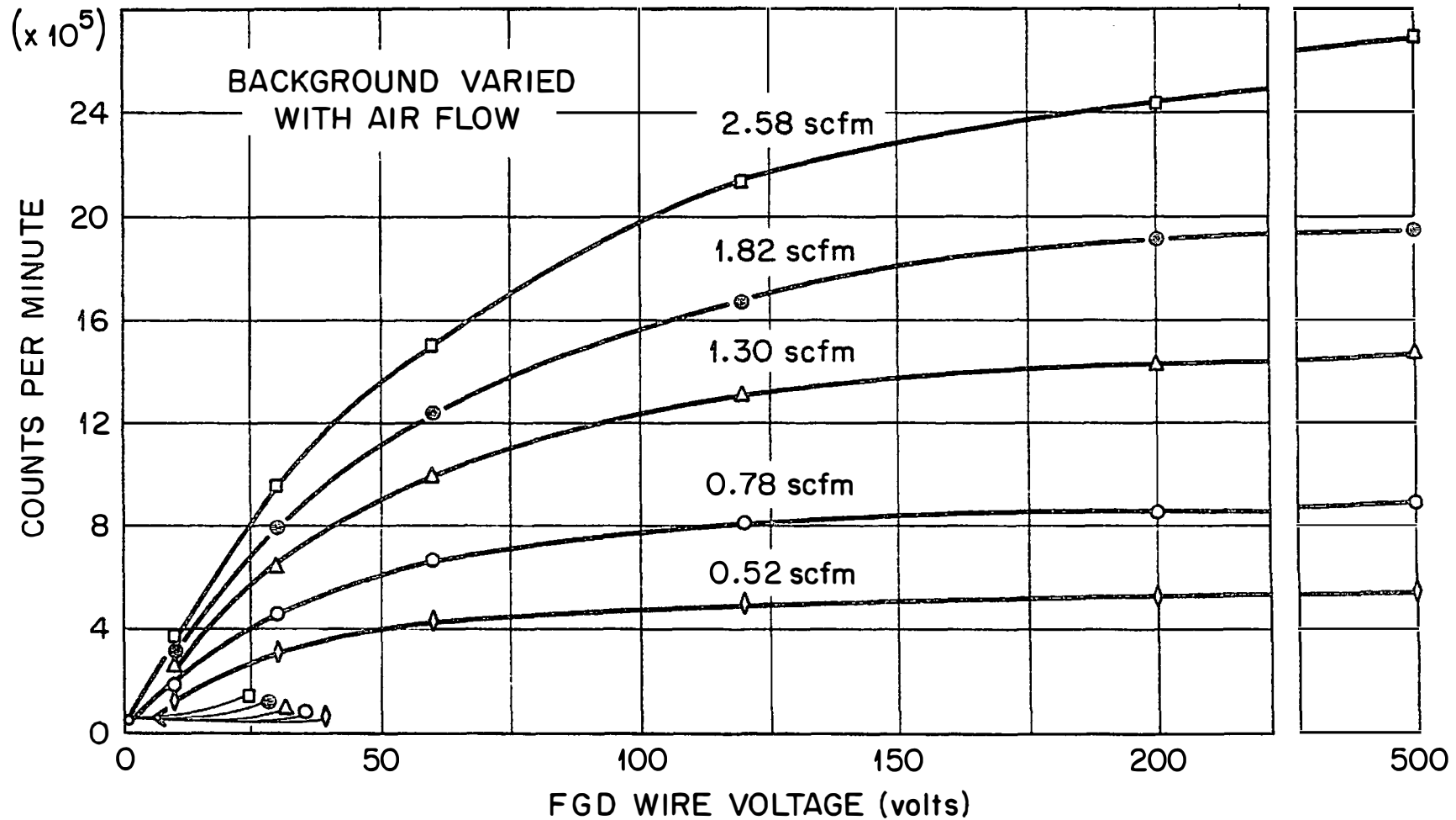
Fig. 28. Count Rate vs Voltage Curves for a Motor Speed of 23 rpm. Background has been Subtracted from Each Curve. Fission Product Concentration was Constant.
