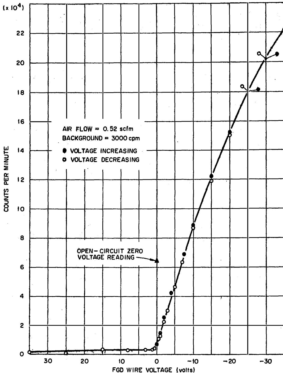
Fig. 10, Count Rate vs Voltage at Constant Air Flow. Negative Wire Voltage Increases to the Right. Background, 3000 Counts per Minute, Has Been Subtracted.
