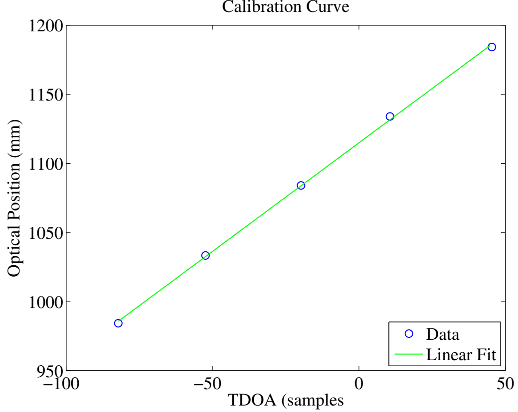
Figure 5.6: Linear calibration curve relating the TDOA measurements in samples to the optical ground truth data in millimeters.
