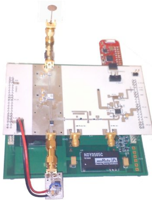
Figure 2.6: The existing integrated tag design using an MSP430-RF2500 development board for tag control. [7]
