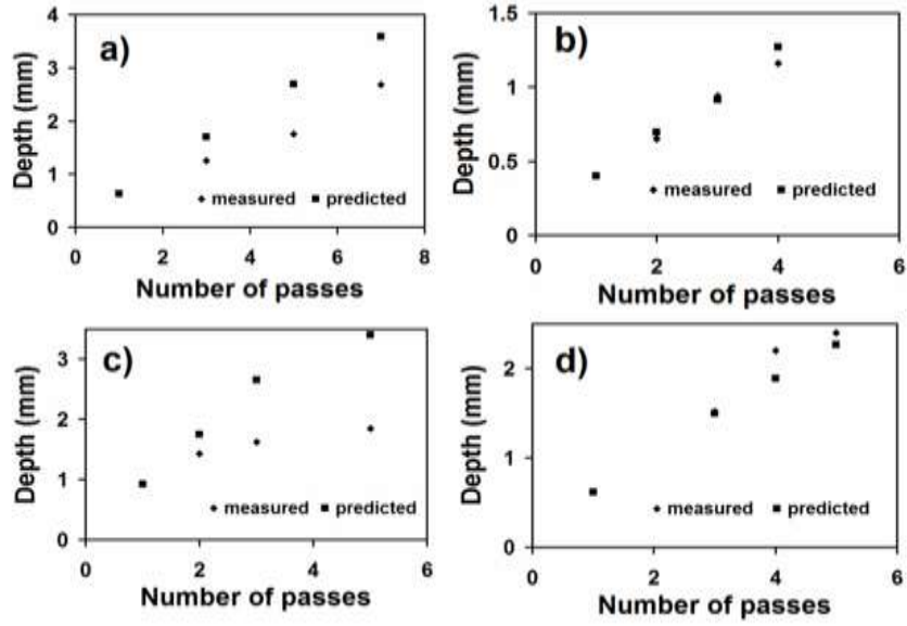
Fig.5.4 Comparison between predicted and measured depth of cavity in a) \text{Al}_2\text{O}_3 , b) \text{Si}_3\text{N}_4 , c) SiC, and d) MgO for different number of passes [167].
