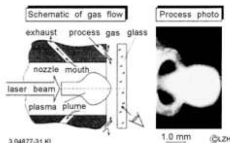
Fig. 10. Formation of plasma plume and its action by gas nozzle. (After Tönthoff and Kappel 70 with permission. Copyright Elsevier.)
