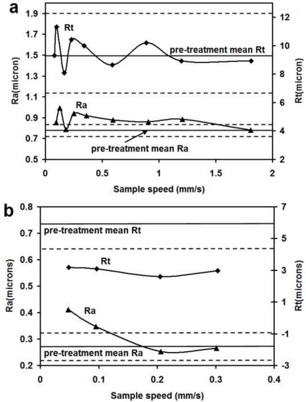
Fig. 1.21 Surface roughness after laser treatment for a) raw \text{Al}_2\text{O}_3 at fluence of 1.8 \text{ J/cm}^2 and b) polished \text{Al}_2\text{O}_3 at fluence of 7.5 \text{ J/cm}^2 [91].
