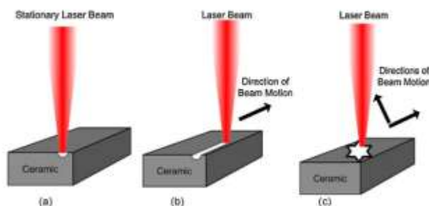
Fig. 14. Schematic of back laser machining processes (a) laser drilling (one-dimensional machining), (b) laser cutting (two-dimensional machining), (c) engraving a star by laser beam (three-dimensional machining).
