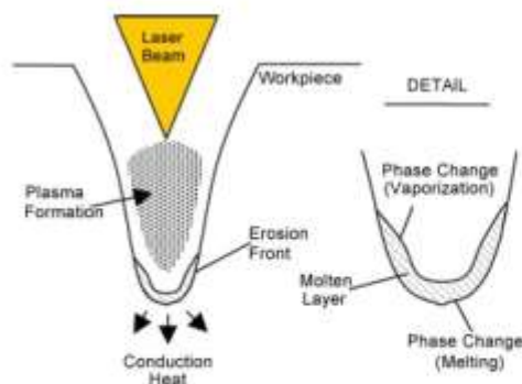
Fig. 15. Laser drilling process schematic. (After Chryssolouris 76 with kind permission of Springer Science + Business Media.)
