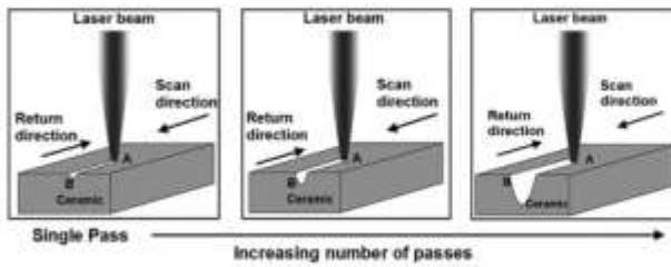
Fig. 1. Schematic illustrating the effect of multiple passes on the depth and width of machined cavity.
