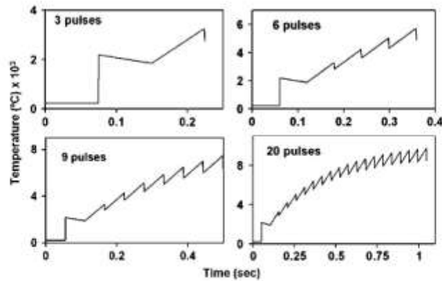
Fig. 3. Heating curves corresponding to laser machining of MgO with various number of pulses corresponding to 100% energy absorption ( \alpha = 1 ).
