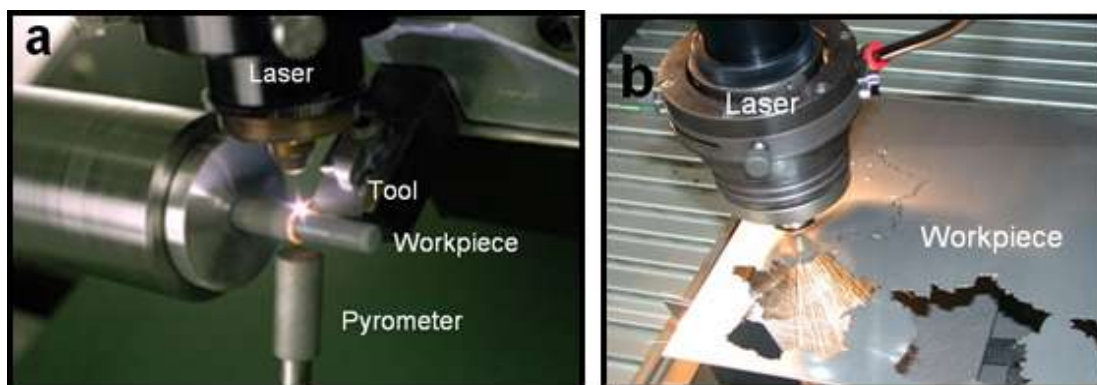
Fig. 1.3 a) Laser assisted machining [32] b) Laser machining [35].
