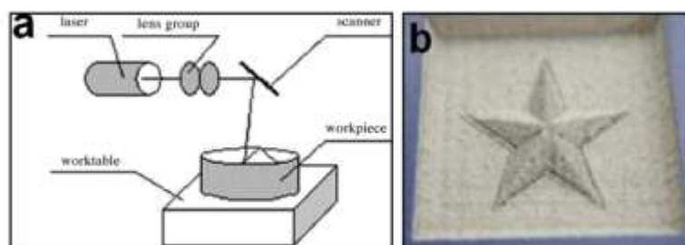
Fig. 24. 3D Laser Carving (a) schematic layout (b) 3D star in alumina ceramic. (After Wang and Zeng 11 with permission. Copyright Elsevier.)
