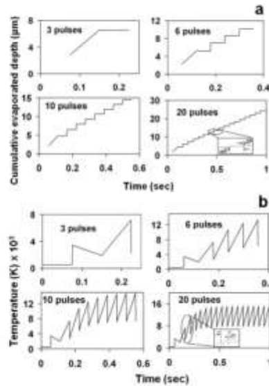
Fig. 2. a) Cumulative evaporated depth b) Heating curves.
