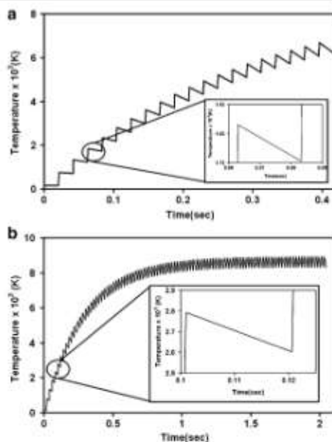
Fig. 4 Heating curves for a 2 mm thick plate and b 3 mm thick plate
