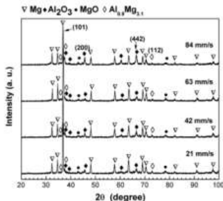
Fig. 2. XRD patterns of the laser processed samples.
