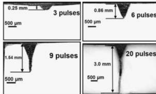
Fig. 34. Machining in \text{MgO} ceramic. (After Samant and Dahotre 62 ).
