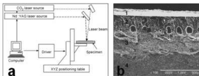
Fig. 18. (a) Configuration of laser cutting using controlled fracture technique. (b) Fracture surface of alumina substrate. (After Tsai and Chen 76 with permission. Copyright Elsevier.)
