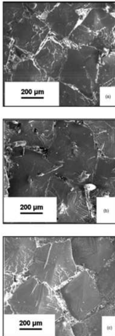
FIG. 1. Faceted grains observed on alumina surface processed by a cw laser at (a) 2.2 \times 10^4 , (b) 2.3 \times 10^5 , and (c) 2.5 \times 10^6 W/cm 2 .
