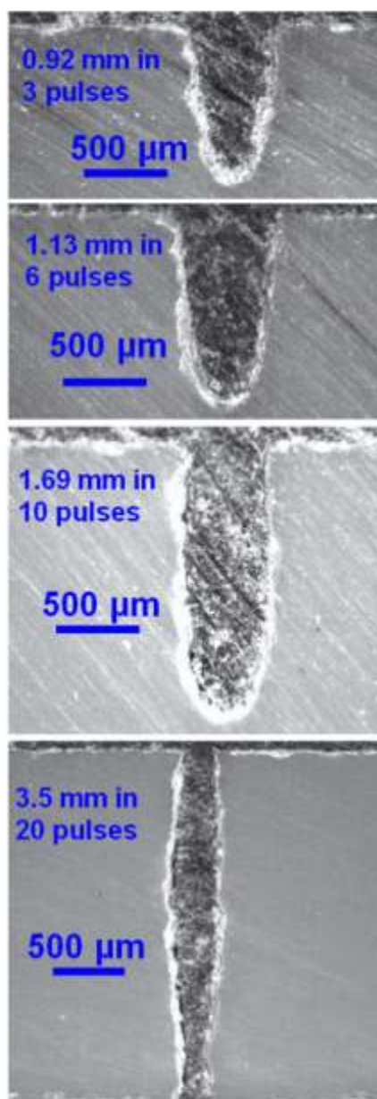
Fig. 26. Drilled holes in silicon nitride. (After Samant and Dahotre 92 ).
