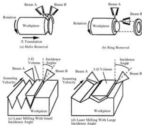
Fig. 19. Three-dimensional laser machining. (After Chryssolouris 34 with kind permission of Springer Science + Business Media.)
