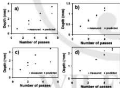
Fig. 4. Comparison between predicted and measured depth of cavity in (a) Al_2O_3 , (b) Si_3N_4 , (c) SiC, and (d) MgO for different number of passes.
