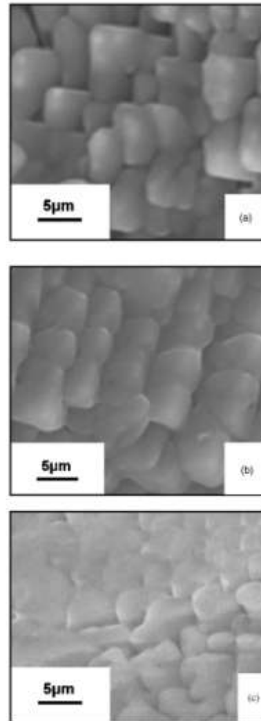
FIG. 2. Surface micrographs for PM laser operation at (a) 1.13 \times 10^5 , (b) 0.47 \times 10^6 , and (c) 0.99 \times 10^6 W/cm 2 .
