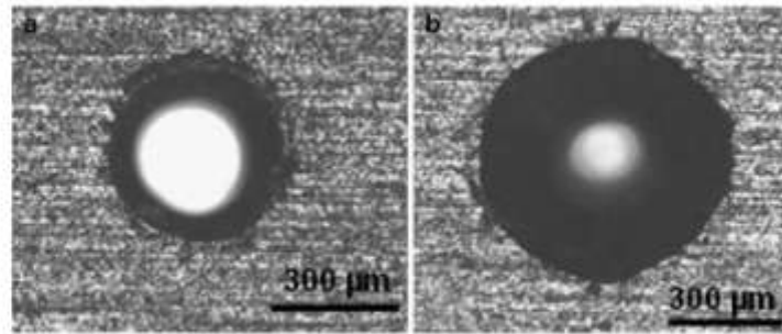
Fig. 1 Front surface showing drilled holes in a 2 mm and b 3 mm SiC plates
