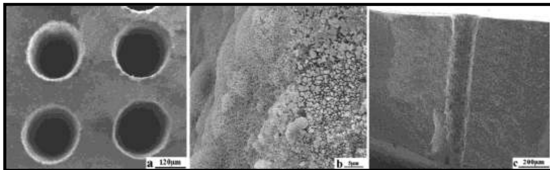
Fig. 1.20 Holes drilled on gelcast green body of \text{Al}_2\text{O}_3 . a) top view, b) hole edge, c) cross section of hole [89].
