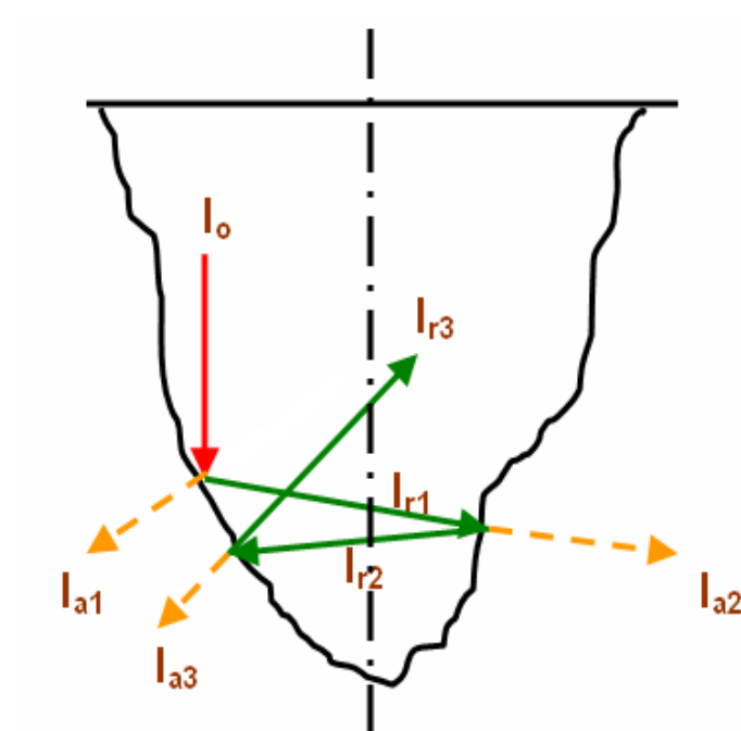
Fig.1.5 Multiple reflections in a machined cavity [43].
