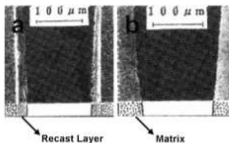
Fig. 9. Cross-section of \text{Si}_3\text{N}_4 ceramic machined in (a) air and (b) water. (After Morita et al. 55 with permission. Copyright American Institute of Physics.)
