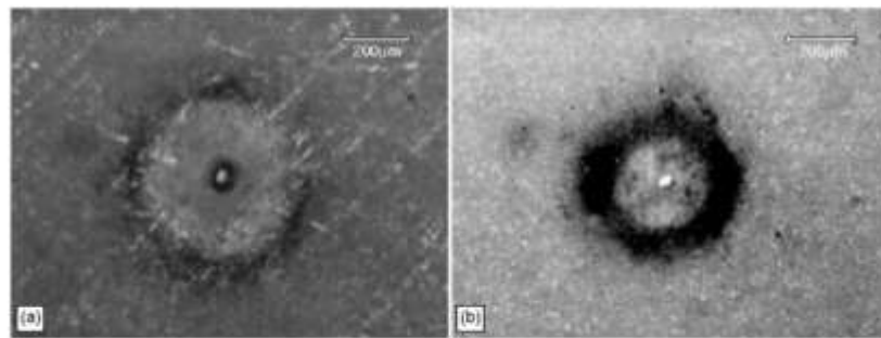
Fig. 33. Hole drilled in \text{ZrO}_2 with minimum taper: (a) top surface, (b) bottom surface. (After Kuar et al. 23 with permission. Copyright Elsevier.)
