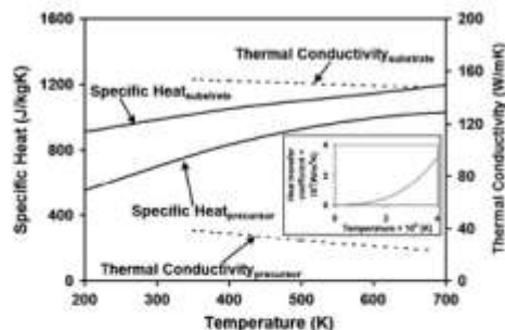
Fig. 1. Variation of thermal conductivity and specific heat of the precursor and substrate with temperature. Inset: Variation of heat transfer coefficient with temperature.
