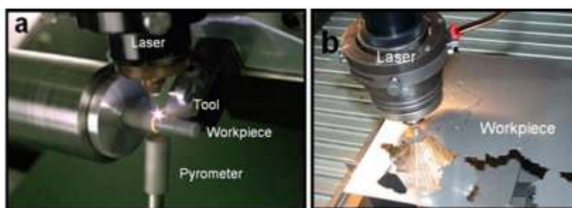
Fig. 3. (a) Laser assisted machining. (After Lei et al. 32 with permission. Copyright Elsevier.) (b) Laser machining. 35
