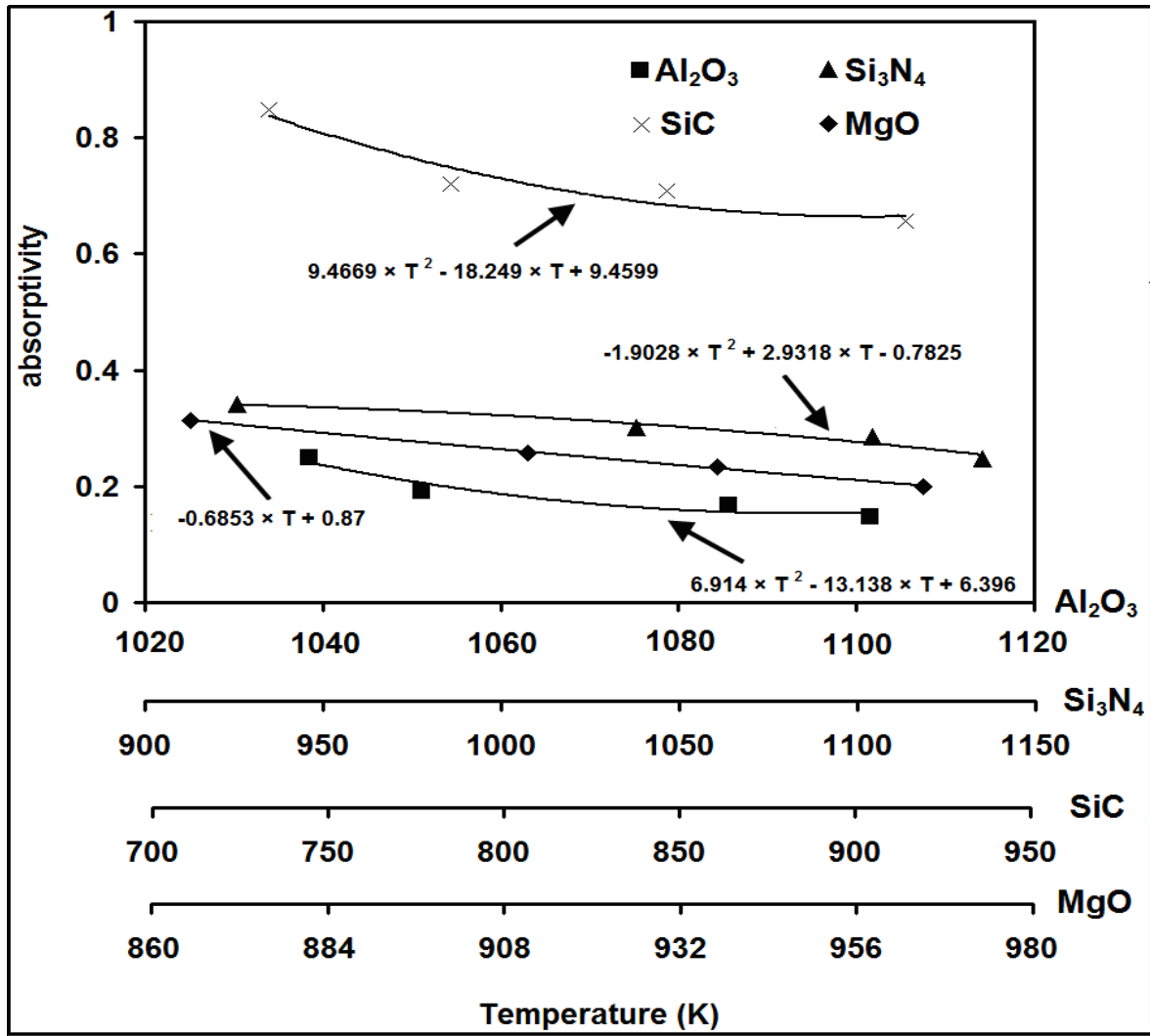
Fig.3.4 Variation of absorptivity with temperature for \text{Al}_2\text{O}_3 , \text{Si}_3\text{N}_4 , \text{SiC} , and \text{MgO} and corresponding governing laws [138].
