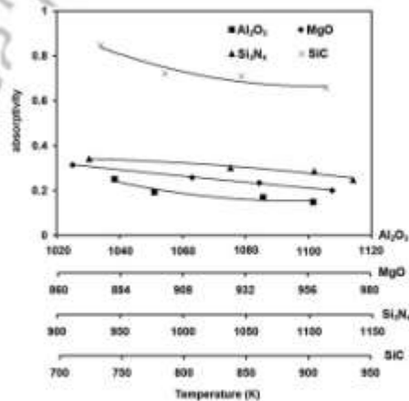
Figure 5 Variation of absorptivity with temperature for different ceramics.
