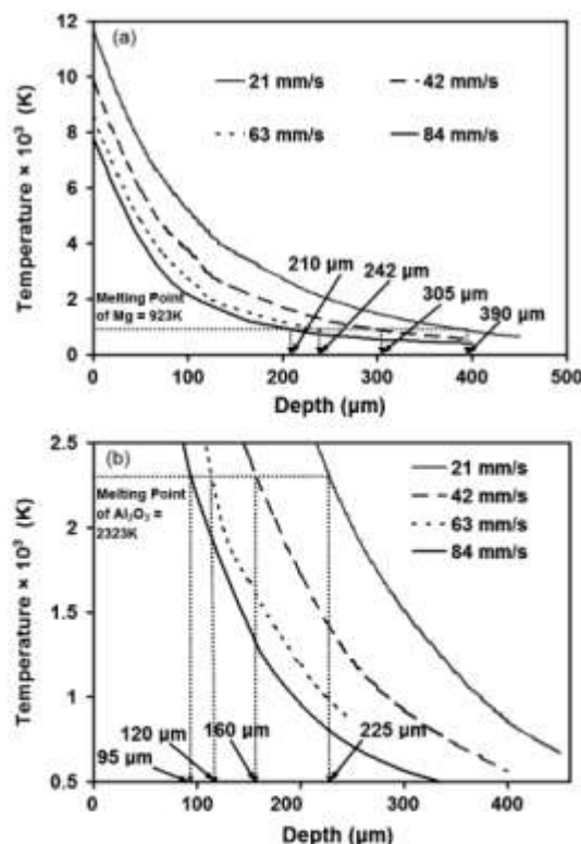
Fig. 7. (a) Prediction of total (final) melt depth. (b) Prediction of melt depth corresponding to the melting point of alumina for different processing speeds.
