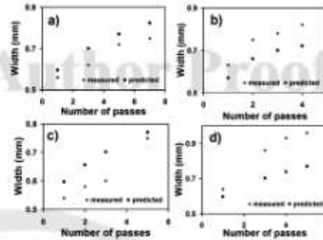
Fig. 5. Comparison between predicted and measured width of cavity in (a) Al_2O_3 , (b) Si_3N_4 , (c) SiC, and (d) MgO for different number of passes.
