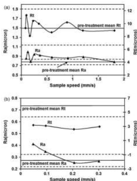
Fig. 23. Surface roughness after laser treatment for (a) raw \text{Al}_2\text{O}_3 at fluence of 1.8 J/cm² and (b) polished \text{Al}_2\text{O}_3 at fluence of 7.5 J/cm². (After Sciti et al. 72 with kind permission of Springer Science + Business Media.)
