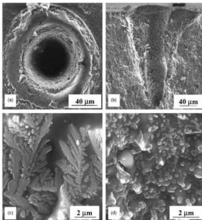
Fig. 16. Microstructural features of hole obtained in SiC (a) hole entry (b) hole section (c) silicate-like dendrite crystals obtained on debris area (d) hole inside walls. (After Sciti and Bellodi 74 with permission. Copyright Elsevier.)
