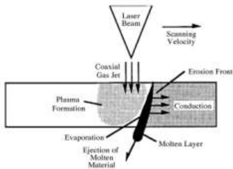
Fig. 17. Schematic of laser cutting process. (After Chrysosouris 76 with kind permission of Springer Science + Business Media.)
