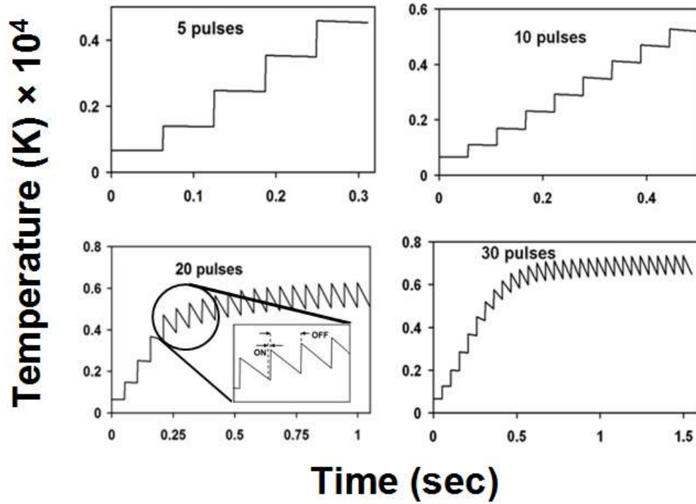
Fig. 2.5 Heating curves for different number of pulses in \text{Al}_2\text{O}_3 [63].
