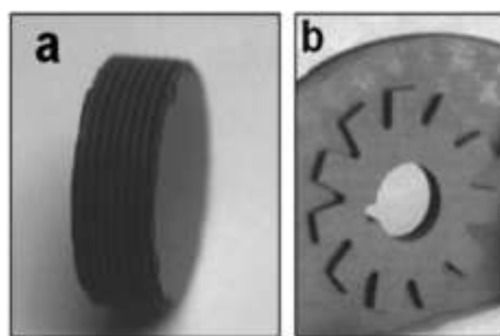
Fig. 20. (a) Turning of threads in \text{Si}_3\text{N}_4 . (After Liu et al. 71 with permission, Copyright Elsevier.) (b) A gear shape cut in \text{SiC}_{18}/\text{Al}_2\text{O}_3 composite. (After Islam 72 with kind permission of Springer Science + Business Media.)
