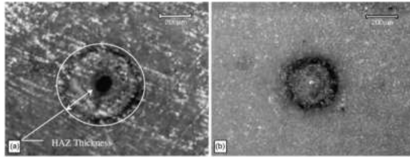
Fig. 32. Minimum HAZ thickness in \text{ZrO}_2 : (a) top surface, (b) bottom surface. (After Kuar et al. 23 with permission. Copyright Elsevier.)
