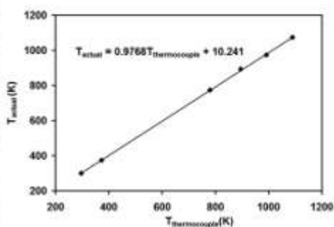
Figure 1 Thermocouple calibration.
