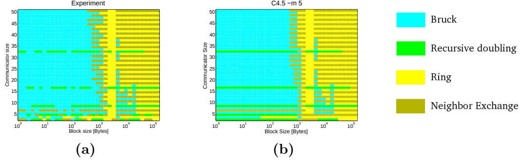
Figure 6.15: Effect of constructive induction on Allgather decision function: (a) experiment (b) c4.5 -m 5 with composite attributes.
