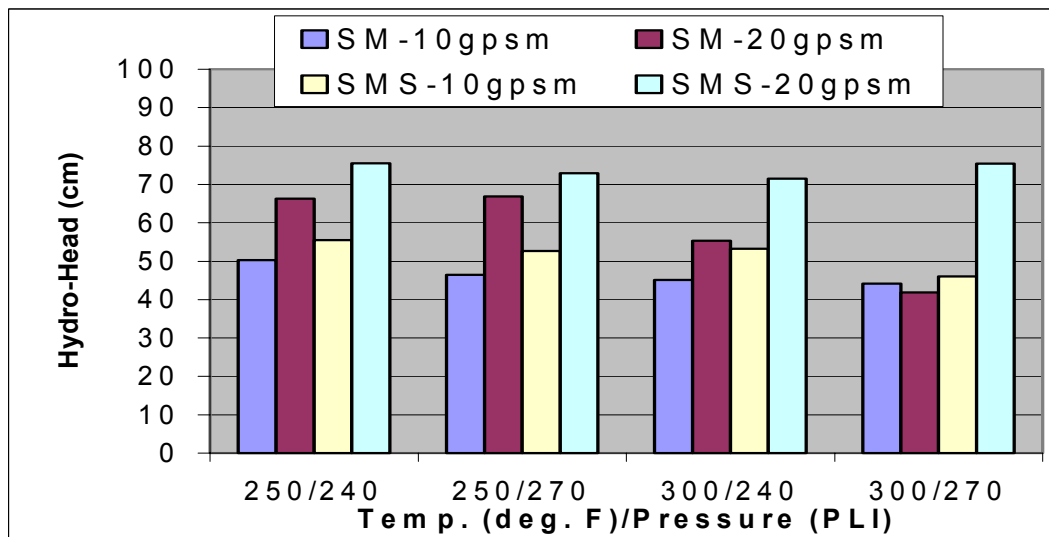
Figure 8. Comparison of SM and SMS Composites in Hydrostatic Head (75%PP/25%PE)
