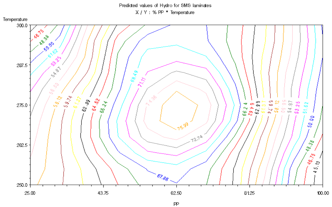
Figure 32: Effect of temperature and %PP on hydrostatic head
