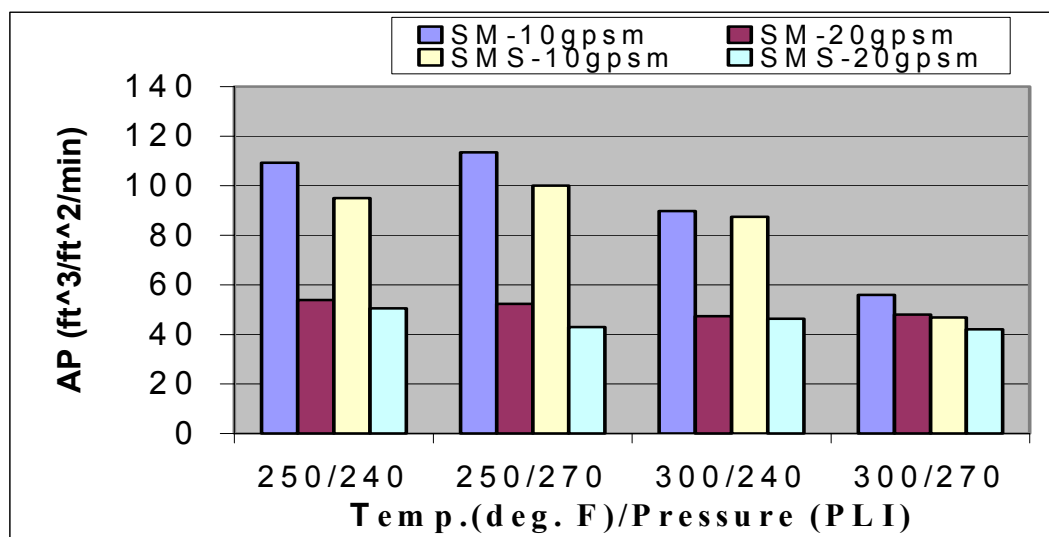
Figure 7. Comparison of SM and SMS Composites in Air permeability (75%PP/25%PE)
