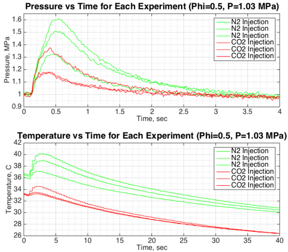
Figure 4.17 Effects of \text{CO}_2 and \text{N}_2 injection on pressure and temperature at center of a methane-air mixture at \phi = 0.5 and chamber pressure of 1.03 MPa (--- with \text{N}_2 injection, --- with \text{CO}_2 injection)
