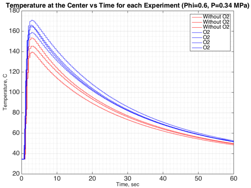
Figure 4.7 Effects of O_2 injection on temperature at center of combustion chamber of methane-air mixture at \phi = 0.6 and chamber pressure of 0.34 MPa (--- without O_2 injection, --- with O_2 injection)
