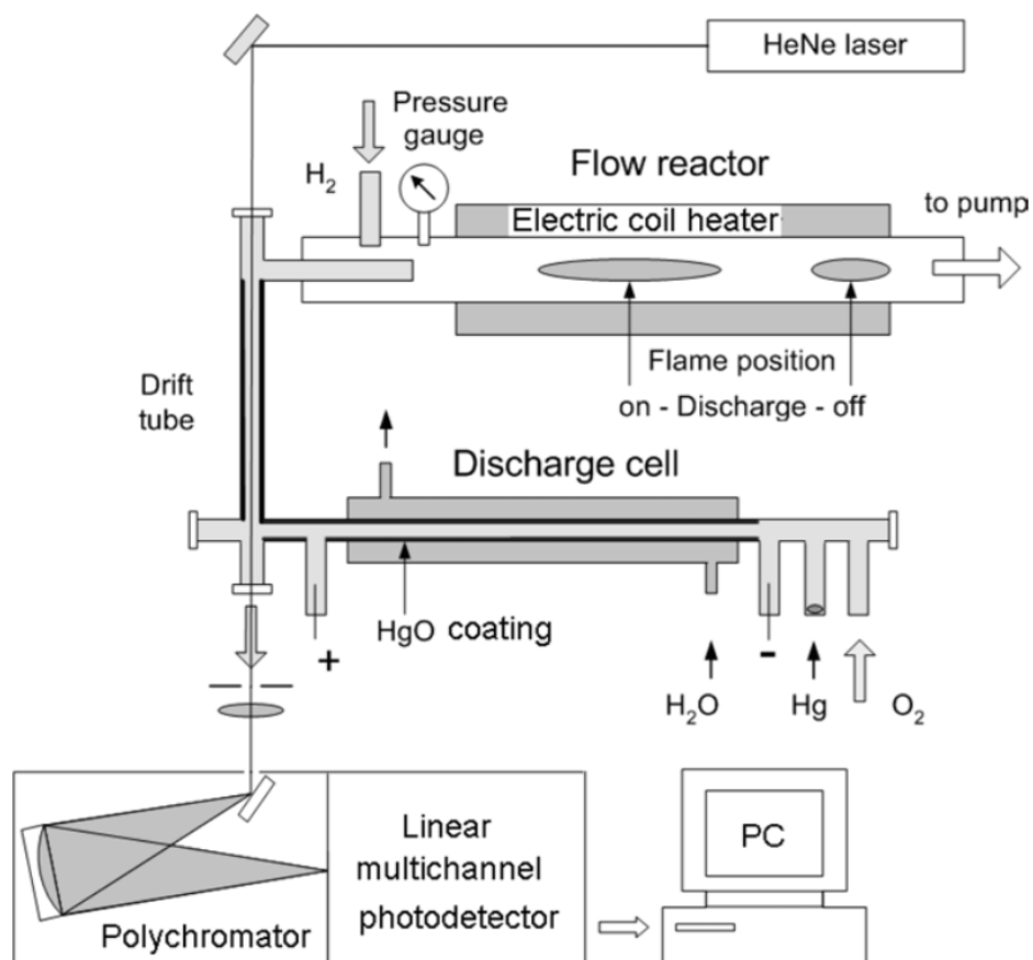
Figure 2.3 Experimental setup on the influence of electronically excited oxygen molecule on combustion of \text{H}_2\text{-O}_2 mixture (Smirnov 2008).
