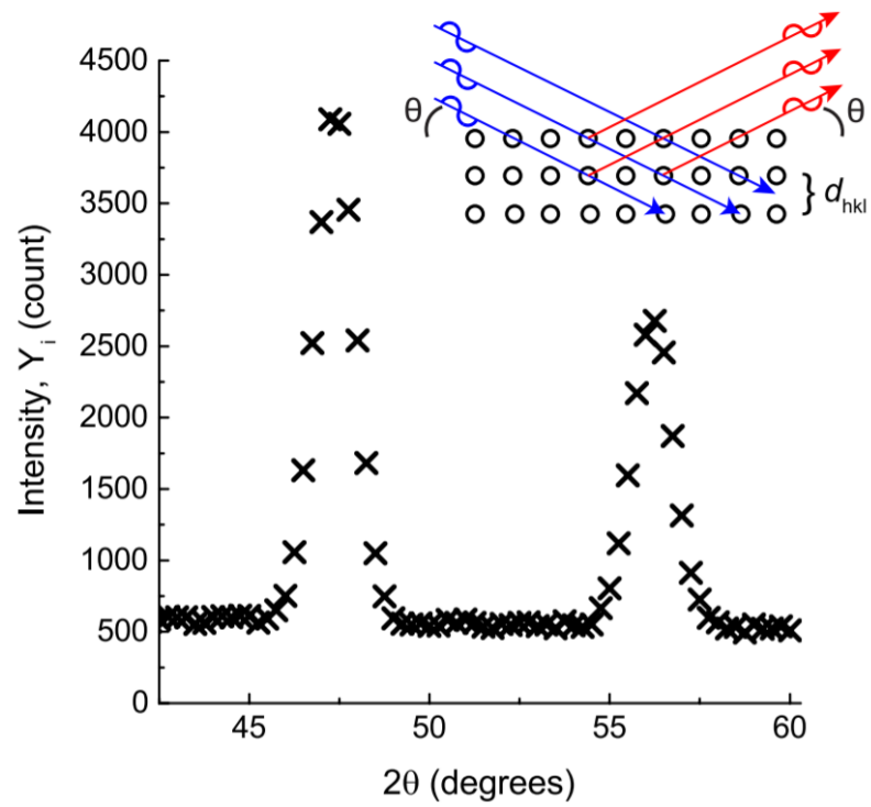
Figure 2-25 Constructive interference of X-rays scattered from planes of atoms which results in the observed peaks at various scattering angles ( 2\theta ) (from Ref. [224]).
