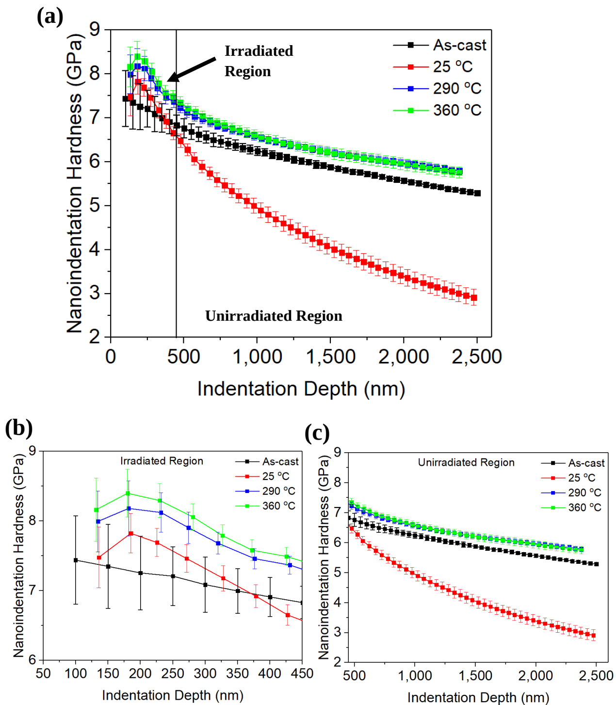
Figure 4-24 Nanoindentation hardness vs. depth for BAM-11 BMG as-cast and irradiated samples (9 MeV \text{Ni}^{3+} to 0.5 dpa) at different temperatures for (a) depths from 100 to 2500 nm, (b) the irradiated region (100-450 nm), and the (c) unirradiated region (450-2500 nm).
