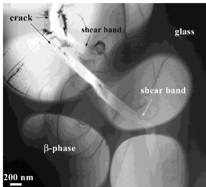
Figure 2-34 TEM image of the shear band propagation through the amorphous and crystalline regions \text{Zr}_{56.3}\text{Ti}_{13.8}\text{Cu}_{6.9}\text{Ni}_{5.6}\text{Nb}_{5.0}\text{Be}_{12.5} BMG based composite. Localization of deformation is observed in the \beta -phase (from Ref. [144]).
