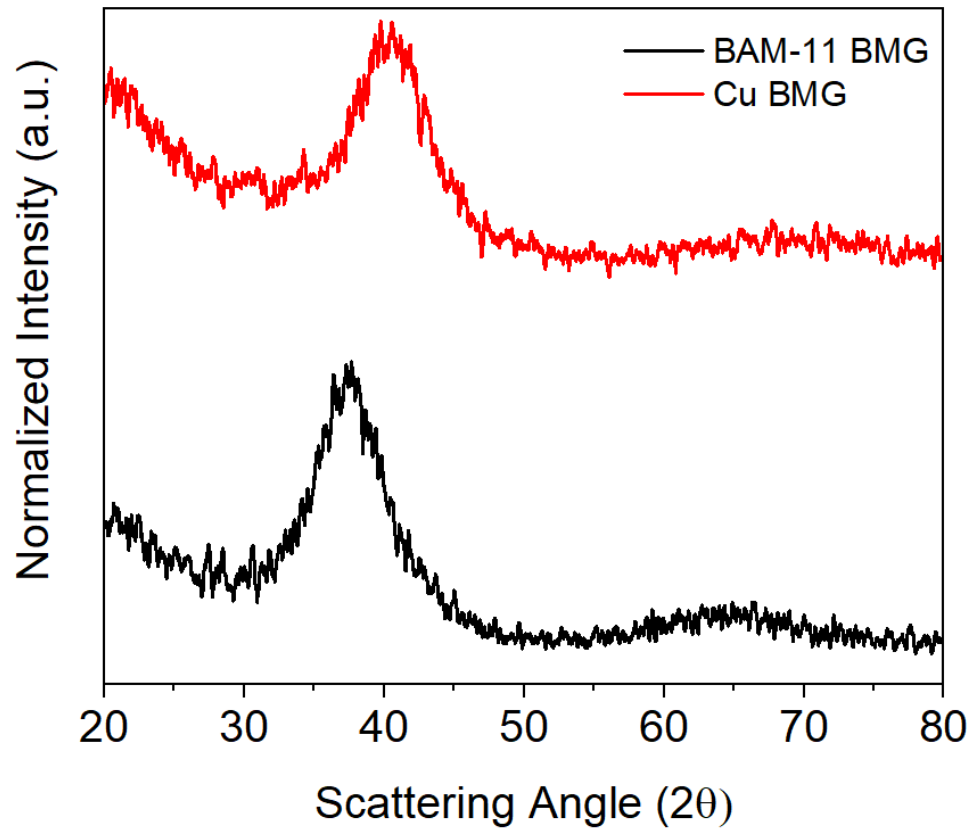
Figure 3-5 XRD patterns for the as-cast \text{Zr}_{52.5}\text{Cu}_{17.9}\text{Ni}_{14.6}\text{Al}_{10}\text{Ti}_5 (BAM-11) and \text{Cu}_{60}\text{Zr}_{20}\text{Hf}_{10}\text{Ti}_{10} BMG alloys.
