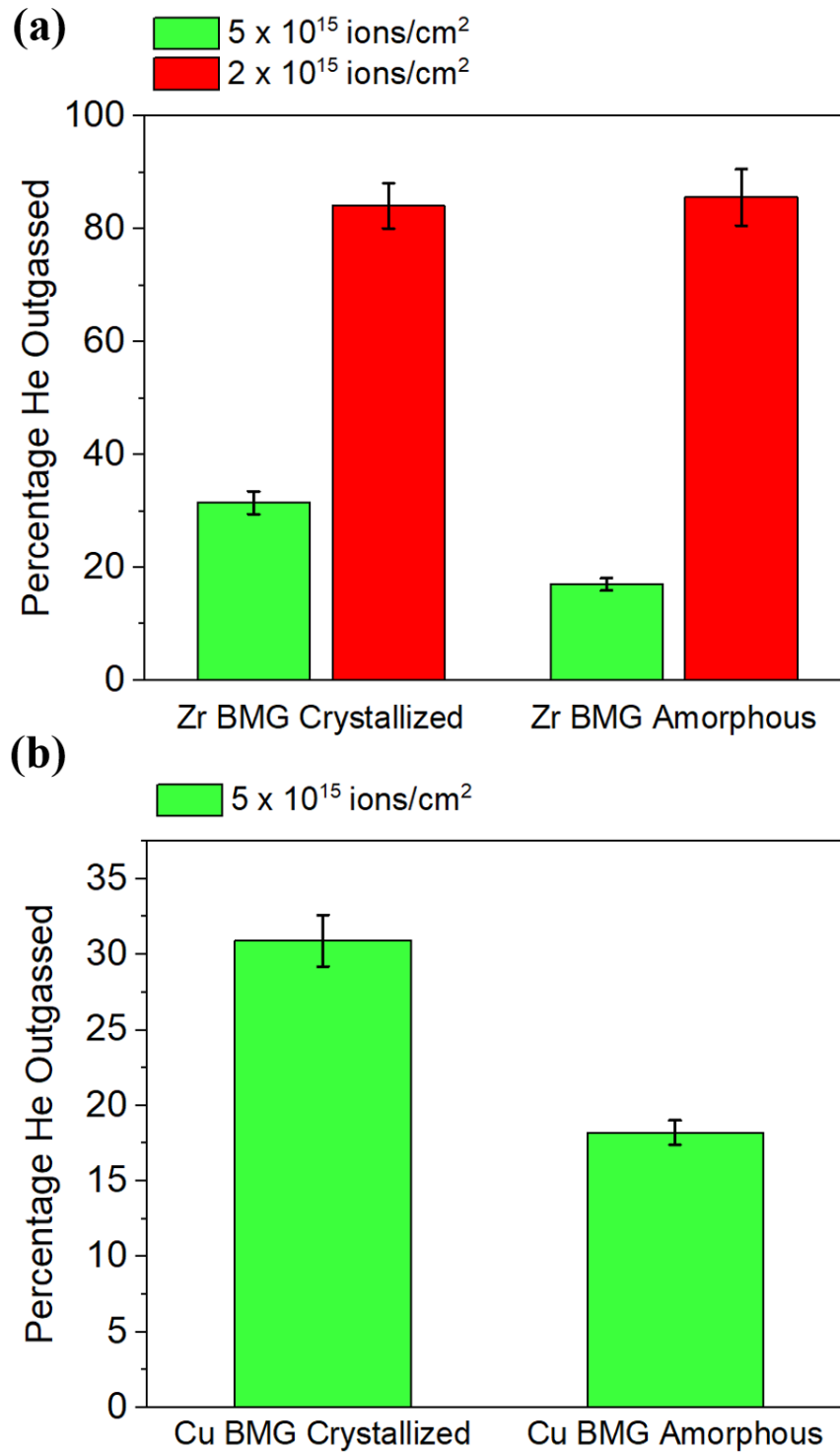
Figure 4-70 Helium outgassing statistics in the (a) BAM-11 BMG samples (implanted He fluences of 2 \times 10^{15} and 5 \times 10^{15} cm -2 ) and the (b) Cu BMG samples (implanted He fluence of 5 \times 10^{15} cm -2 ).
