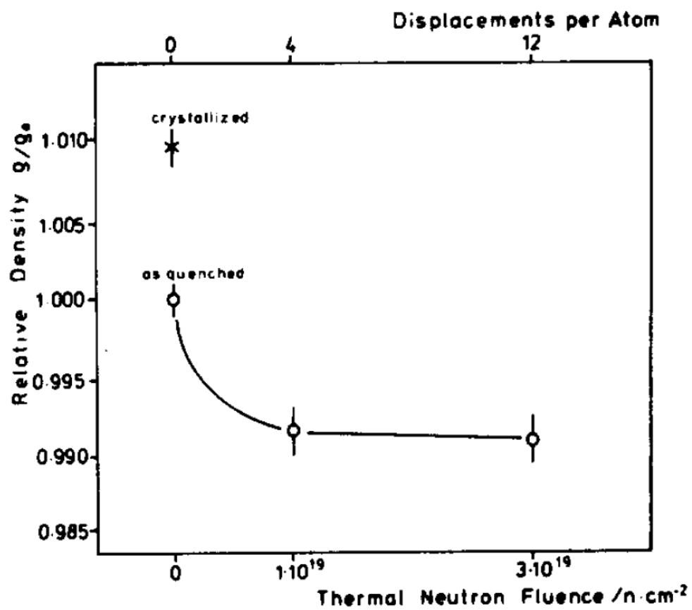
Figure 2-46 The relative density for \text{Fe}_{40}\text{Ni}_{40}\text{B}_{20} in the as-quenched state, crystallized, and neutron irradiated to 12 dpa (from Ref. [348]).
