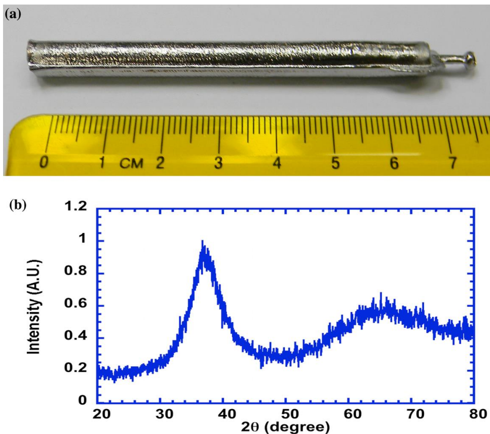
Figure 4-1 (a) Rod of BAM-11 prepared by casting and quenching at Oak Ridge National Laboratory and (b) X-ray diffraction pattern showing the amorphous structure (from Ref. [70]).
