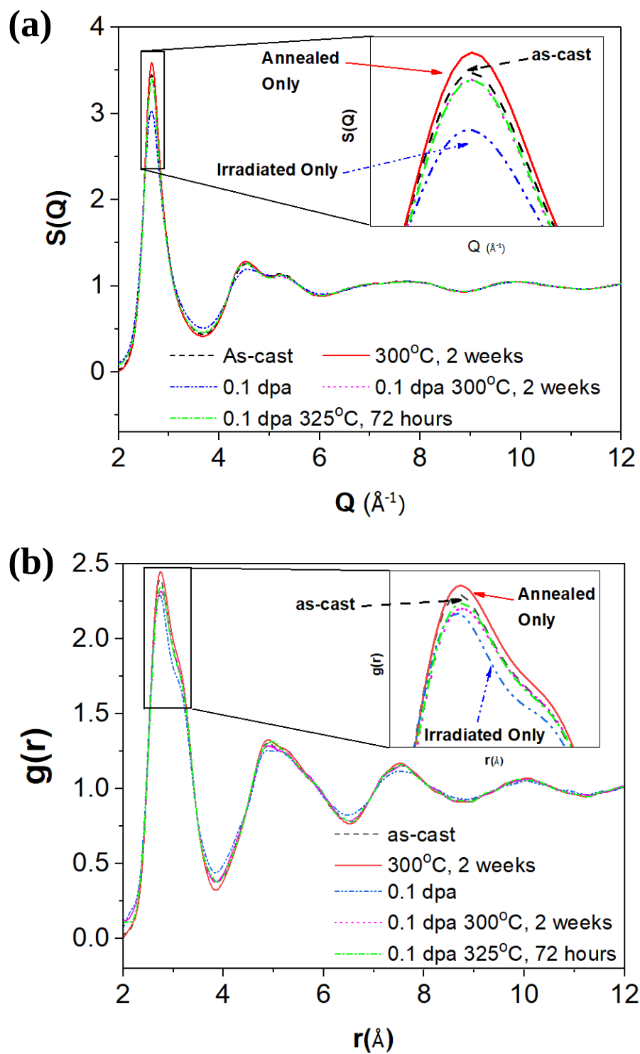
Figure 4-35 The (a) structure function S(Q) and (b) pair distribution function g(r) for the as-cast, neutron irradiated (0.1 dpa), and annealed BAM-11 BMG.
