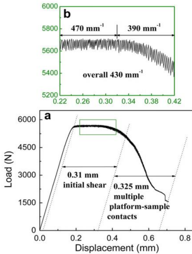
Figure 2-11 (a) Compressive load-displacement curve of \text{Zr}_{64.13}\text{Cu}_{15.75}\text{Ni}_{10.12}\text{Al}_{10} BMG at a nominal strain rate of 2 \times 10^{-4} \text{ s}^{-1} . (b) Enlarged view of the serrated region (from Ref. [135]).
