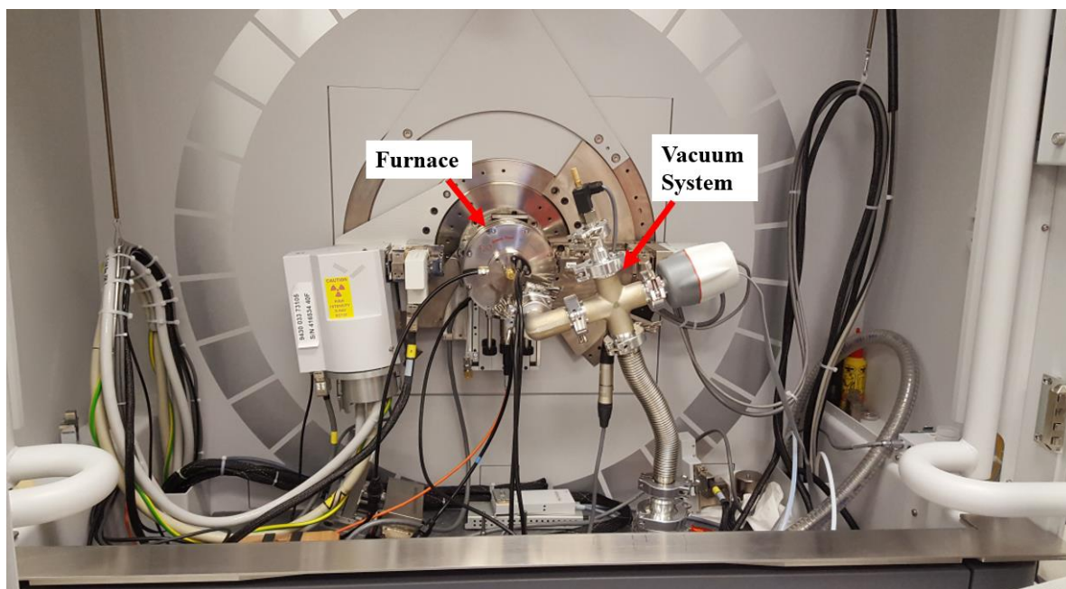
Figure 3-35 Empyrean HTXRD setup which includes a furnace and a vacuum system.
