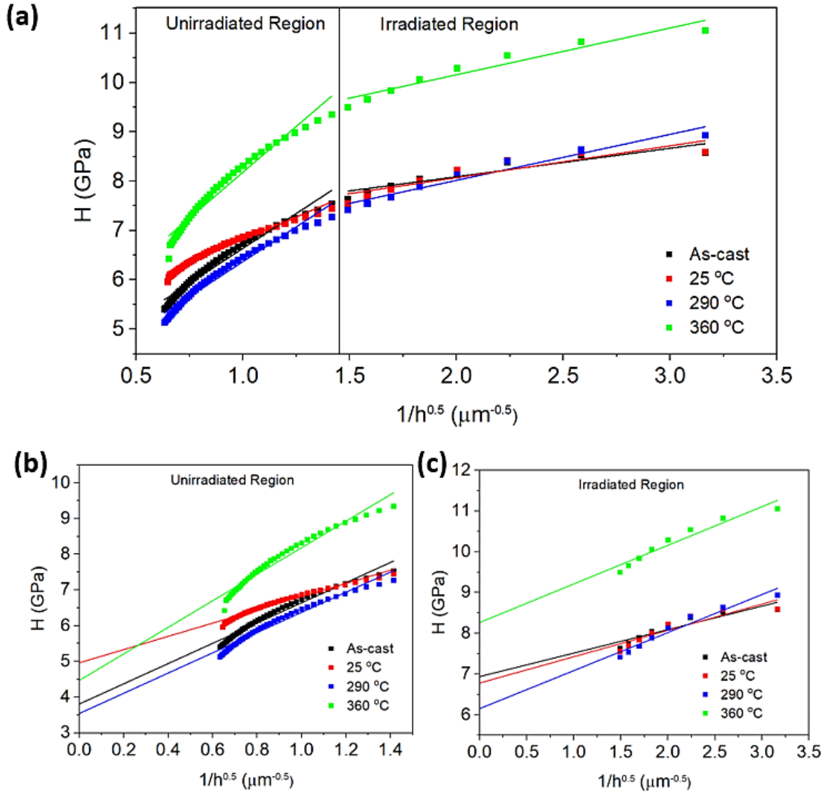
Figure 4-30 H vs. 1/h^{0.5} for as-cast vs. irradiated \text{Cu}_{60}\text{Zr}_{20}\text{Hf}_{10}\text{Ti}_{10} BMG (9 MeV \text{Ni}^{3+} , 10 dpa) at different temperatures for (a) depths ranging from 100-2500 nm, (b) the unirradiated region (450 nm-2500 nm), and (c) the irradiated region (100-450 nm).
