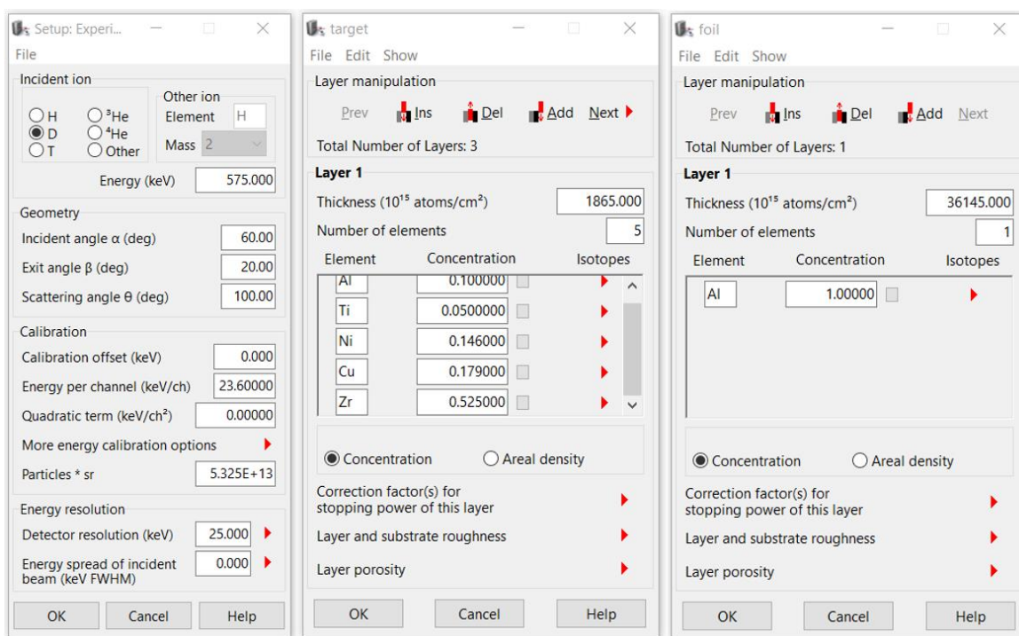
Figure 3-45 SIMNRA software experimental input windows which include the (a) general experimental parameters such as incoming deuteron energy and calibration offsets, (b) specimen target composition and thickness input, and (c) foil composition and thickness input.
