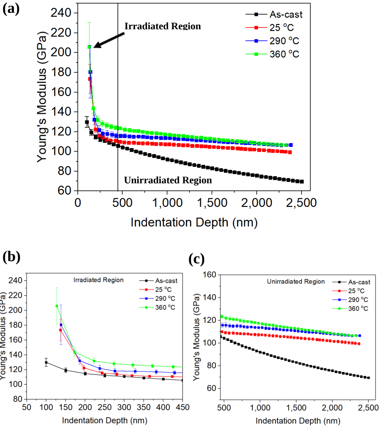
Figure 4-34 Nanoindentation Young's modulus vs. depth for Cu BMG as-cast and irradiated samples (5.5 MeV C^+ , 0.5 dpa) at different temperatures for (a) depths of 100-2500 nm, (b) the irradiated region (100-450 nm), and the (c) unirradiated region (450-2500 nm).
