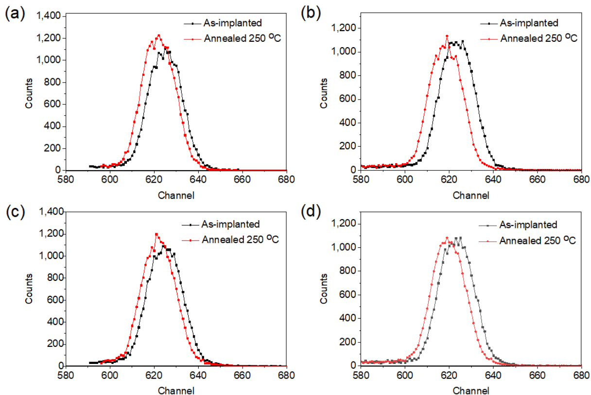
Figure 4-66 Nuclear reaction analysis results for the as-implanted ( 150 \text{ keV He} , 5 \times 10^{15} \text{ cm}^{-2} ) and annealed ( 250 \text{ }^{\circ}\text{C} , 15 minutes) samples (a) Amorphous BAM-11 BMG, (b) partially crystallized BAM-11 BMG, (c) amorphous Cu BMG, and (d) partially crystallized Cu BMG.
