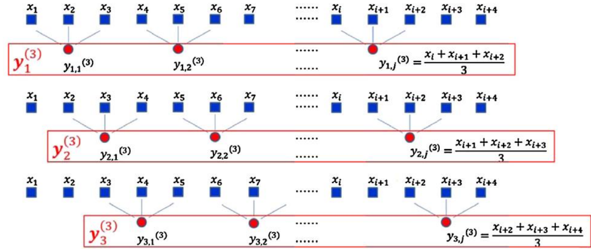
Figure 2-19 Schematic illustration of the coarse-graining procedure (from Ref. [186]).
