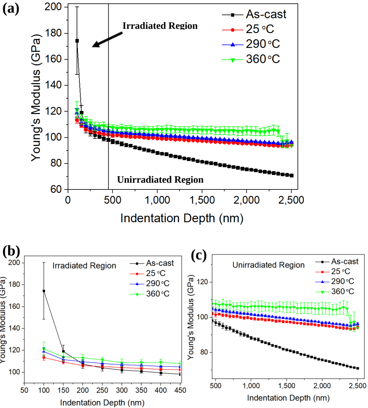
Figure 4-21 Nanoindentation Young's modulus vs. depth for BAM-11 BMG as-cast and irradiated samples (9 MeV \text{Ni}^{3+} , 10 dpa) at temperatures ranging from 25 to 360 °C for (a) depths of 100 to 2500 nm, (b) the irradiated region (100-450 nm), and the (c) unirradiated region (450-2500 nm).
