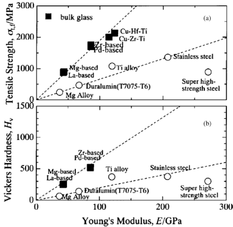
Figure 2-15 The relations between the mechanical properties of typical BMGs: (a) tensile fracture strength and (b) Vicker's hardness as a plot of Young's modulus (from Ref. [113]).
