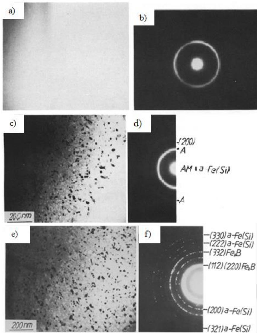
Figure 2-31 BF TEM images and DPs for (\text{Fe}_{0.99}\text{Cu}_{0.01})_{78}\text{Si}_9\text{B}_{13} (a) as-quenched (c) annealed (583 K, 15 min) (e) fully crystallized. Here, (b), (d), and (f) are the corresponding diffraction patterns for (a), (c), and (e) respectively (from Ref. [264]).
