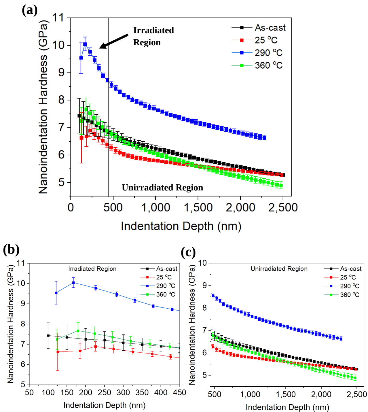
Figure 4-26 Nanoindentation hardness vs. depth for BAM-11 BMG as-cast and irradiated samples (5.5 MeV C^{+} , 0.5 dpa) at different temperatures (a) depths ranging from 100-2500 nm, (b) the irradiated region (100-450 nm), and the (c) unirradiated region (450-2500 nm).
