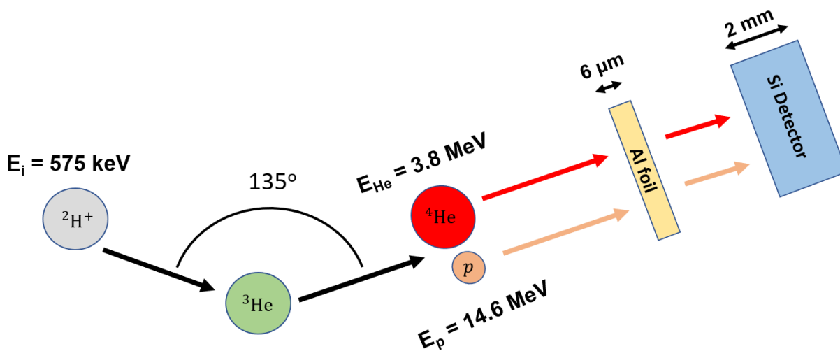
Figure 3-44 Basic schematic of the NRA scattering process (from Ref. [408]).
