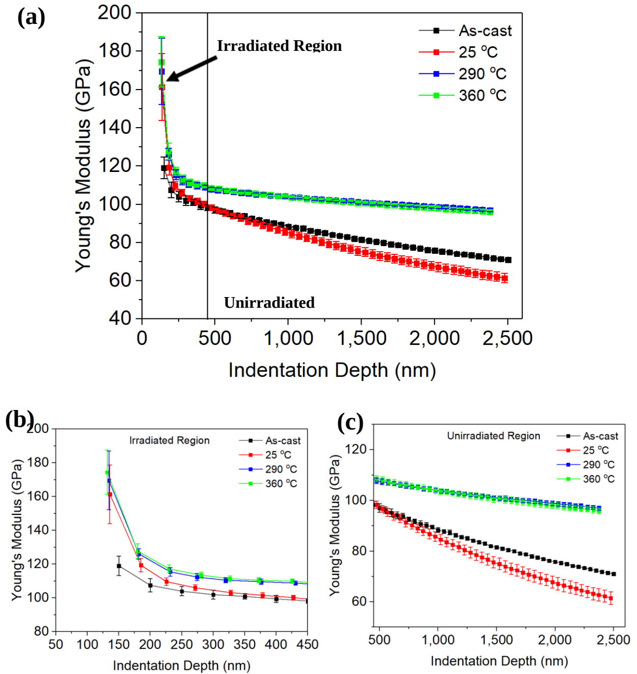
Figure 4-25 Nanoindentation Young's modulus vs. depth for BAM-11 BMG as-cast and irradiated samples (9 MeV \text{Ni}^{3+} to 0.5 dpa) at temperatures ranging from 25 to 360 °C for (a) depths of 100-2500 nm, (b) the irradiated region (100-450 nm), and the (c) unirradiated region (450-2500 nm).
