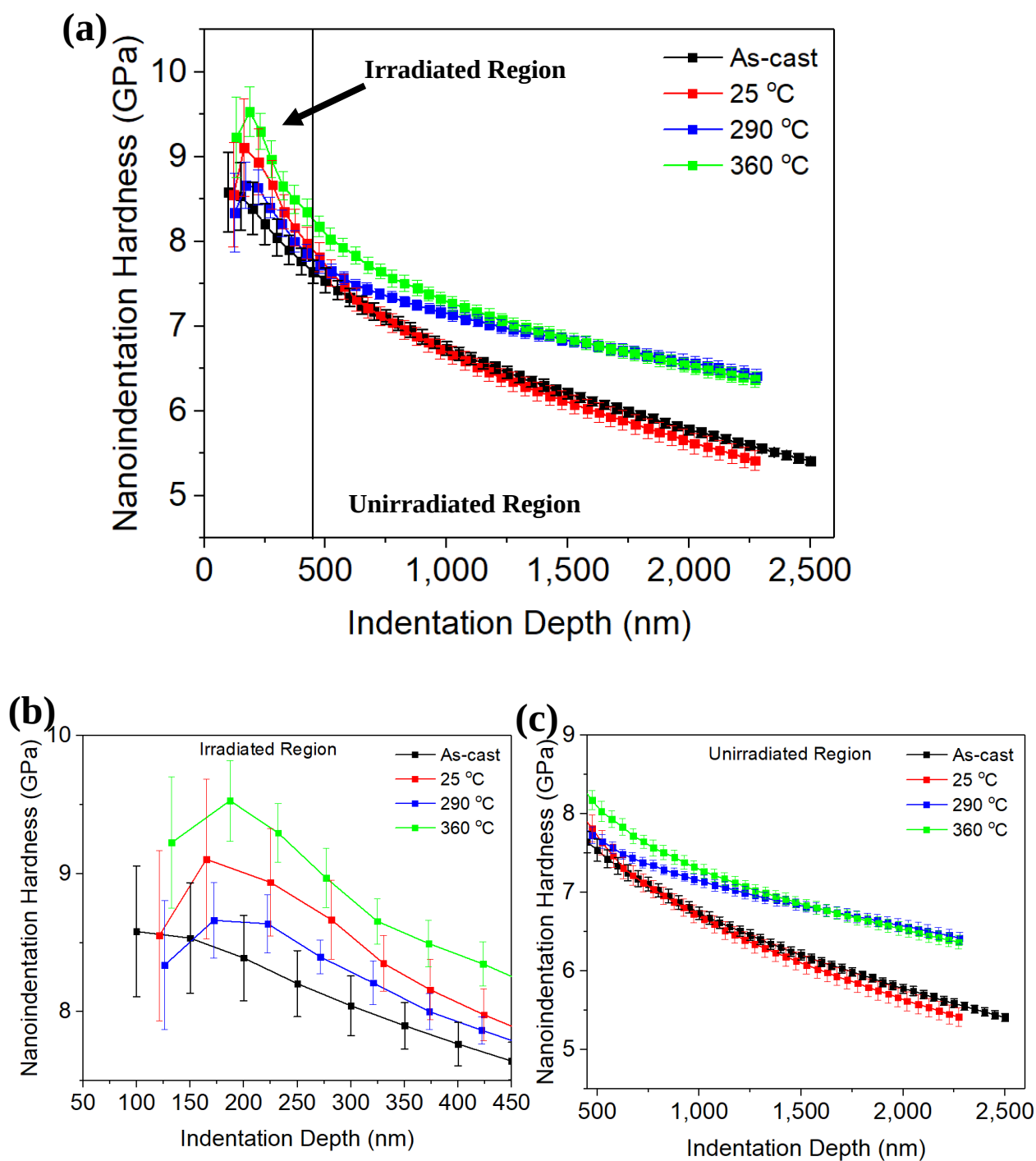
Figure 4-31 Nanoindentation hardness vs. depth for Cu BMG as-cast and irradiated samples (9 MeV \text{Ni}^{3+} , 0.5 dpa) at different temperatures for (a) depths ranging from 100-2500 nm, (b) the irradiated region (100-450 nm), and the (c) unirradiated region (450-2500 nm).
