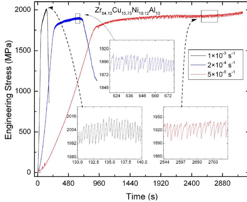
Figure 2-16 Compression stress-time profiles of \text{Zr}_{64.13}\text{Cu}_{15.75}\text{Ni}_{10.12}\text{Al}_{10} BMG cylindrical samples. Samples were compressed at strain rates of 1 \times 10^{-3} \text{ s}^{-1} , 2 \times 10^{-4} \text{ s}^{-1} , and 5 \times 10^{-5} \text{ s}^{-1} at room temperature (from Ref. [136]).
