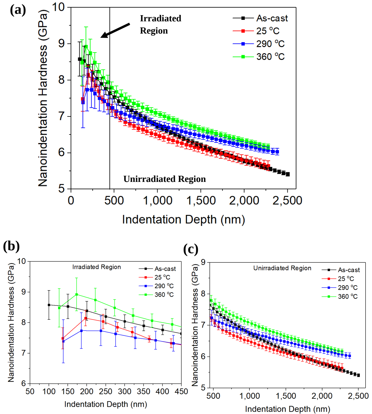
Figure 4-33 Nanoindentation hardness vs. depth for Cu BMG as-cast and irradiated samples (5.5 MeV C^+ , 0.5 dpa) at different temperatures for (a) depths ranging from 100-2500 nm, (b) the irradiated region (100-450 nm), and the (c) unirradiated region (450-2500 nm).
