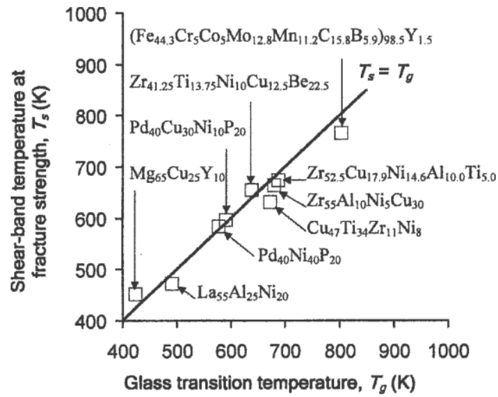
Figure 2-12 Comparison between glass-transition temperature and calculated shear-band temperature at fracture strength for different BMGs (from Ref. [145]).
