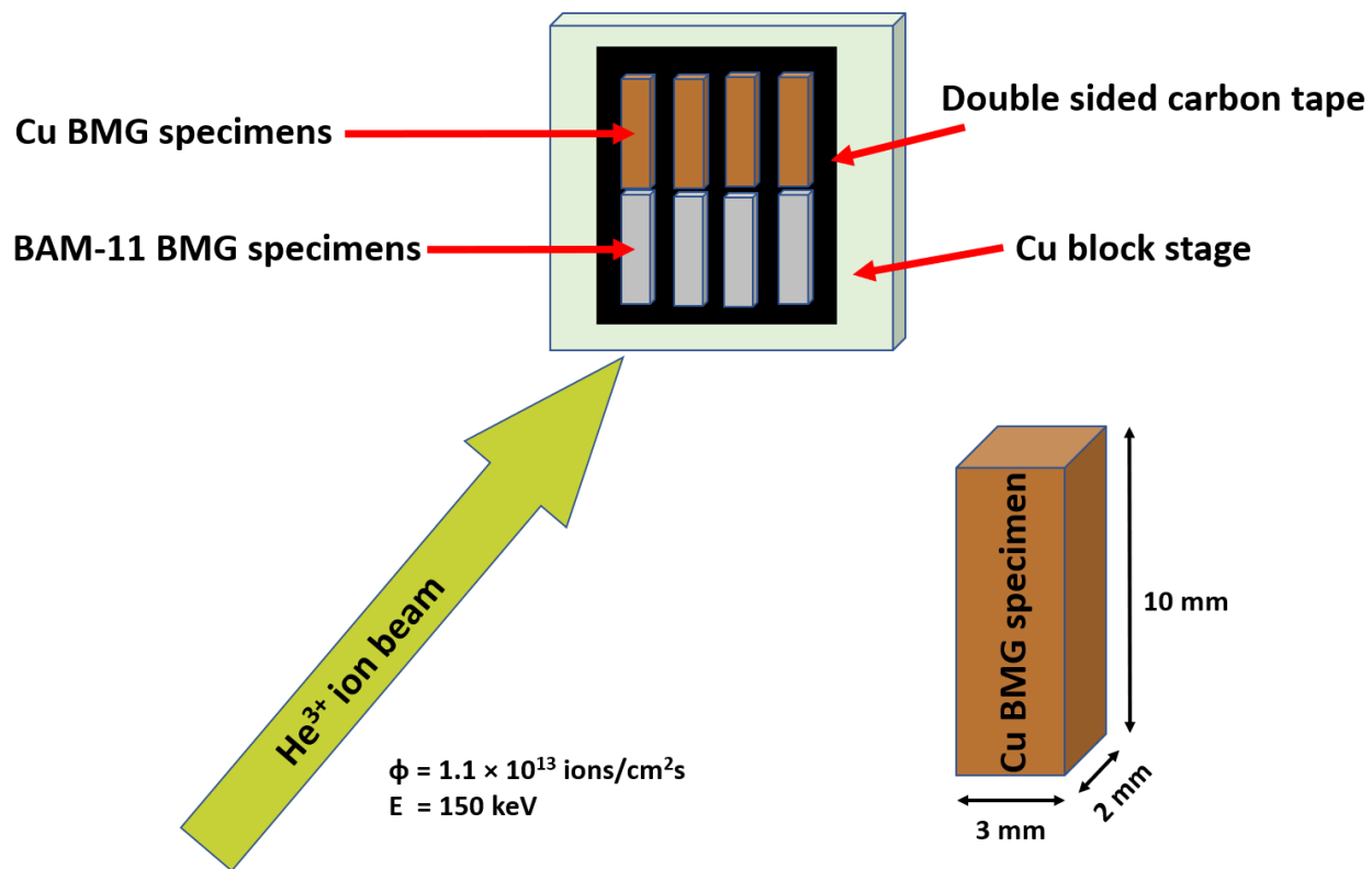
Figure 3-43 Schematic showing the 150 keV ^3\text{He}^+ ion irradiations of the 3 mm \times 2 mm \times 10 mm specimens.
