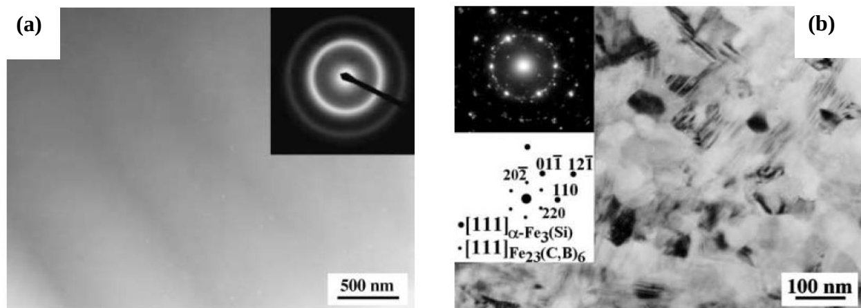
Figure 2-35 TEM bright-field SAED Patterns for \text{Fe}_{72}\text{Si}_{9.1}\text{B}_{14.8}\text{Cr}_{2.2}\text{C}_{1.9} amorphous alloy (a) The as-spun ribbon, (b) Ribbon heated up to 923 K (from Ref. [266]).
