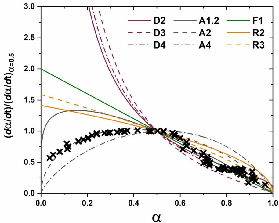
Figure 4-45 Isothermal masterplot and Avrami fit of the formation of tetragonal \text{Zr}_2\text{Ni} (ICDD #04-004-3205 [425]).
