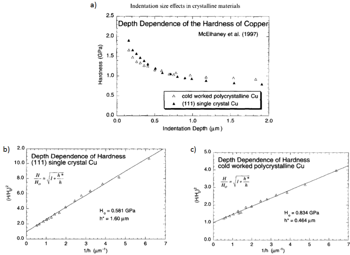
Figure 2-23 (a) Hardness of (111) single crystal and cold worked polycrystalline copper, (from Ref. [212]). (b) Nix-Gao extrapolation of the hardness data of (111) single copper, and (c) Nix-Gao extrapolation of the hardness data of polycrystalline copper.
