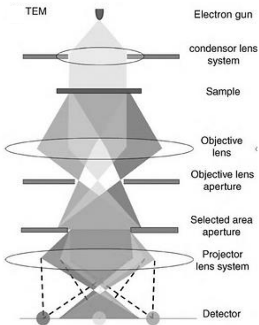
Figure 2-29 Simplified Schematic diagram of the principles of TEM imaging and diffraction (from Ref. [265]).
