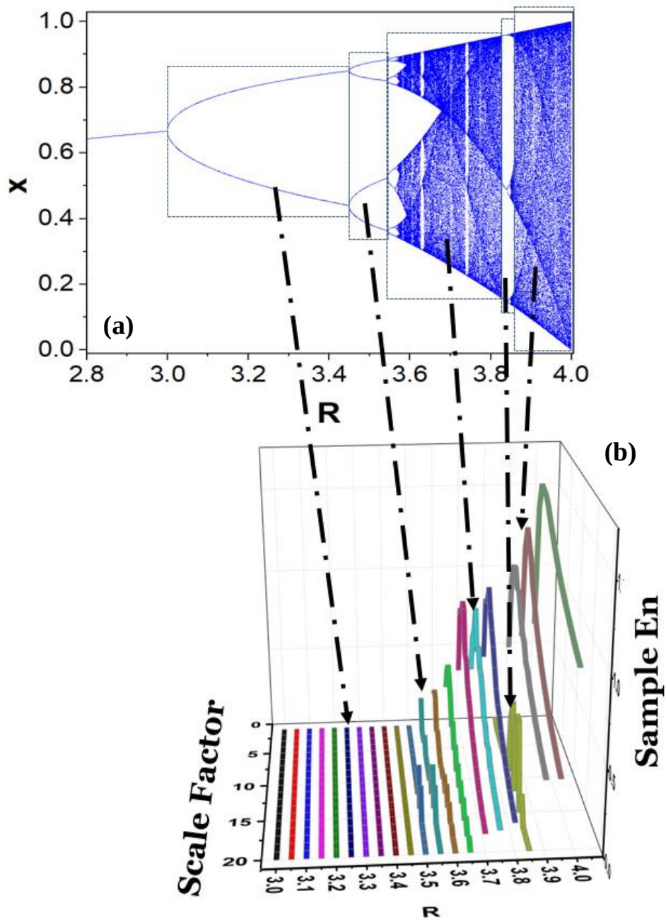
Figure 2-20 (a)-(b) The bifurcation diagram (plotted for 2.8 \leq R \leq 4.0 ) for the logistic map with arrows that link the various regions of the map to its corresponding sample-entropy curves from (Ref. [190]).
