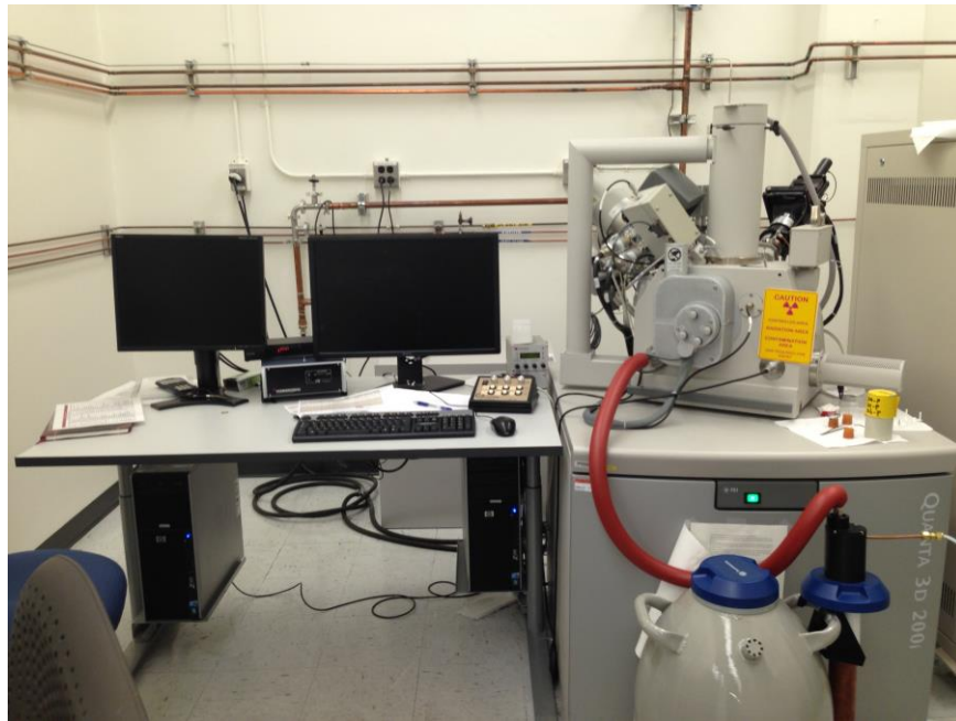
Figure 3-20 FEI Quanta Dual-beam FIB/SEM that is located in the LAMDA facility in ORNL.
