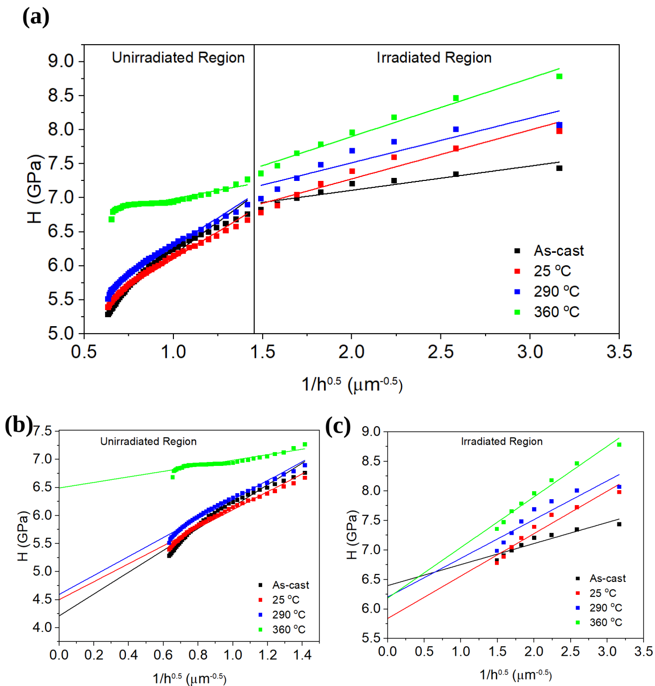
Figure 4-23 H vs. 1/h^{0.5} for BAM-11 BMG in the as-cast and irradiated (9 MeV \text{Ni}^{3+} , 10 dpa at temperatures of 25-360 °C) samples for depths of (a) 100-2500 nm, (b) the unirradiated region (450 nm-2500 nm), and (c) the ion irradiated region (100-450 nm).
