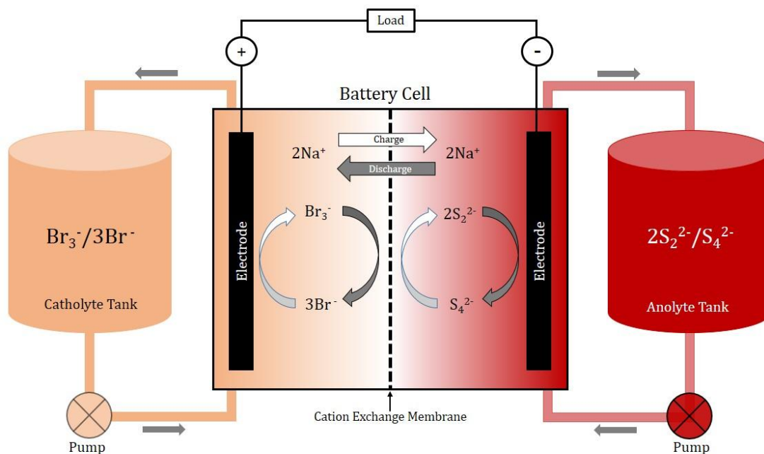
Figure 1: BPSRFB System
