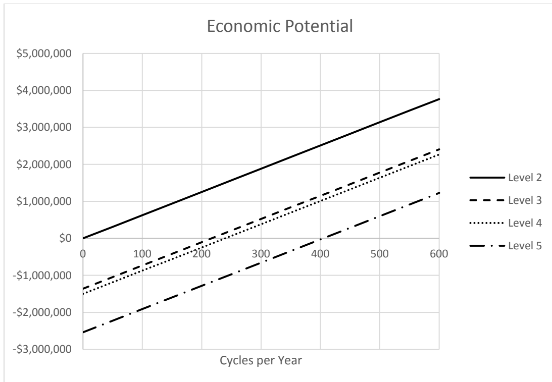
Figure 5: Case 3, 1.1V, 250A/m 2
