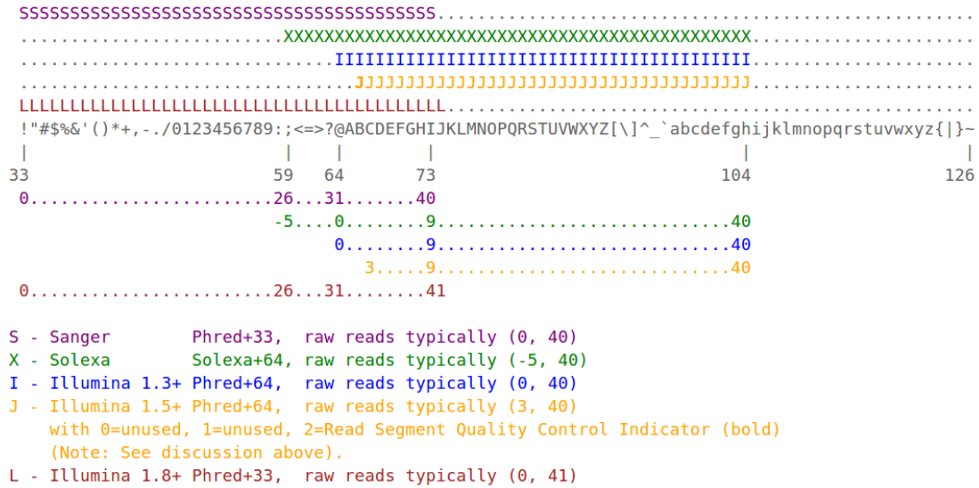
Figure 1.4: The phred quality score for different sequencing vendors. The integer value of valid ascii characters used to encode this information, and the resulting quality score after offset.
