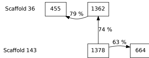
Figure G.99: Paralagous group 59 of the RxLR effector family.
