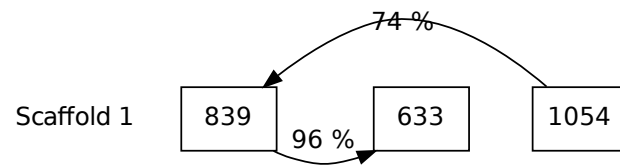
Figure G.83: Paralagous group 66 of the RxLR effector family.
