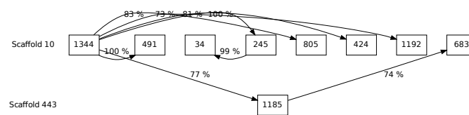
Figure G.117: Paralagous group 33 of the RxLR effector family.
