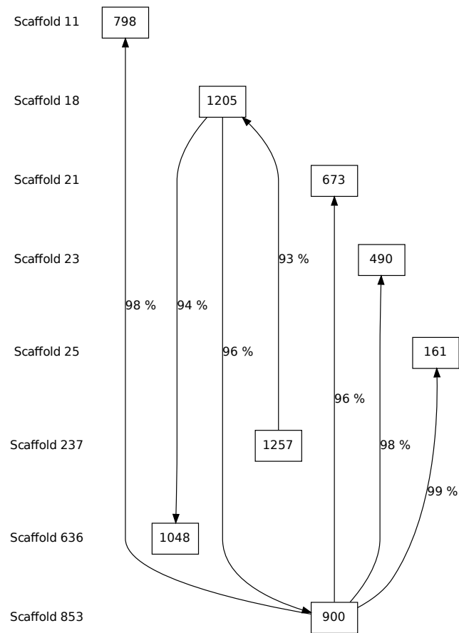
Figure G.112: Paralagous group 109 of the RxLR effector family.
