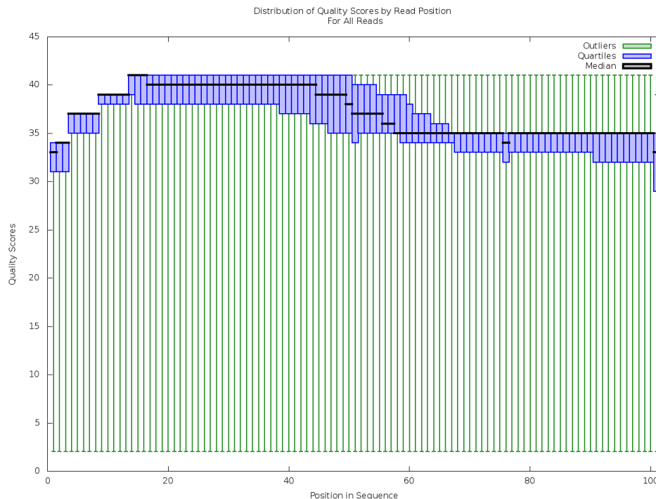
Figure 2.9: Distribution of quality scores at each position in the necrotrophic nucleotide sample.
