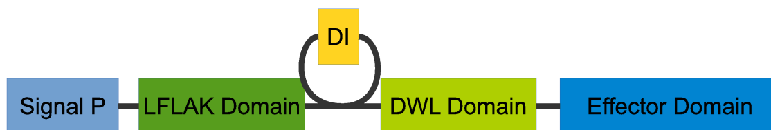
Figure 1.3: The modular structure of the CRN Family. A CRN has a signal peptide, and LFLAK domain, a potential DI domain, a DWL domain, and a trailing effector domain [74].
