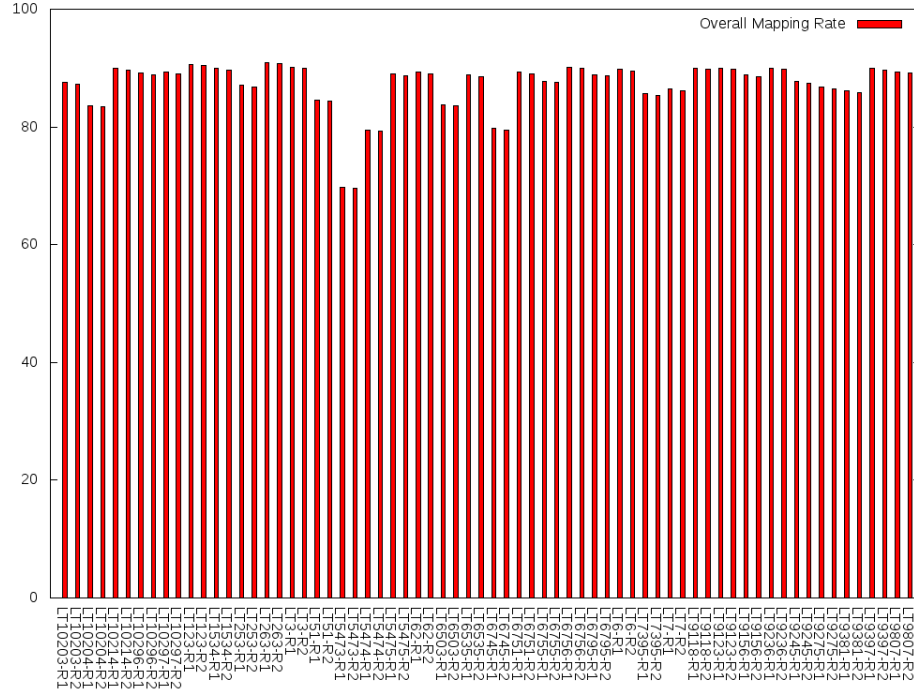
Figure 2.11: Average overall mapping rate of transcriptomic samples. Reported mapping statistics as reported by TopHat2 were arithmetically averaged between each isolate.
