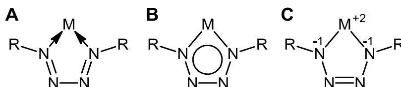
Figure 5.1. Gade's classes of N_4 binding modes found in tetrazene ligands.
