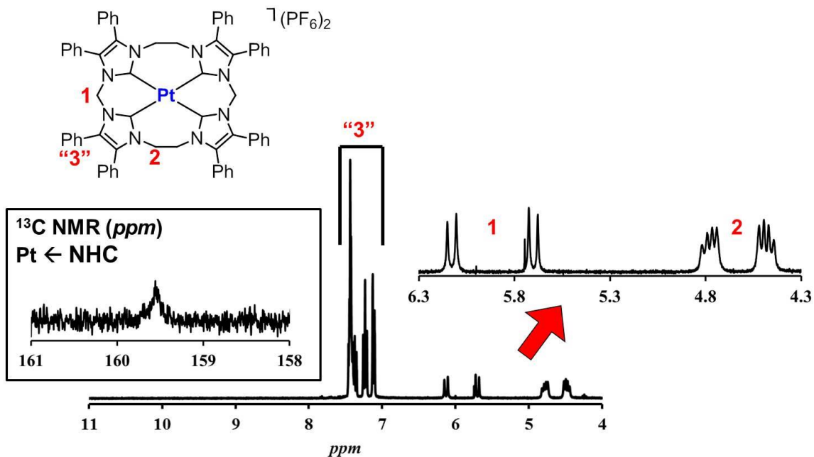
Figure 2.3. Labelled ^1H NMR spectra of [(^{Me, Et}TC^{Ph})Pt](PF_6)_2 and ^{13}C NMR highlight of Pt-NHC chemical shift.
