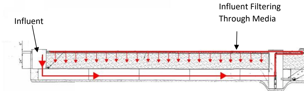
Figure 3.2: RSF Flow
