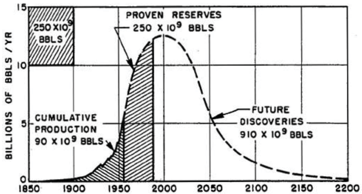
FIGURE 27. Hubbert Curve
