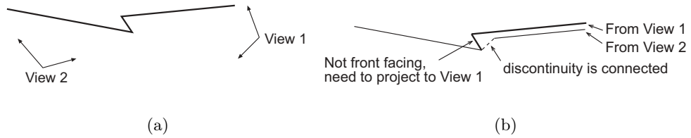
Figure 5.6: Checking overlap for back-facing triangles.
