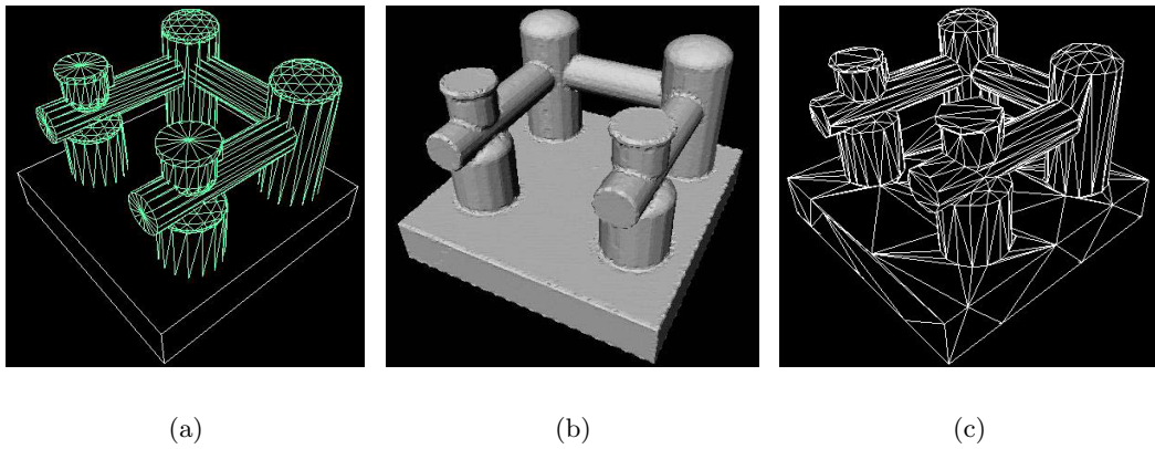
Figure 7.19: Implicit surface-based reconstruction of a synthetic object. (a) Original synthetic model. (b) 44-view reconstructed surface with 119,911 triangles. (c) Simplified surface with 800 triangles.
