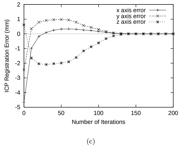
Figure 7.16: ICP refinement. (a) Surface integration result without using the ICP refinement. Note the seam on the forehead. (b) Smooth surface integration result after using the ICP algorithm. (c) Translation errors along three axes during ICP iterations.
