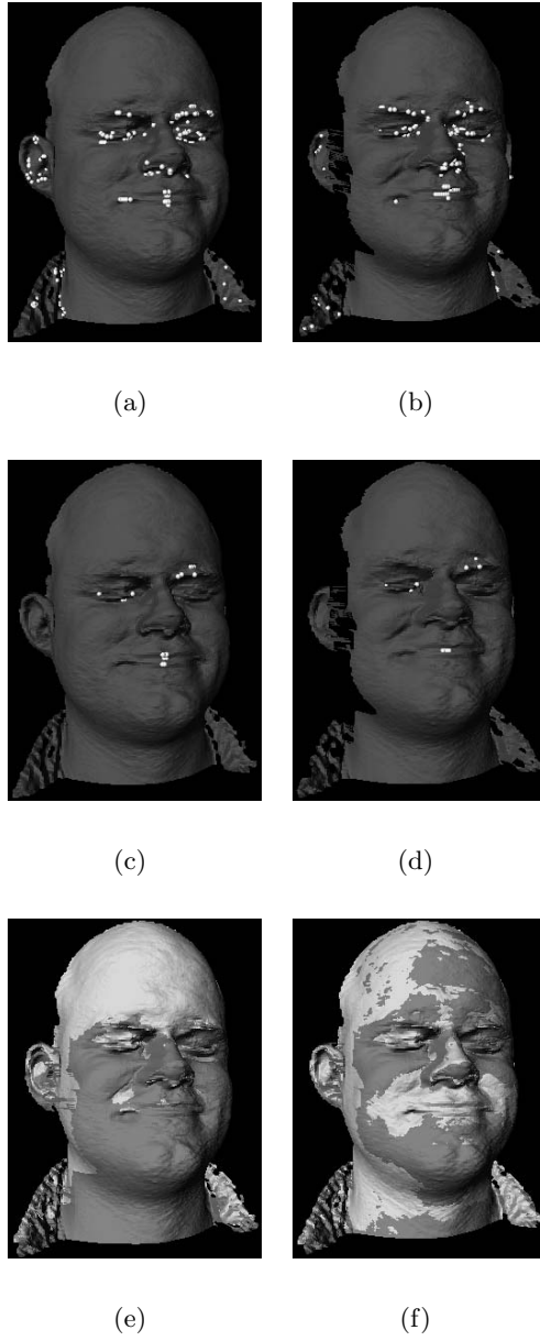
Figure 7.12: Matching surfaces of a face model downloaded from http://sampl.engr.ohio-state.edu/~sampl/database.htm [14]. (a)(b) Extracted feature points on two surfaces. (c)(d) Corresponding points by fingerprint matching. (e) Surface registration. (f) Refined registration using ICP.
