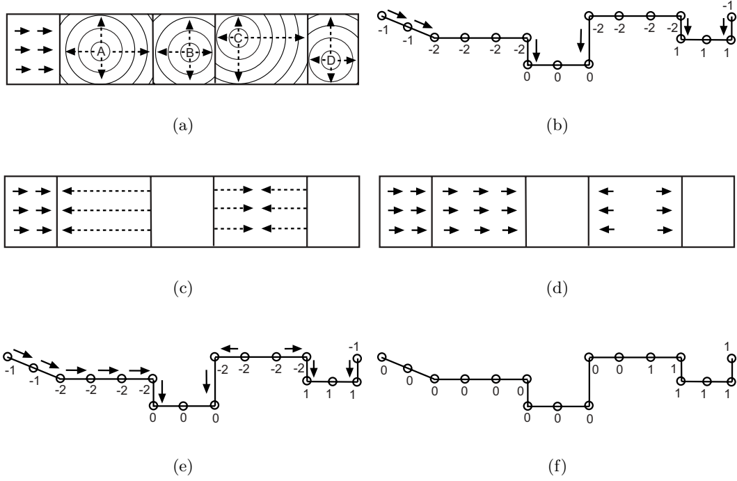
Figure 6.2: Fast marching watershed. (a) A surface patch whose flat regions are extracted by FIFO queue-based flooding. (b) A 2D slice of the height map, on which the minima are uniquely labeled and plateaus are marked as -2. Vertices on ramp and plateau boundaries get v_n represented by solid arrow. (c) Propagate v_n from the plateau boundary by geodesic erosion. (d) v_n at vertex on the plateau is opposite to the erosion direction. (e) All non-minima vertices get v_n . (f) All vertices are labeled by tracing v_n .
