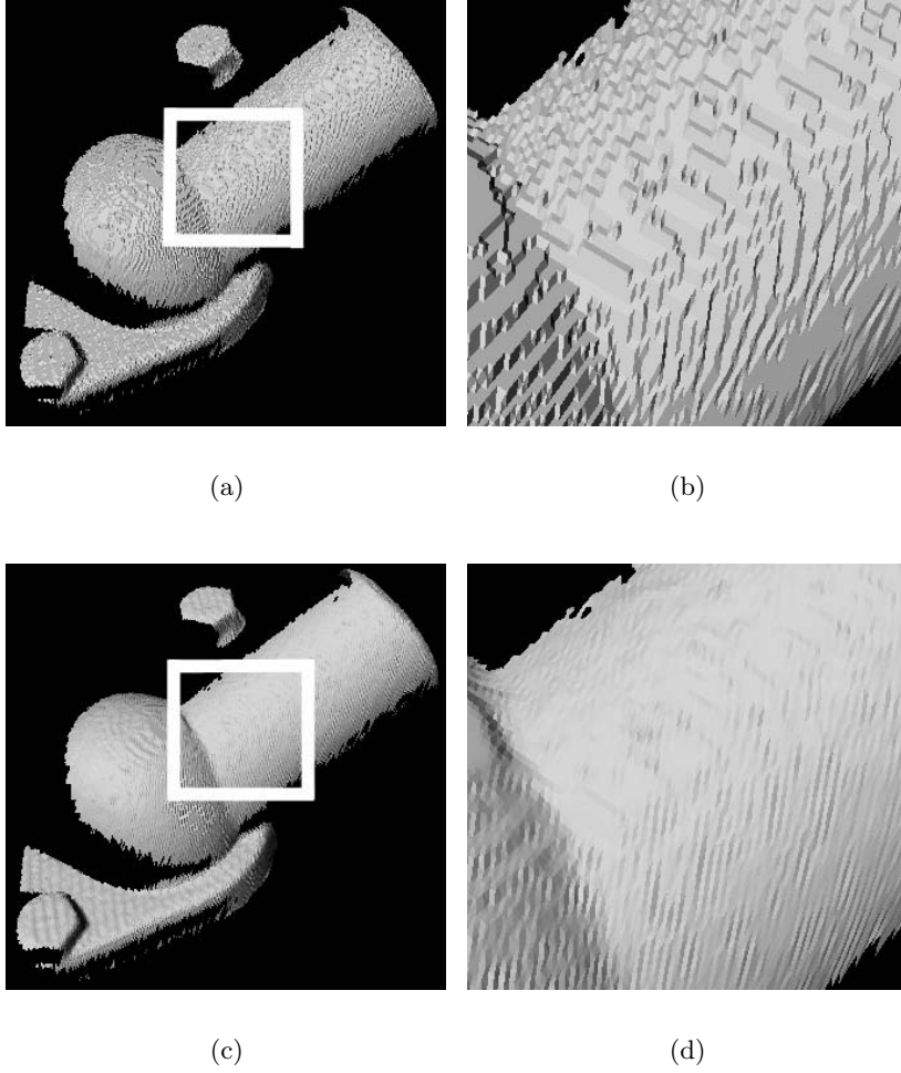
Figure 7.5: Smoothing surfaces from scans of a waterneck captured by the IVP RANGER Profiling System. (a)(b) Surfaces from a range scan of a waterneck and zoomed window. (c)(d) Smoothed surfaces after 2 iterations and zoomed window.
