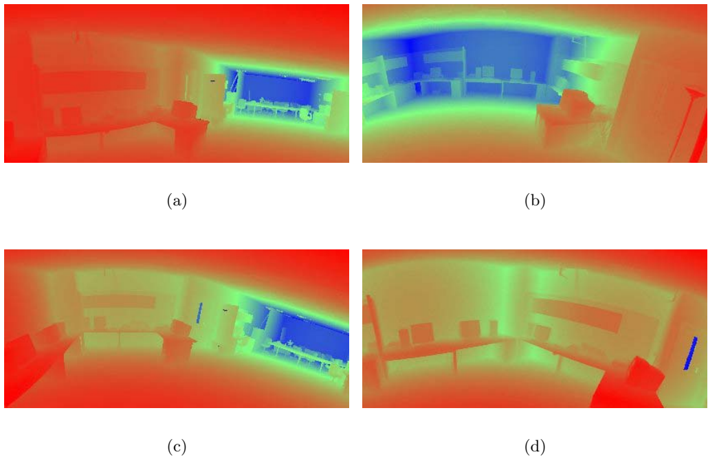
Figure 7.26: Four indoor range images scanned by the RIEGL scanner.
