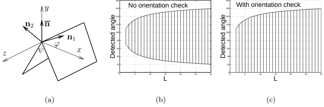
Figure 3.3: Crease edge detection. (a) A crease edge with angle \psi . (b) Angle \psi that can be detected without an orientation check. Edges with sharp angles are missing. (c) Angle \psi that can be detected with an orientation check. L is the factor in (3.48).
