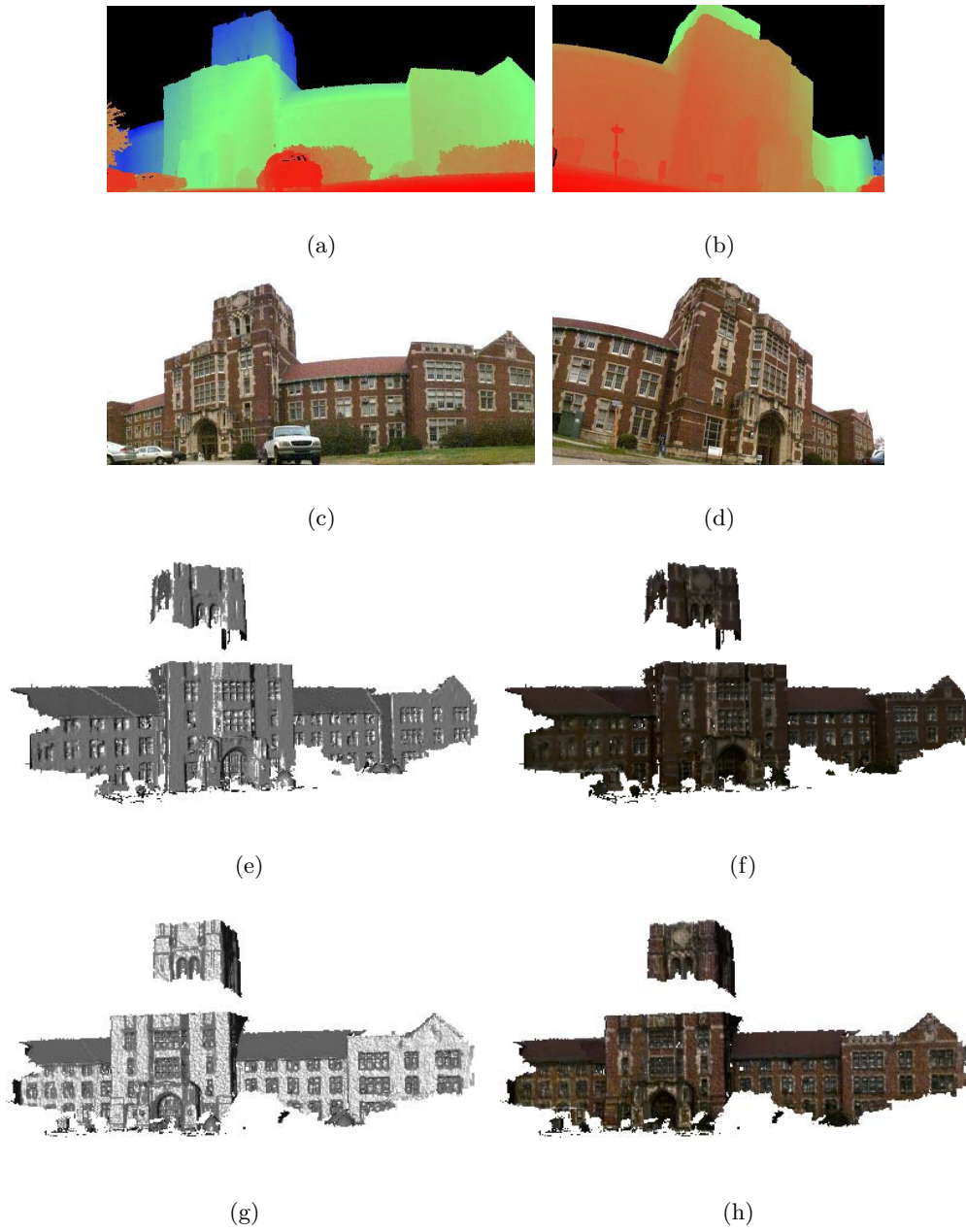
Figure 7.25: Surface modeling using the RIEGL scanner. (a)(b) A pair of range images captured by the RIEGL scanner. (c)(d) Corresponding color images. (e) 2-view 3D reconstruction from (a) and (b) with 159,677 triangles. (f) Reconstructed surface with texture fusion. (g)(h) Reconstructed surface displayed from another viewpoint.
