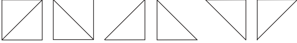
Figure 5.1: Triangulation of a single range image. There are six possible configurations for the creation of triangles from four neighboring points.
