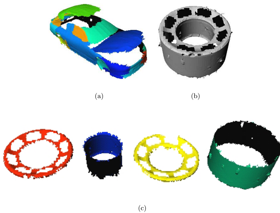
Figure 7.31: Manipulating segmented parts. (a) The hood is open and the top is moved. (b) A 3D pulley model. (c) The decomposition of (b).
