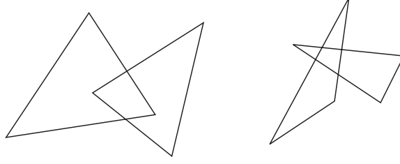
Figure 5.4: Intersecting triangles.
