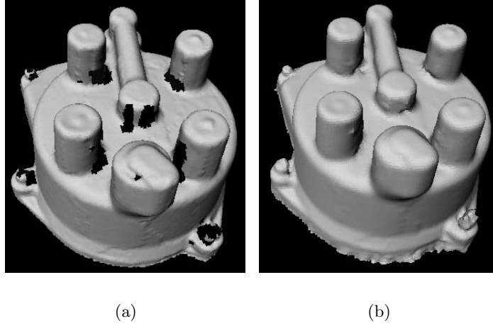
Figure 7.23: Automatic hole filling. (a) Reconstructed surface with holes. (b) Surface after automatically filling holes.
