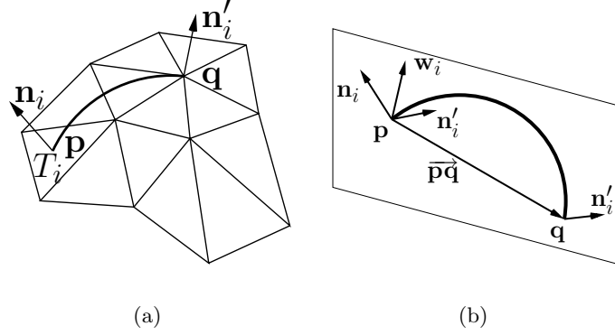
Figure 3.2: Surface normal voting. (a) \mathbf{n}'_i is the voted normal by T_i 's normal \mathbf{n}_i . (b) The normal \mathbf{n}_i at \mathbf{p} is transported through the arc \widehat{\mathbf{p}\mathbf{q}} producing the voted normal \mathbf{n}'_i at \mathbf{q} .
