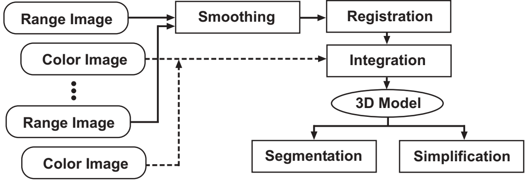
Figure 1.1: A framework for 3D reconstruction and analysis.
