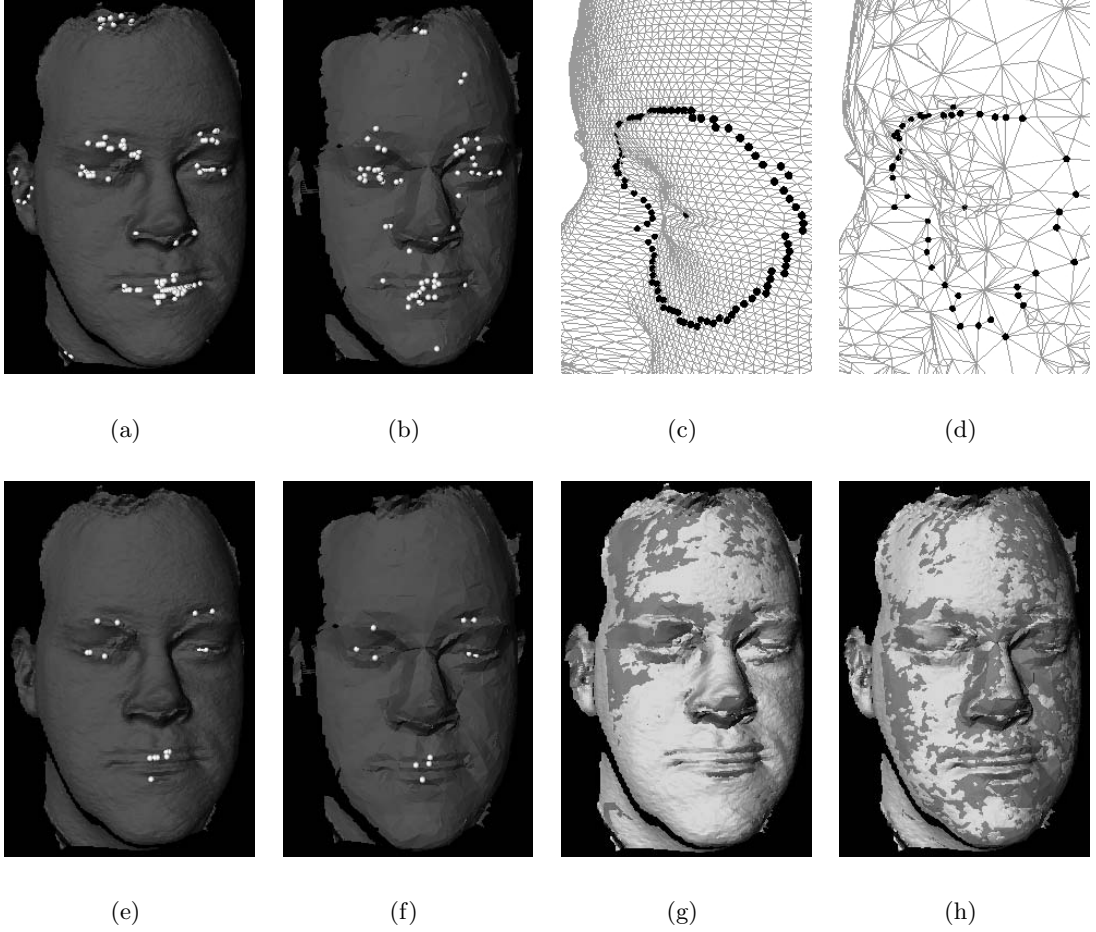
Figure 7.15: Matching surfaces with different resolutions. Original range images were downloaded from http://sampl.engr.ohio-state.edu/~sampl/database.htm [14]. (a)(b) Extracted feature points on two surfaces with 28,964 and 5,000 triangles respectively. (c)(d) Geodesic contours on two surfaces. (e)(f) Corresponding points by fingerprint matching. (g) Surface registration. (h) Refined registration using ICP.
