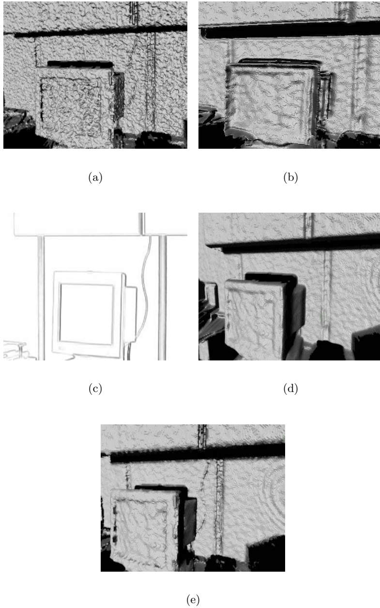
Figure 7.3: Results of median filtering, nonadaptive and adaptive regularization of range data. (a) Result from 3 by 3 median filtering conducted twice. (b) Result from regularization using Laplacian smoothing term. Note the instability along edges. (c) The edge map. (d) Result from nonadaptive regularization. (e) Result from adaptive regularization. Note the wire on the wall preserved by the adaptive method.
