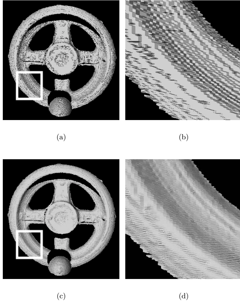
Figure 7.6: Smoothing surfaces from scans of a crank captured by the IVP RANGER Profiling System. (a)(b) Surfaces from a range scan of a crank and zoomed window. (c)(d) Smoothed surfaces after three iterations and zoomed window.
