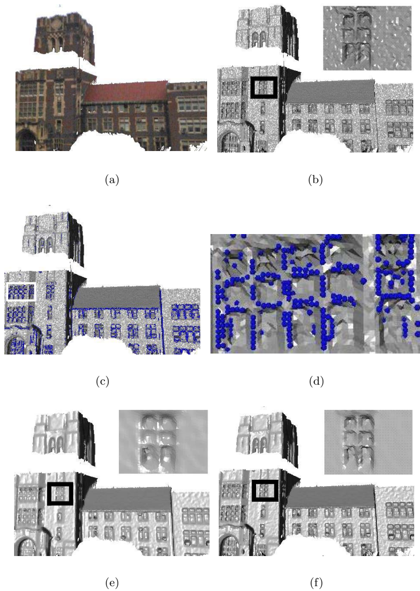
Figure 7.8: Adaptive smoothing of a surface mesh. (a) Raw textured surface captured by the RIEGL laser range scanner. (b) Raw surface without texture, 139,412 triangles. (c) Edge detection. Vertices on the edges are marked by small spheres. (d) Zoomed window frame portion of (c). (e) 5 iterations of nonadaptively smoothed result of (b). (f) 5 iterations of adaptively smoothed result of (b). Note the well preserved window frame structures.
