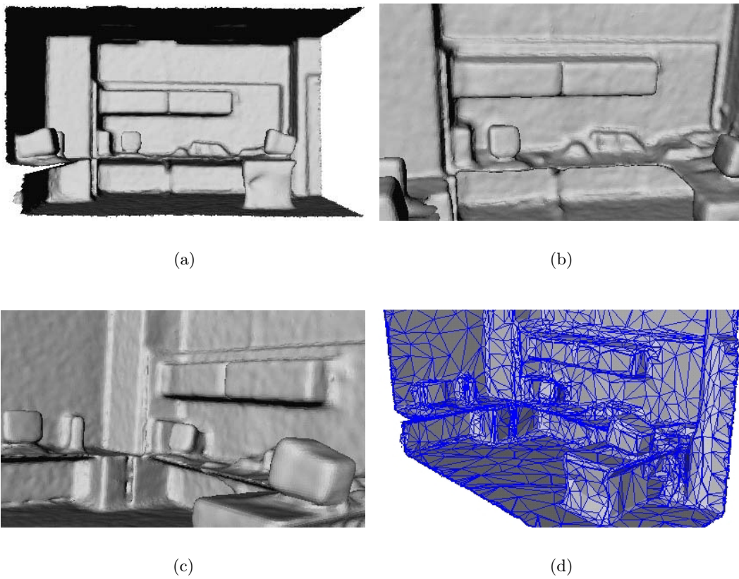
Figure 7.27: Four-view reconstruction using the RIEGL scanner. (a)-(c) Four-view reconstruction using the RIEGL scanner, with 341,639 triangles, displayed from different viewpoints. (d) Simplified model with 5,000 triangles.
