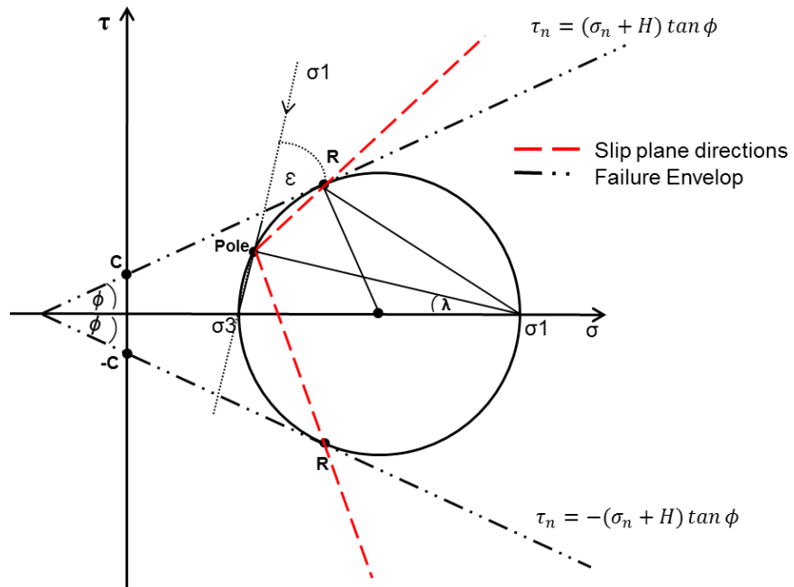
Fig. 4.13. Illustration of slip planes on Mohr-Coulomb diagram.
