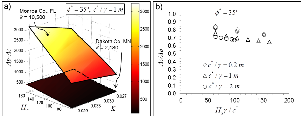
Fig. 5.8. Erosion analyses for the sandy loam soil with \phi = 35^\circ : a) difference in soil loss for the Dakota (dry) and Monroe (wet) Counties; b) A_c / A_p vs H_s \gamma / c^* . Units: A_p - A_c (Mg/Ha/y), R (MJ·mm/ha·h·y), K (Mg·ha·h/ha·MJ·mm), and H_s (m).
