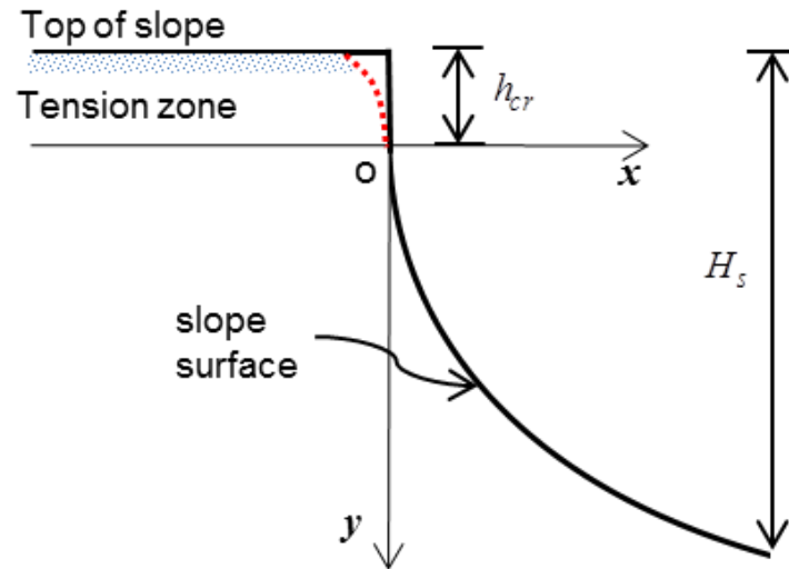
Fig. 5.1. Illustration of the reference frame and the components of the concave slope formulation. In practice the sharp bluff at the top of the slope may be rounded, as indicated by the dashed line.
