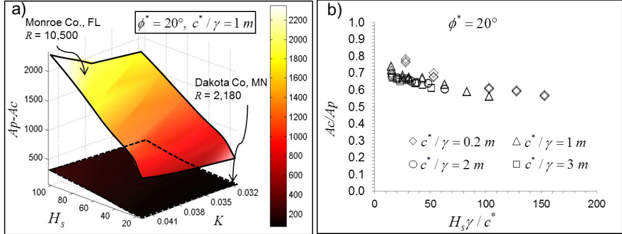
Fig. 5.7. Erosion analyses for the clay soil with \phi = 20^\circ : a) difference in soil loss for the Dakota (dry) and Monroe (wet) Counties; b) A_c / A_p vs H_s \gamma / c^* . Units: A_p - A_c (Mg/Ha/y), R (MJ·mm/ha·h·y), K (Mg·ha·h/ha·MJ·mm), and H_s (m).
