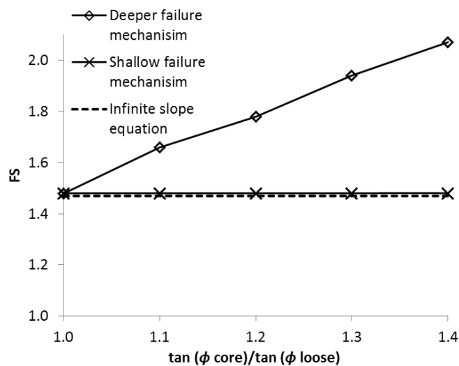
Fig. 2.8. FEM analyses of the global stability for various values of \tan \phi_{core} / \tan \phi_{loose} and the infinite slope equation
