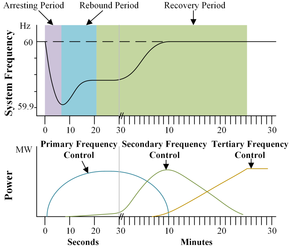
Figure 1.1: Frequency regulation following a disturbance [5, 10].
