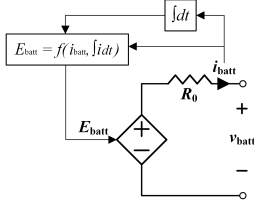
Figure 2.18: Dynamic circuit model for Li-Ion and Pb-Acid batteries [73, 74].
