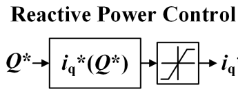
Figure 3.14: Reactive power control for BESS emulator.
