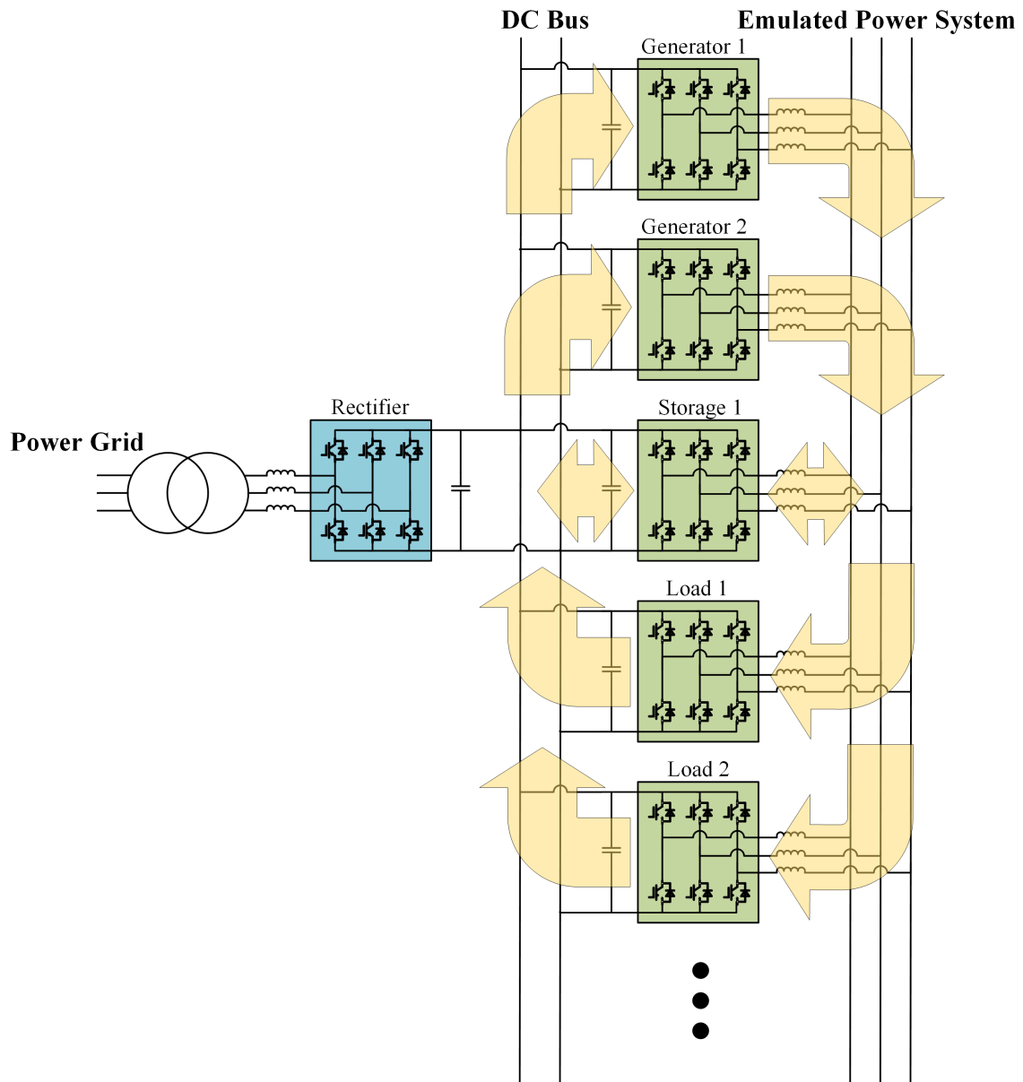
Figure 1.5: Power circulation within the HTB.
