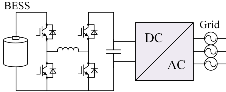
Figure 2.6: Buck-boost cascaded topology for BESS interface [23, 27].
