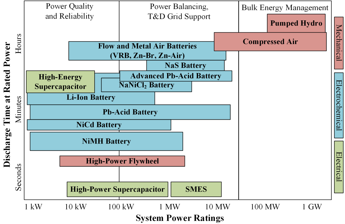
Figure 1.2: Discharge time vs. power rating of energy storage technologies [6, 9, 22, 23, 24, 25].
