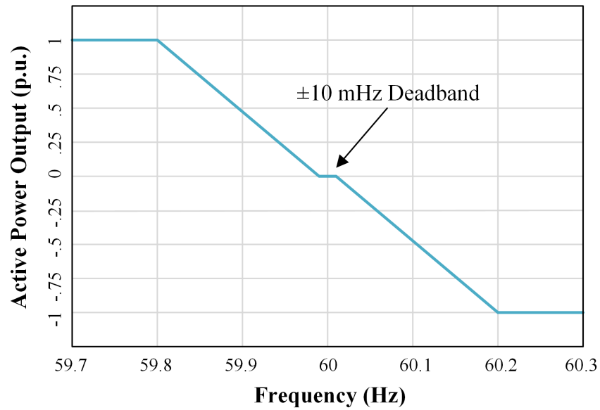
Figure 2.25: Proportional frequency control typical of storage systems [13, 69].
