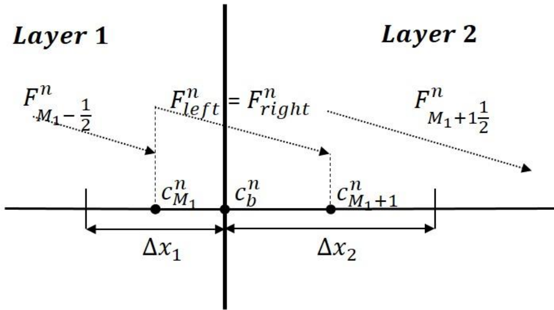
Figure 5.5 Schematic of boundary between two domains.
