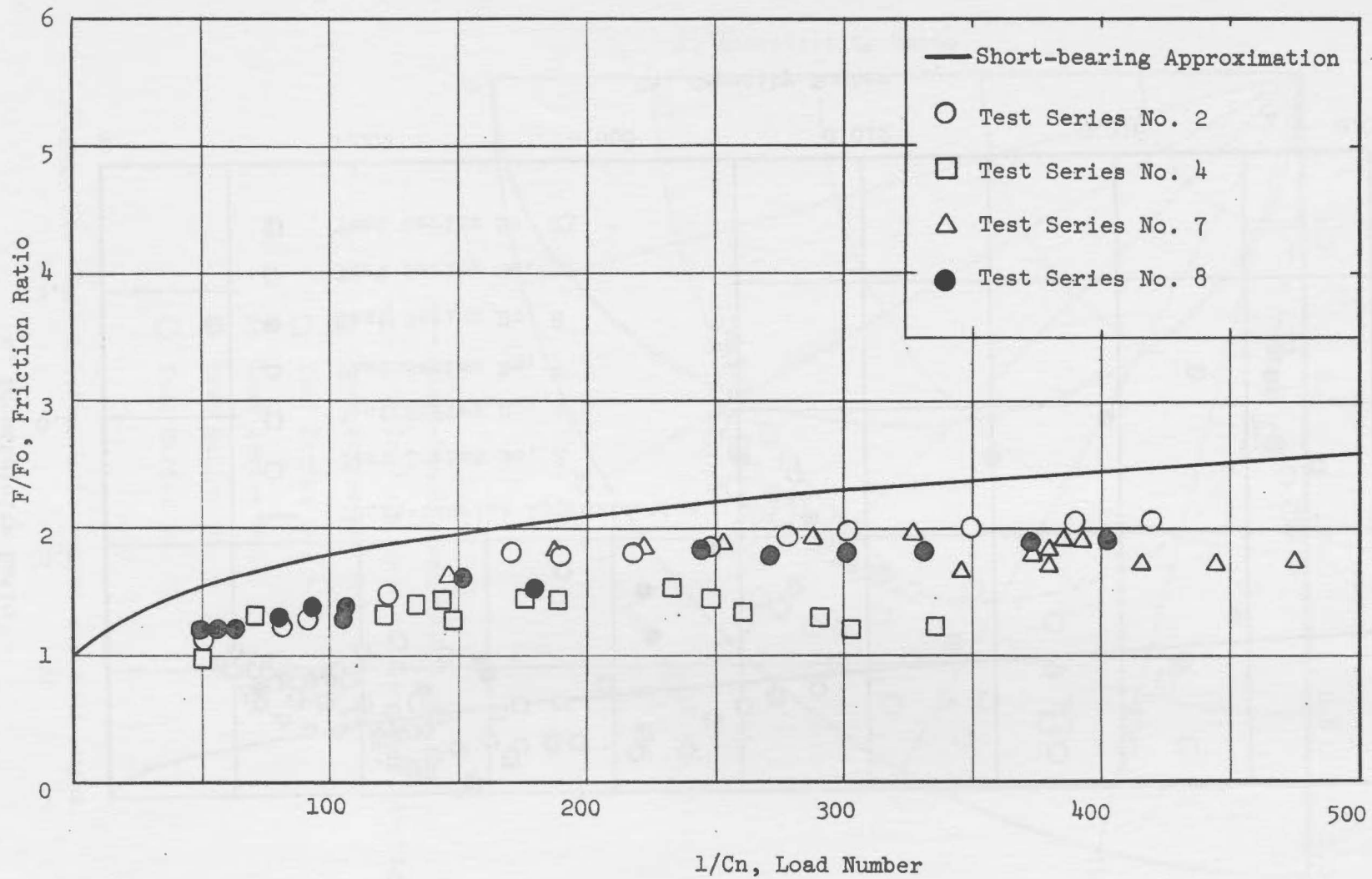
Figure 13. Load number versus friction ratio.
