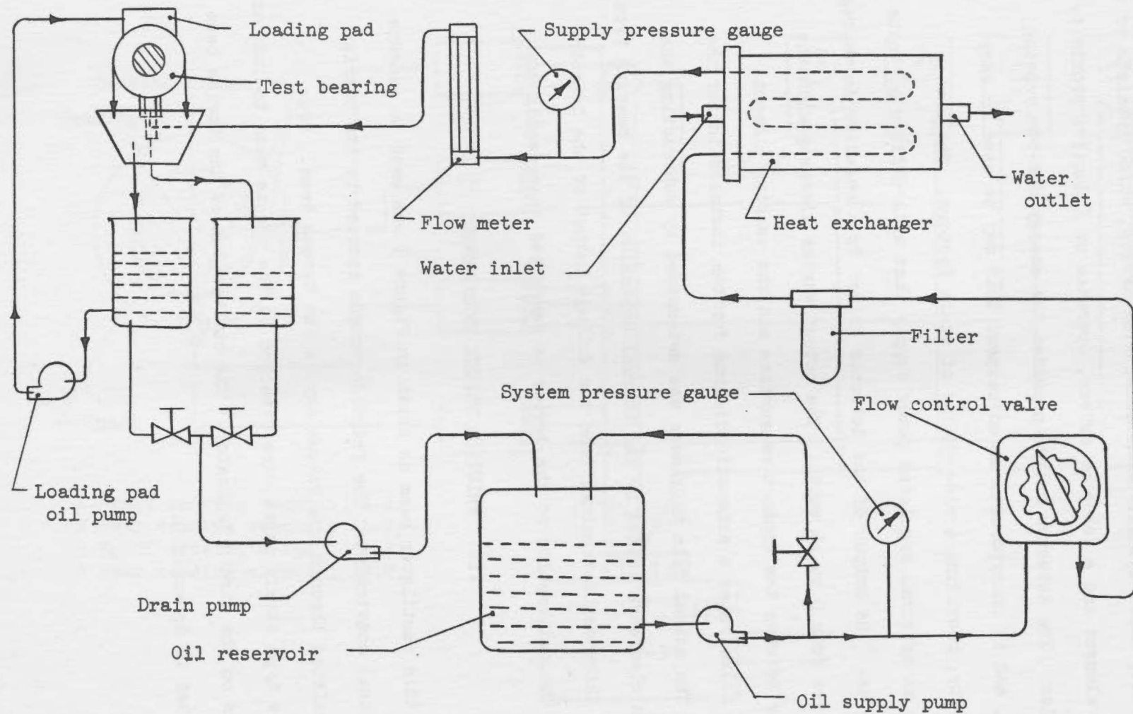
Figure 5. Hydraulic system schematic.
