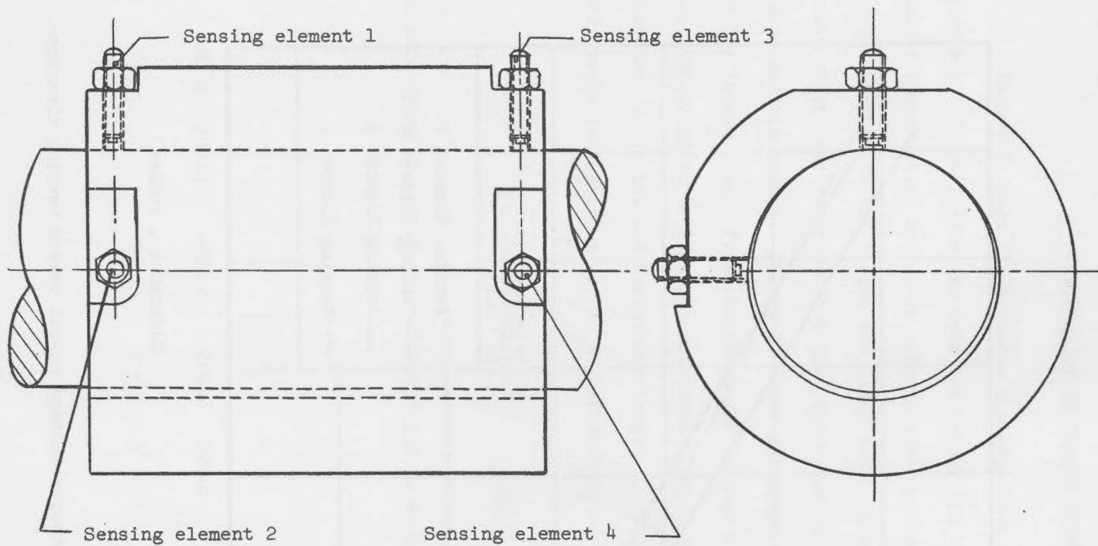
Figure 19. Relative position of sensing elements at the time of calibration.
