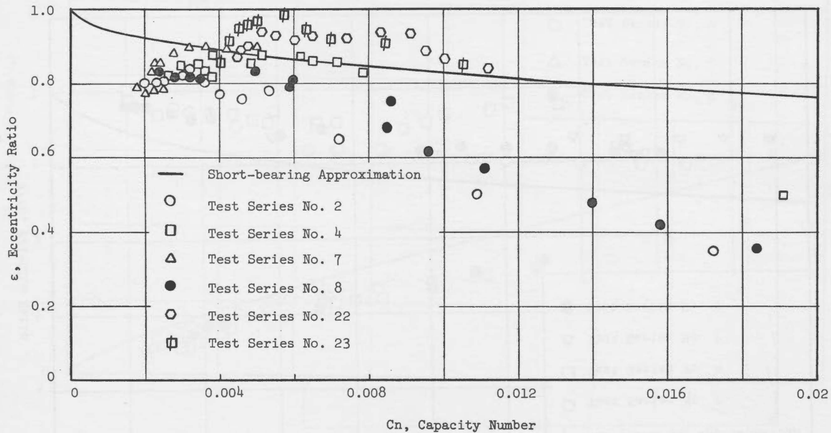
Figure 12. Capacity number versus eccentricity ratio.
