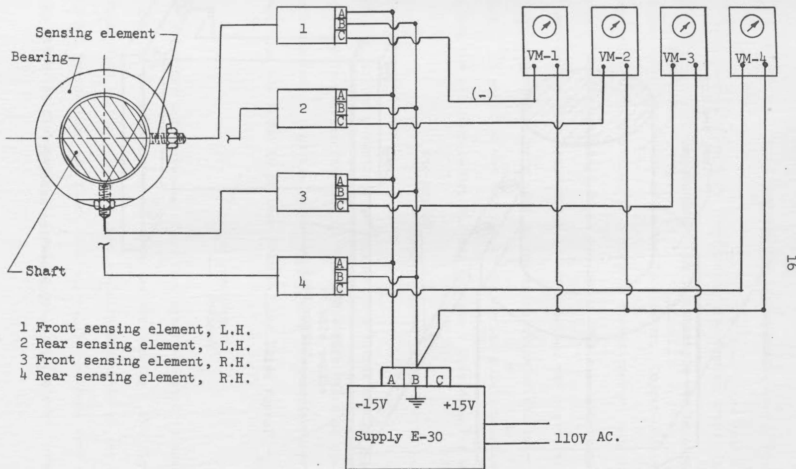
Figure 6. Eccentricity measuring system schematic.
