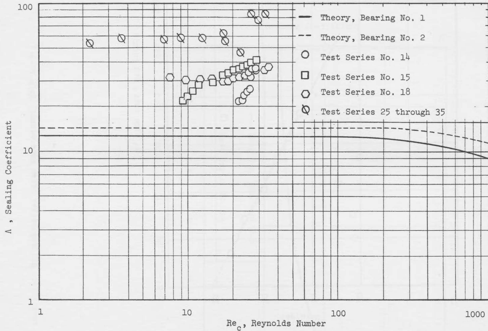
Figure 15. Reynolds number versus sealing coefficient.
