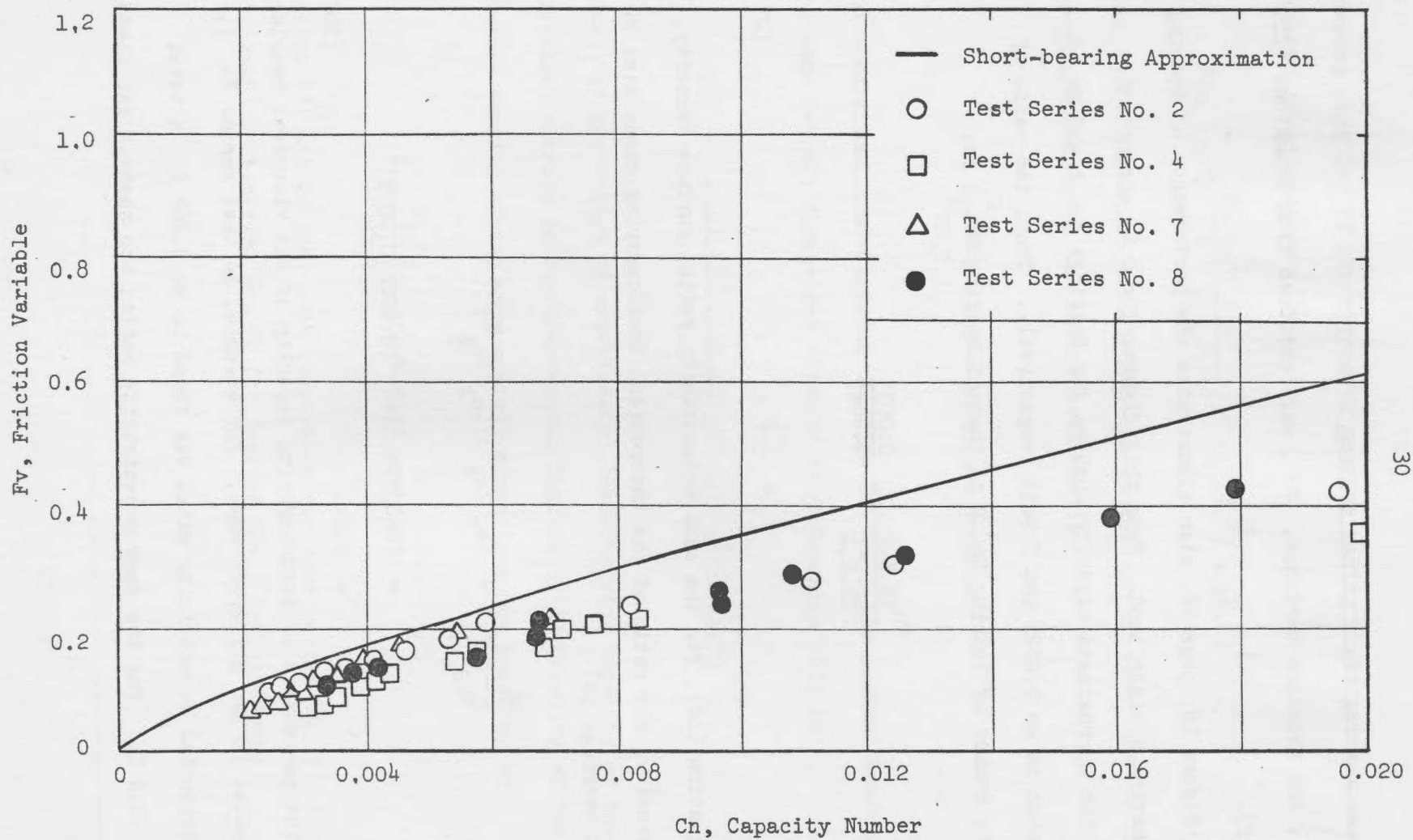
Figure 14. Capacity number versus friction variable.
