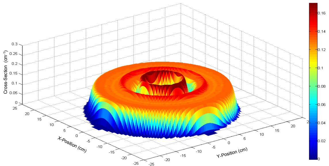
Figure 7-33. A 3D view of the barrel measurement generated using the corrected data. The z-axis and color mapping indicate the estimated material cross sections.
