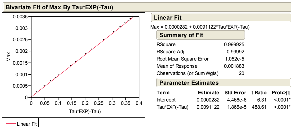
Figure 6-7. A plot of the Maximum of the Gaussian PScF fit versus \tau \text{EXP}(-\tau) for carbon at D = 50 cm. A linear fit of the data is shown. Asterisks in the “Prob>|t|” column indicate statistical significance at the p=0.05 level. Other asterisks indicate multiplication. The “^” symbol indicates exponentiation.
