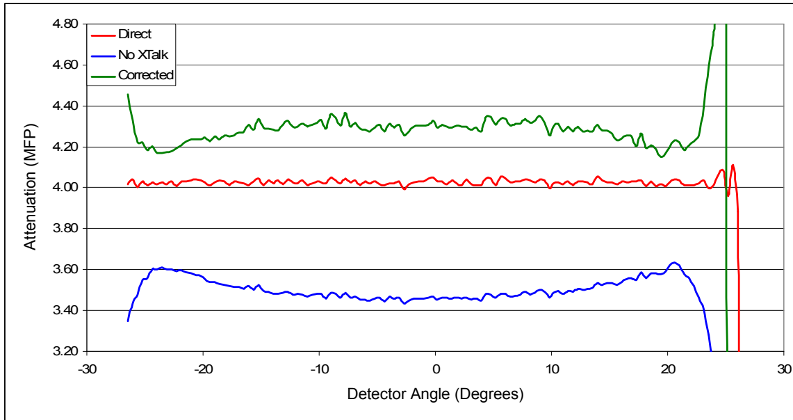
Figure I-7. The attenuation curves for the PoPb scenario. The PSRA used lead PSrF values to correct the scatter.
