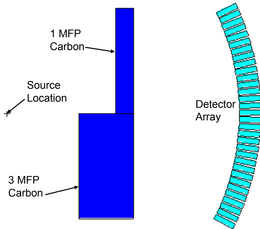
Figure 7-12. The geometry used for simulating measurements of slabs composed of two thicknesses of material. The configuration shown is the C13S scenario.
