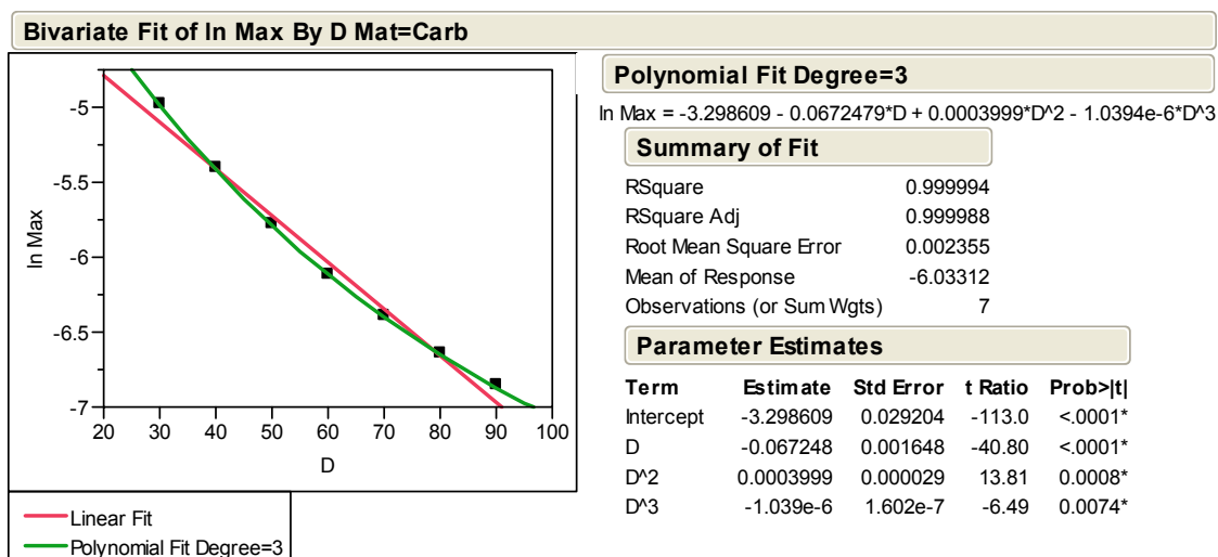
Figure 6-5. A graph of \ln(\text{Max}) of the PScF fit versus object-to-detector distance (D) in cm for 1.5 MFP of carbon. A linear and 3 rd order polynomial fit of the data is shown. Asterisks in the “Prob>|t|” column indicate statistical significance at the p=0.05 level. Other asterisks indicate multiplication. The “^” symbol indicates exponentiation.
