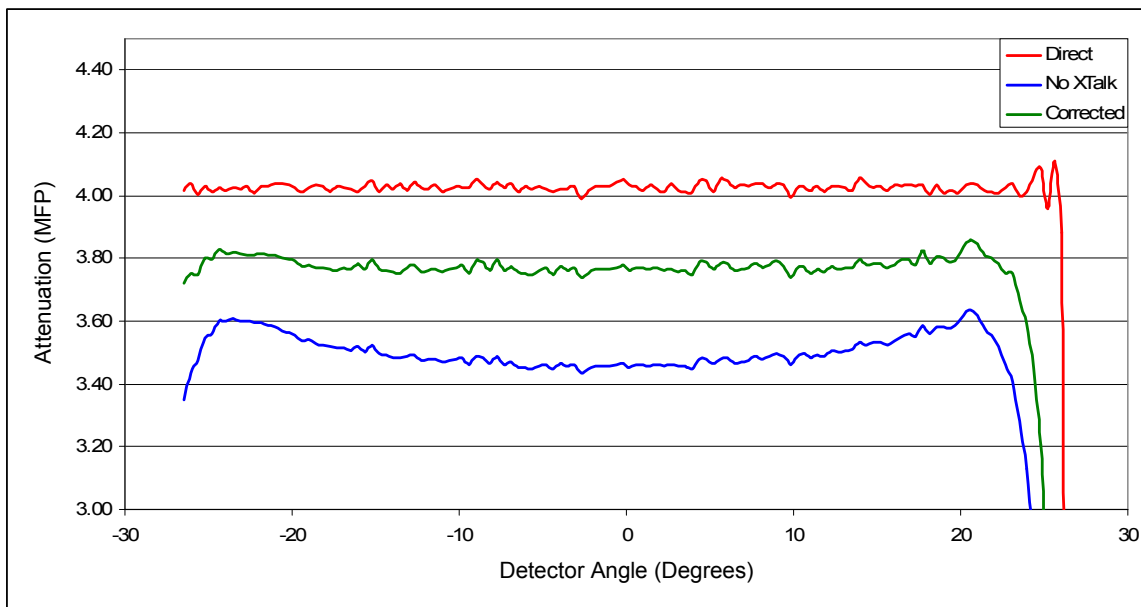
Figure I-8. The attenuation curves for the PoPb scenario. The PSRA used polyethylene PSrF values to correct the scatter.
