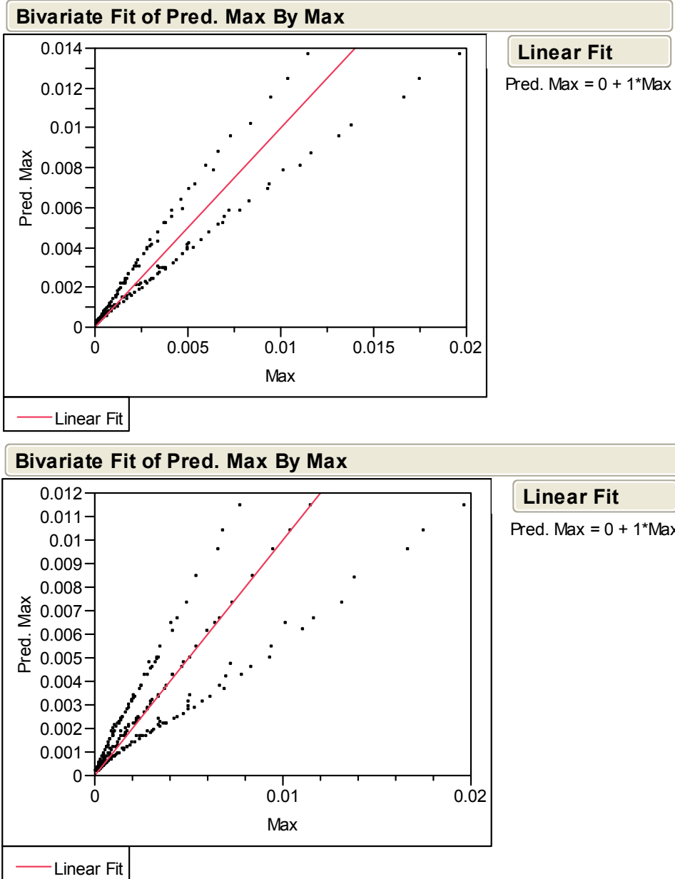
Figure 6-17. Graphs of the predicted PScF Maximum values versus the actual values for material 5 (top) and material 6 (bottom). Points lying on the line correspond to predicted values which match the actual ones. Note the grouping of points that correspond to the individual materials which are being averaged in the definition of these two materials.
