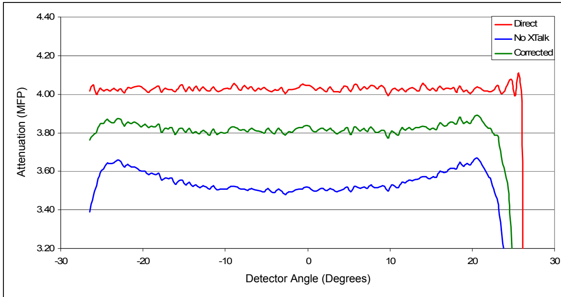
Figure 7-25. The attenuation curves for the PbPo scenario. The PSRA used polyethylene PScF values to correct the scatter.
