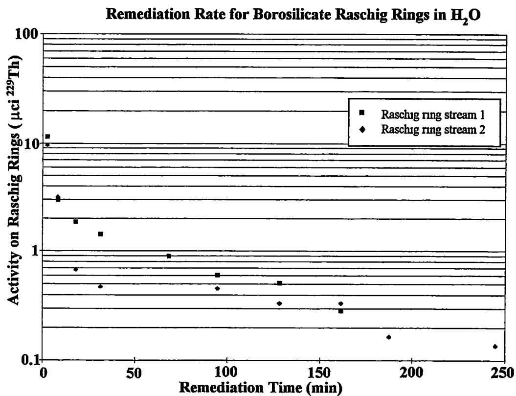
Figure 3.5 Remediation rate for two independent waste streams of radioactively contaminated borosilicate Raschig rings with deionized water and mechanical stirrer agitation.
