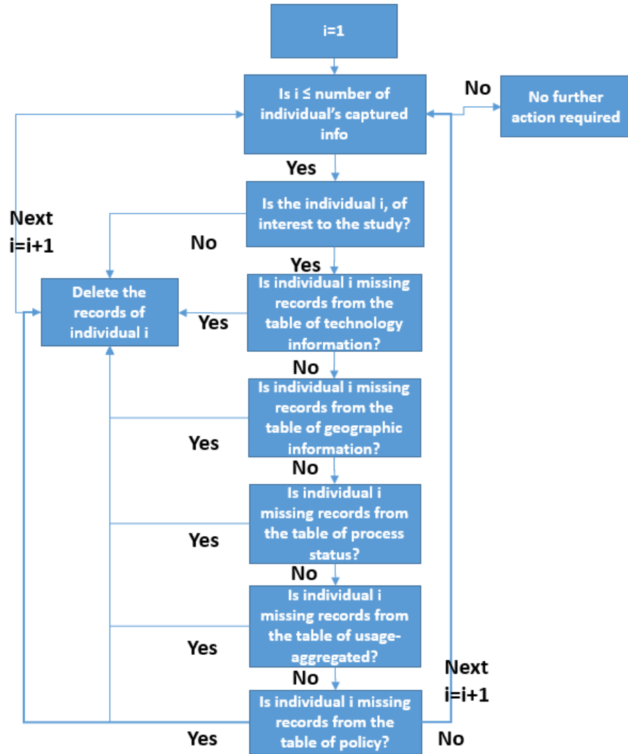
Figure 3.5: Database Accuracy Algorithm
