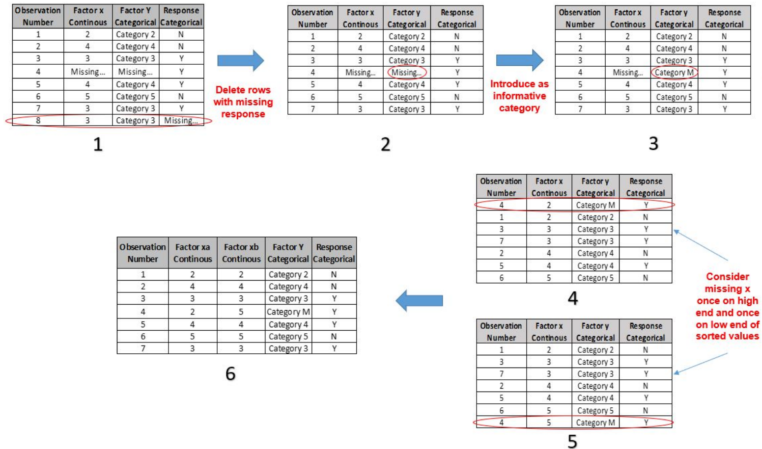
Figure 3.8: Example of Handling the Missing Data by ETAM
