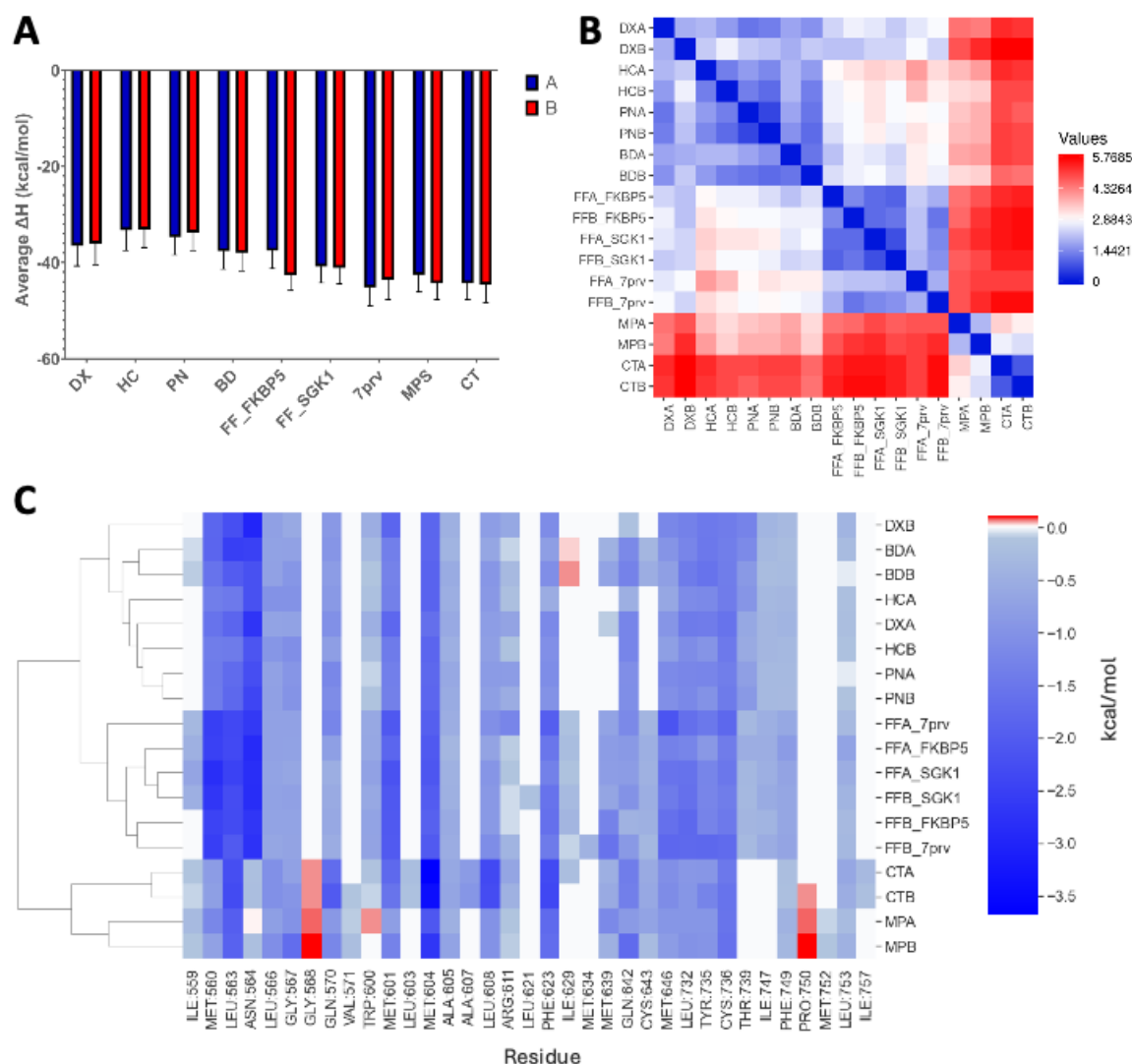
Figure 0.117 – MMPBSA analysis results. A) Average binding free energy of ligand-protein complex for both chain A and chain B. B) Pairwise heat map using Euclidean distance matrix to calculate similarities between ligands. C) Decomposition binding free energy values showing per-residue energy contribution for all amino acids. Scale: all values in kcal/mol, white color indicates no interaction between ligand and residue. Clustering analysis: Euclidean distance clustering method grouping ligands based on decomp raw values.
