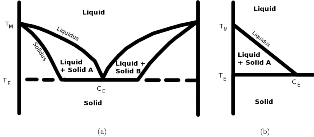
Figure 1.2: The full phase diagram for a binary system is given in (a), whereas the simplified phase diagram that will be used in our analyses is given in (b).
