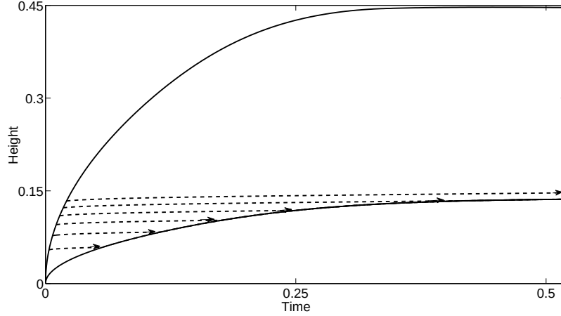
Figure 4.1: Characteristics terminate along a eutectic solid-mush interface. The solid curves are the solid-mush (lower) and mush-liquid (upper) interfaces, and the dashed curves are characteristics. The characteristics shown begin at evenly-spaced time intervals.
