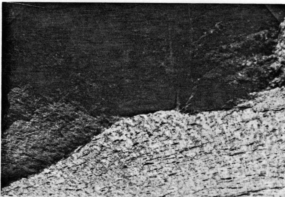
Figure 9. Fault surface within the Thunderhead Sandstone which displays stepped appearance due to fibrous mineral growth. Photo taken at locality 45 (Figure 1, page 2). The horizontal field of view is approximately 45 cm.
