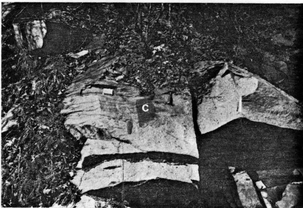
Figure 4. Photograph of Thunderhead Sandstone showing a mudrock clast (C) 70 cm in length. Photo taken at locality 54 (Figure 1, page 2). Fieldbook at upper left is approximately 20 cm in length.
