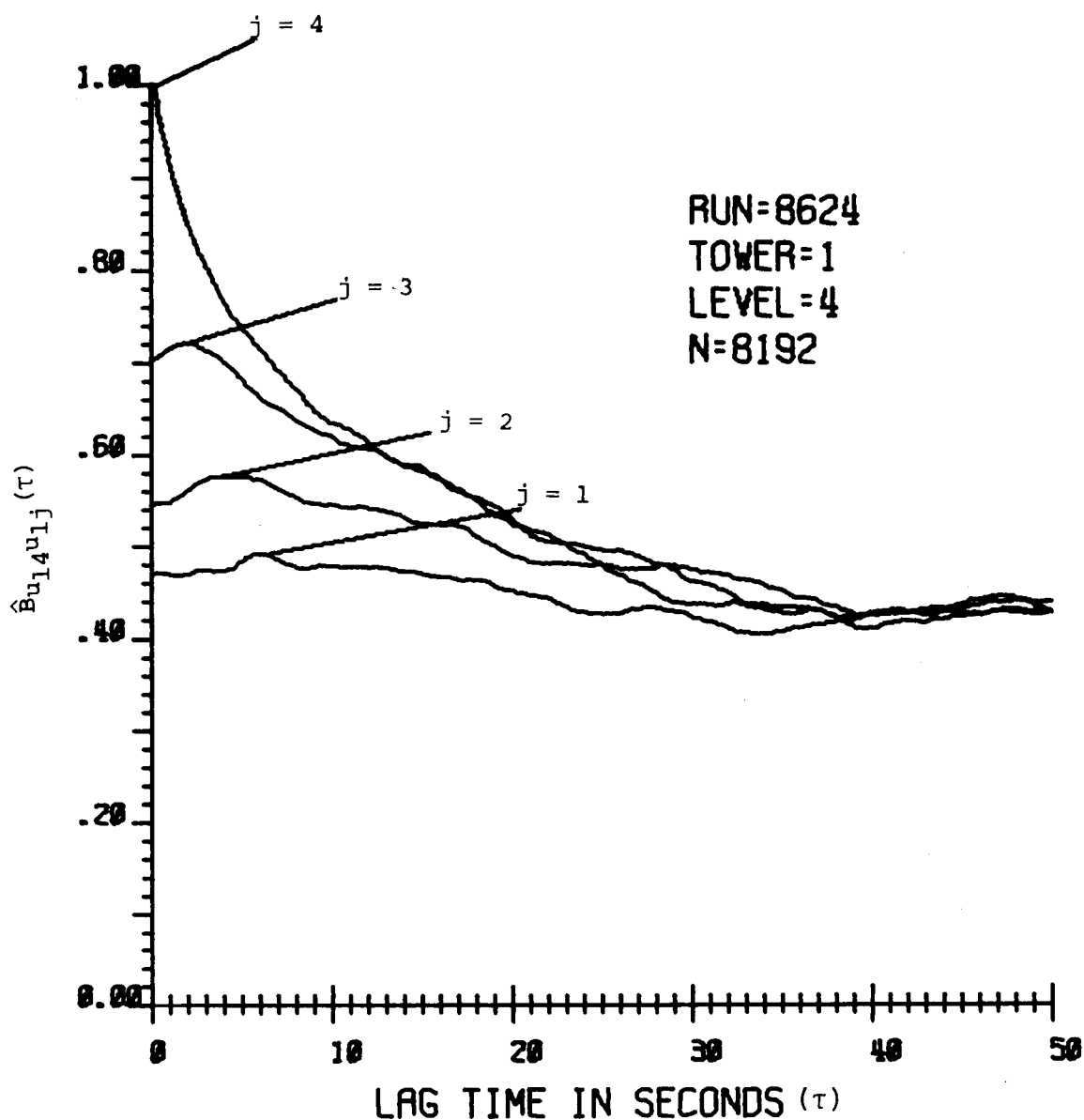
Figure 5-6 Vertical correlations relative to T1L4.
