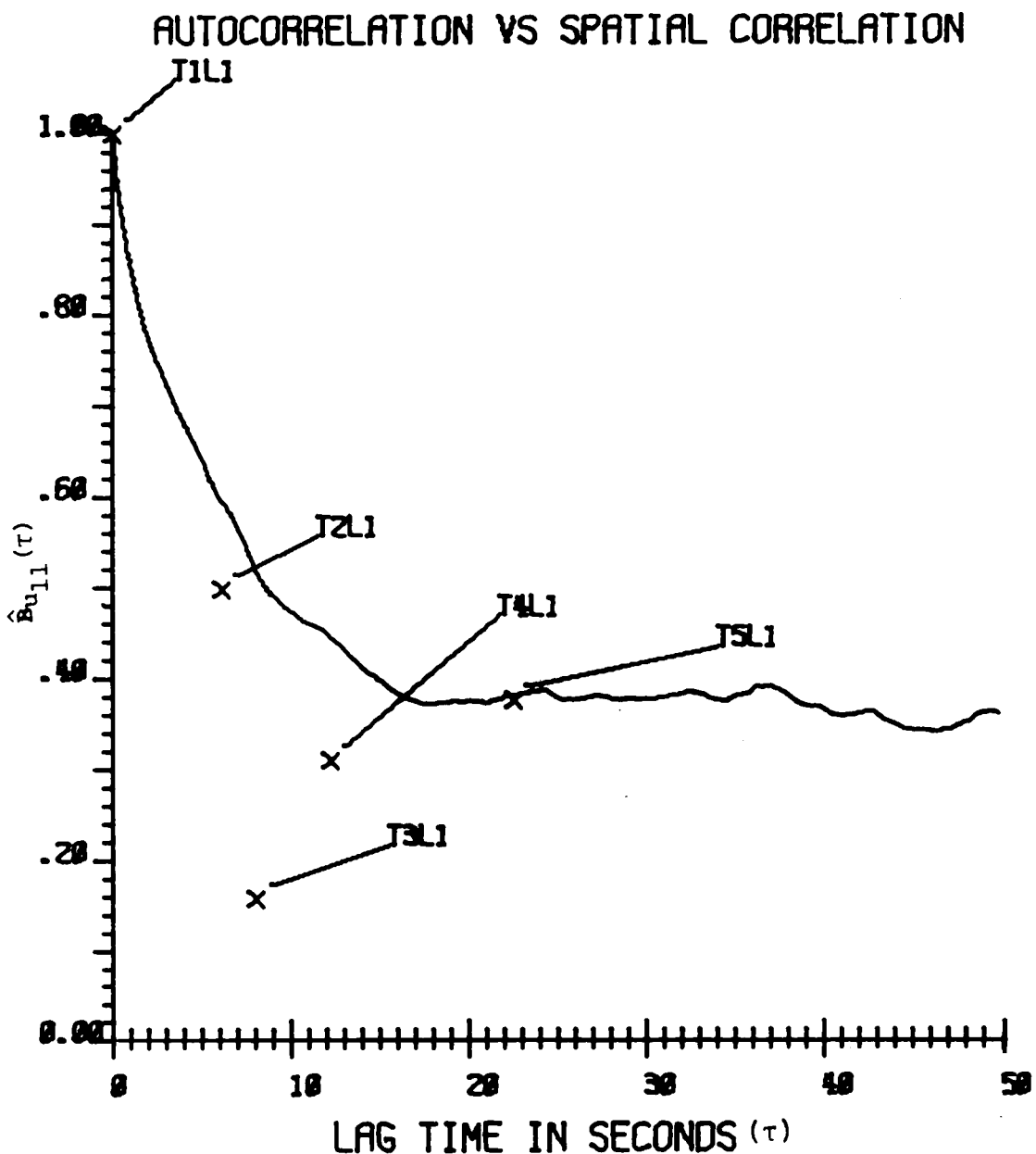
Figure 5-13 Comparison of autocorrelations computed by FFT procedures to autocorrelations computed by assuming Taylor's hypothesis.
