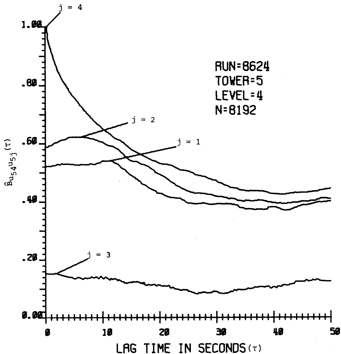
Figure 5-7 Vertical correlations relative to T5L4.
