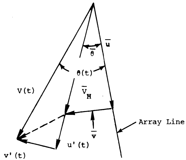
Figure 4-4 Definition of wind fluctuations u' and v' .
