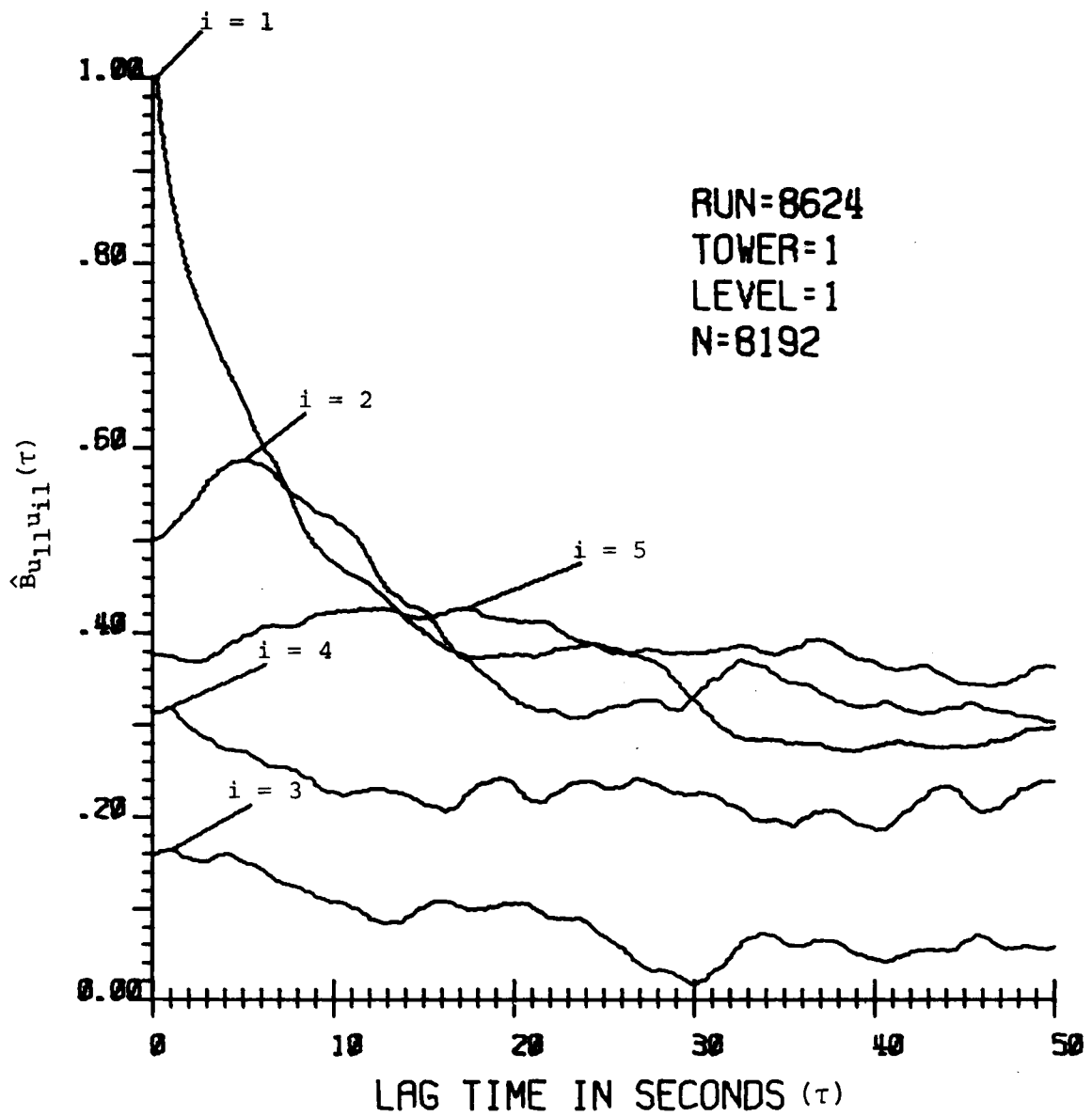
Figure 5-8 Horizontal correlations relative to T1L1.
