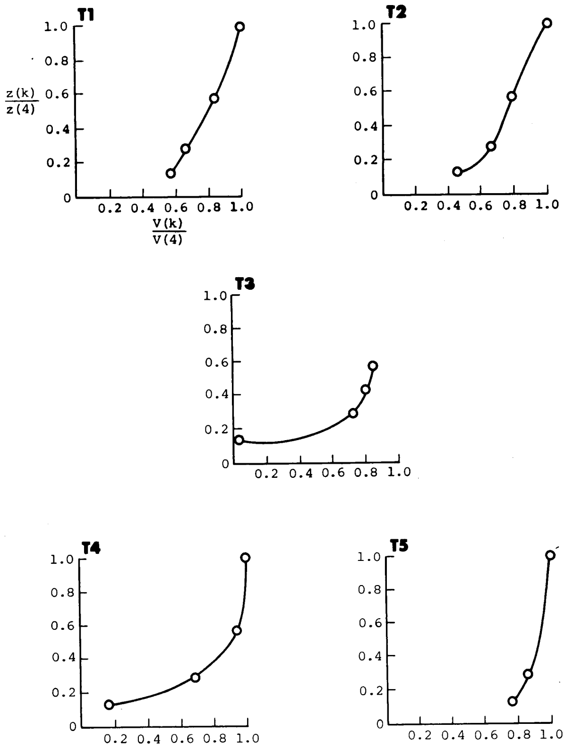
Figure 5-1 Mean non-dimensional velocities with the block building in the tower array, Run #8624.
