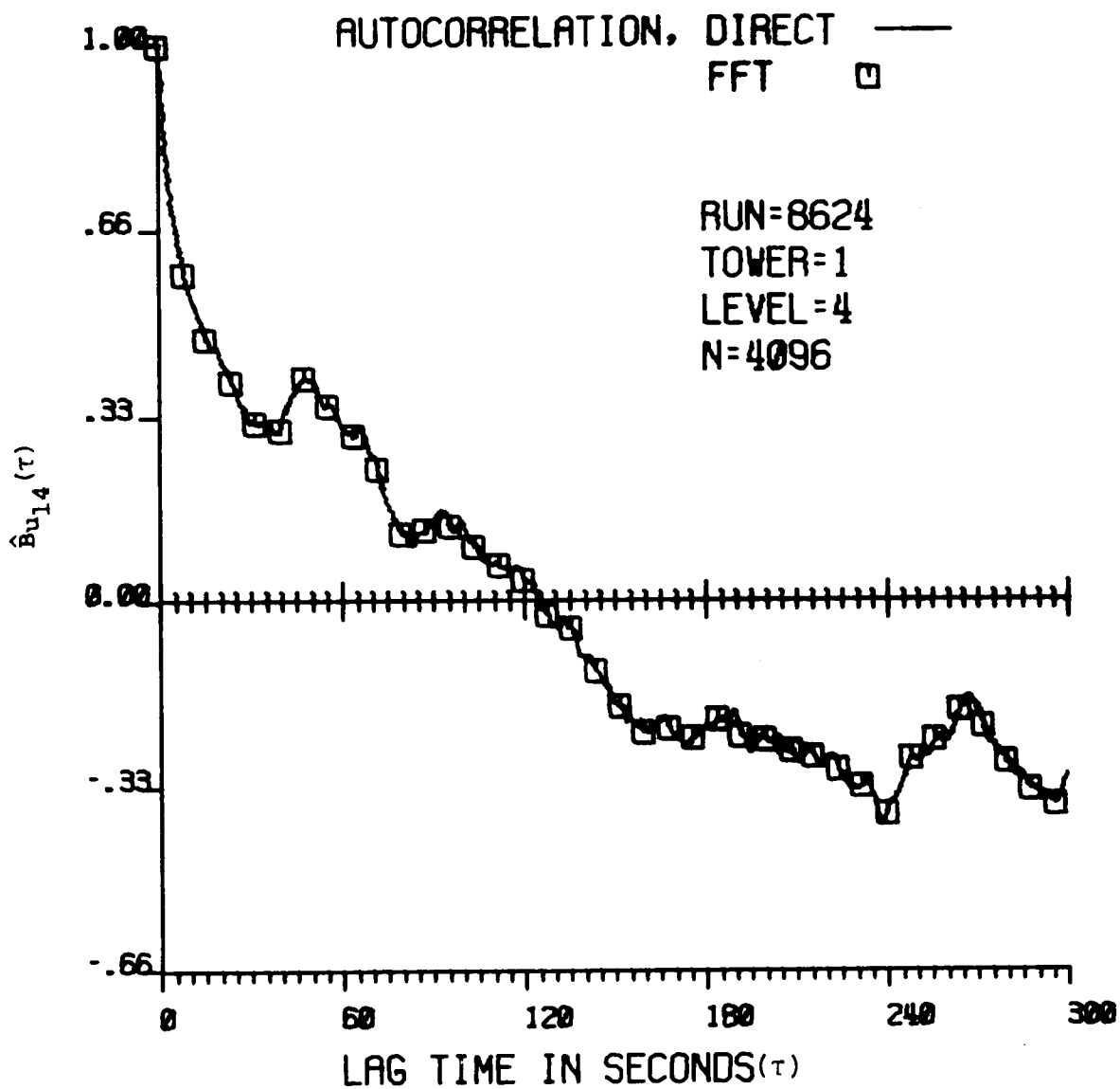
Figure 5-12 Comparison of direct and FFT methods for computing an autocorrelation function.
