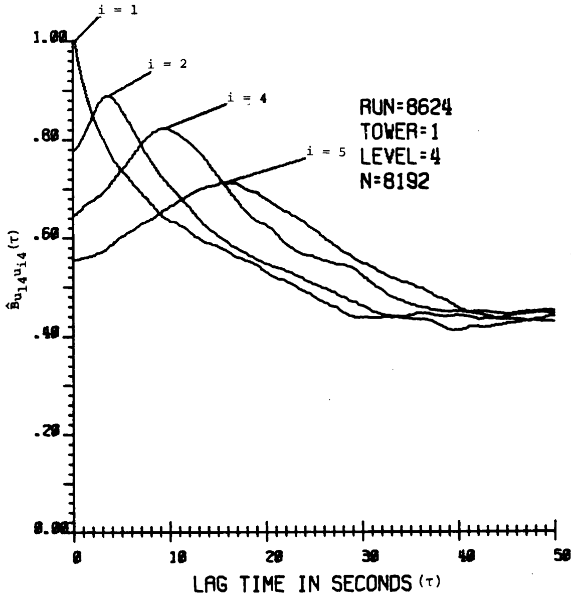
Figure 5-11 Horizontal correlations relative to T1L4.
