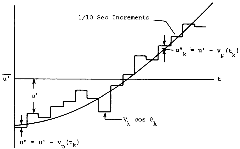
Figure 4-5 Illustration of trend removal.
