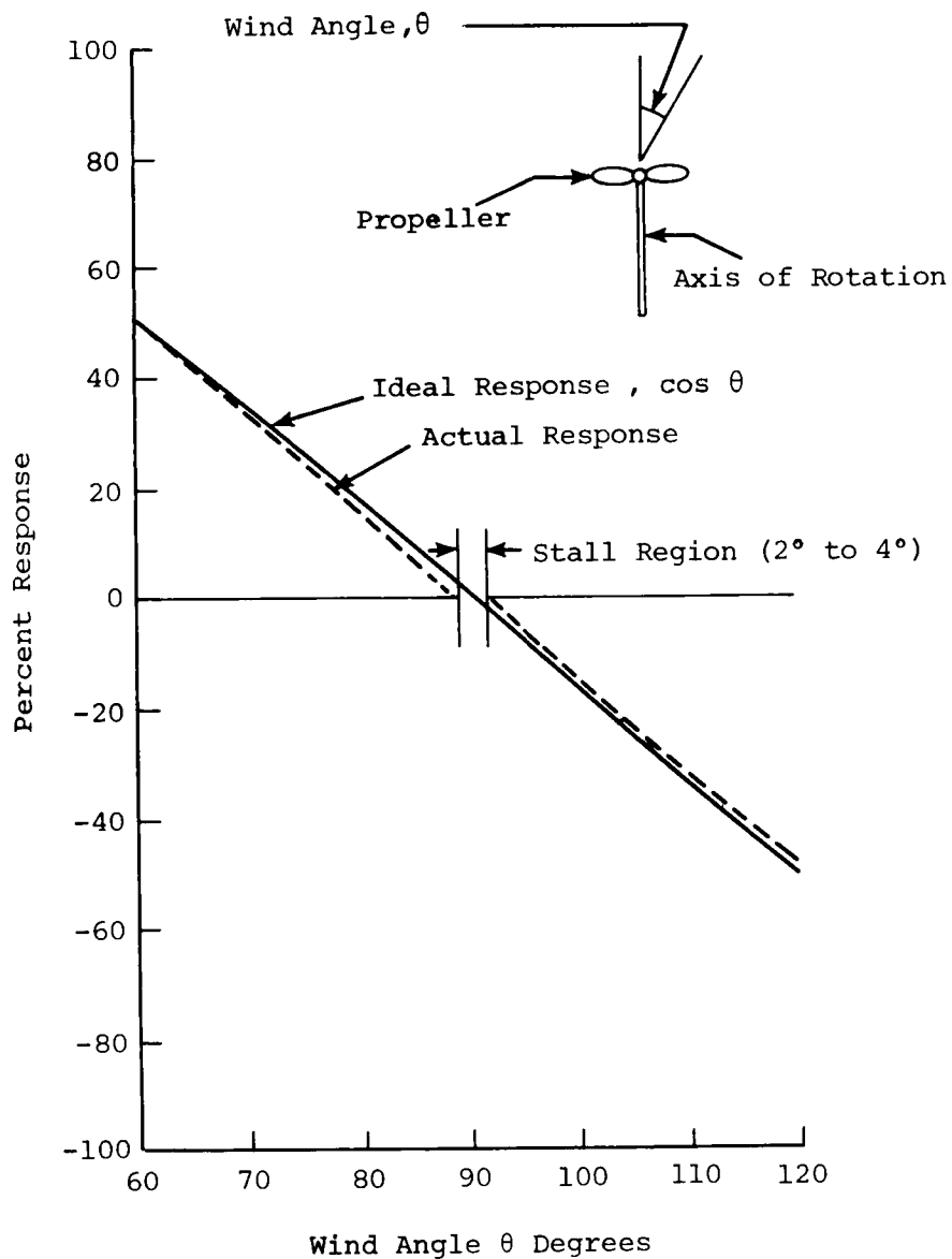
Figure 2-7 Propeller response versus wind angle between 60 and 120 degrees (four-blade polystyrene propeller) [2].
