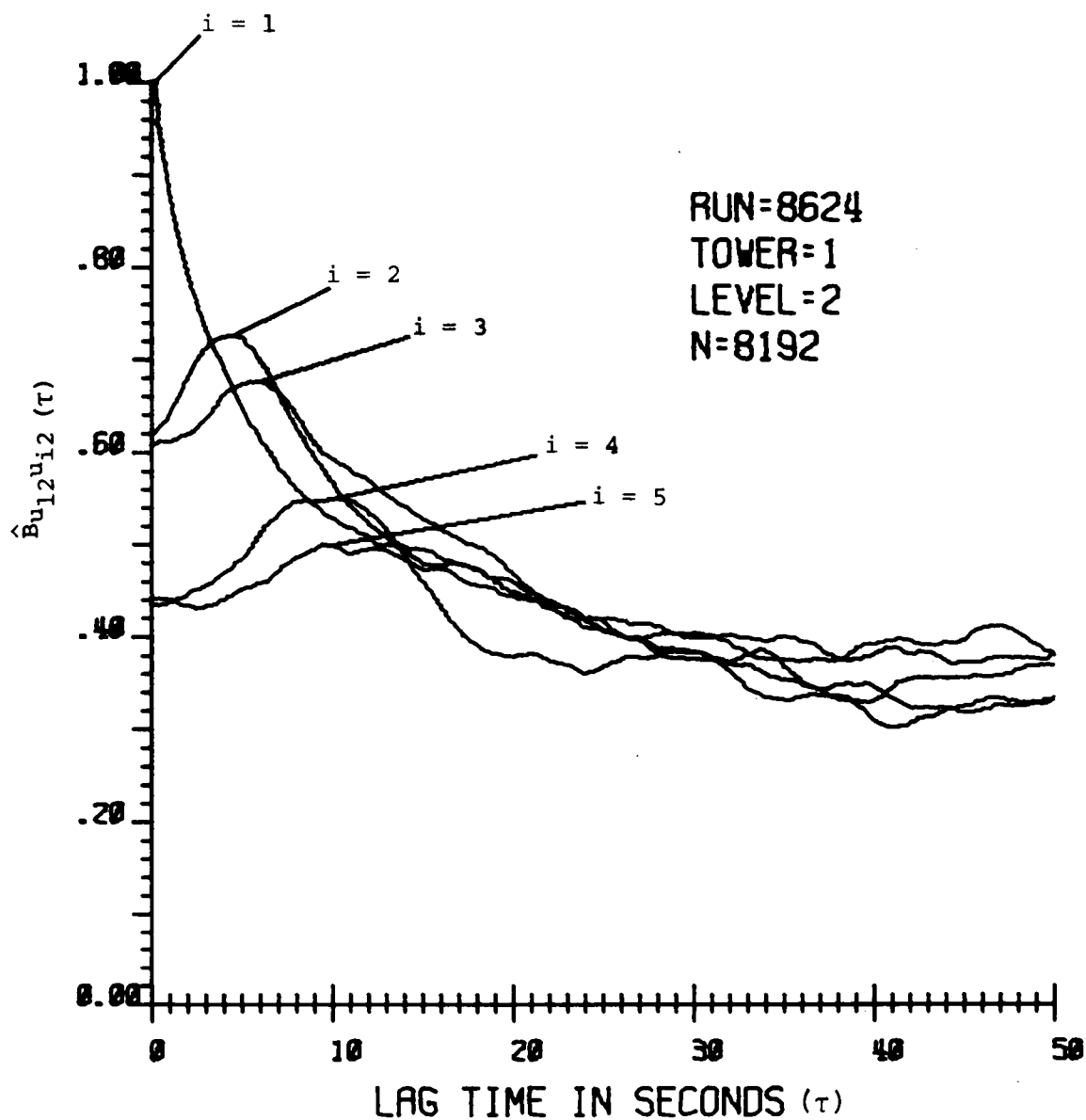
Figure 5-9 Horizontal correlations relative to T1L2.
