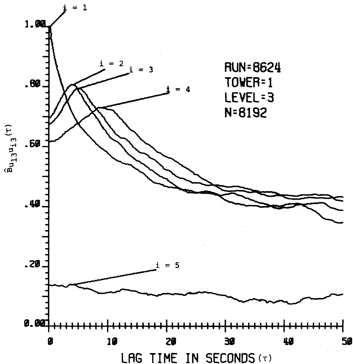
Figure 5-10 Horizontal correlations relative to T1L3.
