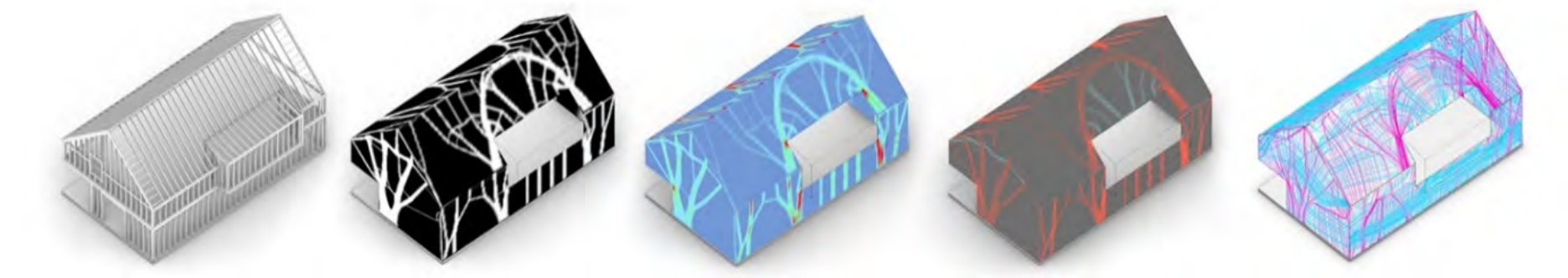
Model house comparing timber framing & 2D topology optimization (fig. 1)
