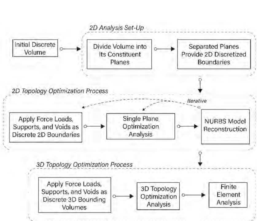
Workflow diagram for finding an optimized topology (fig. 8)
