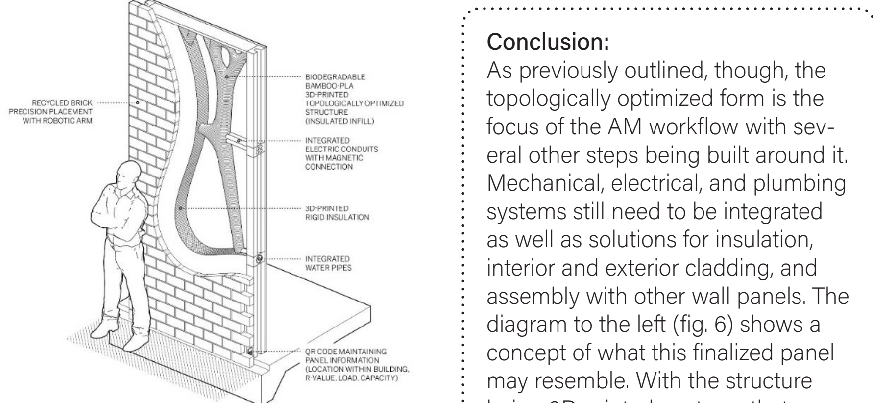
Concept sketch of a wall panel utilizing optimized structure (fig. 6)
