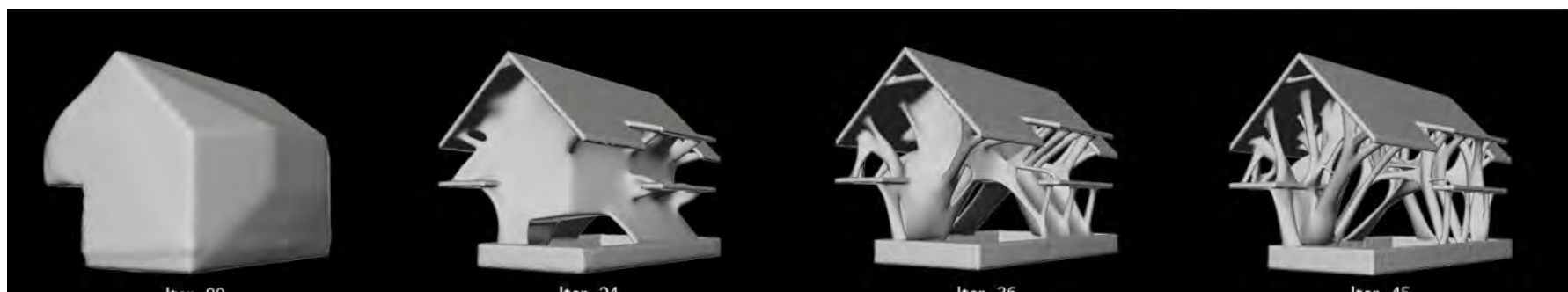
Results of model treated as one volume (3D topology optimization) (fig. 2)
