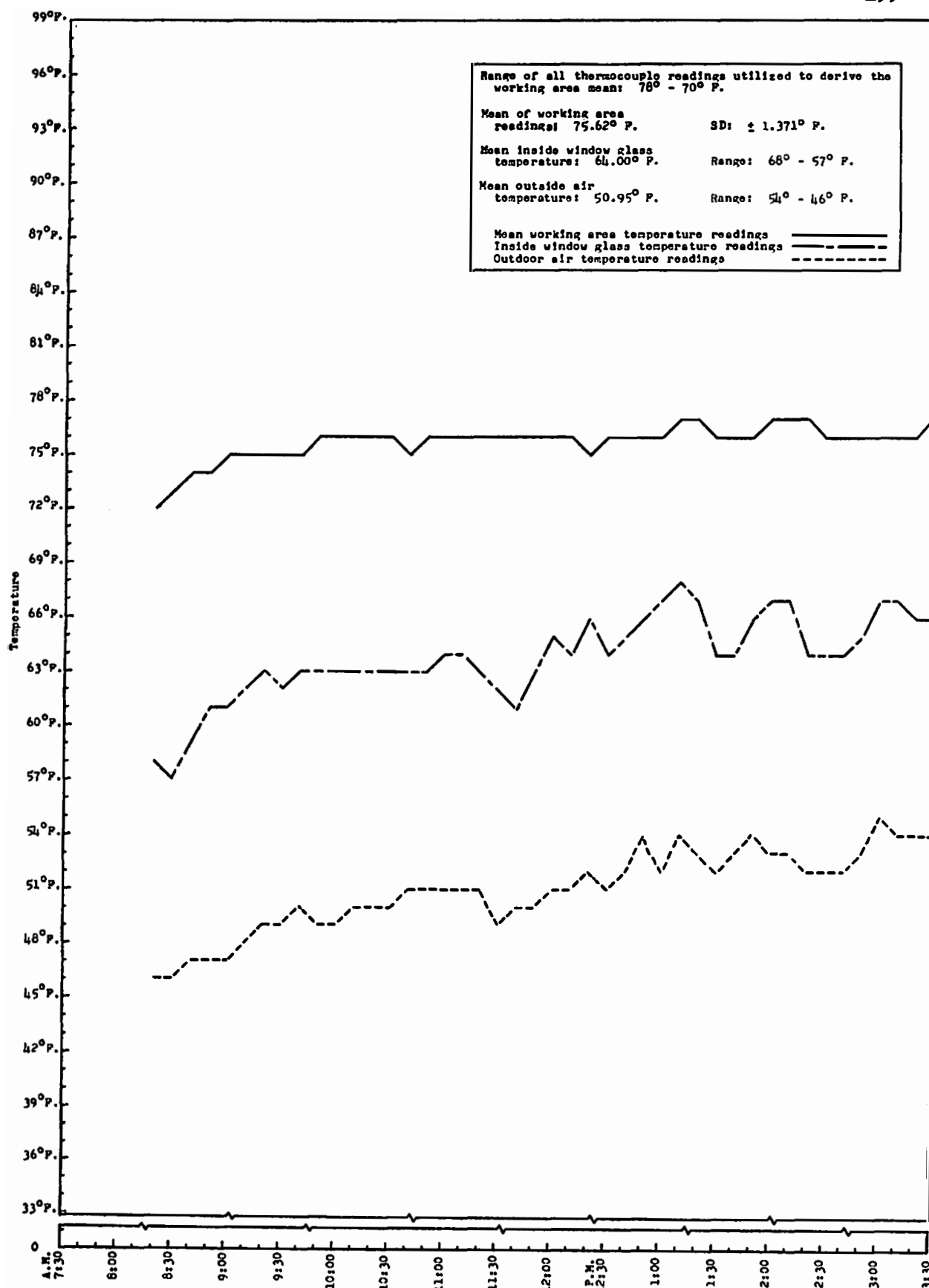
Figure 25. Comparison of thermocouple temperature readings of the classroom working area, inside window glass, and outside air for Classroom H-2.
