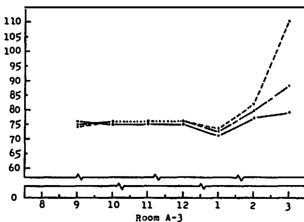
Figure 30. Comparison of air temperature, globe thermometer readings, and mean radiant temperature in classrooms in School A.
