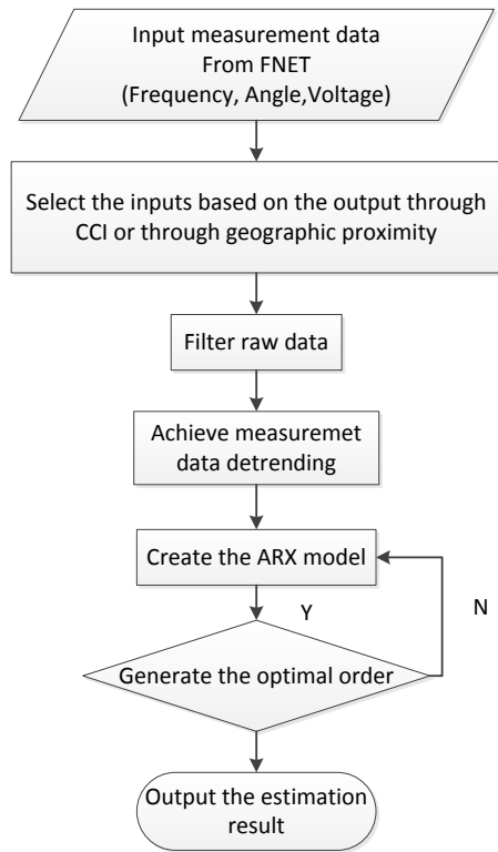
Figure 2–1 Flowchart of the system dynamic response estimation
