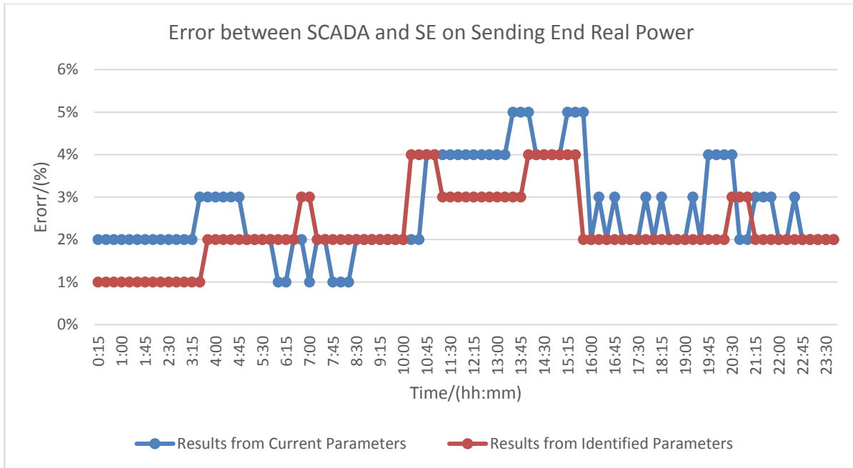
Figure 6–9 Comparison of real power of sending end on Mar. 12, 2016
