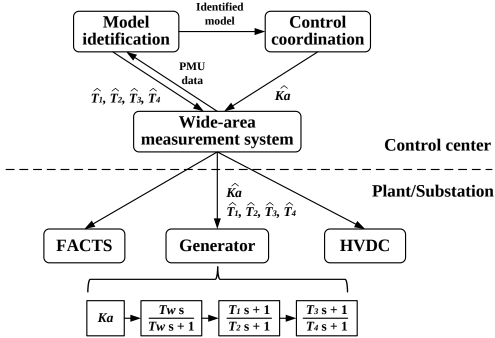
Figure 3–3 Architecture of the adaptive and coordinated oscillation damping control system
