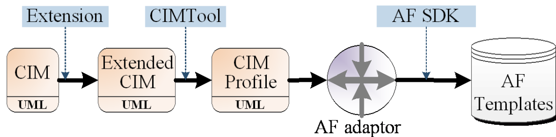
Figure 5–6 Flowchart of generating the AF templates based on CIM
