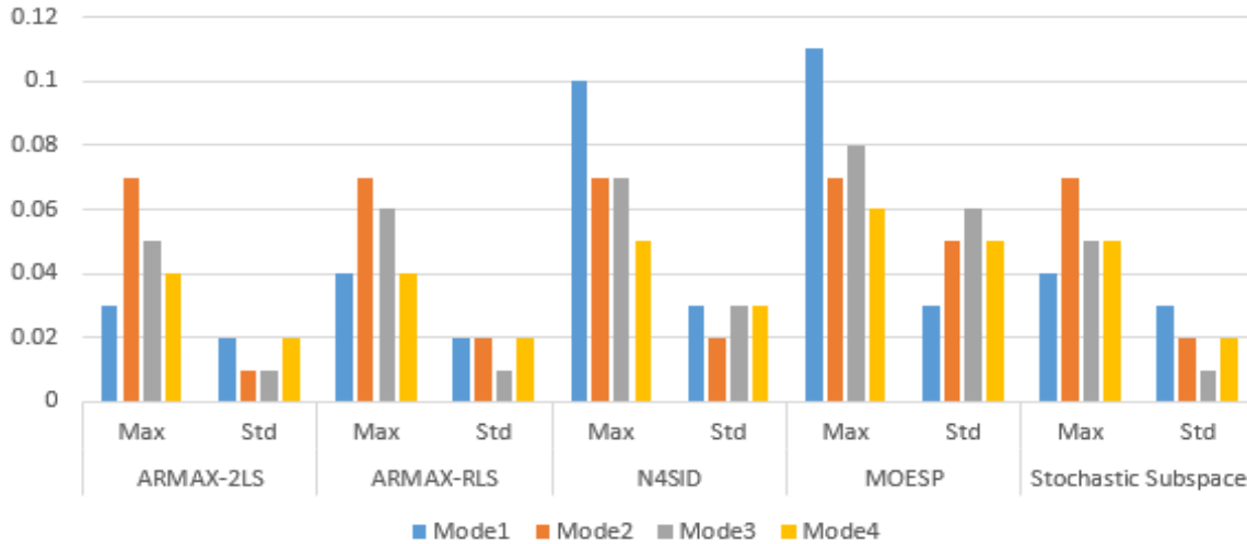
Figure 4–8 Accuracy comparison of image part of modes for five methods
