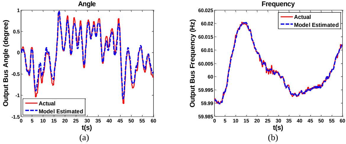
Figure 2-9 Comparison between the actual measurement and estimation in case 8
