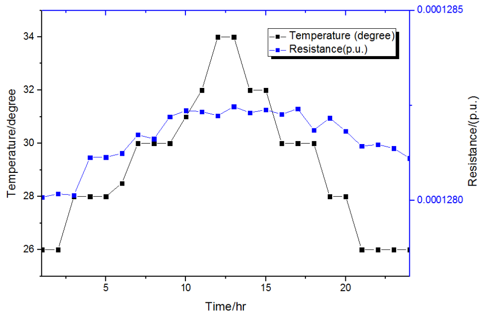
Figure 6–18 Impact of the temperature on resistance on Jan 19, 2016
