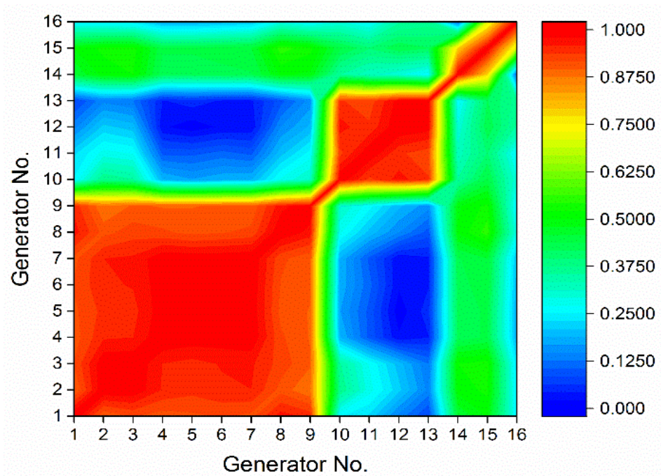
Figure 3–6 Coherency analysis based on CCI
