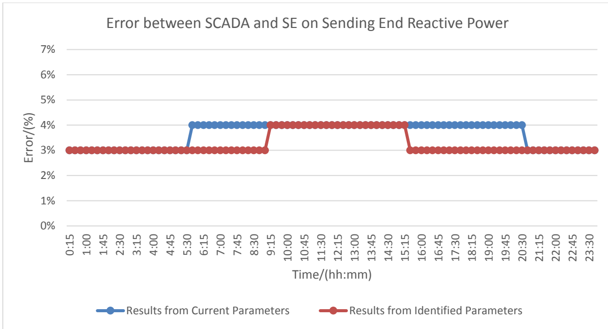
Figure 6–7 Comparison of reactive power of sending end on Jan. 19, 2016
