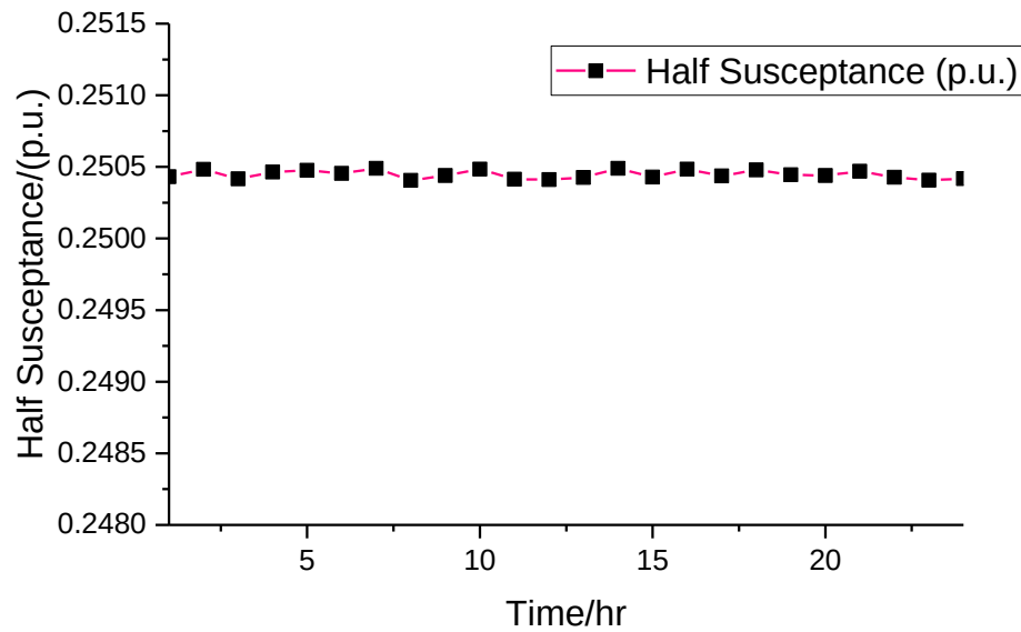
Figure 6–4 Identification results of the transmission-line susceptance within 24hrs
