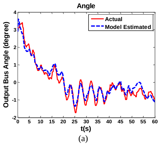
Figure 2-8 Comparison between the actual measurement and estimation in case 7
