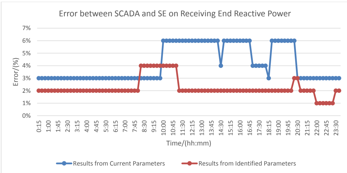
Figure 6–16 Comparison of reactive power of receiving end on May. 26, 2016
