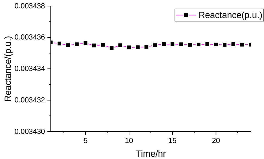
Figure 6-2 Identification results of the transmission-line reactance within 24hrs
