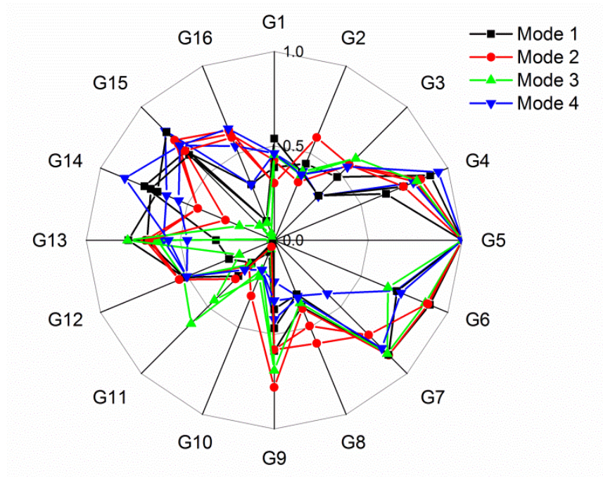
Figure 3-7 Observation signal selection results using FFT analysis of three tests
