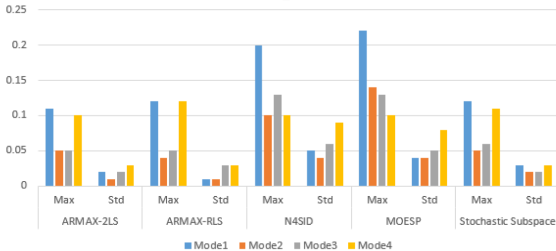
Figure 4–7 Accuracy comparison of real part of modes for five methods
