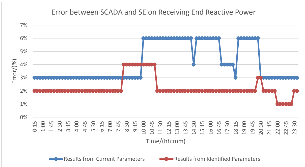
Figure 6–12 Comparison of reactive power of receiving end on Mar. 12, 2016
