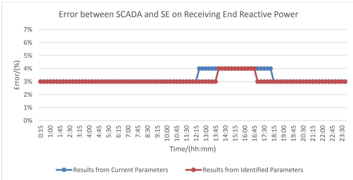
Figure 6–8 Comparison of reactive power of receiving end on Jan. 19, 2016
