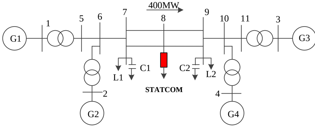
Figure 3–16 Two-area four-machine system
