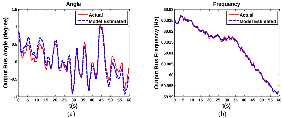
Figure 2-11 Comparison between the actual measurement and estimation in case 10
