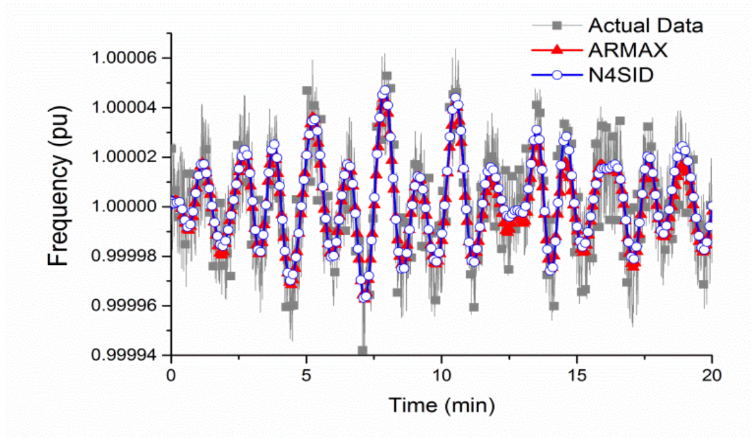
Figure 3-9 Comparison of bus frequency response at Bus 5
