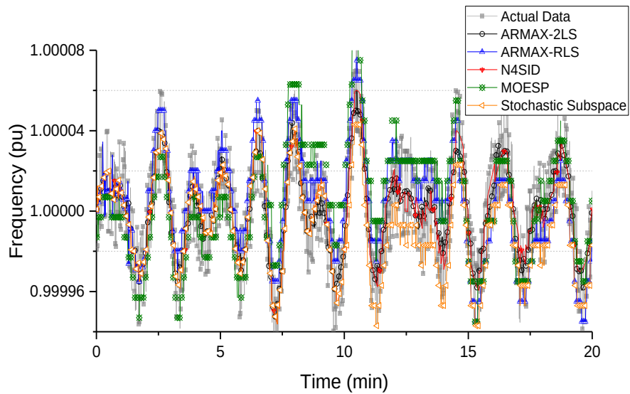
Figure 4–1 Identification results and comparison using ambient data
