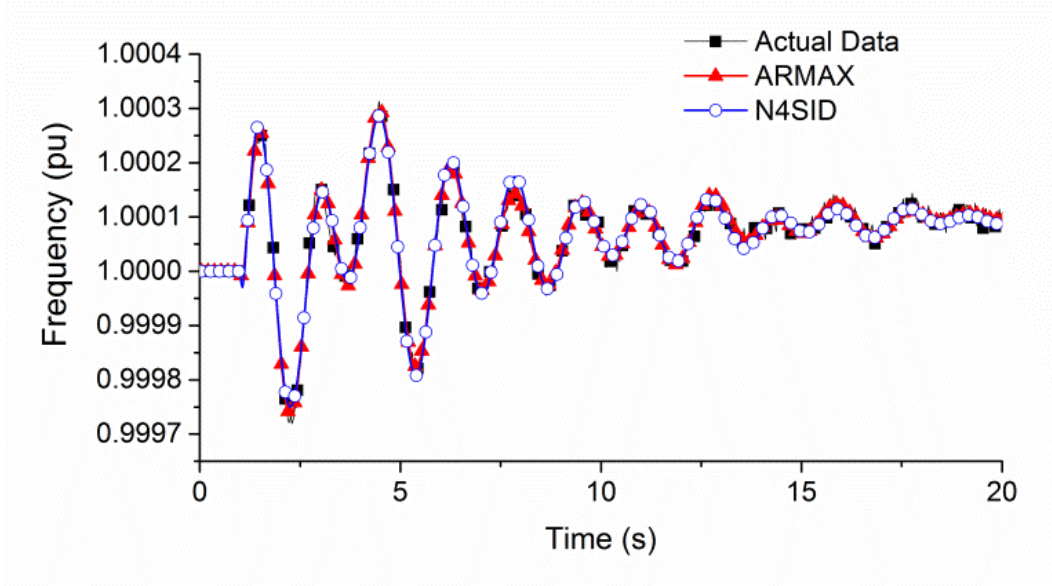
Figure 3–13 Comparison of bus frequency response at Bus 5
