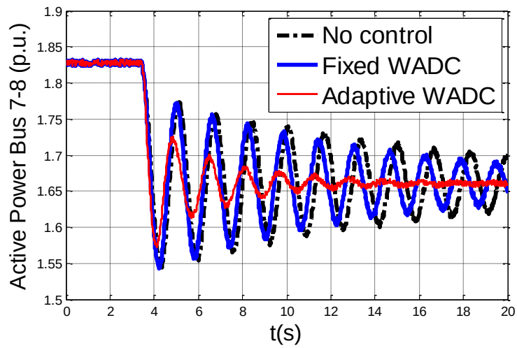
Figure 3–19 Control effect comparison of fixed WADC and adaptive WADC in scenario 2
