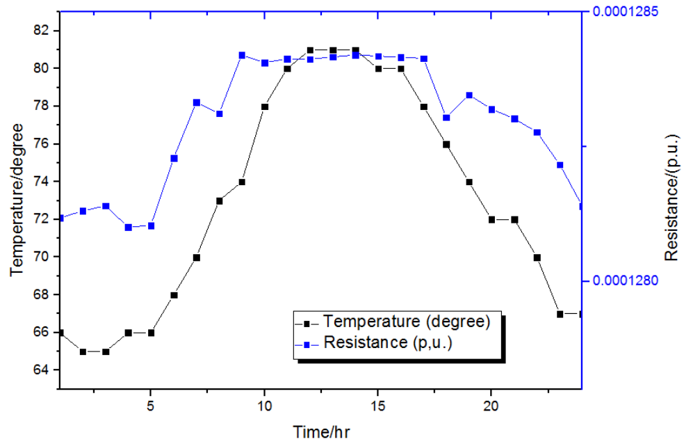
Figure 6–17 Impact of the temperature on resistance on May 26, 2016
