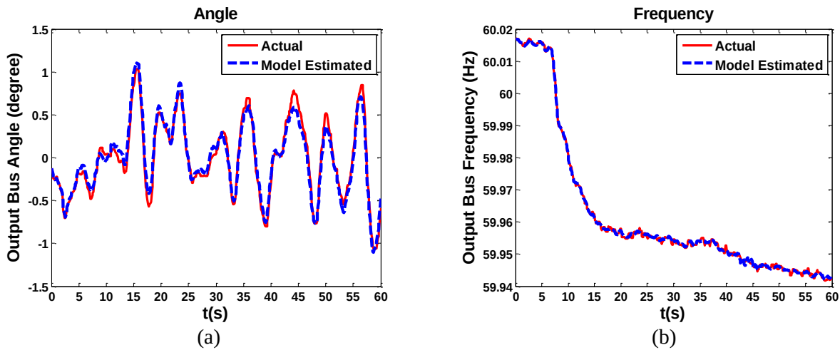
Figure 2–6 Comparison between the actual measurement and estimation in case 5
