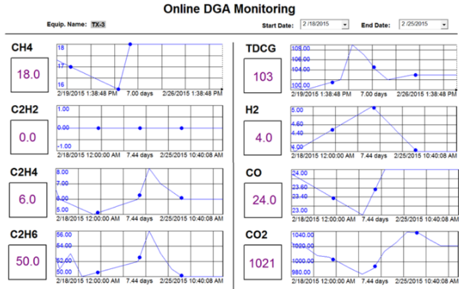
Figure 5–10 DGA visualization dashboard for transformer TX3
