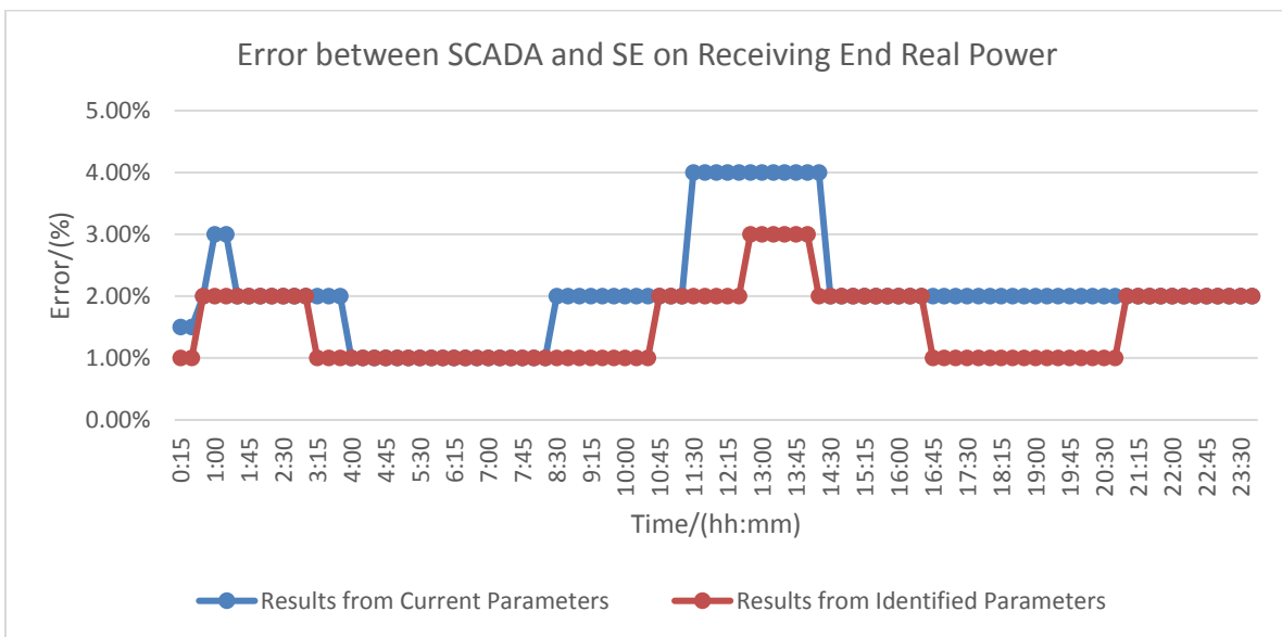
Figure 6–6 Comparison of real power of receiving end on Jan. 19, 2016
