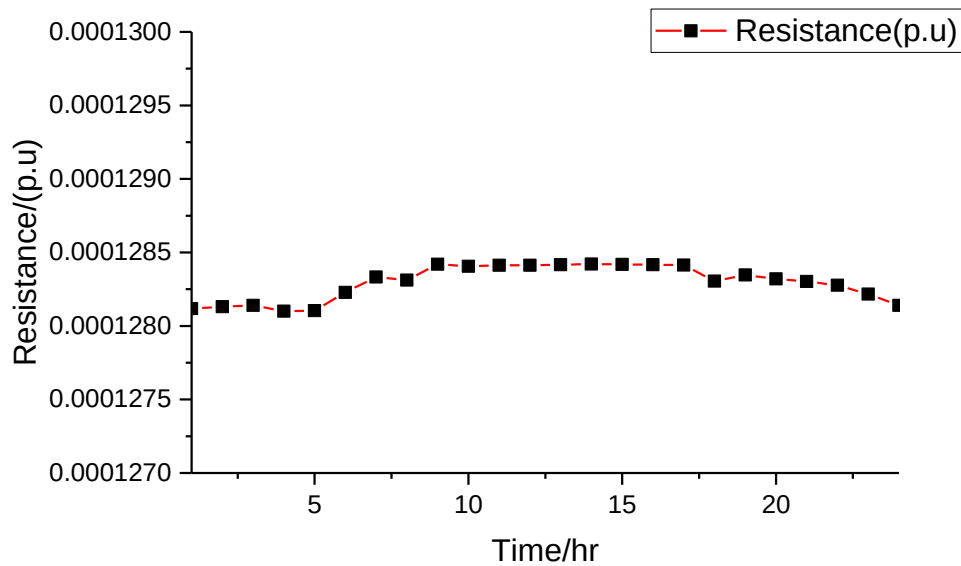
Figure 6-3 Identification results of the transmission-line resistance within 24hrs
