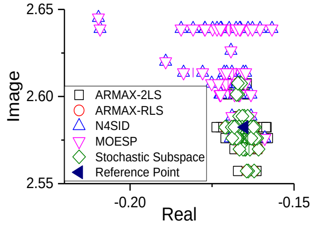
(b) Mode 2 (0.41Hz)
