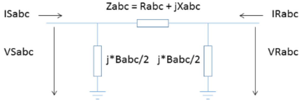
Figure 6–1 Transmission-line \pi model
