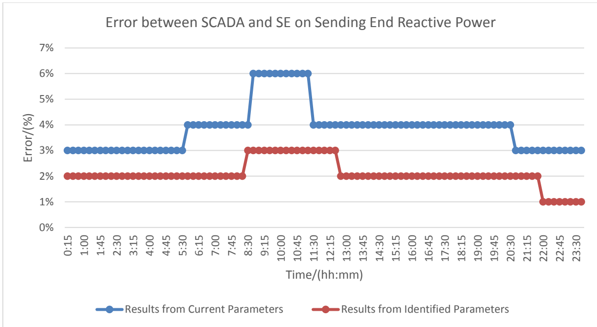
Figure 6–11 Comparison of reactive power of sending end on Mar. 12, 2016
