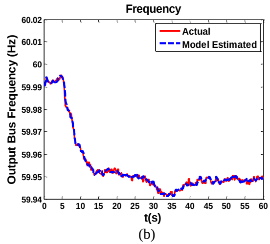
Figure 2-7 Comparison between the actual measurement and estimation in case 6
