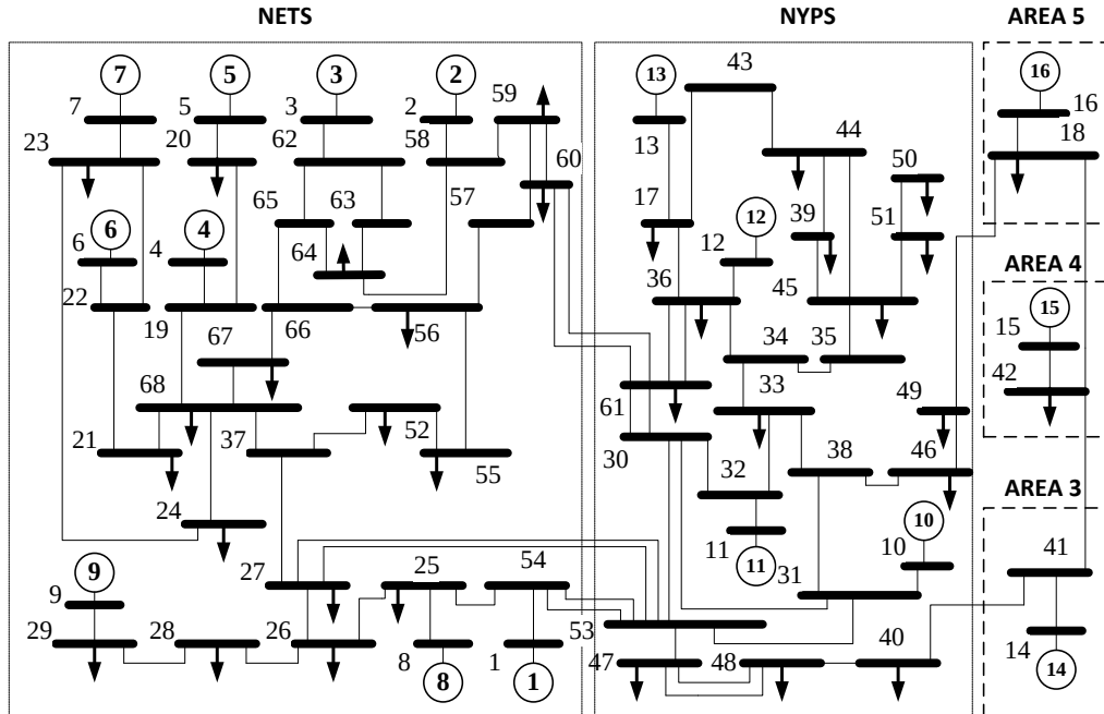
Figure 3–5 Single line diagram of the 16-machine 68-bus NPCC system
