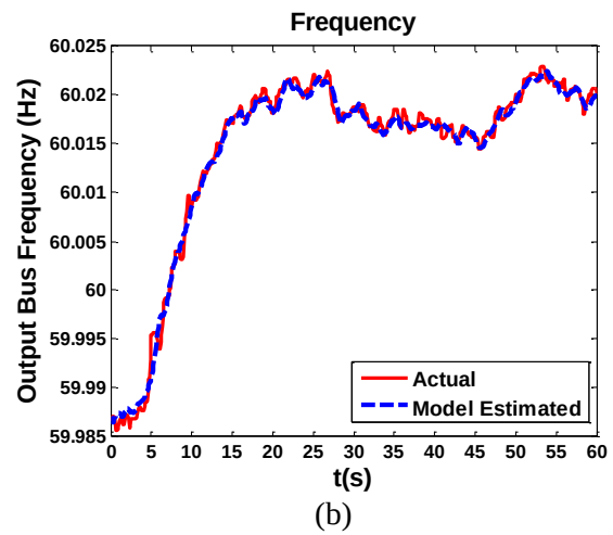
Figure 2-8 Comparison between the actual measurement and estimation in case 7
