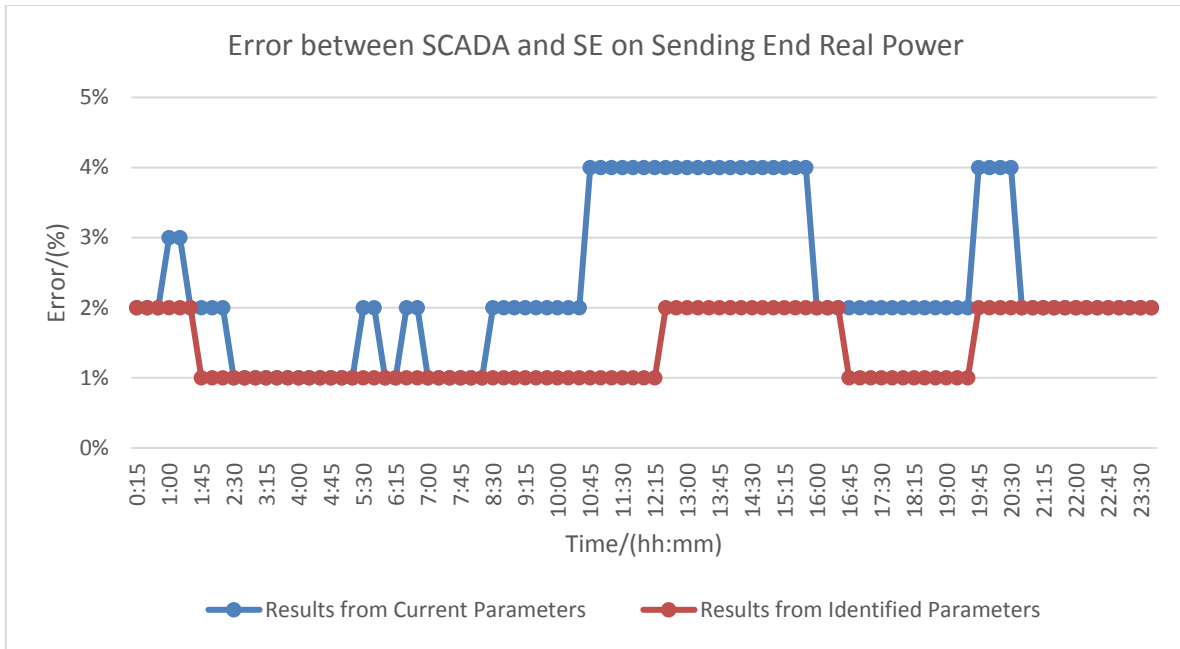
Figure 6–5 Comparison of real power of sending end on Jan. 19, 2016
