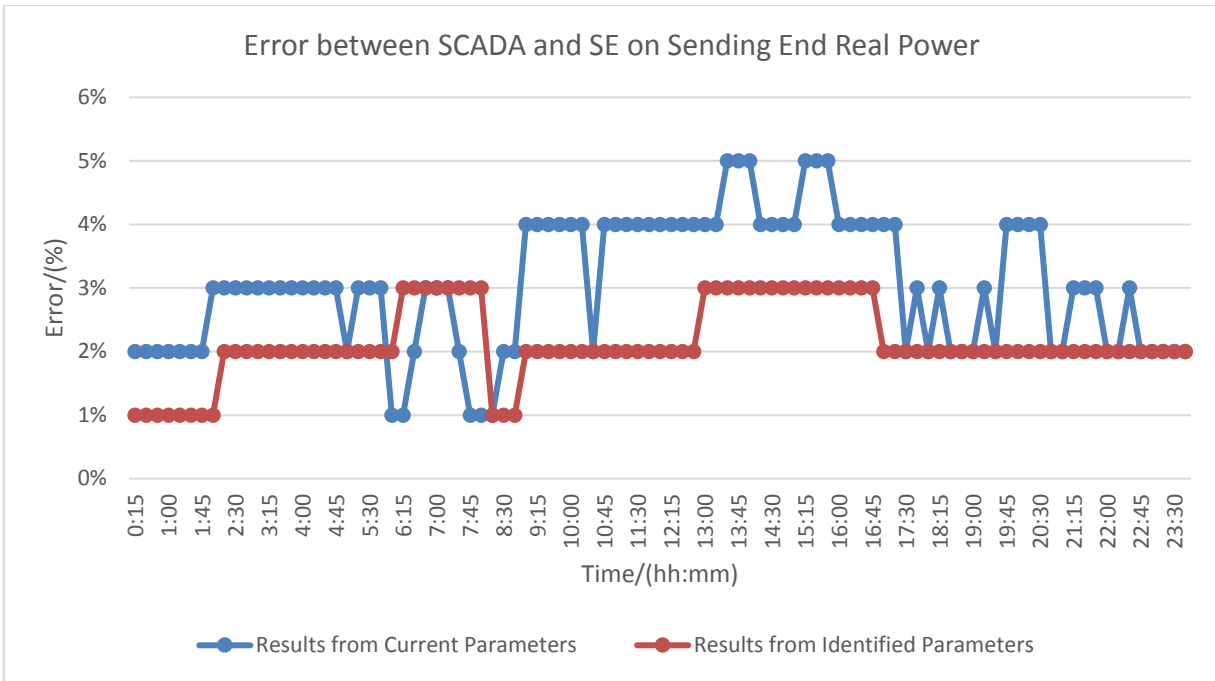
Figure 6–13 Comparison of real power of sending end on May. 26, 2016
