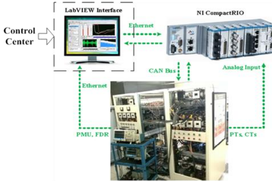
Figure 3–15 CURENT hardware testbed
