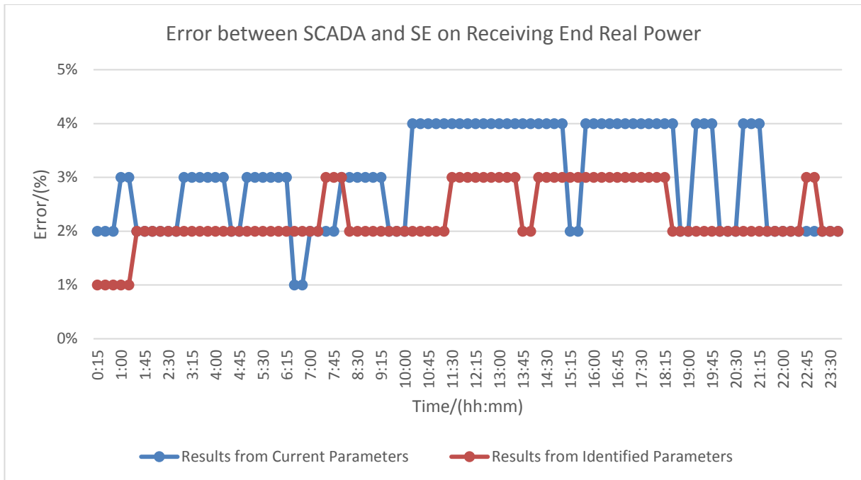
Figure 6–14 Comparison of real power of receiving end on May. 26, 2016
