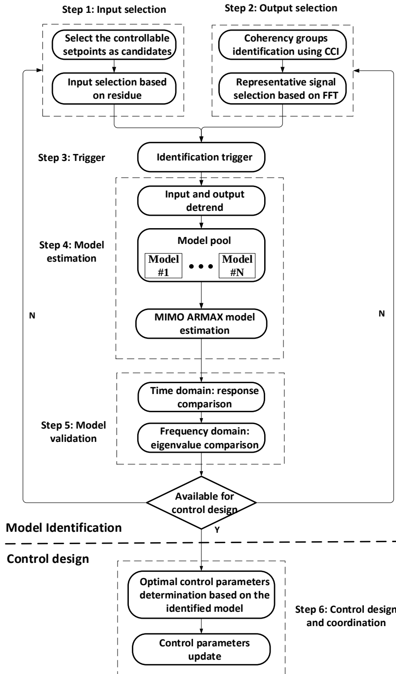
Figure 3–1 Flowchart of the proposed model identification methodology
