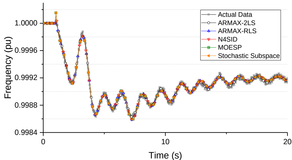
Figure 4–5 Identification results and comparison using ring-down data
