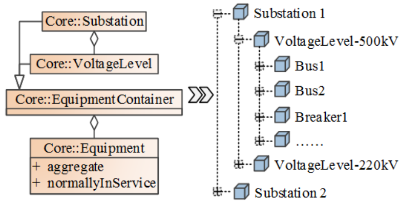
Figure 5–7 Aggregation between Equipment and EquipmentContainer
