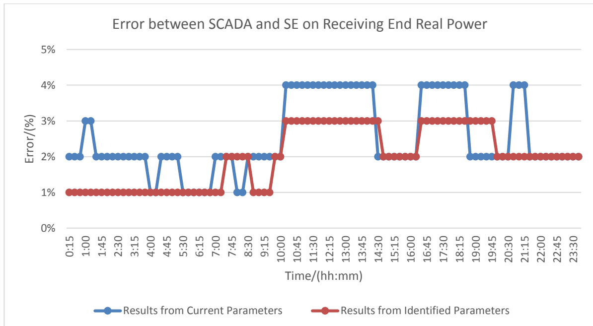
Figure 6–10 Comparison of real power of receiving end on Mar. 12, 2016
