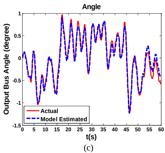
Figure 2–3 Comparison between the actual measurement and estimation in case 2
