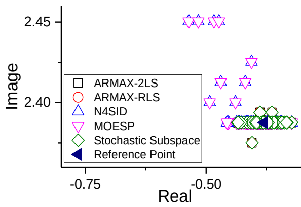
(a) Model 1 (0.38Hz)
