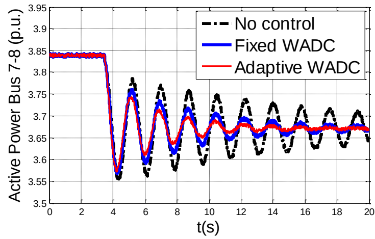
Figure 3–18 Control effect comparison of fixed WADC and adaptive WADC in scenario 1
