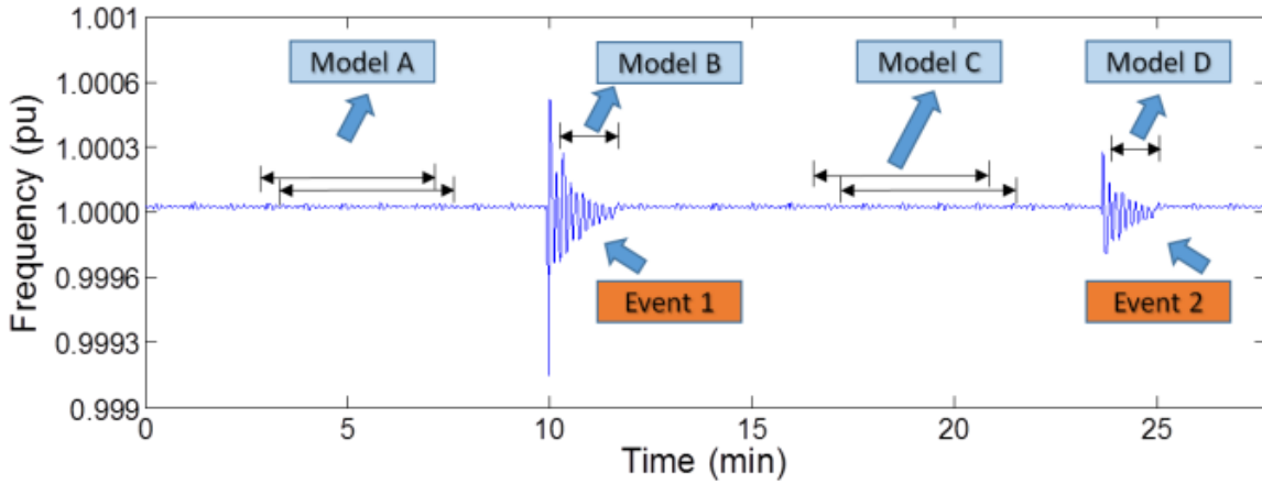
Figure 3–4 Time sequence of the adaptive approach
