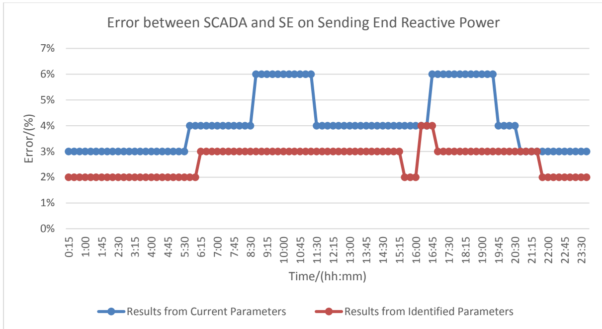
Figure 6–15 Comparison of reactive power of sending end on May. 26, 2016
