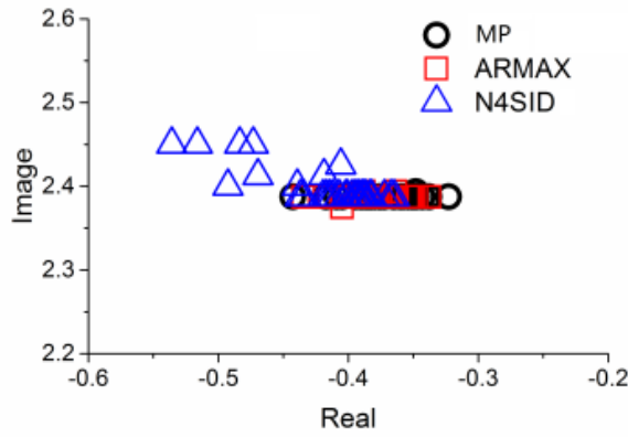
(a) Model 1(0.38Hz)
