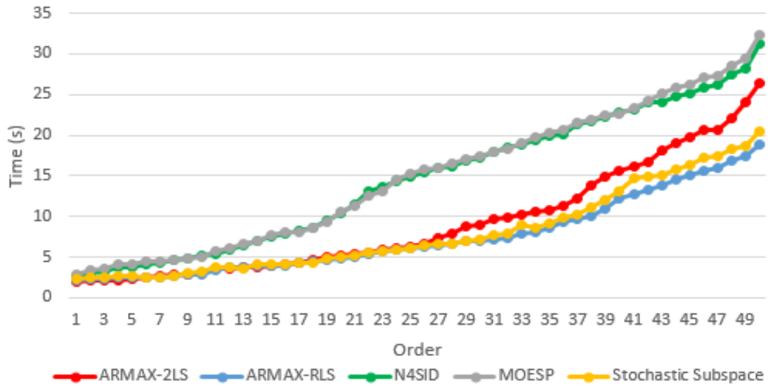
Figure 4–9 Computation time of five methods
