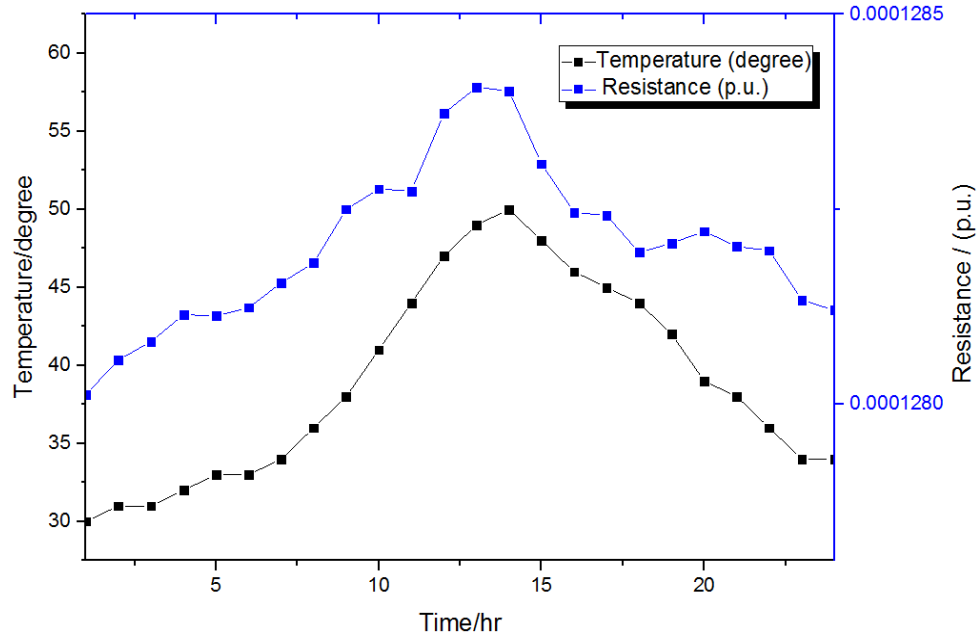
Figure 6–19 Impact of the temperature on resistance on Mar 12, 2016
