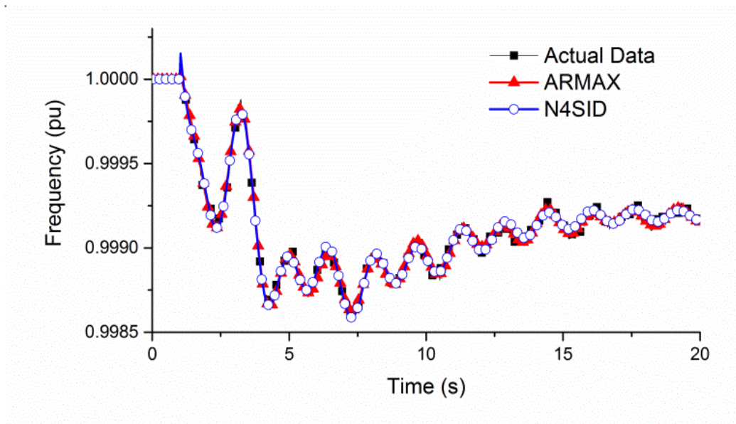
Figure 3–12 Comparison of bus frequency response at Bus 5
