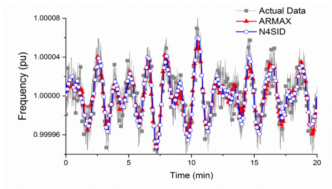
Figure 3-10 Comparison of bus frequency response at Bus 5
