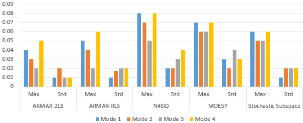
Figure 4–3 Accuracy comparison of real part of modes for five methods
