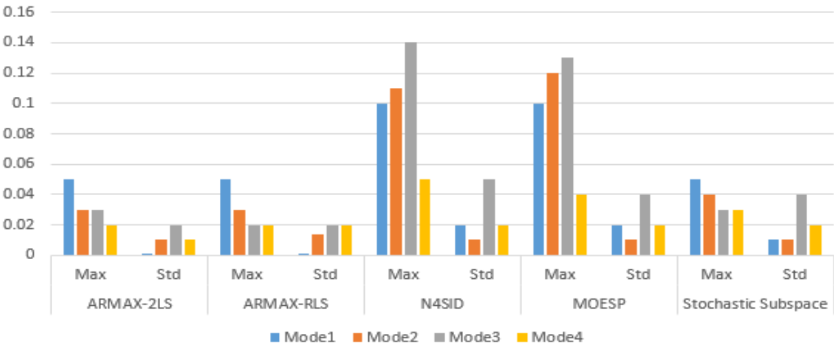
Figure 4–4 Accuracy comparison of image part of modes for five methods
