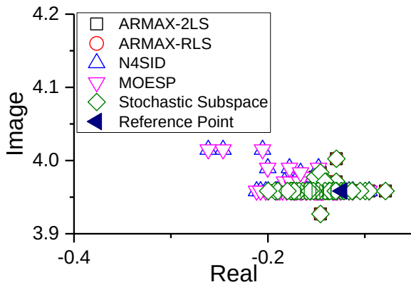
(c) Mode 3 (0.63Hz)
