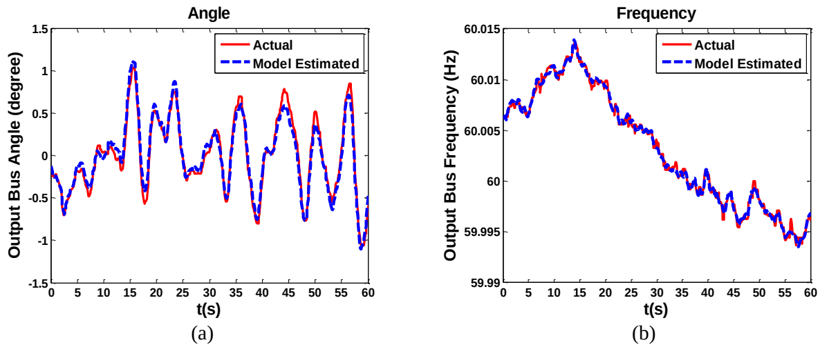
Figure 2–10 Comparison between the actual measurement and estimation in case 9
