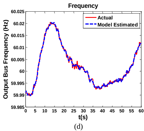
Figure 2–3 Comparison between the actual measurement and estimation in case 2
