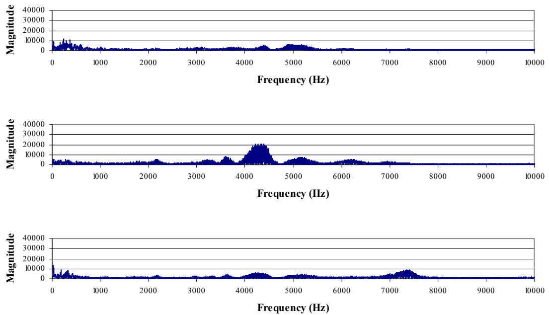
Figure A-177. FFT data from the greater trochanter accelerometer for a metal-on-metal THA, subjected to a 1900 Newton impact load. The signals are for the D1-axis (upper), D2-axis (middle) and D3-axis (lower).
