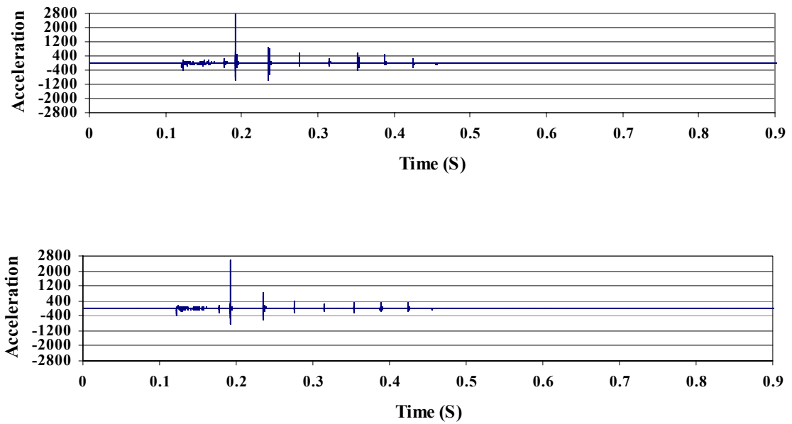
Figure 36. Comparison of Acceleration Signal Without Filtering (top) and with Filtering (bottom)
