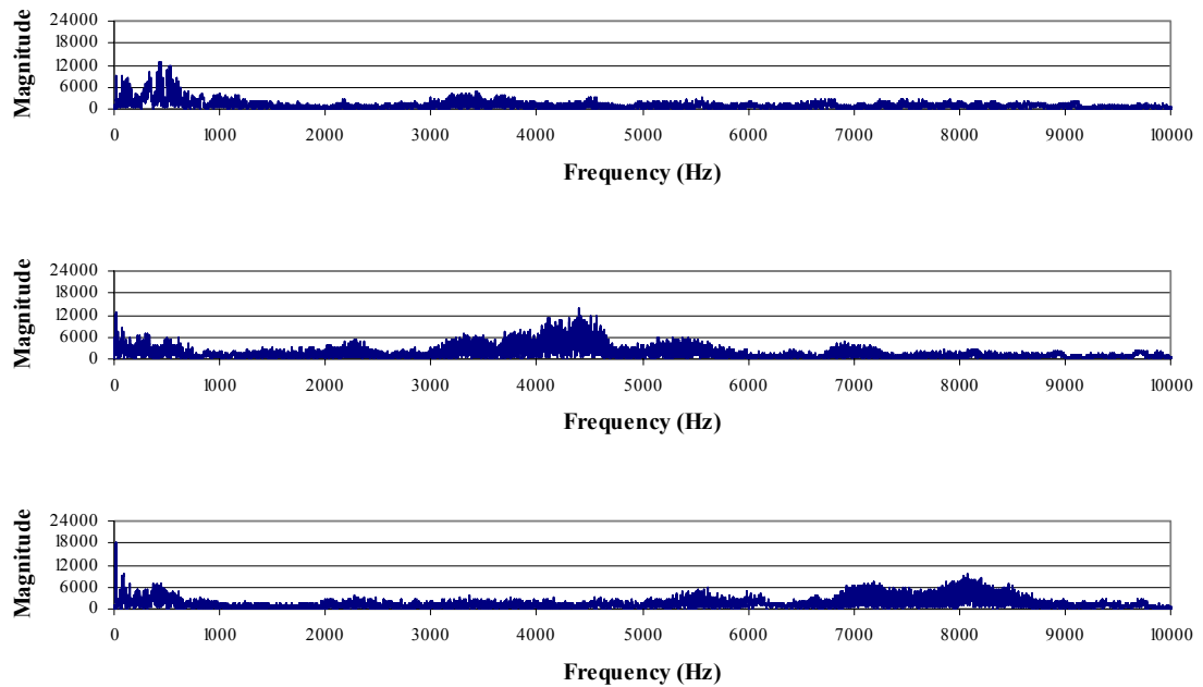
Figure A-157. FFT data from the greater trochanter accelerometer for a ceramic-on-ceramic THA, subjected to a 1500 Newton impact load. The signals are for the D1-axis (upper), D2-axis (middle) and D3-axis (lower).
