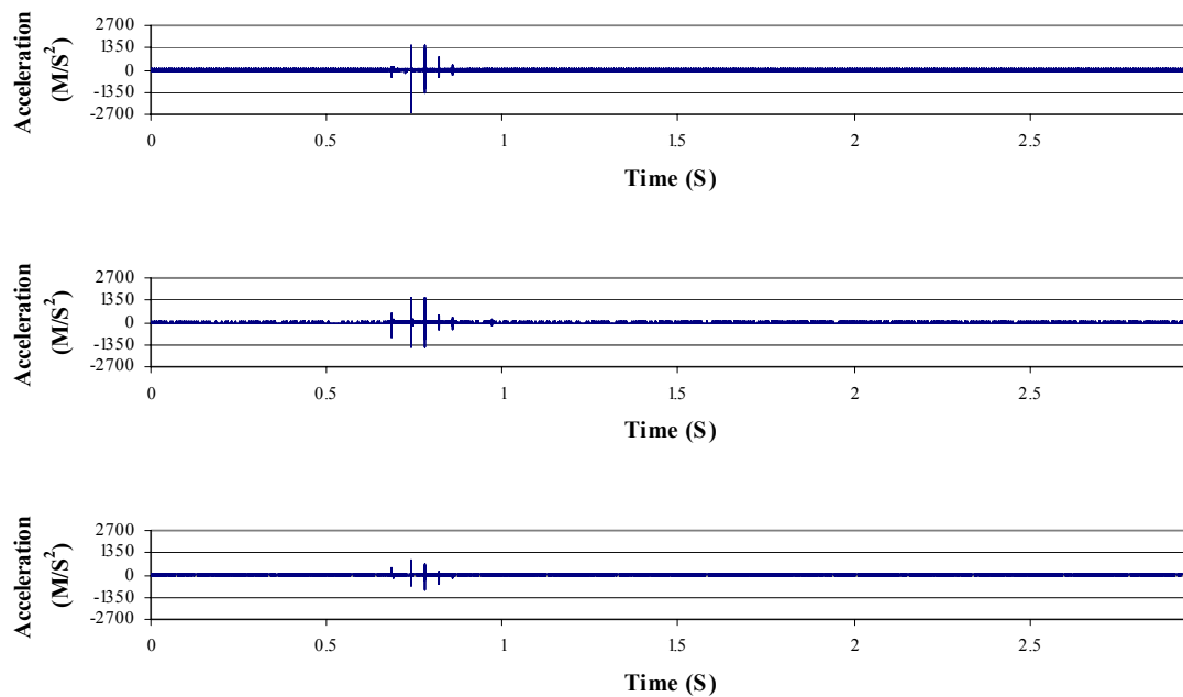
Figure A-79. Acceleration data from the acetabular cup accelerometer for a metal-on-metal THA, subjected to a 1500 Newton impact load. The signals are for the B1-axis (upper), B2-axis (middle) and B3-axis (lower).
