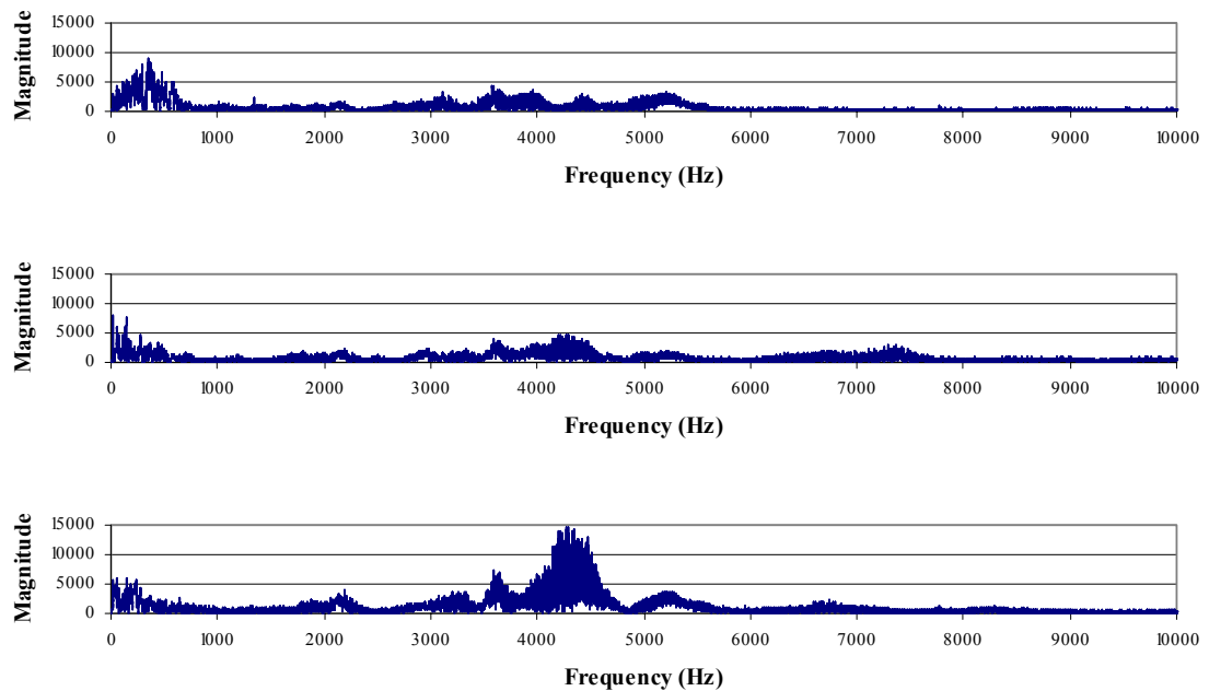
Figure A-141. FFT data from the greater trochanter accelerometer for a metal-on-metal THA, subjected to a 1280 Newton impact load. The signals are for the D1-axis (upper), D2-axis (middle) and D3-axis (lower).
