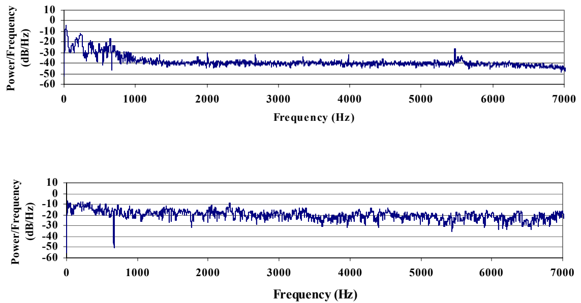
Figure 44. Comparison of PSD Signals for MOP at Minimum Test Load (top) and Maximum Test Load (lower).
