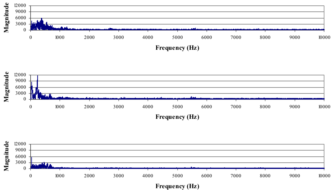
Figure A-137. FFT data from the greater trochanter accelerometer for a metal-on-polyethylene THA, subjected to a 1280 Newton impact load. The signals are for the D1-axis (upper), D2-axis (middle) and D3-axis (lower).
