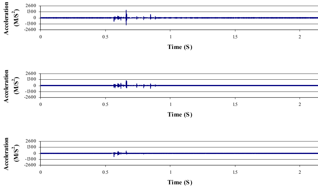
Figure A-100. Acceleration data from the femoral stem accelerometer for a metal-on-polyethylene THA, subjected to a 1900 Newton impact load. The signals are for the C1-axis (upper), C2-axis (middle) and C3-axis (lower).
