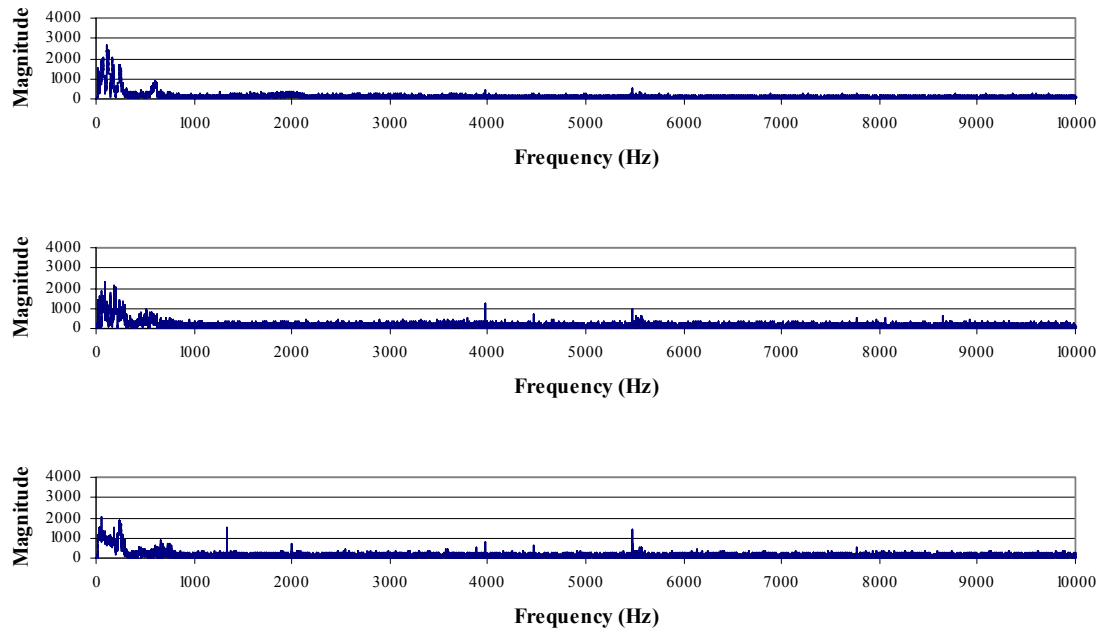
Figure A-116. FFT data from the femoral stem accelerometer for a metal-on-metal THA, subjected to a 680 Newton impact load. The signals are for the C1-axis (upper), C2-axis (middle) and C3-axis (lower).
