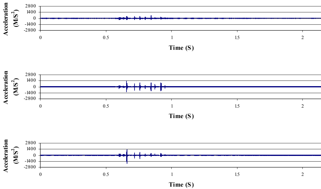
Figure A-109. Acceleration data from the greater trochanter accelerometer for a ceramic-on-ceramic THA, subjected to a 1900 Newton impact load. The signals are for the D1-axis (upper), D2-axis (middle) and D3-axis (lower).
