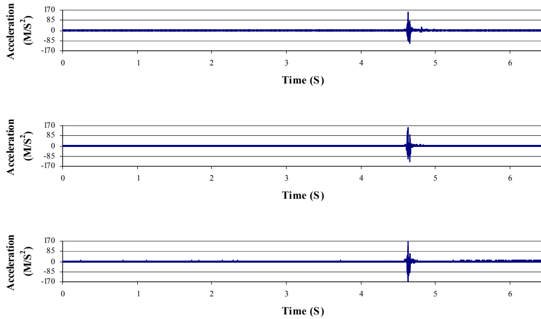
Figure A-76. Acceleration data from the femoral stem accelerometer for a metal-on-polyethylene THA, subjected to a 1500 Newton impact load. The signals are for the C1-axis (upper), C2-axis (middle) and C3-axis (lower).
