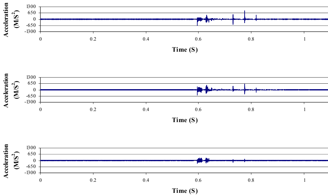
Figure A-96. Acceleration data from the femoral stem accelerometer for a ceramic-on-ceramic THA, subjected to a 1730 Newton impact load. The signals are for the C1-axis (upper), C2-axis (middle) and C3-axis (lower).
