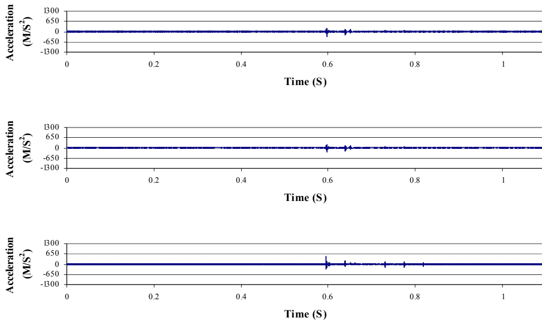
Figure A-94. Acceleration data from the pelvis accelerometer for a ceramic-on-ceramic THA, subjected to a 1730 Newton impact load. The signals are for the A1-axis (upper), A2-axis (middle) and A3-axis (lower).
