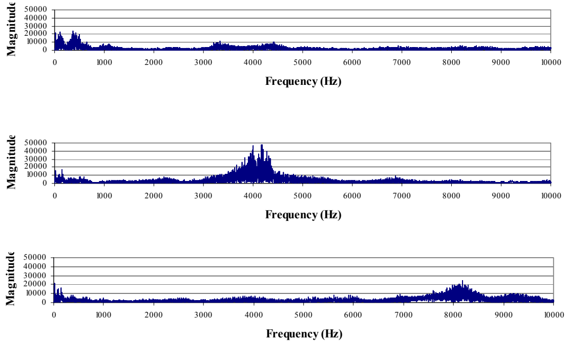
Figure A-181. FFT data from the greater trochanter accelerometer for a ceramic-on-ceramic THA, subjected to a 1900 Newton impact load. The signals are for the D1-axis (upper), D2-axis (middle) and D3-axis (lower).
