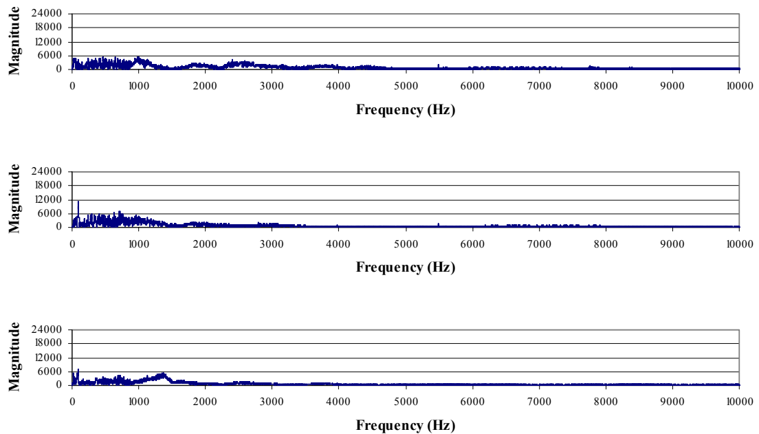
Figure A-159. FFT data from the acetabular cup accelerometer for a metal-on-polyethylene THA, subjected to a 1730 Newton impact load. The signals are for the B1-axis (upper), B2-axis (middle) and B3-axis (lower).
