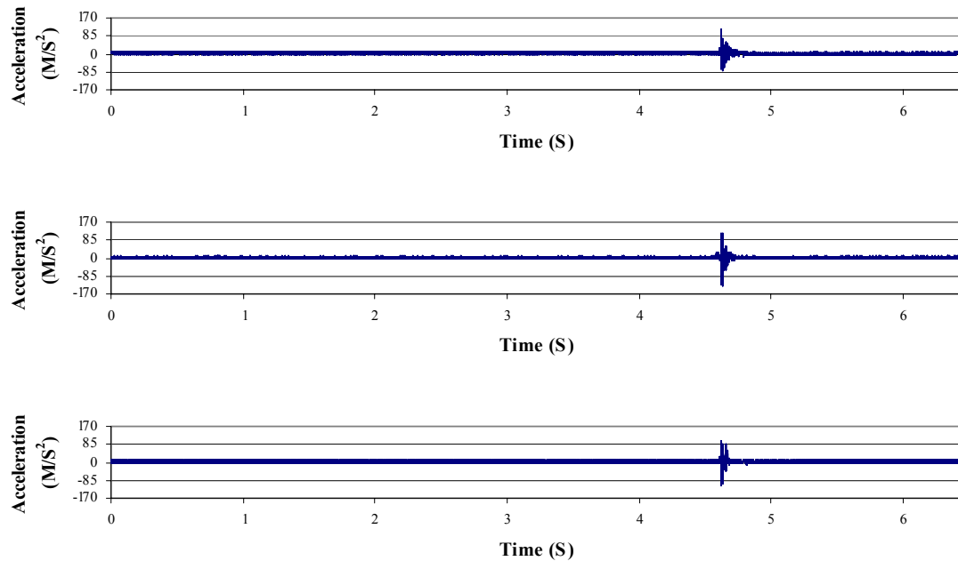
Figure A-77. Acceleration data from the greater trochanter accelerometer for a metal-on-polyethylene THA, subjected to a 1500 Newton impact load. The signals are for the D1-axis (upper), D2-axis (middle) and D3-axis (lower).
