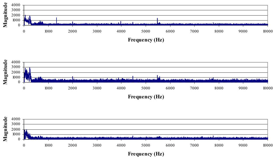
Figure A-117. FFT data from the greater trochanter accelerometer for a metal-on-metal THA, subjected to a 680 Newton impact load. The signals are for the D1-axis (upper), D2-axis (middle) and D3-axis (lower).
