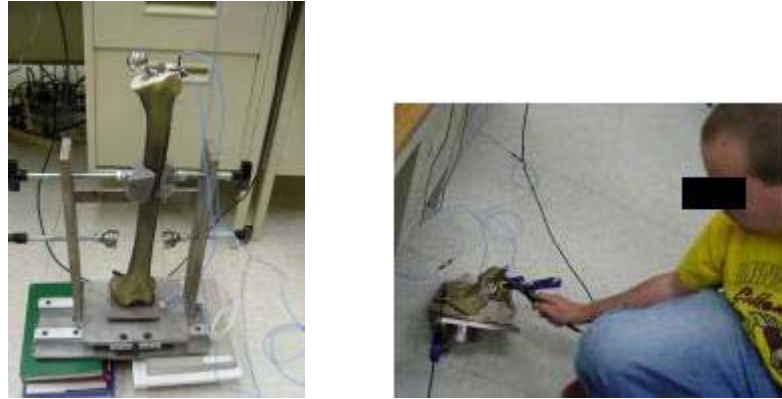
A. B. Figure 28. Resonant Test for A.) Femur and B.) Pelvis in Corresponding Fixtures
