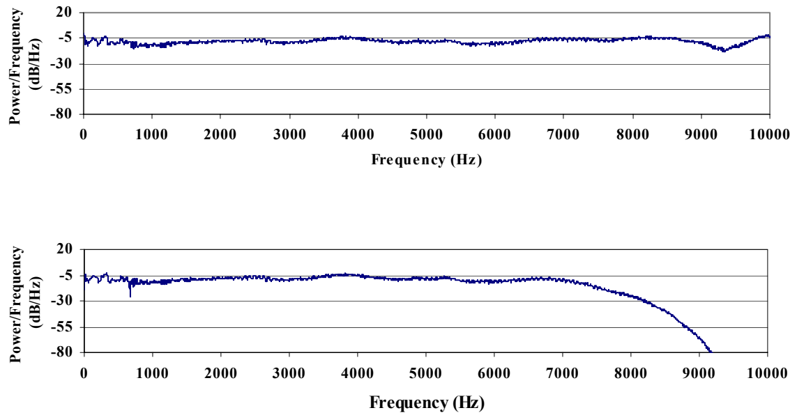
Figure 37. Comparison of PSD Signal Without Filtering (top) and with Filtering (bottom)
