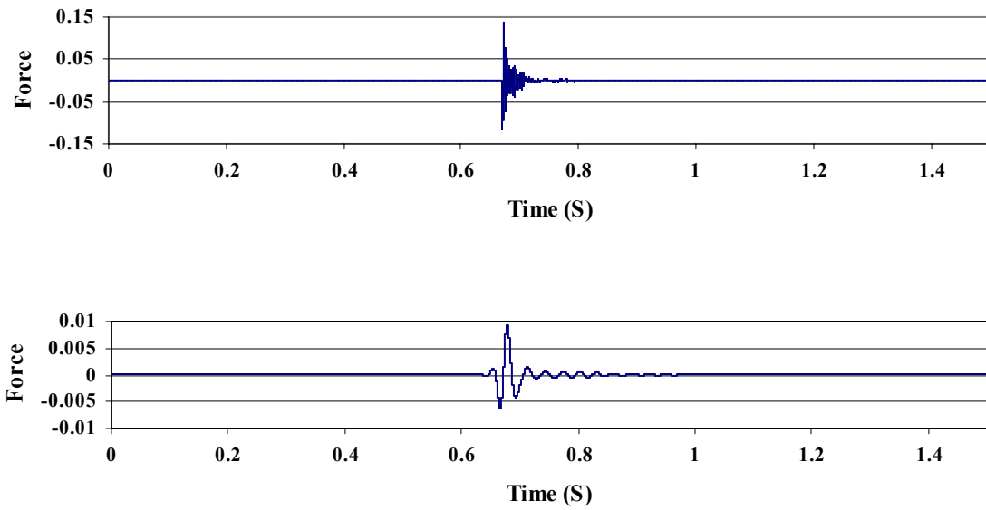
Figure 38. Comparison of Force Signal and Force Signal After a Smoothing Filter is Applied
