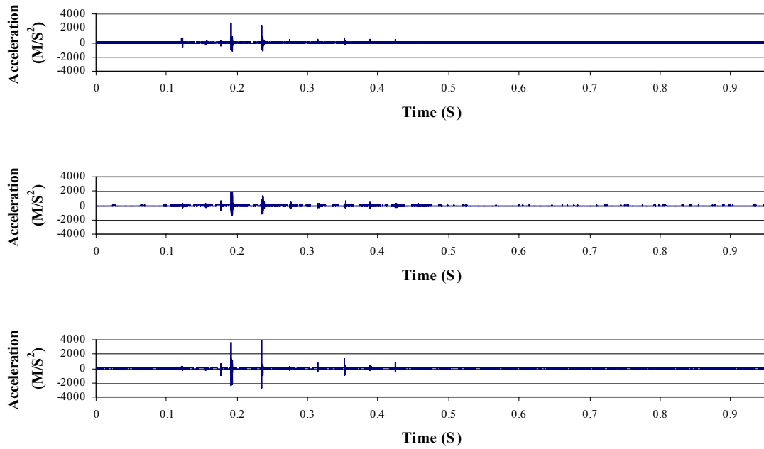
Figure A-59. Acceleration data from the acetabular cup accelerometer for a ceramic-on-ceramic THA, subjected to an 1150 Newton impact load. The signals are for the B1-axis (upper), B2-axis (middle) and B3-axis (lower).
