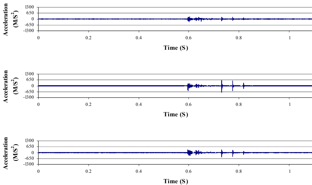
Figure A-97. Acceleration data from the greater trochanter accelerometer for a ceramic-on-ceramic THA, subjected to a 1730 Newton impact load. The signals are for the D1-axis (upper), D2-axis (middle) and D3-axis (lower).
