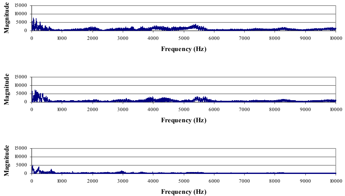
Figure A-140. FFT data from the femoral stem accelerometer for a metal-on-metal THA, subjected to a 1280 Newton impact load. The signals are for the C1-axis (upper), C2-axis (middle) and C3-axis (lower).
