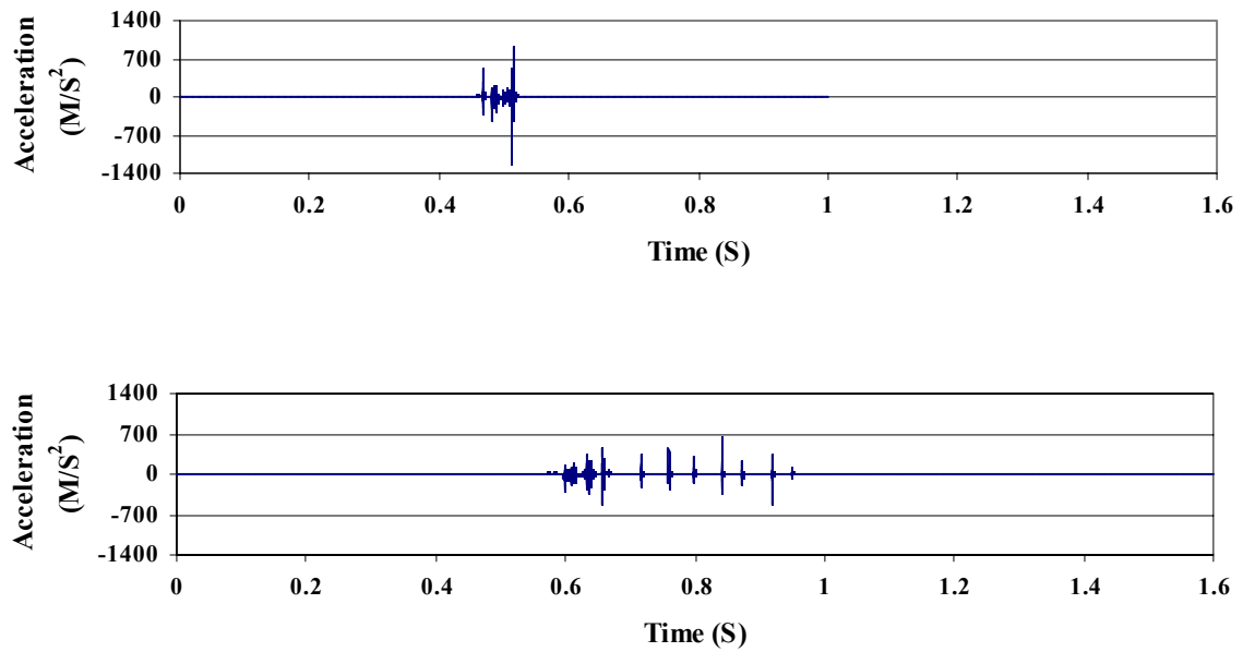
Figure 43. Comparison of Acceleration Signals for COC at Minimum Test Load (top) and Maximum Test Load (lower).
