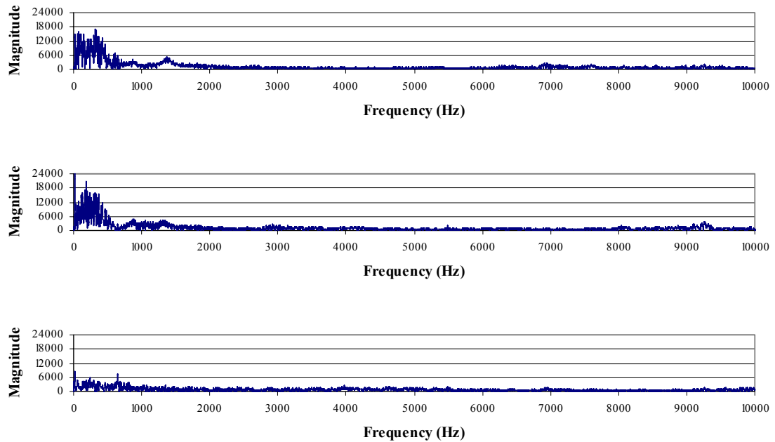
Figure A-160. FFT data from the femoral stem accelerometer for a metal-on-polyethylene THA, subjected to a 1730 Newton impact load. The signals are for the C1-axis (upper), C2-axis (middle) and C3-axis (lower).
