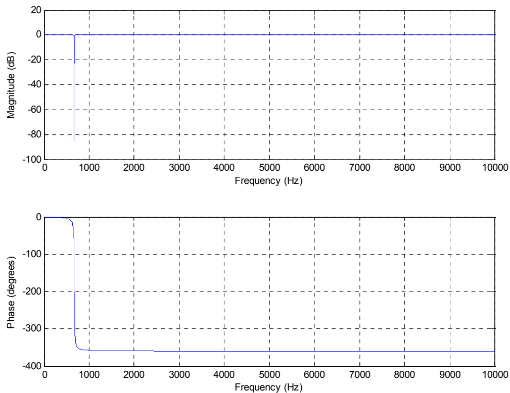
Figure 34. Magnitude and Phase of the Stopband Filter
