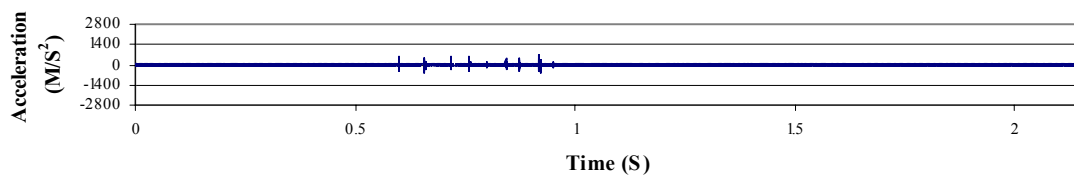
Figure A-106. Acceleration data from the pelvis accelerometer for a ceramic-on-ceramic THA, subjected to a 1900 Newton impact load. The signals are for the A1-axis (upper), A2-axis (middle) and A3-axis (lower).
