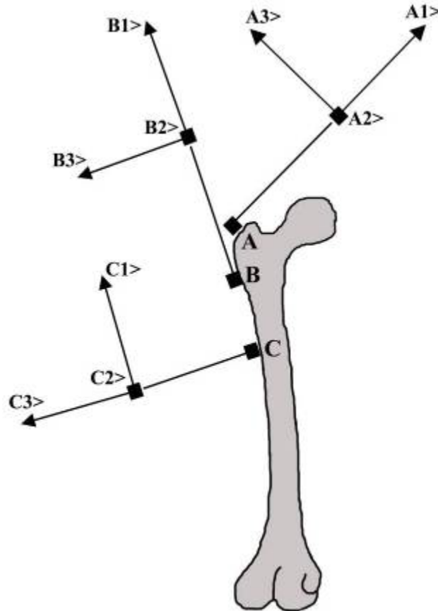
Figure 16. Orientation of Accelerometers During Normal Femur Testing
