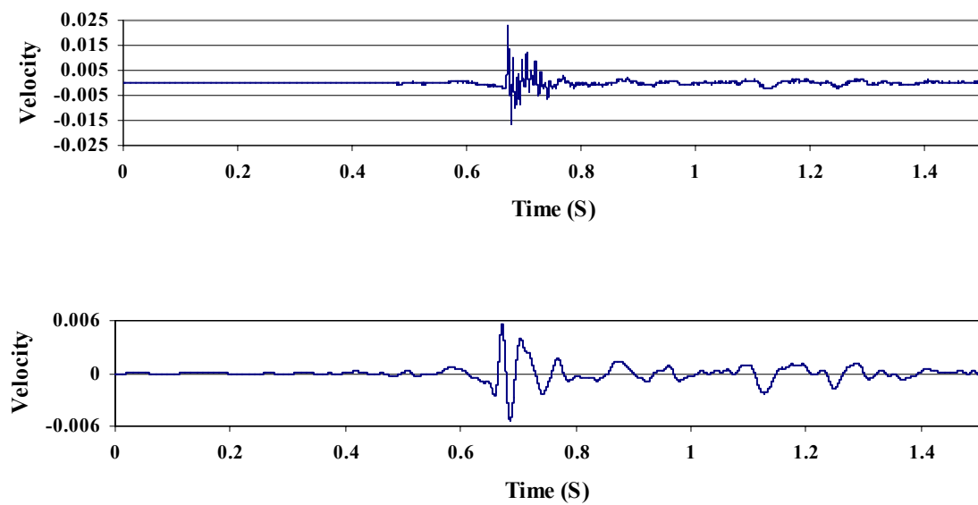
Figure 39. Comparison of Velocity Signal and Velocity Signal After a Smoothing Filter is Applied
