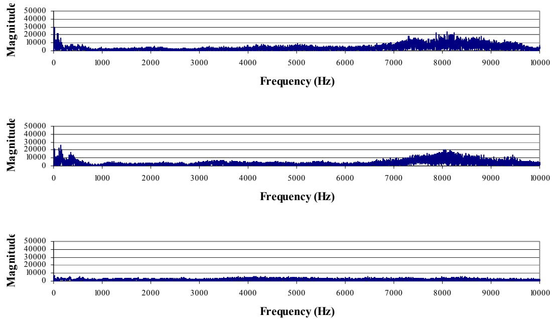
Figure A-180. FFT data from the femoral stem accelerometer for a ceramic-on-ceramic THA, subjected to a 1900 Newton impact load. The signals are for the C1-axis (upper), C2-axis (middle) and C3-axis (lower).
