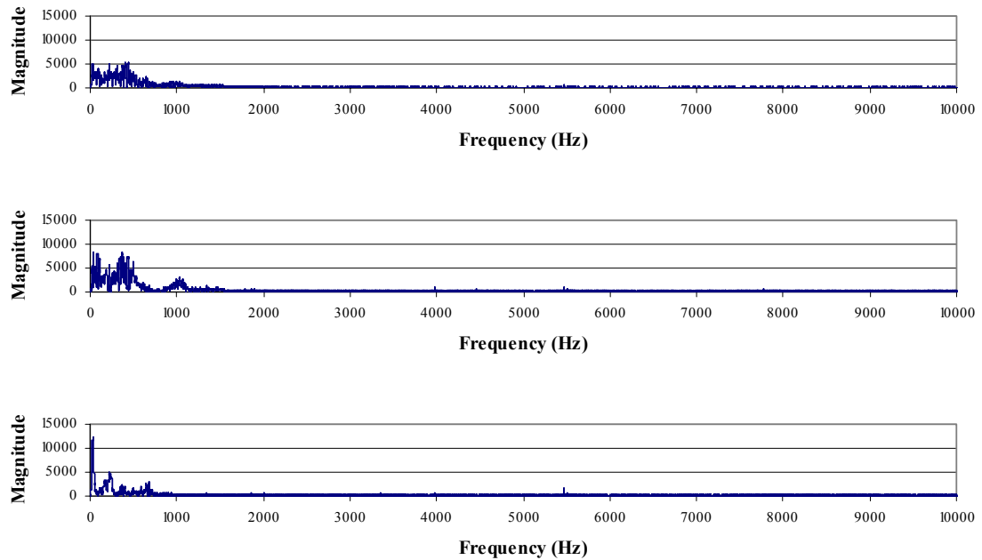
Figure A-112. FFT data from the femoral stem accelerometer for a metal-on-polyethylene THA, subjected to a 680 Newton impact load. The signals are for the C1-axis (upper), C2-axis (middle) and C3-axis (lower).
