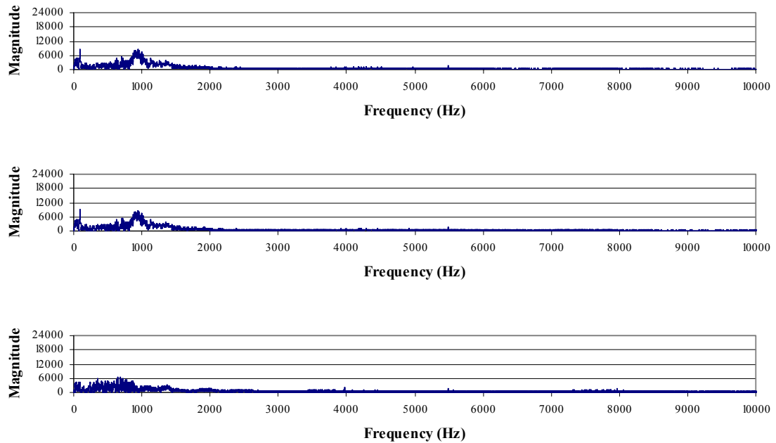
Figure A-158. FFT data from the pelvis accelerometer for a metal-on-polyethylene THA, subjected to a 1730 Newton impact load. The signals are for the A1-axis (upper), A2-axis (middle) and A3-axis (lower).
