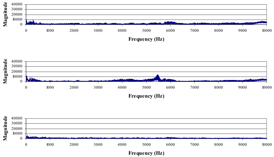
Figure A-176. FFT data from the femoral stem accelerometer for a metal-on-metal THA, subjected to a 1900 Newton impact load. The signals are for the C1-axis (upper), C2-axis (middle) and C3-axis (lower).
