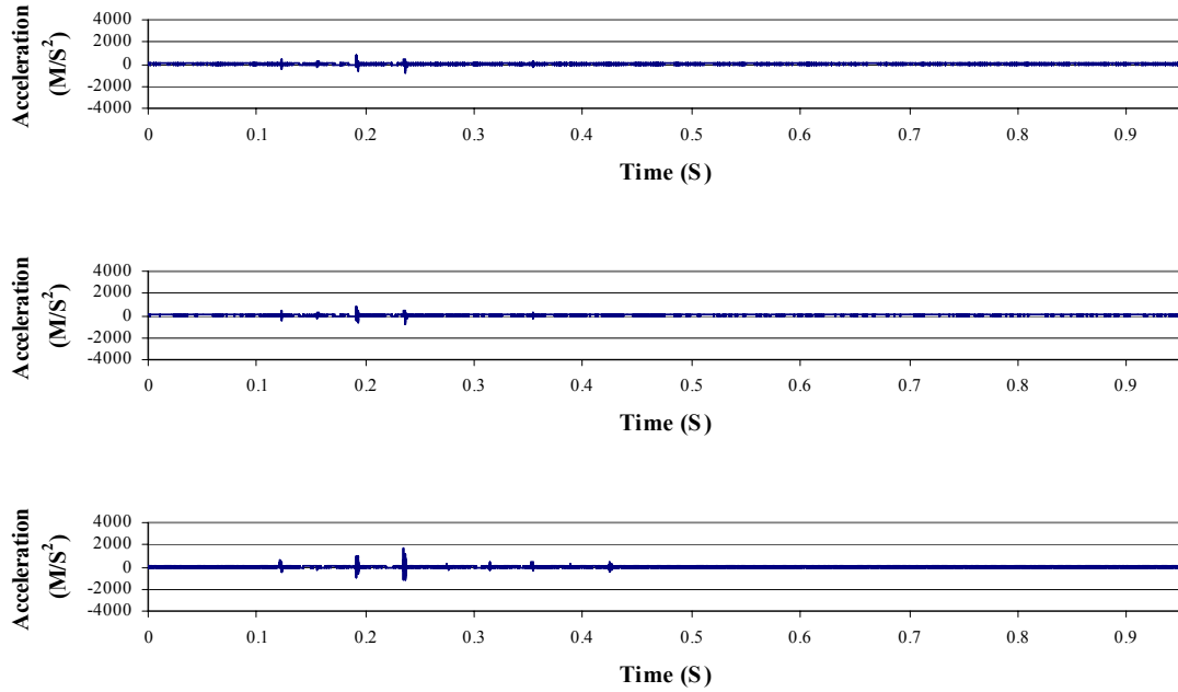
Figure A-58. Acceleration data from the pelvis accelerometer for a ceramic-on-ceramic THA, subjected to an 1150 Newton impact load. The signals are for the A1-axis (upper), A2-axis (middle) and A3-axis (lower).
