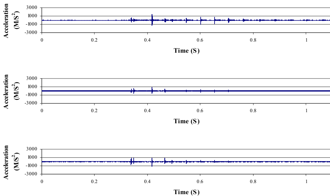
Figure A-71. Acceleration data from the acetabular cup accelerometer for a ceramic-on-ceramic THA, subjected to a 1280 Newton impact load. The signals are for the B1-axis (upper), B2-axis (middle) and B3-axis (lower).
