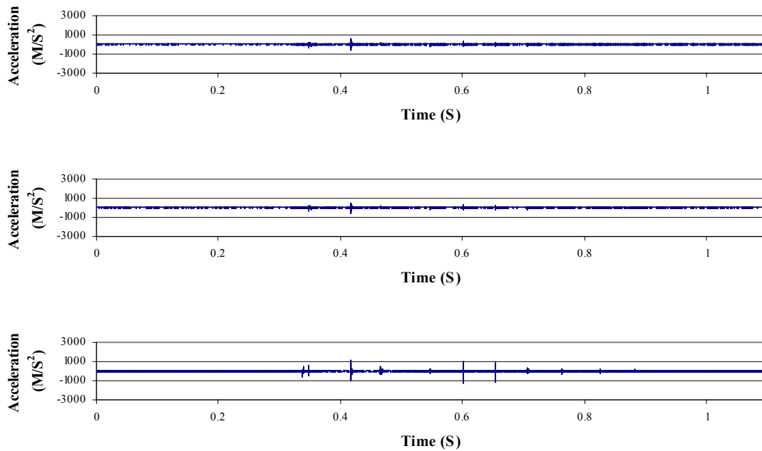
Figure A-70. Acceleration data from the pelvis accelerometer for a ceramic-on-ceramic THA, subjected to a 1280 Newton impact load. The signals are for the A1-axis (upper), A2-axis (middle) and A3-axis (lower).
