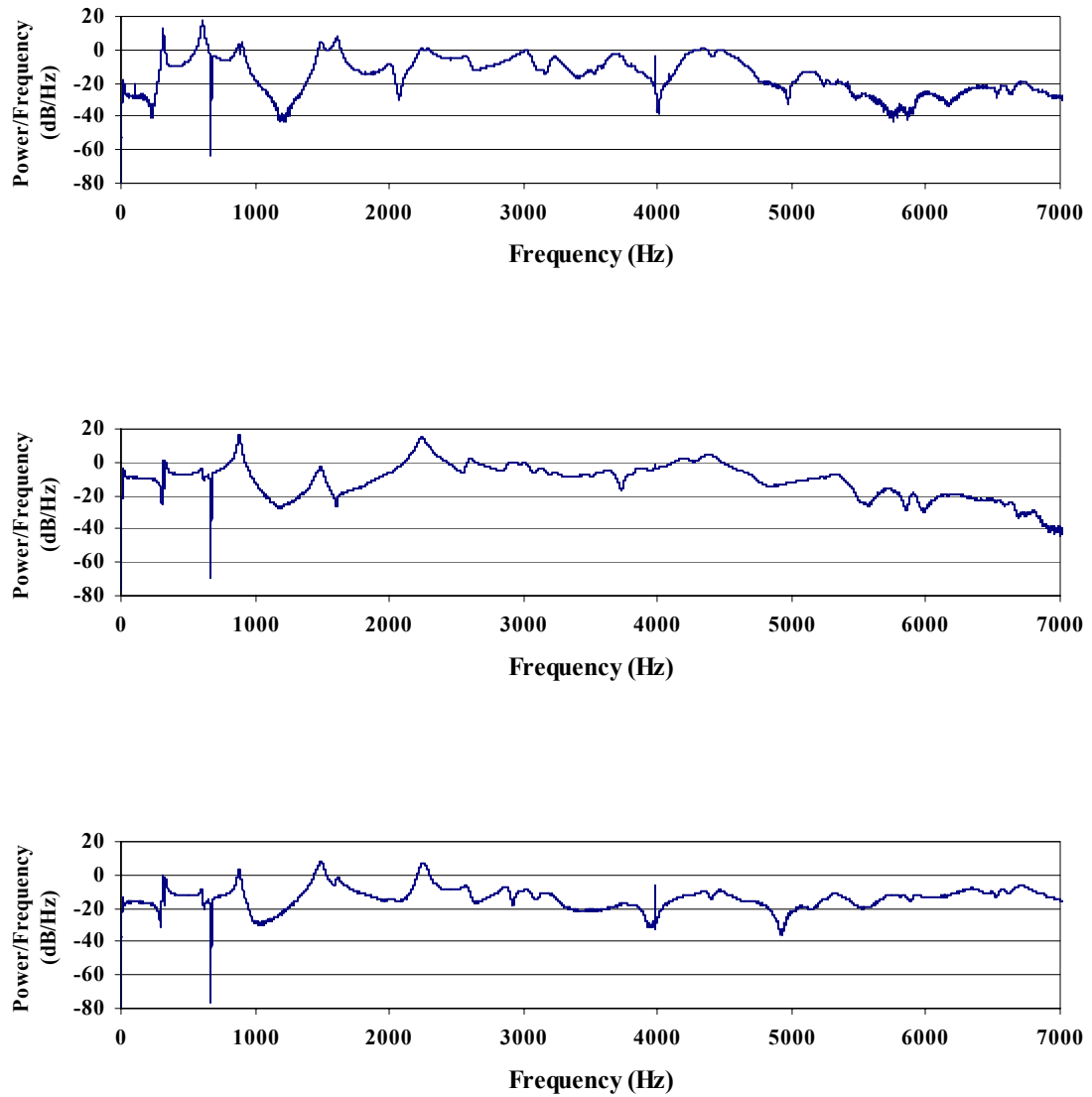
Figure 48. PSD Data for the Unimplanted Femur Resonance Test. The Accelerometer Shown Here was Mounted on the Greater Trochanter and the Signals are for the A1-axis (upper), A2-axis (middle), and the A3 -axis (lower).
