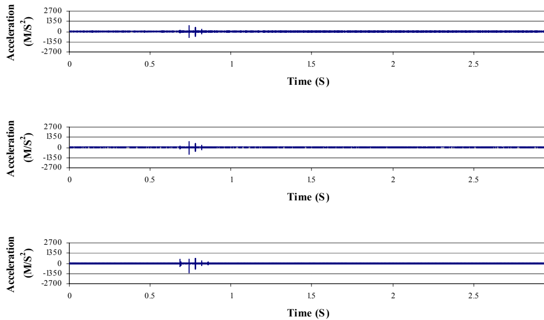
Figure A-78. Acceleration data from the pelvis accelerometer for a metal-on-metal THA, subjected to a 1500 Newton impact load. The signals are for the A1-axis (upper), A2-axis (middle) and A3-axis (lower).
