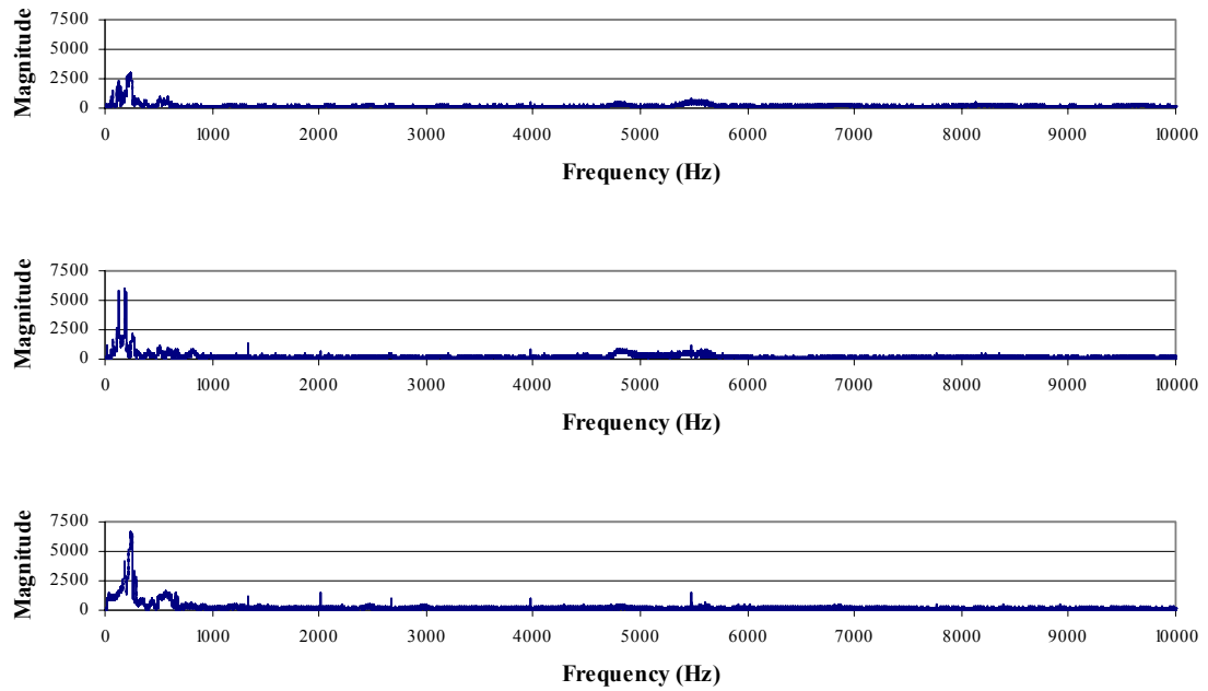
Figure A-128. FFT data from the femoral stem accelerometer for a metal-on-metal THA, subjected to an 1150 Newton impact load. The signals are for the C1-axis (upper), C2-axis (middle) and C3-axis (lower).
