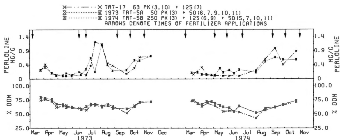
Figure 20. Comparison of the effects of three, six, and seven fertilizer applications on tall fescue digestibility and perloline content in 1973-74.
