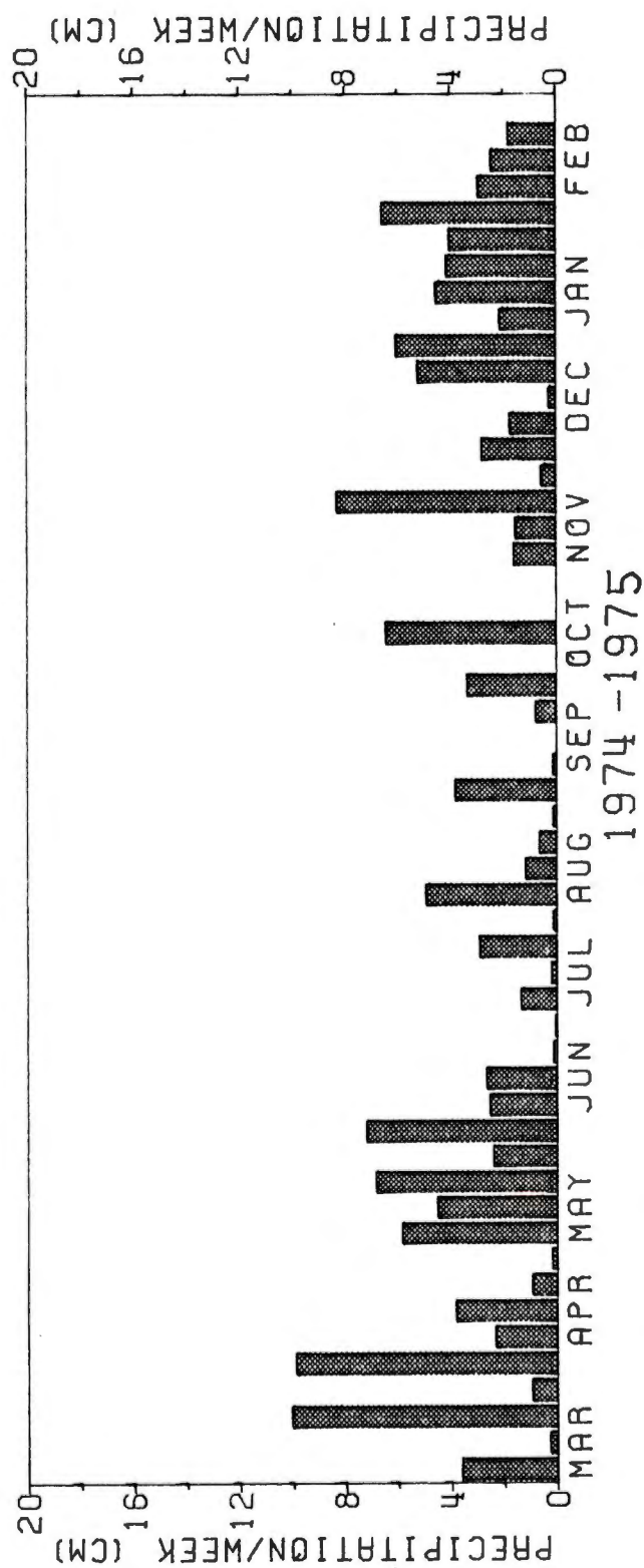
Figure 40. Weekly precipitation for March 1974-March 1975 in cm.
