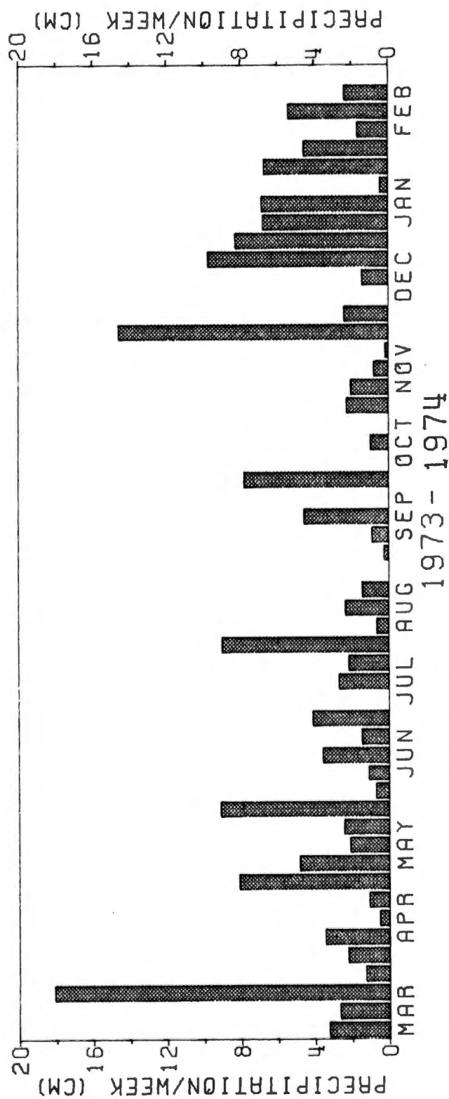
Figure 39. Weekly precipitation for March 1973-March 1974 in cm.
