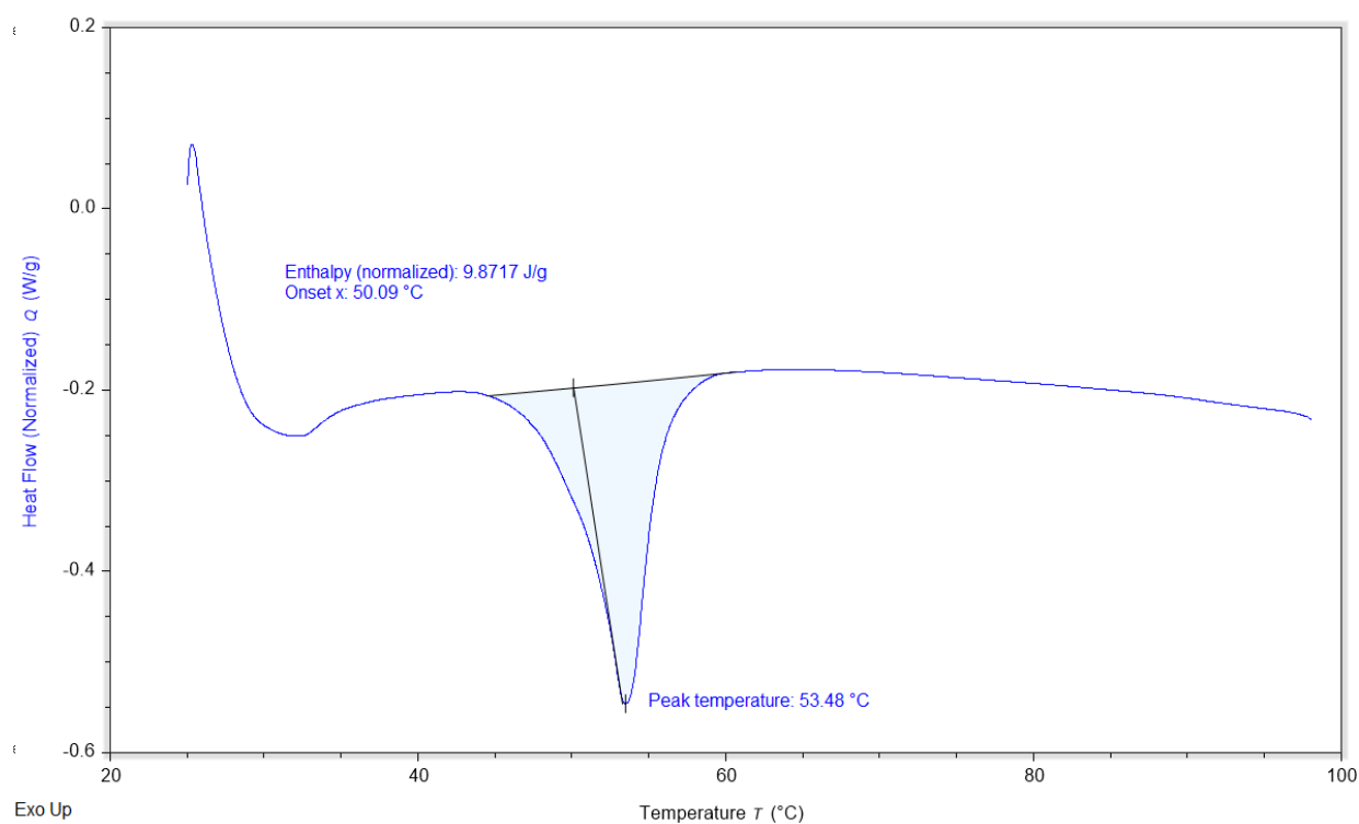
Figure 37. DSC melting curve of TEW
