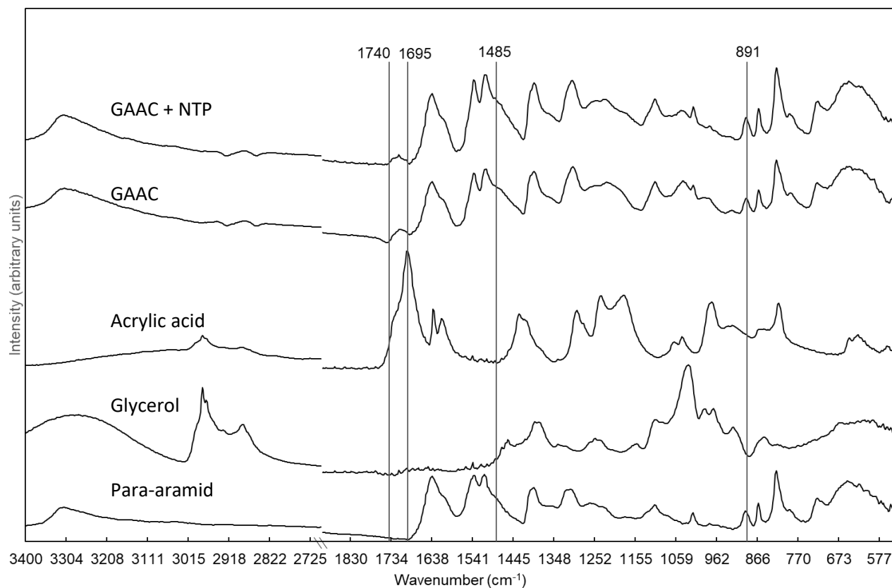
Figure 12. FTIR of para-aramid fabric, glycerol, acrylic acid, and glycerol and acrylic acid pretreatment on the surface of para-aramids before and after NTP treatment
