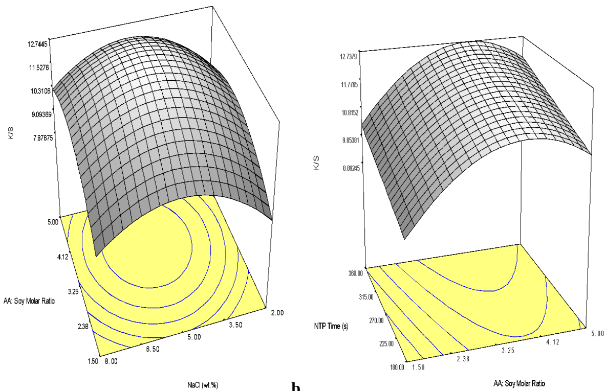
Figure 8. K/S value surface plot of molar ratio of soybean oil to acrylic acid , NaCl concentration, and NTP time after the first detergent wash with a. NTP treatment time held constant at 360 s and b. NaCl concentration held constant at 5.0 wt.% ( r^2 = 0.8065 )
