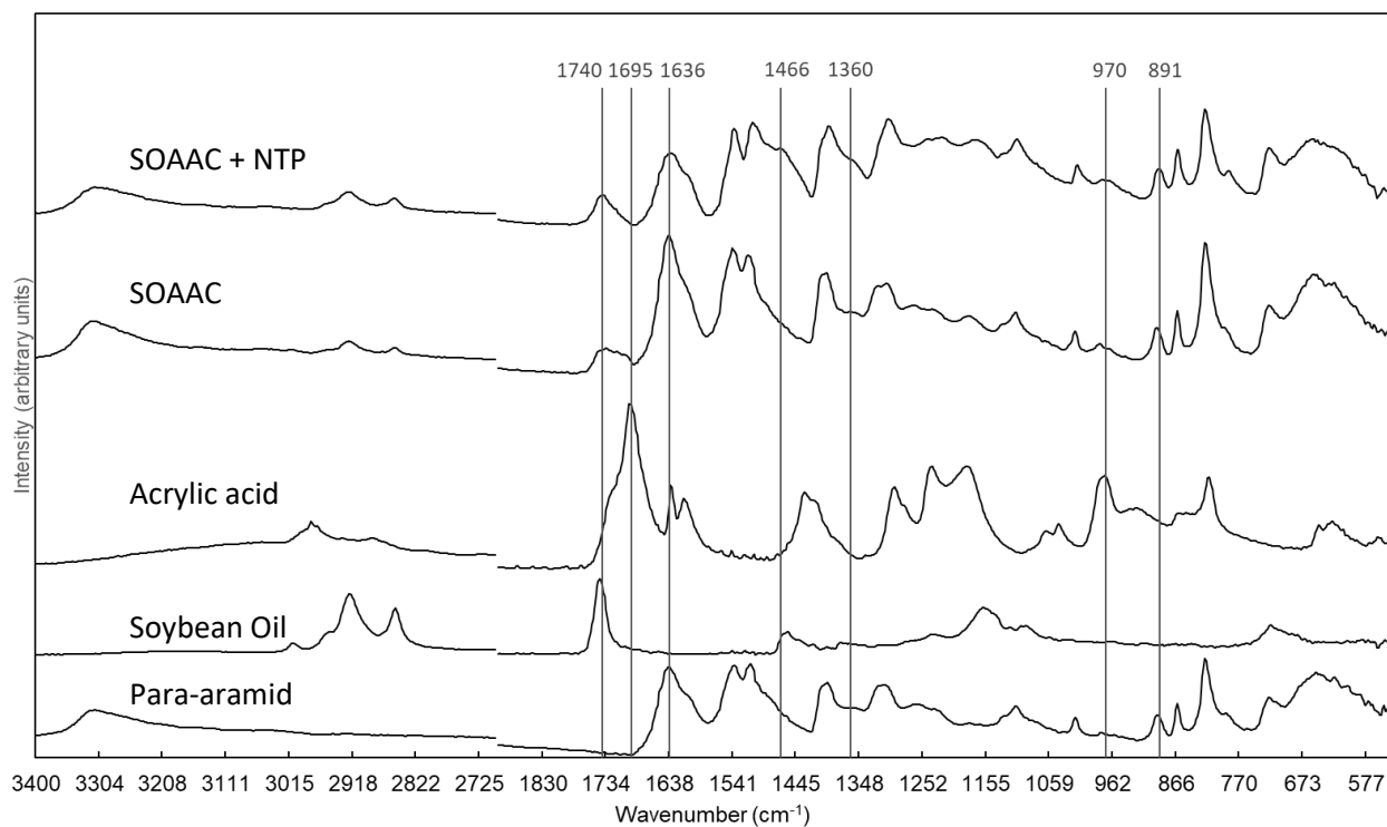
Figure 11. FTIR of para-aramid fabric, soybean oil, acrylic acid, and soybean oil and acrylic acid pretreatment on the surface of para-aramids before and after NTP treatment
