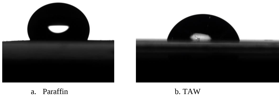
Figure 41. Surface contact angle images of paraffin and TAW with 10 \mu\text{L} of deionized water deposited on the surface.
