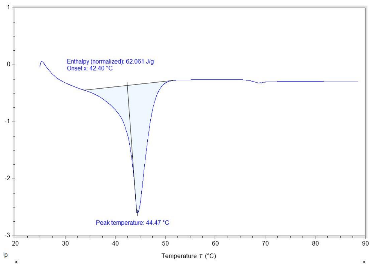
Figure 35. DSC melting curve of TAW
