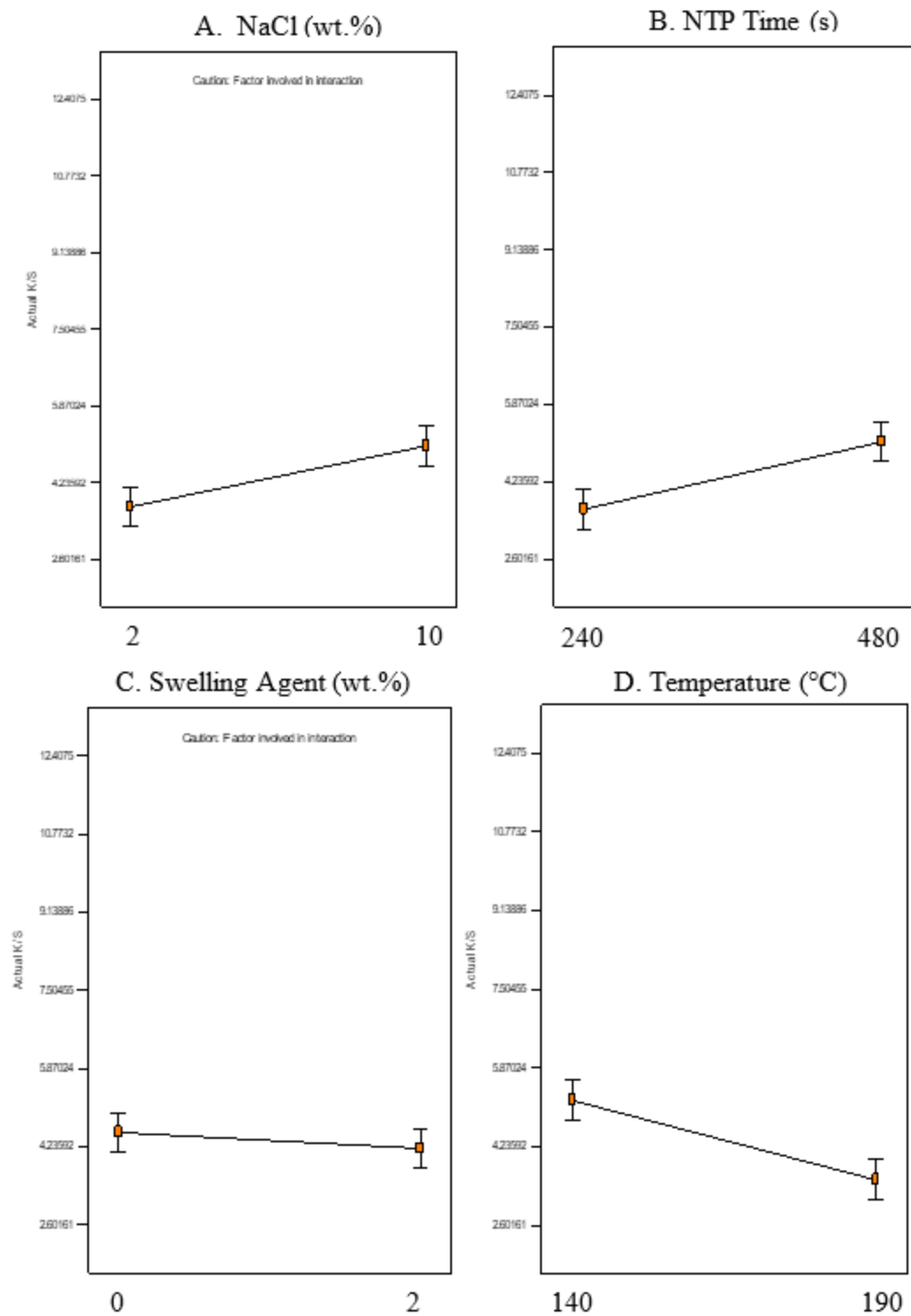
Figure 21. Main effect and interactions of swelling agent, NaCl, and NTP treatment, and temperature.
