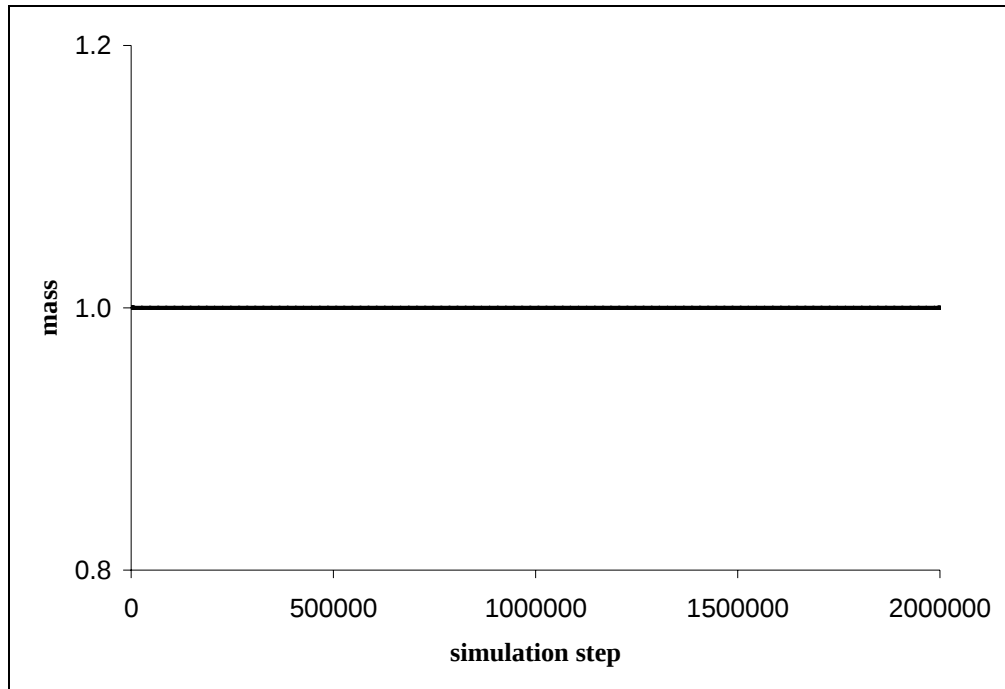
Figure 3.1-1 Mass vs. simulation steps for an ideal gas system, with \mu^{*set} = \mu^*(t_0) .
