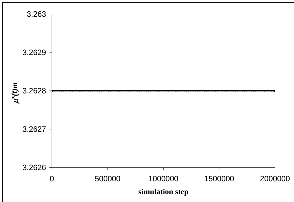
Figure 3.1-2 \mu^*(t)m vs. simulation steps for an ideal gas system, with \mu^{*set} = \mu^*(t_0) .
