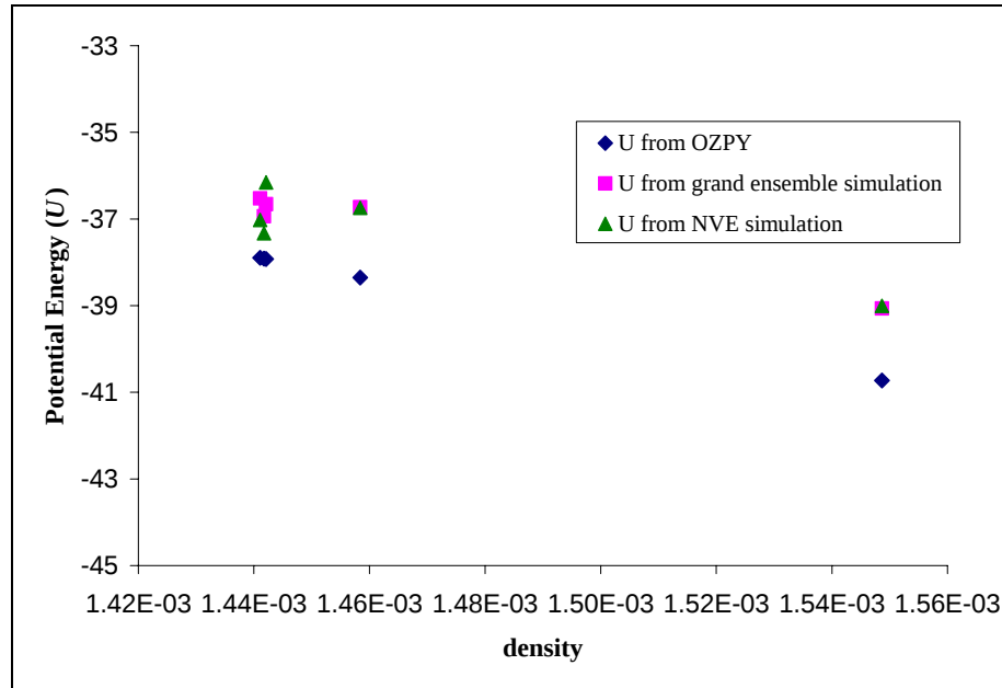
Figure 3.4-5 The potential energy from \mu V\mathcal{E} , NVE and OZPY vs. density.
