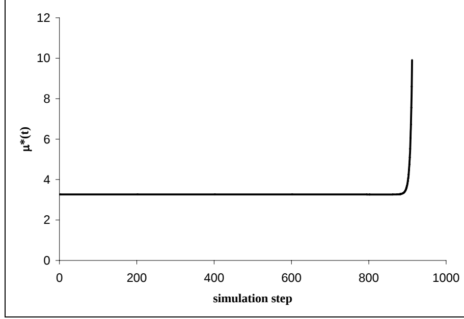
Figure 3.3-1 \mu^*(t) vs. simulation step for a dilute gas system, specific potential energy case, with \mu^{*set} = \mu^*(t_0) .
