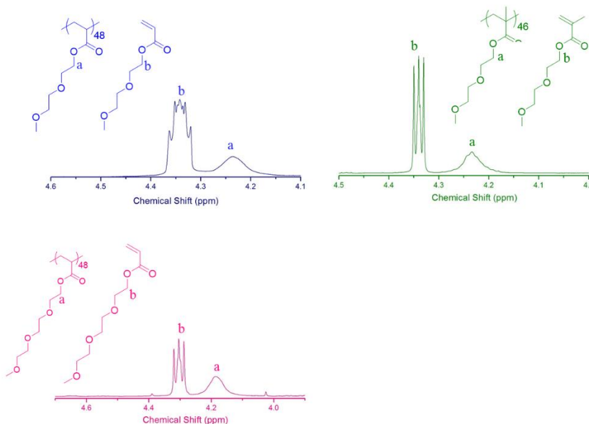
Figure 3: ^1\text{H} -NMR graphs focusing on the 2 main peaks used for ^1\text{H} -NMR analysis. ‘b’ represents 2 H atoms on the monomer peak while ‘a’ represents 2 H atoms on the polymer peak.
