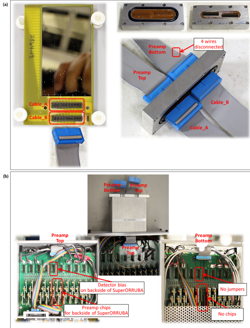
Figure A.8: Cable setup for SuperORRUBA detector and preamplifier box. (a) A SuperORRUBA detector (left) has two 40pin high-density connectors on the backside. A feedthrough (top right) also includes two sets of 40 jumper pins to interconnect inside and outside the vacuum chamber. The channel number order will be swapped at the feedthrough. (b) Top (left) and bottom (right) of the preamplifier box can be identified by bias jumper pin JP5 and preamp chips on slot 17-20 (middle 4 slots).
