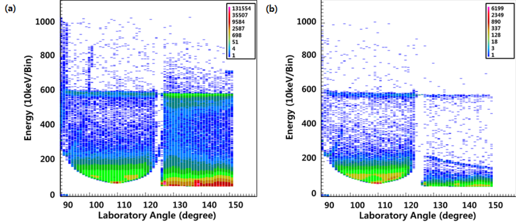
Figure 4.11: A 2D spectrum before (a) and after (b) gating on the TAC. Real events were filtered by the TAC peak and most sources of noise and contamination were removed.
