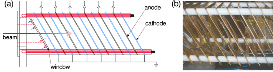
Figure 1: (Color online) (a) The cross-sectional view of the fast ionization chamber, and (b) the picture of the electrodes assembled in the chamber are shown in the figure.
