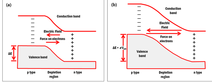
Figure 3.6: (a) p-n junction diode without bias. When n-type and p-type materials are brought into contact, the depletion region is created to allow charge particles ionize electrons, creating holes with their kinetic energy in the process. (b) p-n junction with reverse bias (a cathode connected to the n-type side). The depleted region becomes larger and the magnitude of the electric field increases with the reverse bias [16].
