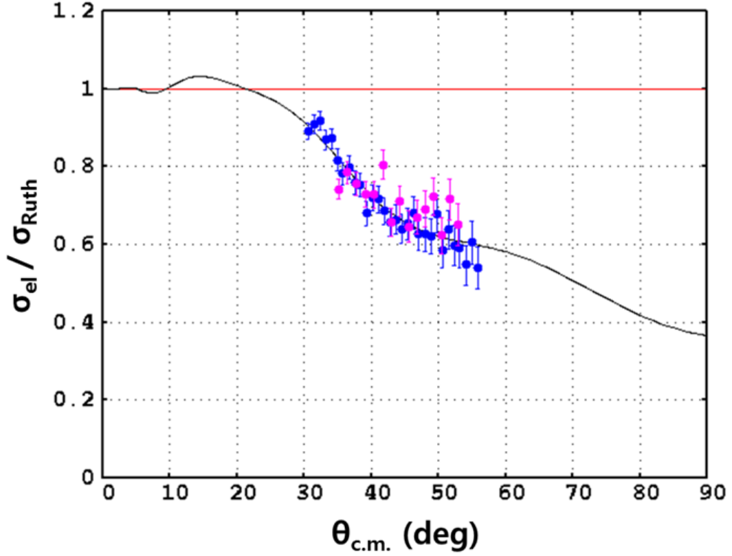
Figure 4.13: Ratio of measured data to the Rutherford differential cross section. The data are scaled to the elastic scattering calculation (black curve). Blue dots shows the data from the Super X3 detectors and purple dots are from the BB15 detector. The fit was confined to data with \theta_{\text{c.m.}} < 54^\circ as shown.
