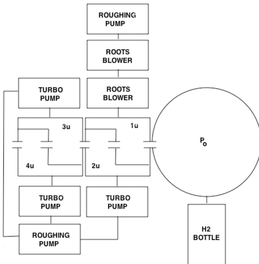
Figure 2.2: Schematic of the differential pumping system
