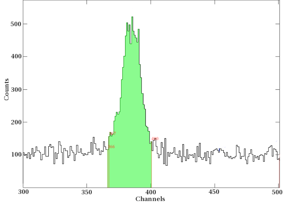
Figure 4.7: TAC spectrum for the E_{lab} = 19.07 MeV measurement. The shaded region indicates the region in which the events in Figure 4.6 fall.
