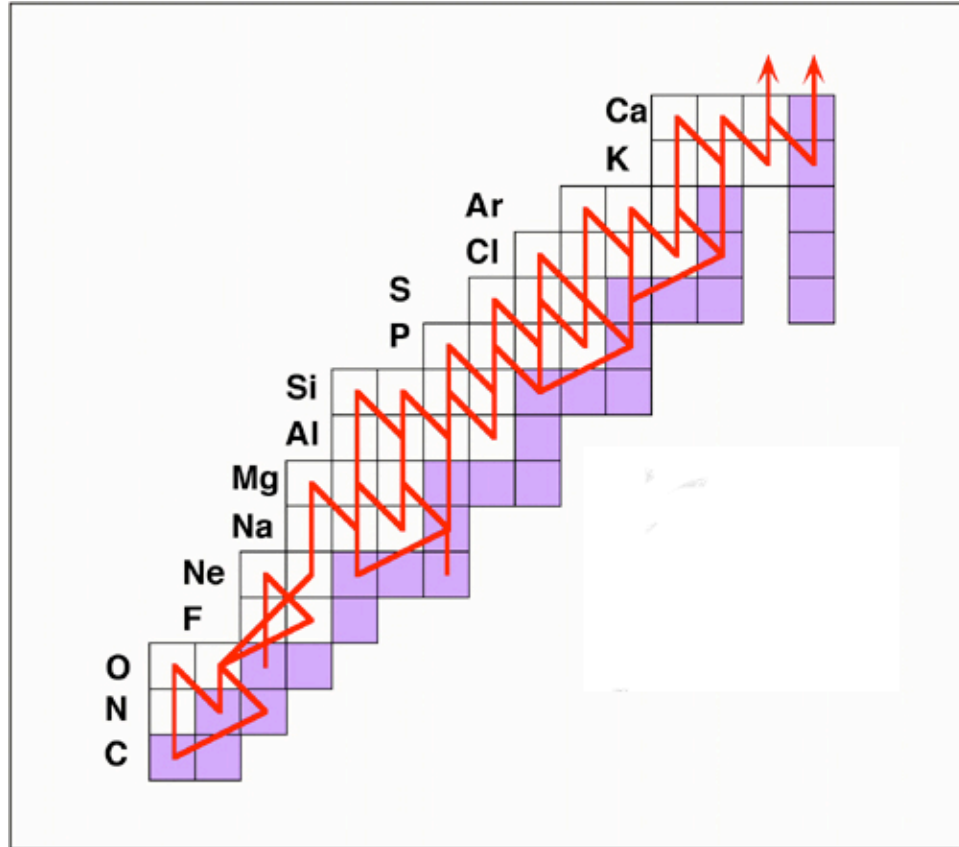
Figure 1.5: The rp -process in more energetic novae. Figure taken from Ref. [Cha92].
