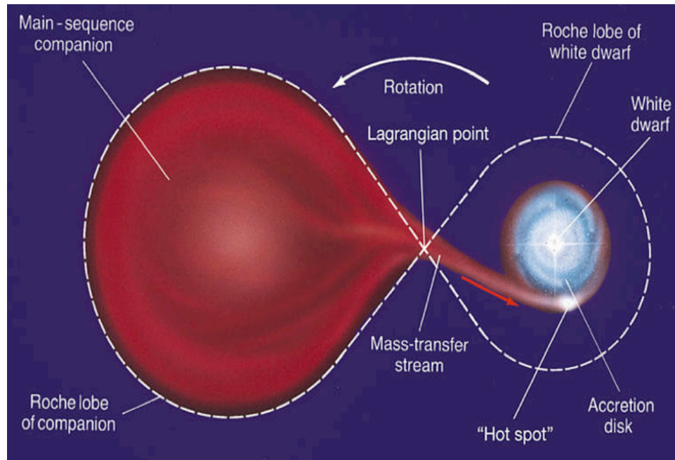
Figure 1.2: Schematic of the accretion of hydrogen and helium from a main-sequence star onto the surface of a white dwarf. Figure taken from Ref. [Pea05].
