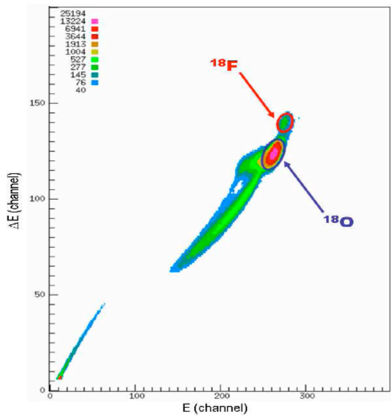
Figure 5.5: Sample ion counter spectrum from the ^{18}\text{F}(\text{p},\alpha)^{15}\text{O} reaction study by Chae [Cha06].
