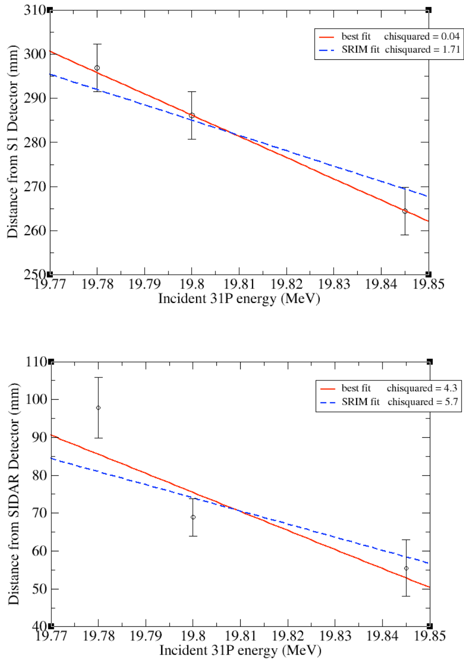
Figure 4.13: The reaction vertex plotted against the distance to the plane of the S1 detector (top) and SIDAR (bottom). The red (solid) lines represent the best least-squares fits to the data while the blue (dashed) lines are fits using a slope from the stopping power given by SRIM [Zie03] where the intercept was varied in order to minimize \chi^2 .
