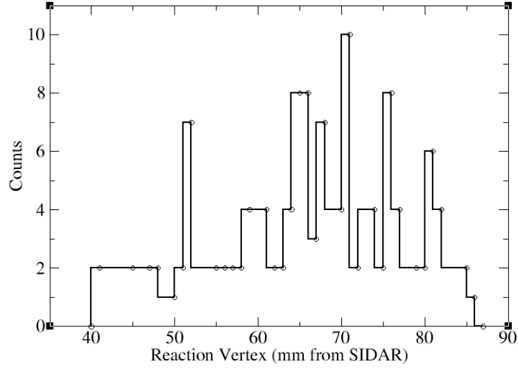
Figure 4.8: The distribution of ^1\text{H}(^{31}\text{P}, \alpha)^{28}\text{Si} events as a function of the distance from the plane of SIDAR (mm) at an incident ^{31}\text{P} energy of E_{lab} = 19.07 MeV.
