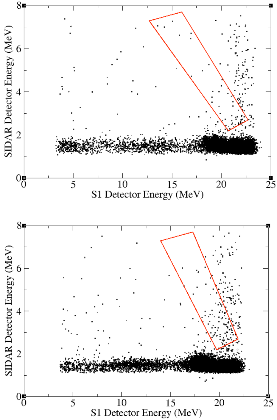
Figure 4.14: The energy of particles detected in SIDAR plotted against the energy of coincident particles in the S1 detector for an incident ^{35}\text{Cl} energy of 21.70 MeV (top) (off-resonance) and 20.01 MeV (bottom) (on-resonance). The drawn box is where (p, \alpha ) events are expected to fall.
