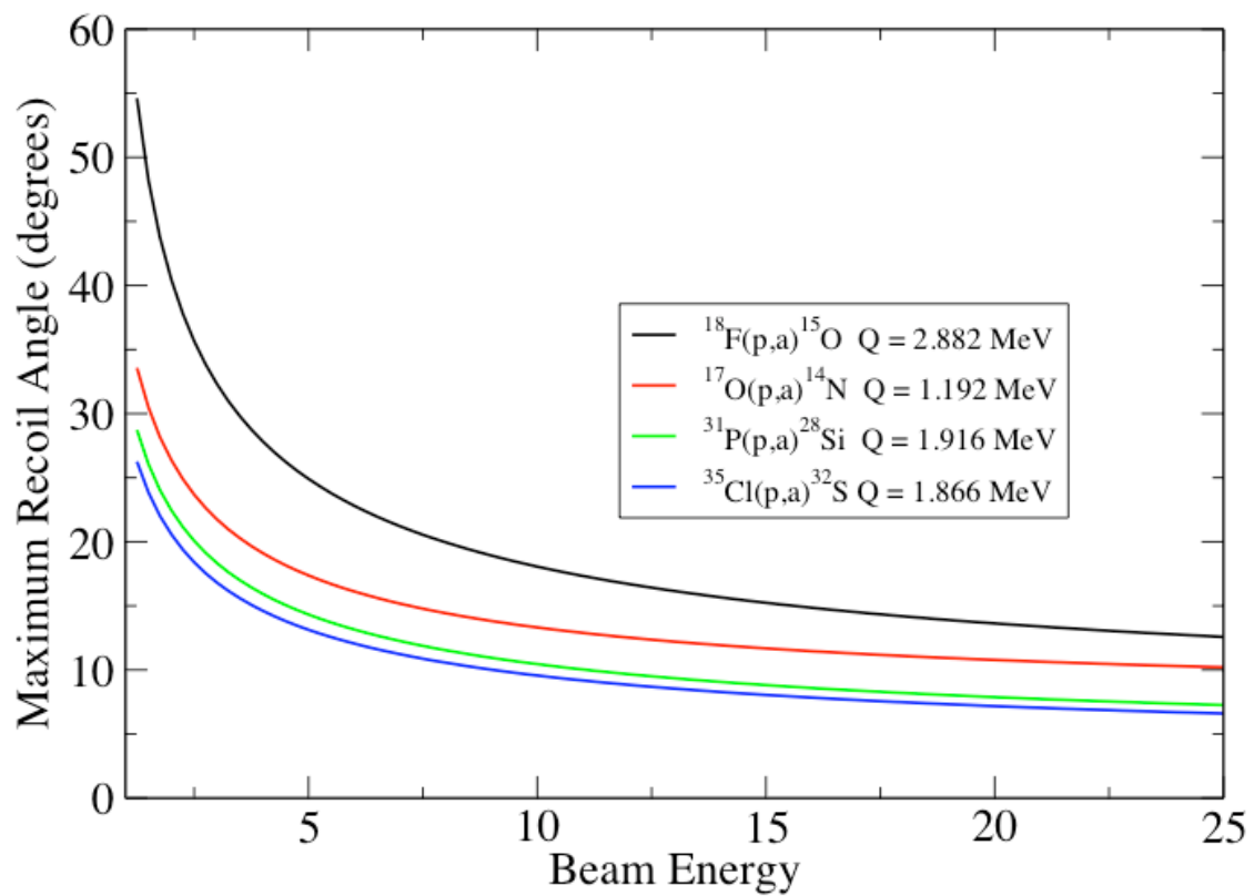
Figure 2.9: Maximum recoil angle (degrees) versus incoming beam energy (MeV) for several (p,α) reactions
