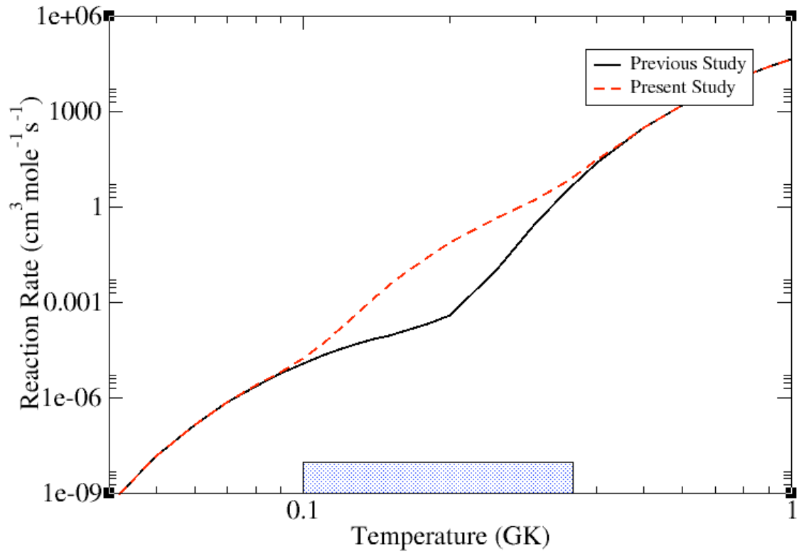
Figure 3.9: The ^{17}\text{O}(p, \alpha)^{14}\text{N} reaction rate as a function of temperature. The black curve is from a parametrization of the NACRE reaction rate [Ang99] while the red curve utilizes the new 183 keV resonance strength. The shaded region indicates nova temperatures.
