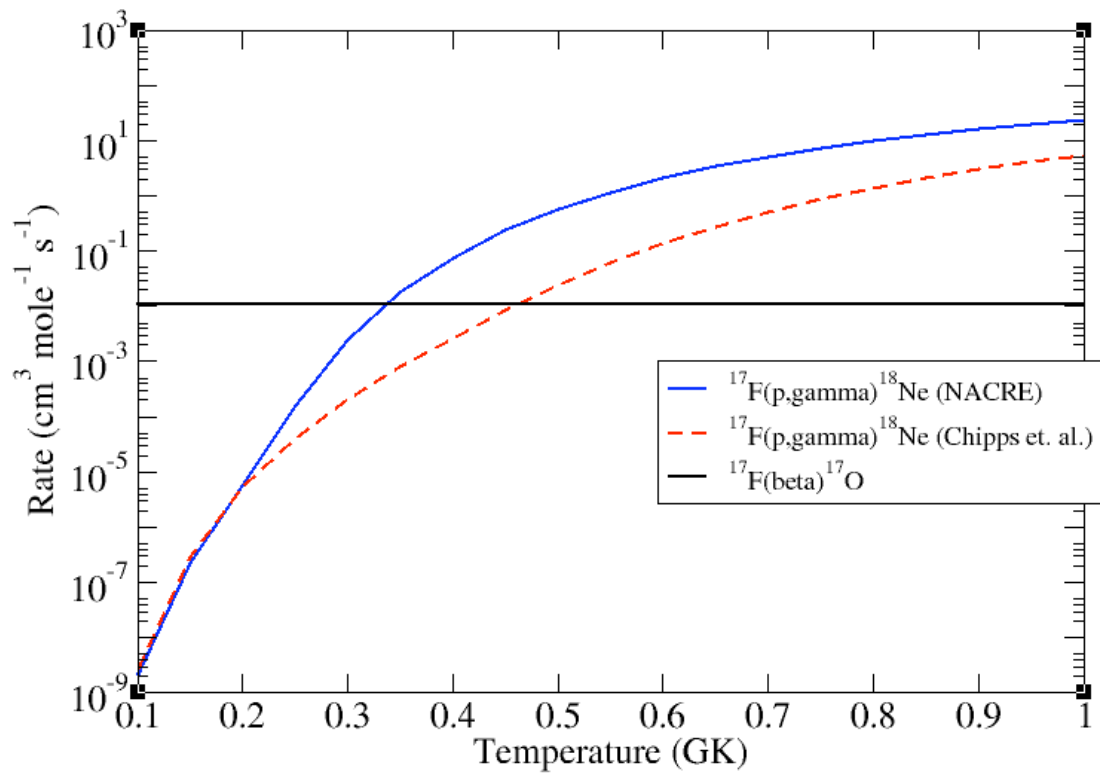
Figure 3.11: The competing ^{17}\text{F}(\beta)^{17}\text{O} and ^{17}\text{F}(p,\gamma)^{18}\text{Ne} reaction rates. The blue (solid) curve is the ^{17}\text{F}(p,\gamma)^{18}\text{Ne} reaction rate from Ref. [Ang99] while the red (dashed) is from the more recent study by Chipps et al. [Chi09].
