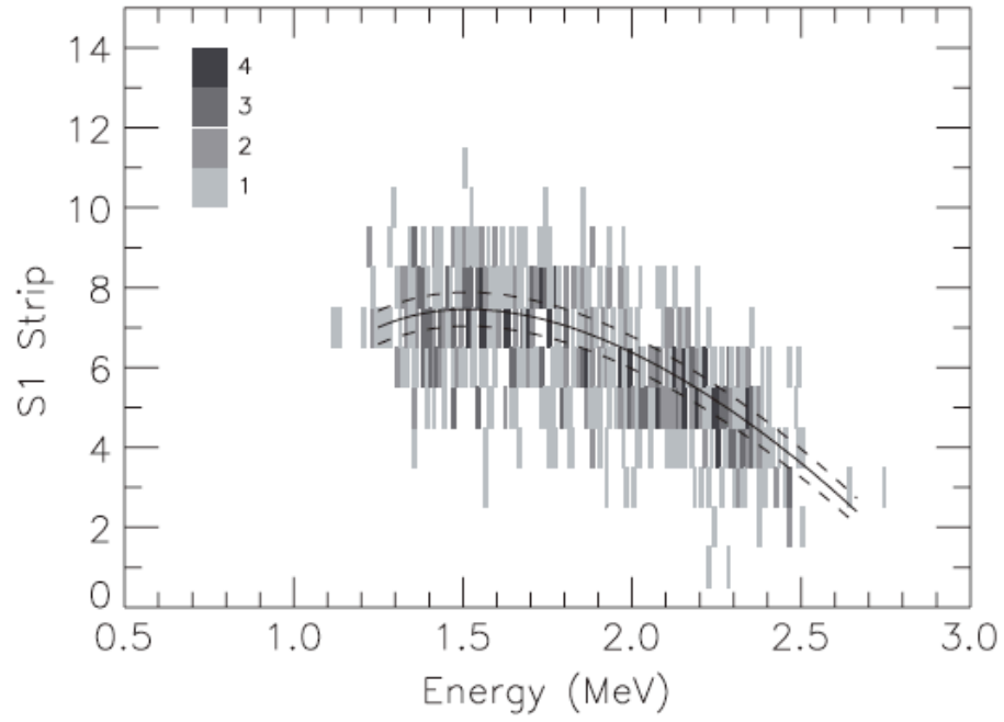
Figure 3.5: The distribution of {}^1\text{H}({}^{17}\text{O},\alpha){}^{14}\text{N} events by {}^{14}\text{N} angle (strip number) for an incident {}^{17}\text{O} beam energy of 3.34 MeV. The solid curve shows the best fit to the distribution by varying the distance to the reaction vertex. The dashed curves represent the upper and lower 1\sigma limits.
