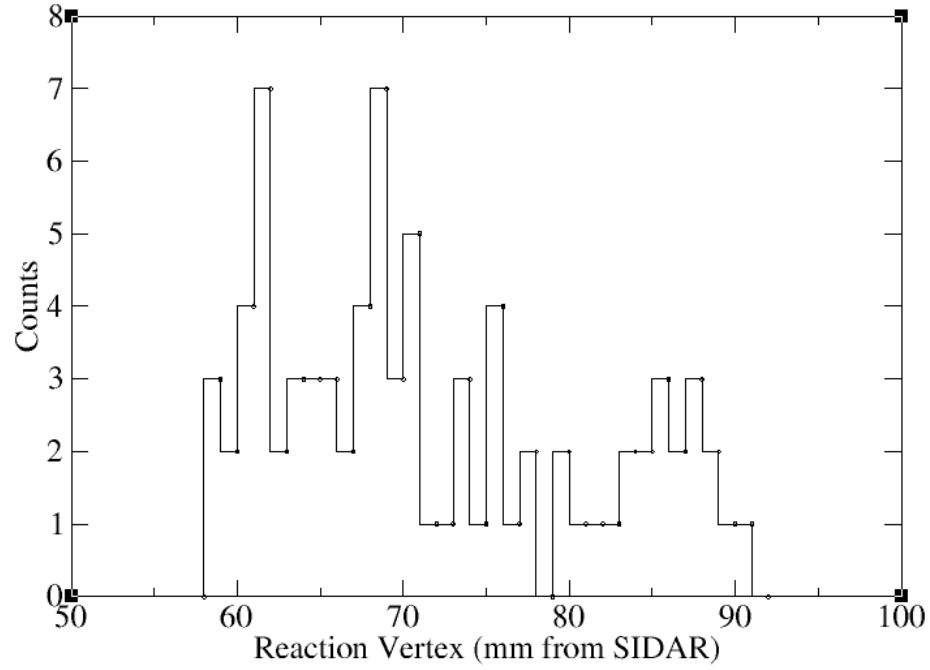
Figure 4.16: The distribution of ^1\text{H}(^{35}\text{Cl},\alpha)^{31}\text{S} events as a function of the distance from the plane of SIDAR (mm) at an incident ^{35}\text{Cl} energy of E_{\text{lab}} = 21.87 MeV.
