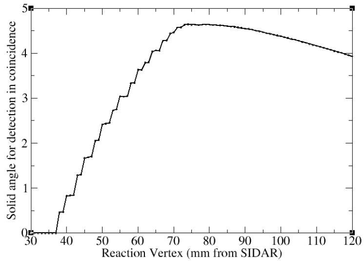
Figure 4.17: Total solid angle (center-of-mass frame) for detection of \alpha particles in coincidence with detection of the ^{31}\text{S} recoil versus the reaction vertex (measured from the plane of SIDAR) for the E_{\text{cm}} = 611 keV resonance in ^{35}\text{Cl}(\text{p},\alpha)^{31}\text{S} .
