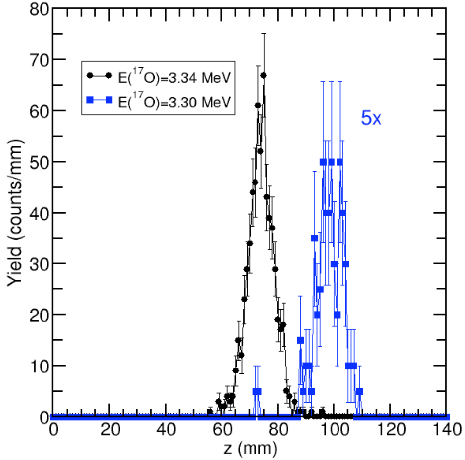
Figure 3.4: The distribution of ^1\text{H}(^{17}\text{O},\alpha)^{14}\text{N} events as a function of the distance ( z ) from the plane of SIDAR (mm) at a pressure of 4 Torr. The 3.30 MeV yield has been multiplied by a factor of 5 for purposes of comparison.
