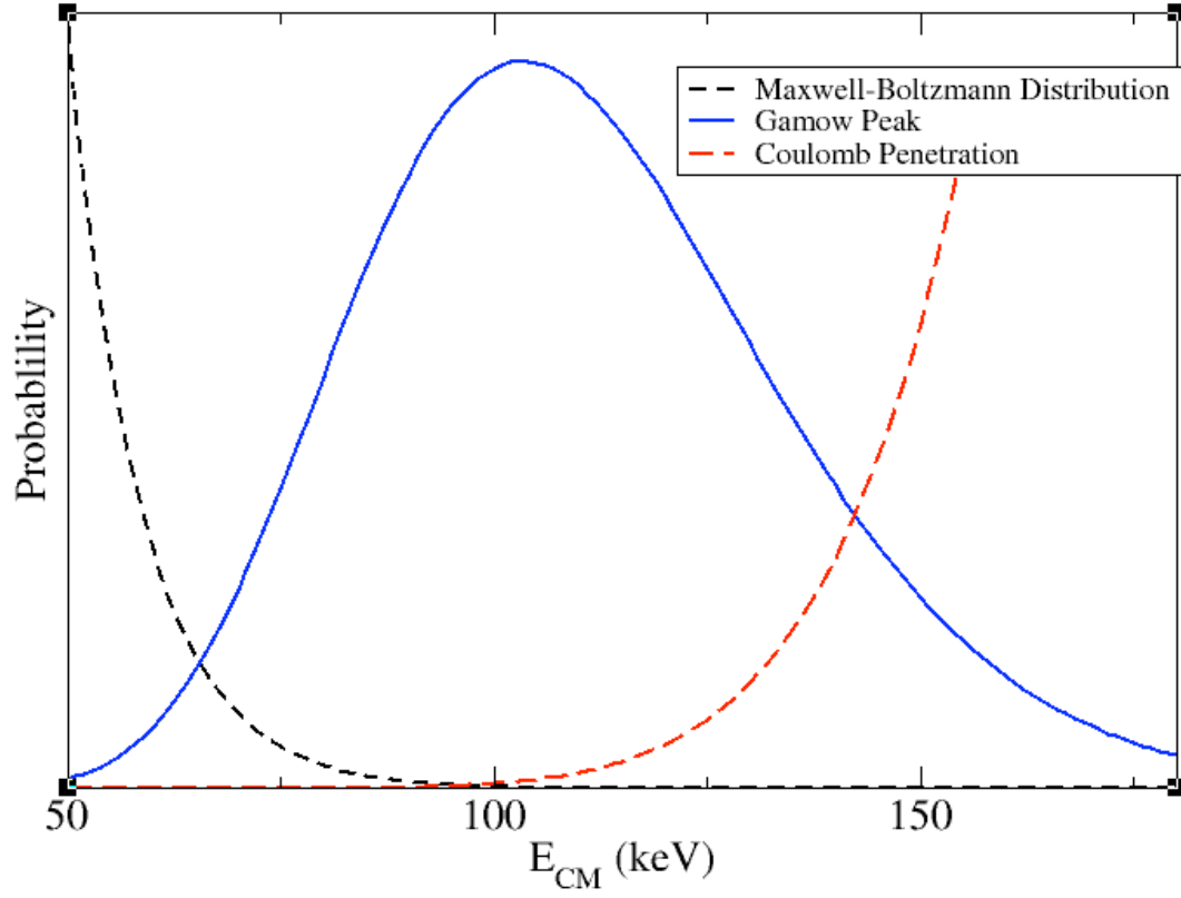
Figure 1.7: The Gamow window for the ^{17}\text{O} + p system for a stellar temperature of T_9 = 0.1 . The values of each curve have been multiplied by different factors for purposes of comparison.
