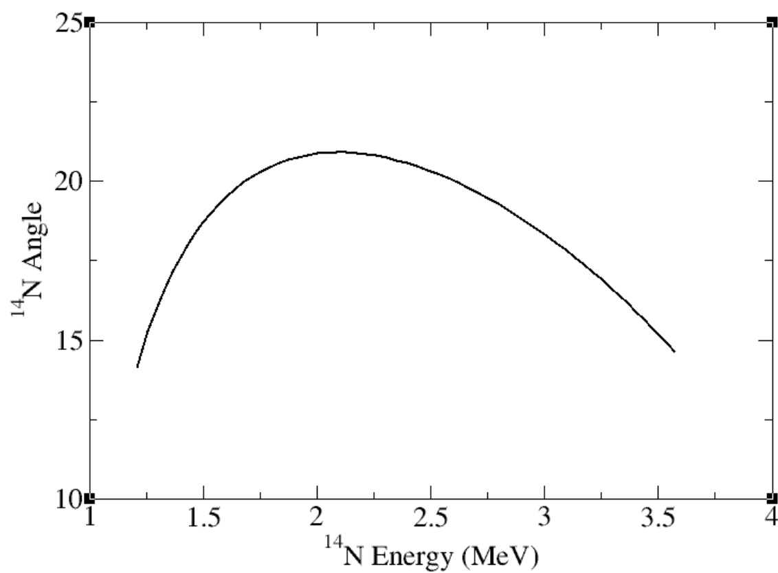
Figure 2.7: Calculated Angle vs. Energy for the ^{14}\text{N} recoils in the ^{17}\text{O}(\text{p},\alpha)^{14}\text{N} reaction at a beam energy of 3.27 MeV. The turnaround angle can be seen to be located at 21^\circ
