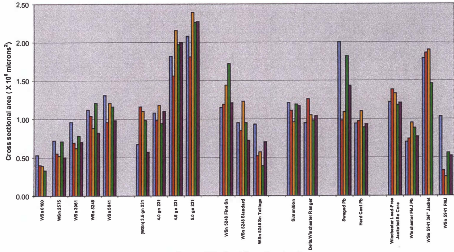
Figure 13. Profilometer Area
