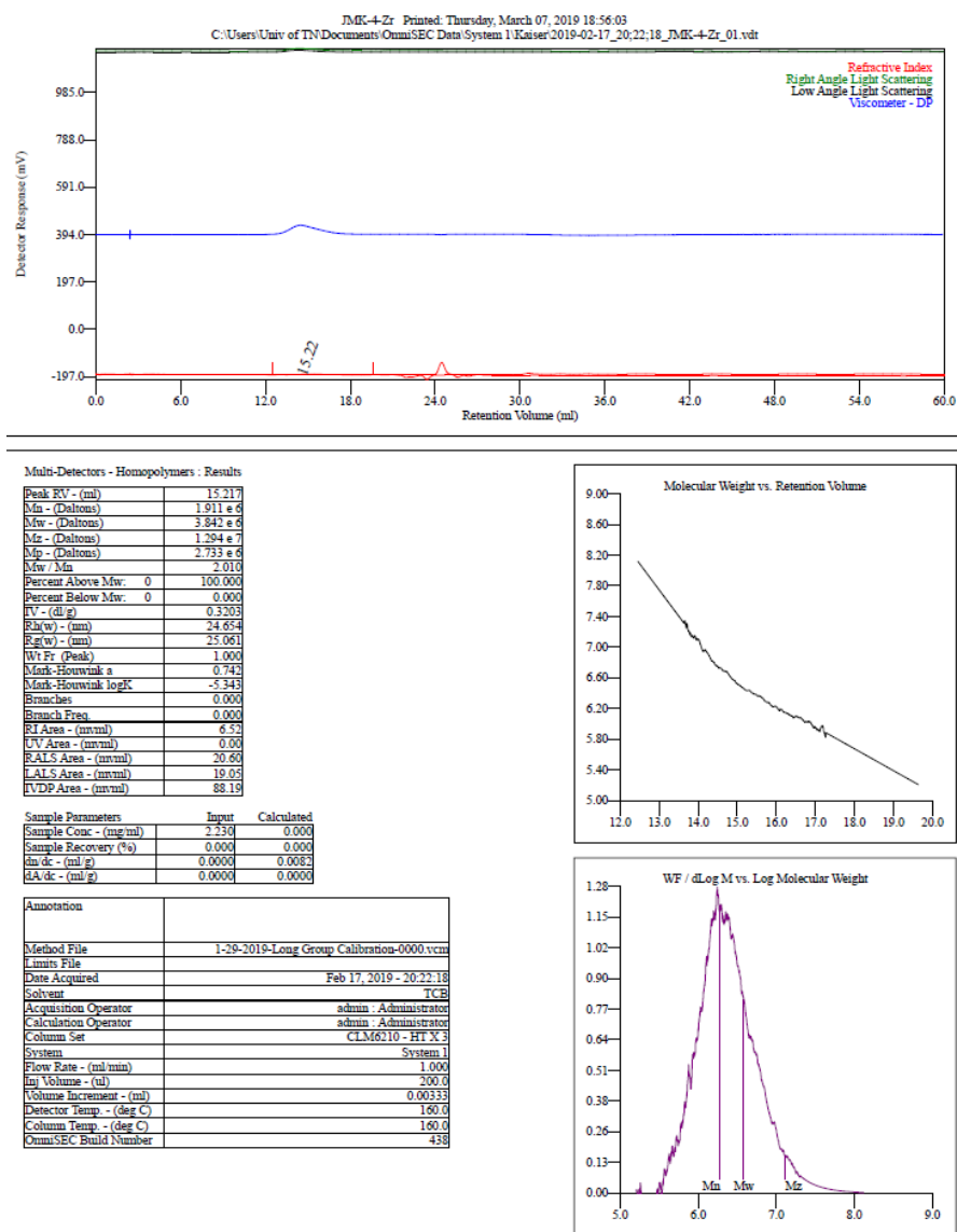
Figure A.22 GPC of polyethylene. (Table 3.4, entry 1)
