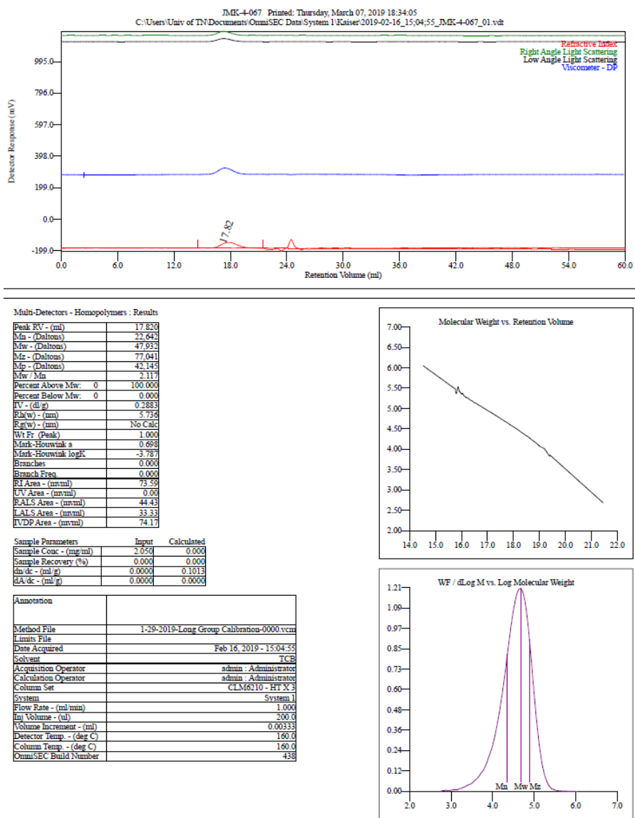
Figure A.13 GPC of poly(1-hexene). (Table 3.2, entry 2)
