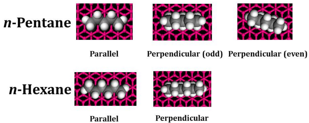
Figure 62 – Minimum energy configurations for pentane and hexane adsorbed on the basal plane of graphite
