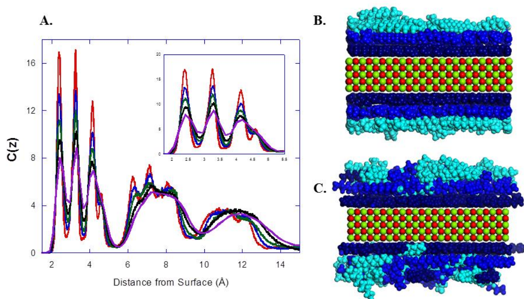
Figure 39 – (A) Representative selection of trilayer-coverage concentration profiles in the z direction, C(z) , for decane molecules on MgO(100). The inset highlights the behavior of the layer nearest to the surface. The temperature profiles pictured are as follows with the temperature shown as a fraction of the bulk triple point in parentheses and color scheme in brackets: 40 K (0.16) [red], 100 K (0.41) [blue], 160 K (0.66) [green], 220 K (0.90) [black], and 280 K (1.15) [purple]. (B) ( T = 40 K) and (C) ( T = 280 K): snapshots of trilayer coverage nonane on MgO(100) with molecules in the nearest layer (dark blue), bilayer (royal blue), and trilayer/bulk (light blue) highlighted to show interlayer mobility as a function of temperature
