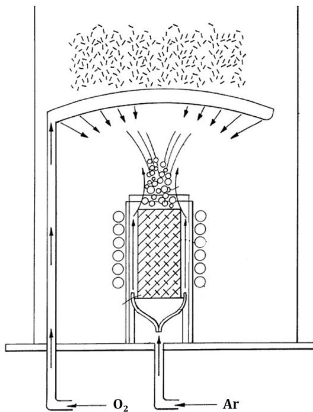
Figure 17 – Diagram for the metal oxide synthesis chamber (Kunnmann-Larese 2001)
