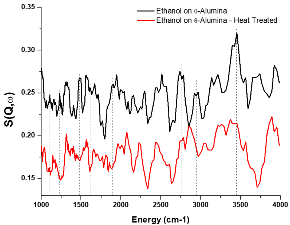
Figure 85 – INS spectrum of monolayer ethanol on \theta -alumina (black) compared with the heat-treated ethanol on alumina (red) in the high energy regime (1000-4000 cm -1 ).
