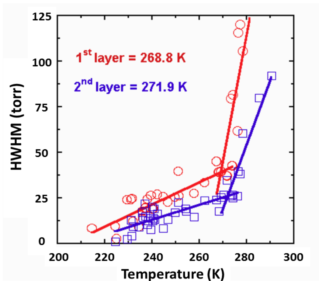
Figure 29 – Half-width at half-maximum (HWHM) for the fitted Gaussian function plotted against temperature for octane on MgO. Note the abrupt change in slope at 268.8 K for the first layer (red circles) and 271.9 K for the second layer (blue squares).
