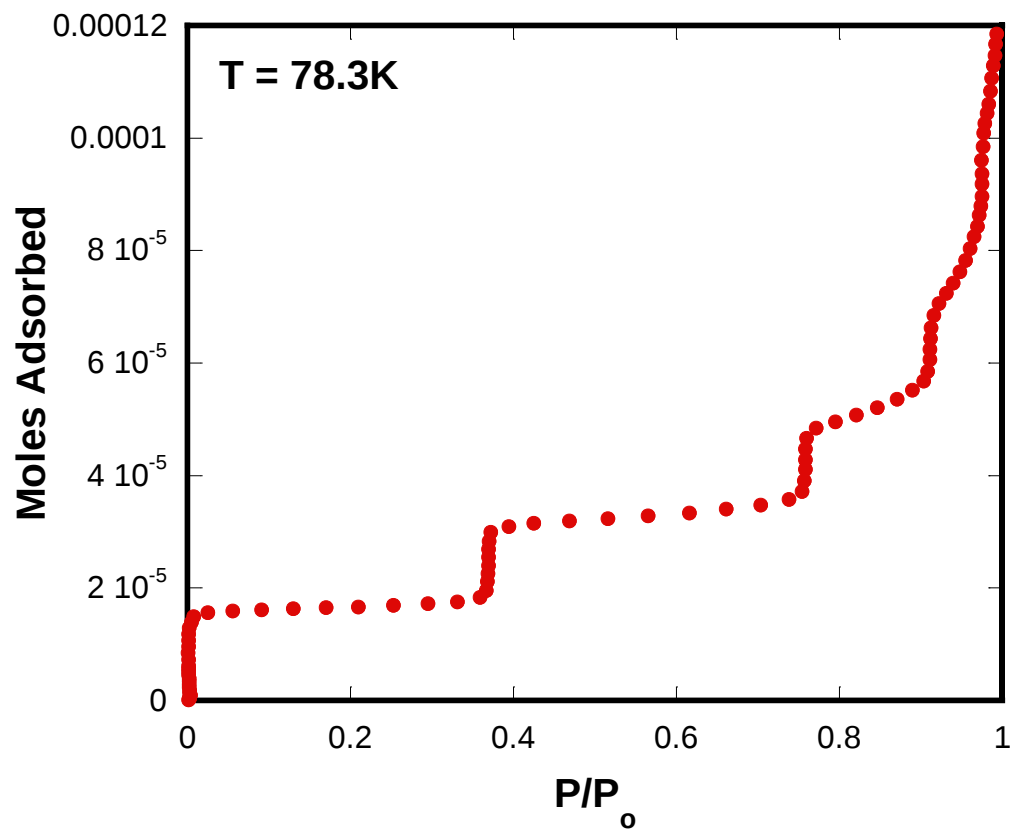
Figure 4 – Adsorption isotherm of methane on graphite at T = 78.3 K
