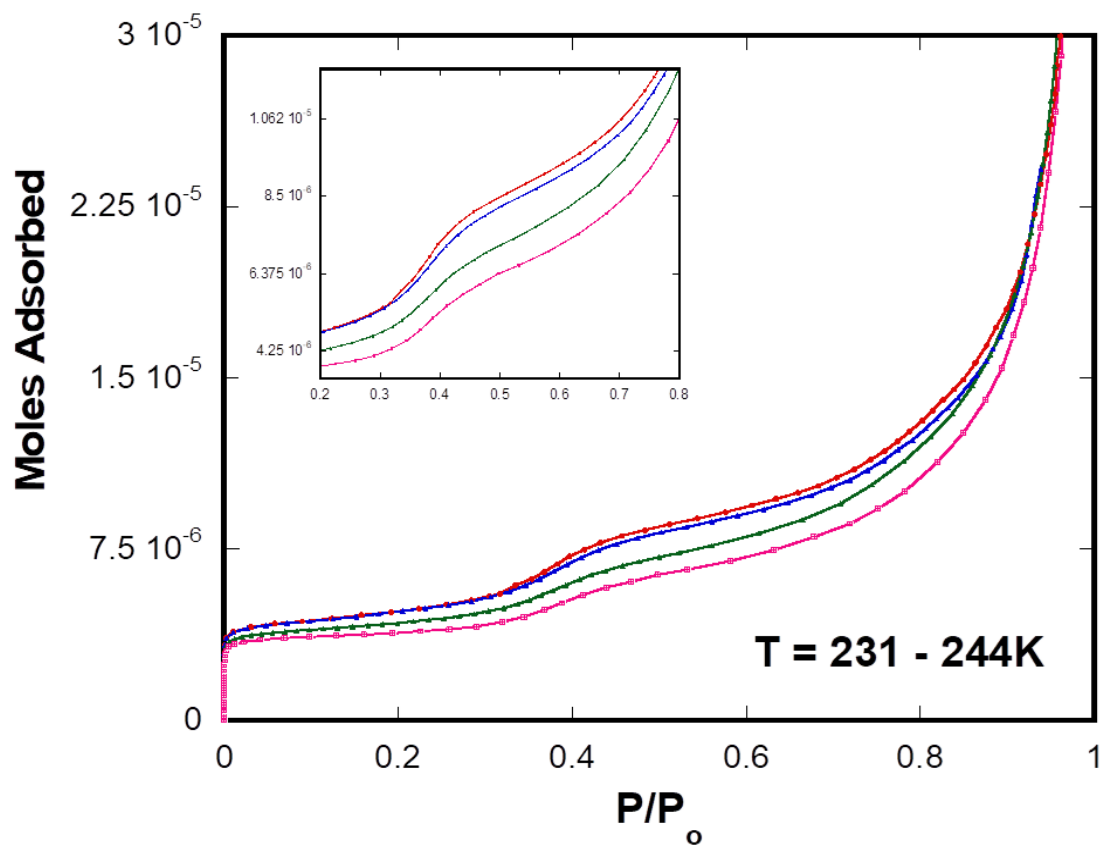
Figure 57 – Plot of moles adsorbed versus reduced vapor pressure ( P/P_0 = equilibrium vapor pressure/saturated vapor pressure) for hexane adsorbed on graphite in the temperature range, T = 231\text{-}244\text{ K} .
