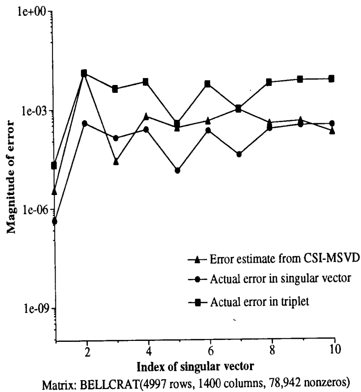
Figure 5.2. Variation in the reliability of the error estimate as an upper-bound for clustered singular values.
