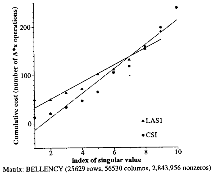
Figure 5.1. Comparison of cumulative overhead when computing singular triplets by LAS1 and CSI-MSVD. CSI-MSVD requires fewer matrix-vector multiplications to calculate each triplet, but LAS1 has a lower cumulative count for k > 8 because more than one singular triplet can be deflated at each step.
