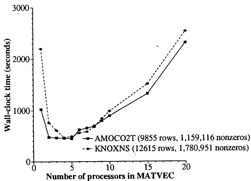
Figure 5.8. CSI-MSVD wall-clock times (seconds) for execution for matrices with \approx 10^6 non-zeros on a network of SUN workstations.
