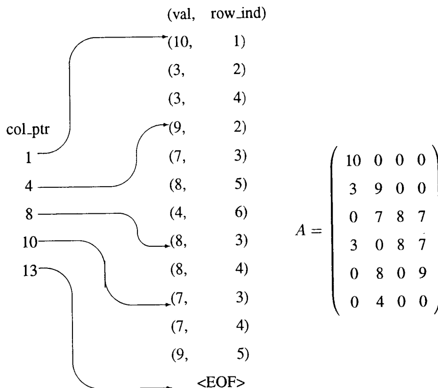
Figure 3.1. Example of the Harwell-Boeing storage format for a 6 \times 4 sparse matrix A .
