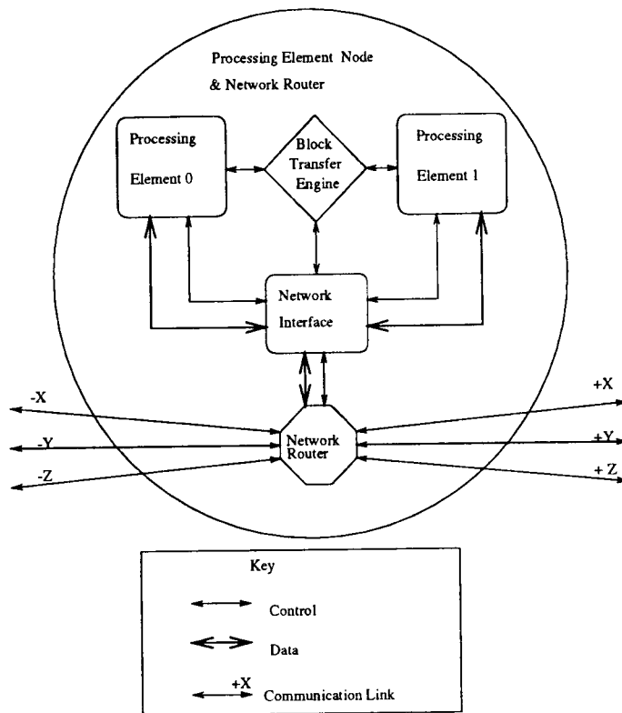
Figure 4.1. Processing element node and interconnect components on the CRAY T3D
