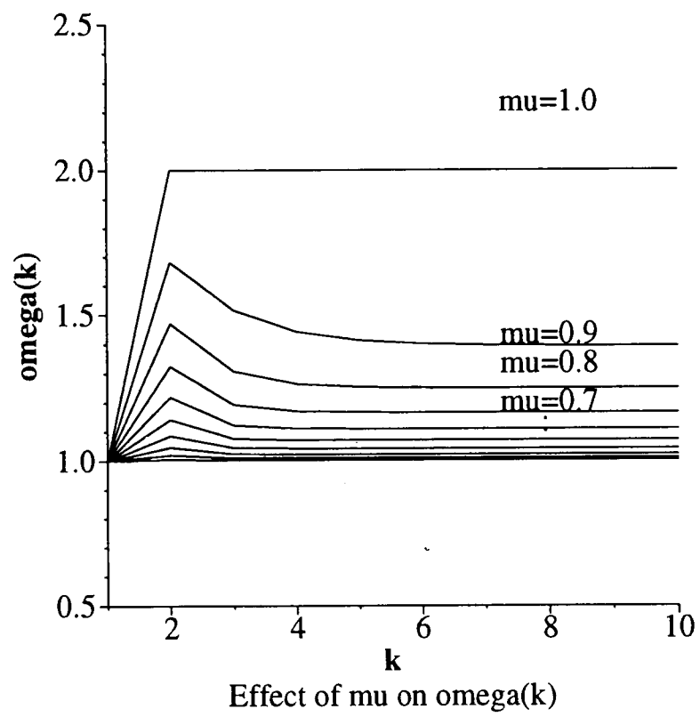
Figure 2.5. Effect of parameter \mu
