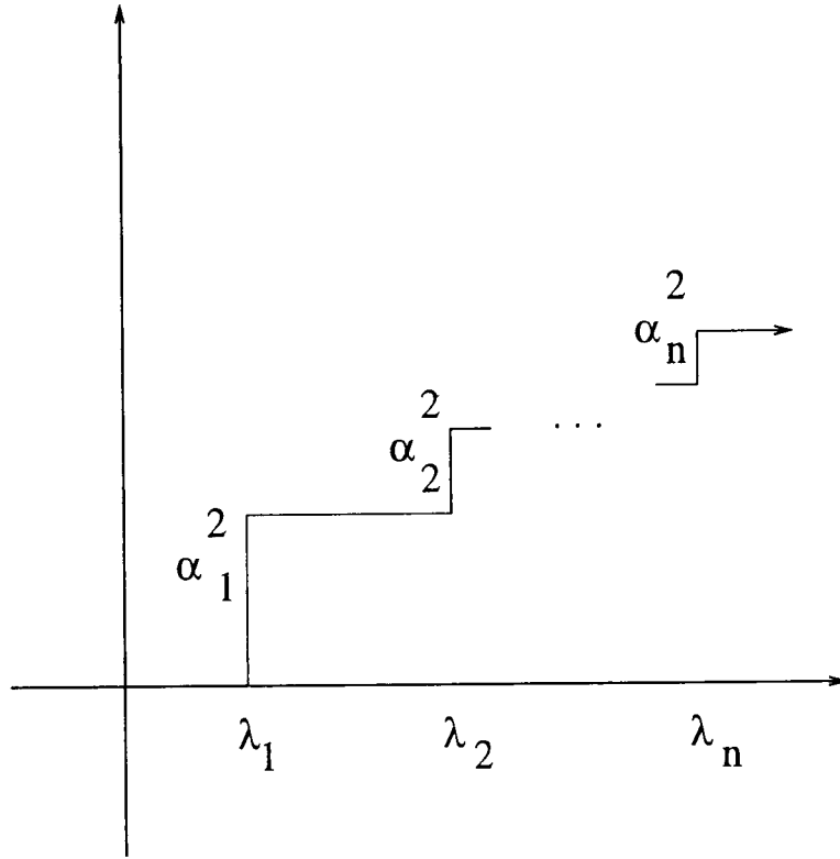
Figure 2.1. The discrete measure d\alpha(\lambda)
