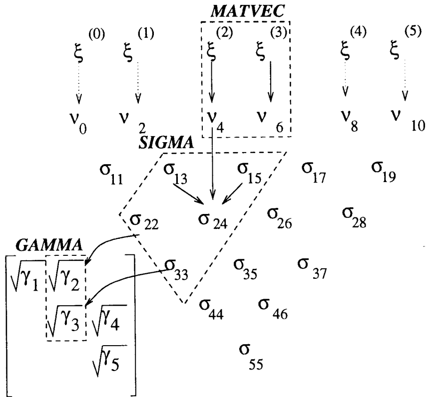
Figure 2.3. A single pass of two-cyclic CSI-MSVD
