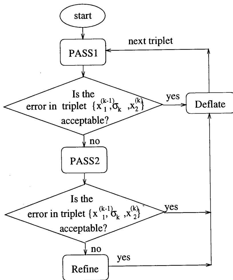
Figure 2.4. Flow chart for computing the k -largest singular triplets using CSI-MSVD
