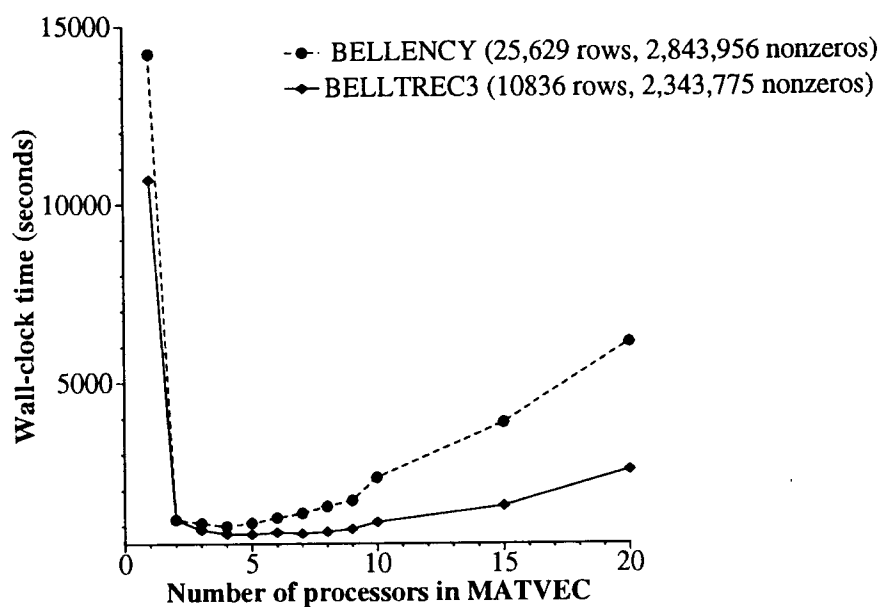
Figure 5.7. CSI-MSVD wall-clock times (seconds) for execution for matrices with \approx 2 \times 10^6 non-zeros on a network of SUN workstations.
