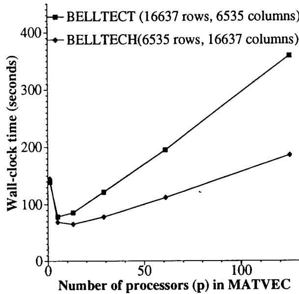
Figure 5.4. Effect of m , the number of rows, on wall-clock times in seconds obtained on the CRAY T3D. BELLTECT is the transpose of the BELLTECH. The communication-overhead is proportional to the number of rows in the matrix, which causes higher wall-clock times for BELLTECT.
