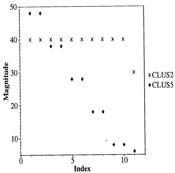
Figure 4.3. Clustered spectra of two 50 \times 50 test matrices.
