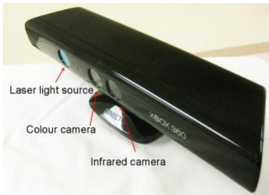
Figure 1. Image of the Kinect with arrows indicating the identity of the cameras. (Dutta 2011)
