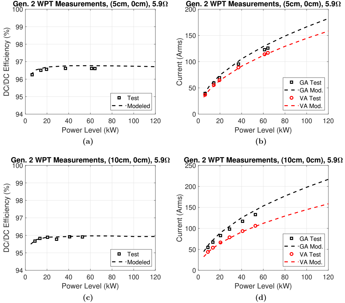
Figure 20: Tests of the Gen. 2 demonstrator at different alignments compared to modeled values near unity gain (grid offset of (-7 mm, -5 mm)) and an airgap of 125 mm. (a) DC/DC efficiency and (b) GA and VA current at (5 cm, 0 cm). (c) DC/DC efficiency and (d) GA and VA current at (10 cm, 0 cm).
