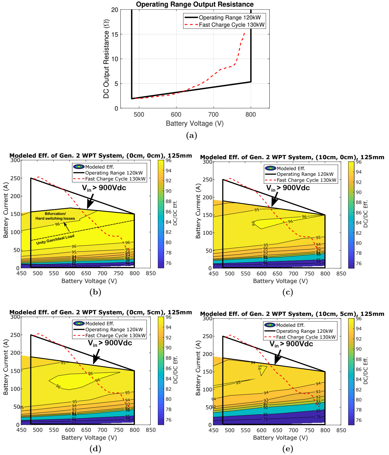
Figure 6.2: Modeled performance of the Gen. 2 demonstrator: (a) Operating range and 130 kW fast charge cycle equivalent output resistance. Efficiency contours of the Gen. 2 System at 125 mm airgap at different alignments: (b) (0 cm, 0 cm), (c) (10 cm, 0 cm), (d) (0 cm, 5 cm), and (e) (10 cm, 5 cm).
