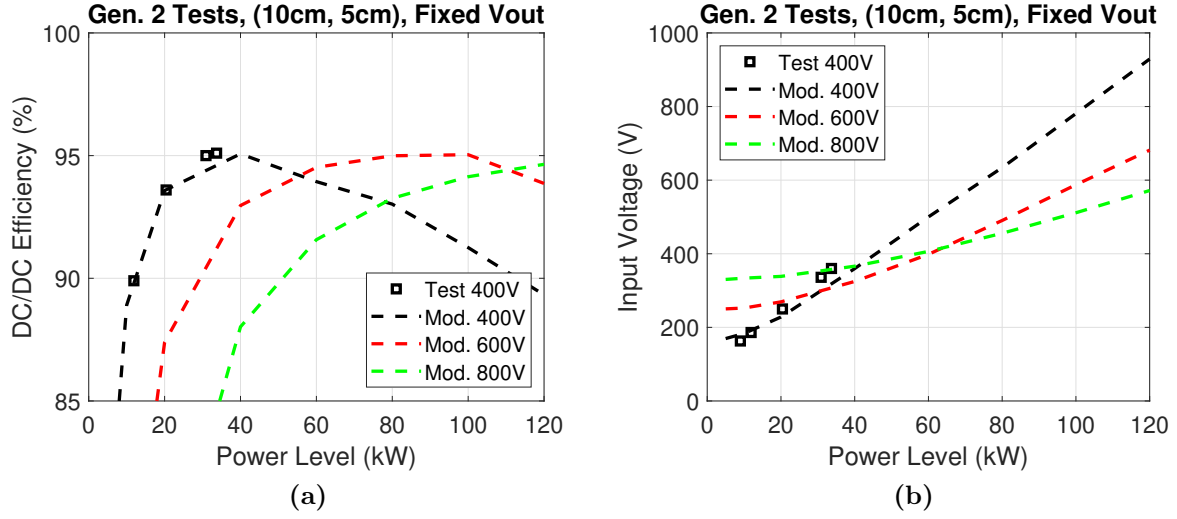
Figure 24: Tests of the Gen. 2 demonstrator at different alignments compared to modeled values at fixed output voltages (grid offset of (-7 mm, -5 mm)) and an airgap of 125 mm. (a) DC/DC efficiency and (b) output power vs. input voltage at (10 cm, 5 cm).
