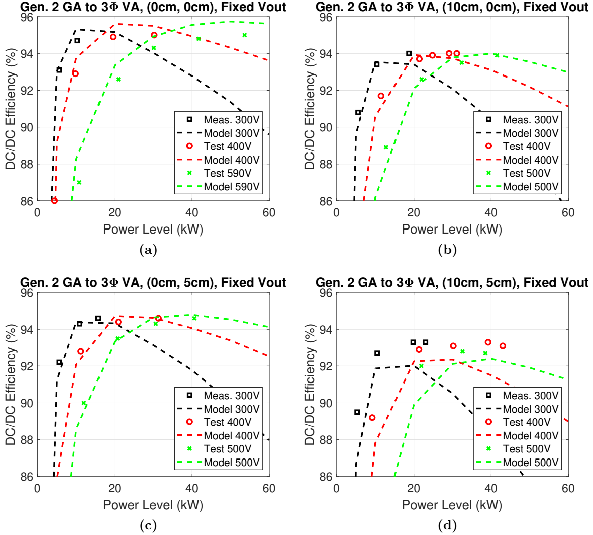
Figure 6.22: Tests of the Gen. 2 GA and 3 \Phi VA at different alignments compared to modeled values at fixed output voltages and an airgap of 125 mm. Output power vs. DC/DC efficiency at alignments of (a) (0 cm, 0 cm), (b) (10 cm, 0 cm), (c) (0 cm, 5 cm), and (d) (10 cm, 5 cm).
