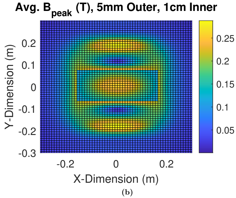
Figure 5.6: Comparison of the ferrite flux density at 120 kW with a 125 mm airgap at alignment. (a) Ferrite flux density with a fixed 1 cm ferrite thickness throughout. (b) Ferrite flux density with an inner 30.7 cm by 13.0 cm region of 1 cm ferrite thickness and an outer ferrite thickness of 5 mm.
