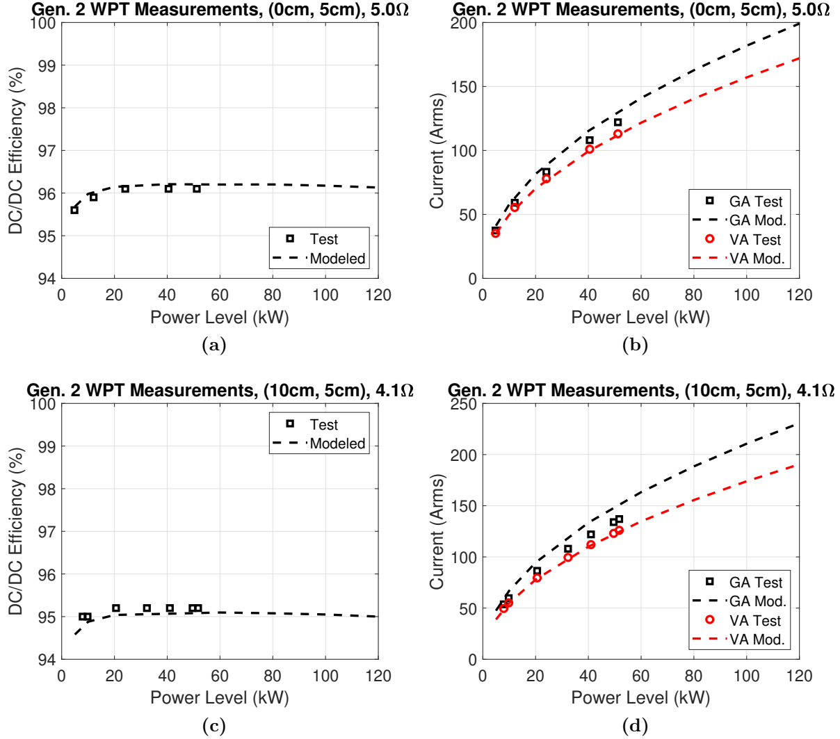
Figure 21: Tests of the Gen. 2 demonstrator at different alignments compared to modeled values near unity gain (grid offset of (-7 mm, -5 mm)) and an airgap of 125 mm. (a) DC/DC efficiency and (b) GA and VA current at (0 cm, 5 cm). (c) DC/DC efficiency and (d) GA and VA current at (10 cm, 5 cm).
