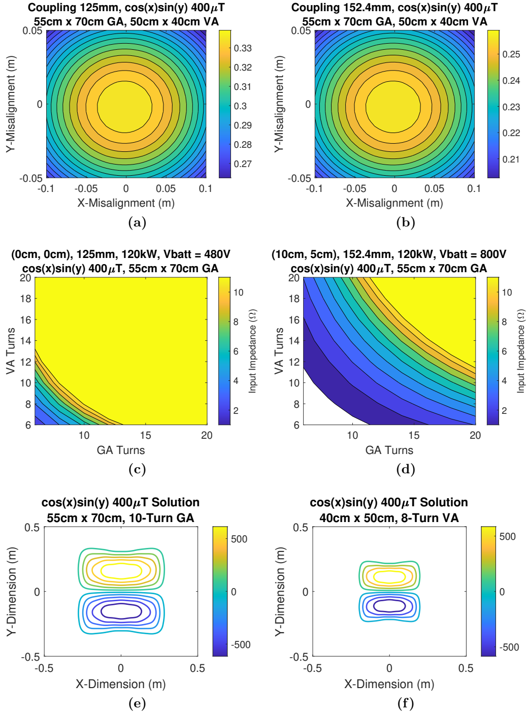
Figure 6.7: Coupling and input impedance of a 55 cm \times 70 cm GA with a 40 cm \times 50 cm VA with the B_{\text{str},\text{lim}} = 400\text{ }\mu\text{T} , \cos x \sin y geometry. Coupling of the GA and VA over misalignment at a (a) 125 mm and (b) 152.4 mm airgap. The input impedance magnitude of the system with different numbers of GA and VA turns when (c) aligned at a 125 mm airgap with the minimum battery output resistance and (d) fully misaligned at (10 cm, 5 cm) at a 152.4 mm airgap with the maximum battery output resistance. The geometries of the (e) 10-turn GA and (f) 8-turn VA.
