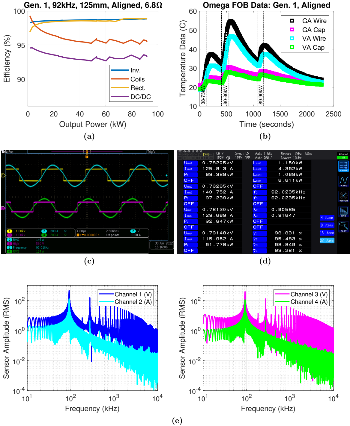
Figure 5.40: Test of the Gen. 1 system at alignment (grid offset of (-7 mm, -5 mm)) and 125 mm. (a) Efficiency breakdown up to 91.8 kW output power. (b) Thermal measurements of the system during testing points around 91.8 kW. (c) Waveforms at 91.8 kW output. (d) Power analyzer screenshot at 91.8 kW. (e) FFT of the waveforms at 91.8 kW.
