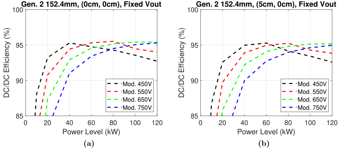
Figure 25: Modeled Gen. 2 demonstrator performance near alignment at fixed output voltages and an airgap of 152.4 mm. (a) DC/DC efficiency at (0 cm, 0 cm) and (b) (5 cm, 0 cm).
