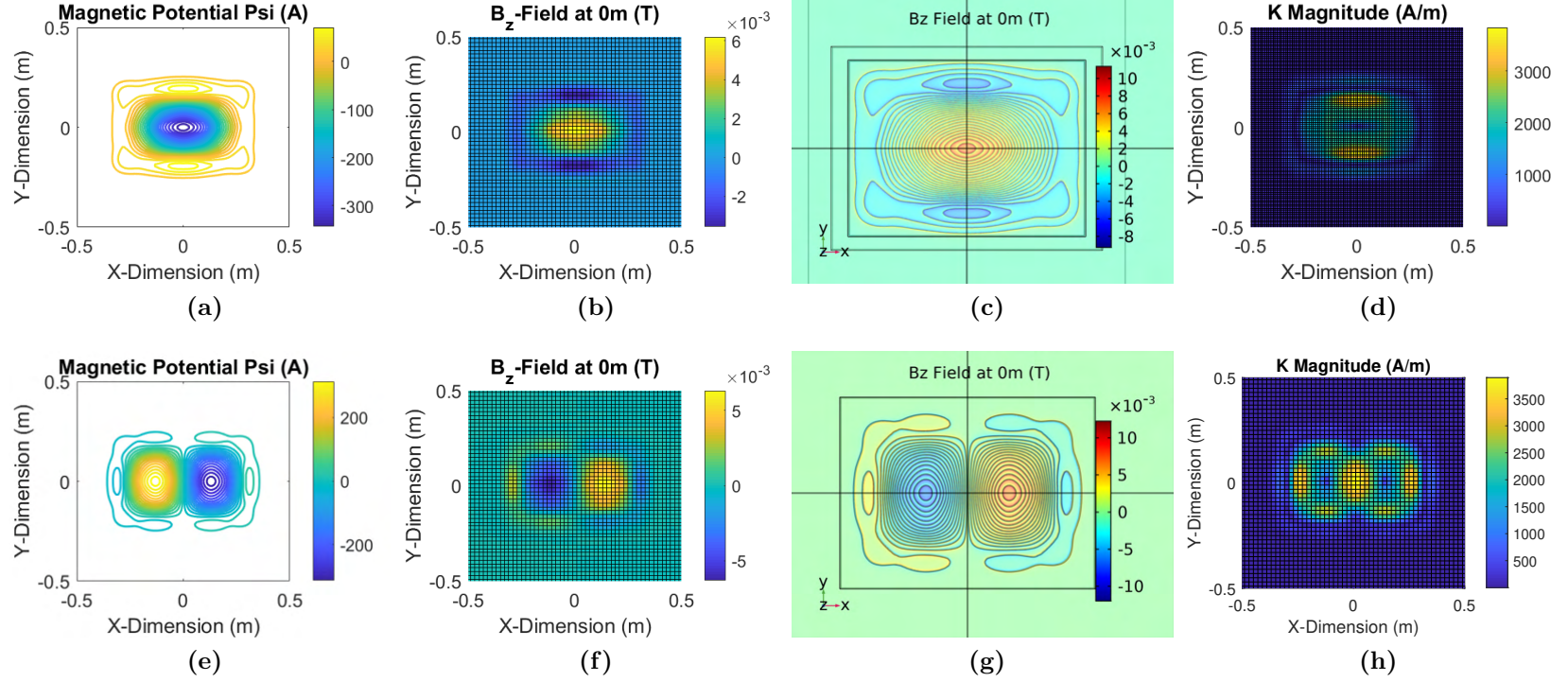
Figure 3.7: Points from the optimization where B_{str,max} = 100 \mu\text{T} shown when f = 85 \text{ kHz} and P = 6.6 \text{ kW} . (a) Coil structure from the \cos x \cos y set with N_T = 25 . (b) Discretized surface field of the \cos x \cos y coil shape. (c) FEA output of the \cos x \cos y coil. (d) Surface current magnitude of the \cos x \cos y coil. (e) Coil structure from the \sin x \cos y set with N_T = 30 . (f) Discretized surface field from the \sin x \cos y coil. (g) FEA output of the \sin x \cos y coil. (h) Surface current magnitude of the \sin x \cos y coil.
