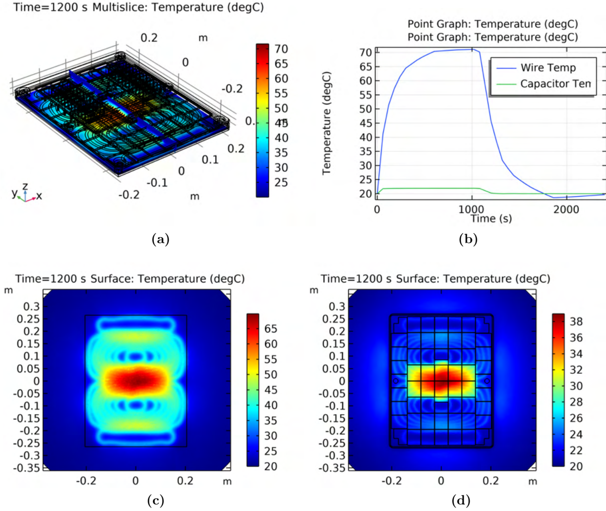
Figure 5.14: Thermal FEA simulations of the Gen. 2 120 kW coil at maximum misalignment with the modeled worst-case losses at 120 kW with 20 minutes of operation: 1200 W of wire loss, 600 W of capacitor loss, and 800 W of ferrite loss. (a) Isometric view of the simulation after 20 minutes. (b) Temperature over time of the center of the wire and one of the backside capacitors. (c) Temperature distribution on the surface of the wire. (d) Temperature distribution 2.5 mm from the surface of the ferrite.
