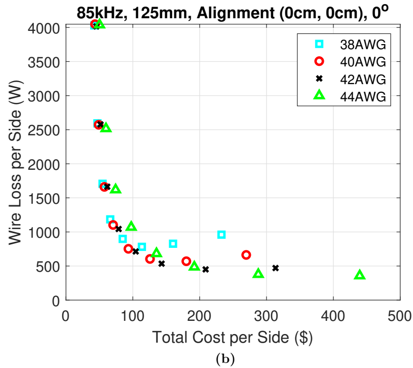
Figure 5.7: The loss, cost, and weight of different litz wire diameters and stranding. The overall cable size is swept from 16 AWG to 2 AWG equivalents from left to right. (a) Weight and loss plot. (b) Cost and loss plot.
