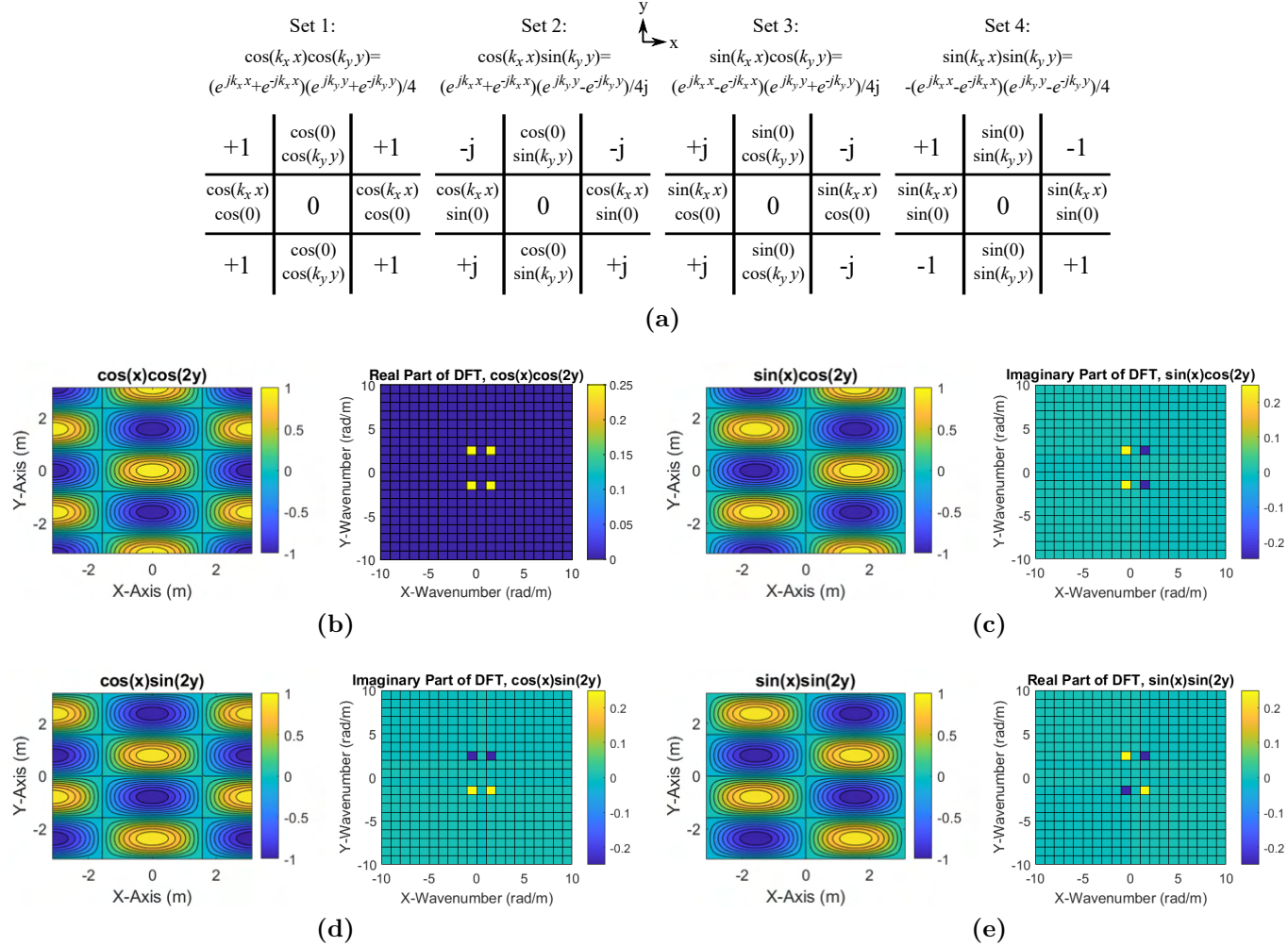
Figure 3.1: Diagrams of the 4 Basis Functions sets considered in the Fourier Analysis Method. (a) The symmetry conditions for each basis function set comprised of real and complex conjugate relationships. With these relationships, each basis function can be represented by one value in the first quadrant, limiting the number of variables and constraints needed in the optimization function. (b) Example of a \cos k_x x \cos k_y y basis function. (c) Example of the \sin k_x x \cos k_y y basis function. (d) Example of the \cos k_x x \sin k_y y basis function. (e) Example of the \sin k_x x \sin k_y y basis function.
