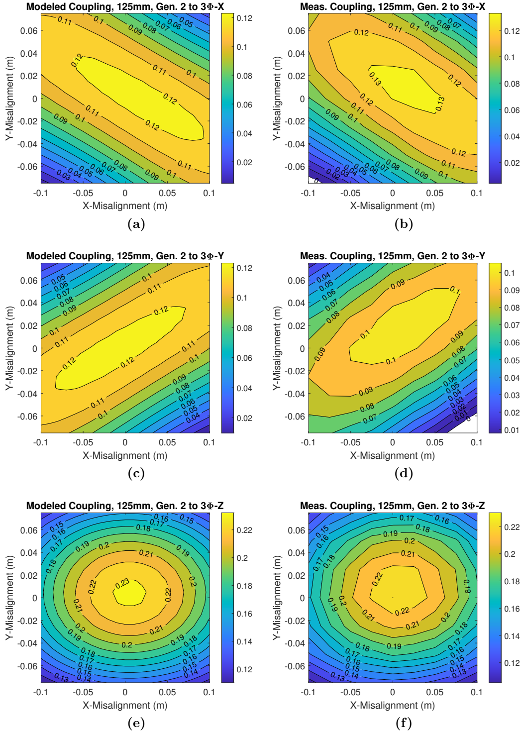
Figure 6.20: Comparison of the FAM-derived and measured coupling over misalignment of the Gen. 2 GA and the ORNL 50 kW 3 \Phi Coil at 125 mm airgap with the Z-winding aligned with the Gen. 2 GA. (a) Modeled and (b) measured coupling to the X-winding. (c) Modeled and (d) measured coupling to the Y-winding. (e) Modeled and (f) measured coupling to the Z-winding.
