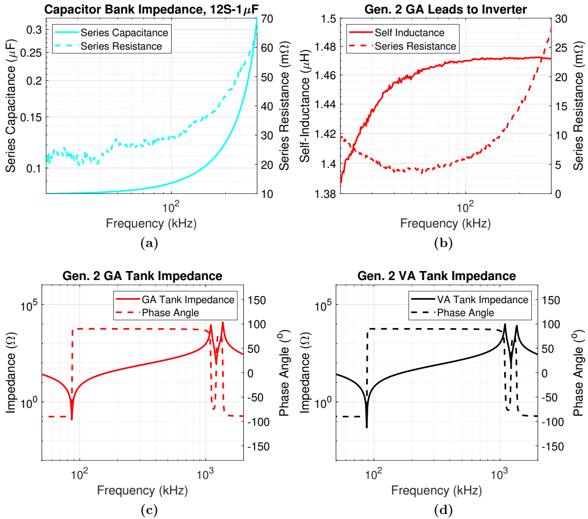
Figure 5.39: Measurements of the tank elements comprised of twelve 1 \mu F Celestion CSM 150/300 capacitors and series tank impedance with the Gen. 2 coils. (a) Measured capacitor bank series capacitance and resistance. (b) Measured lead impedance to and from the GA and VA to the inverter and rectifier. (c) Cured measurements of the Gen. 2 GA tank. (d) Cured measurements of the Gen. 2 VA tank.
