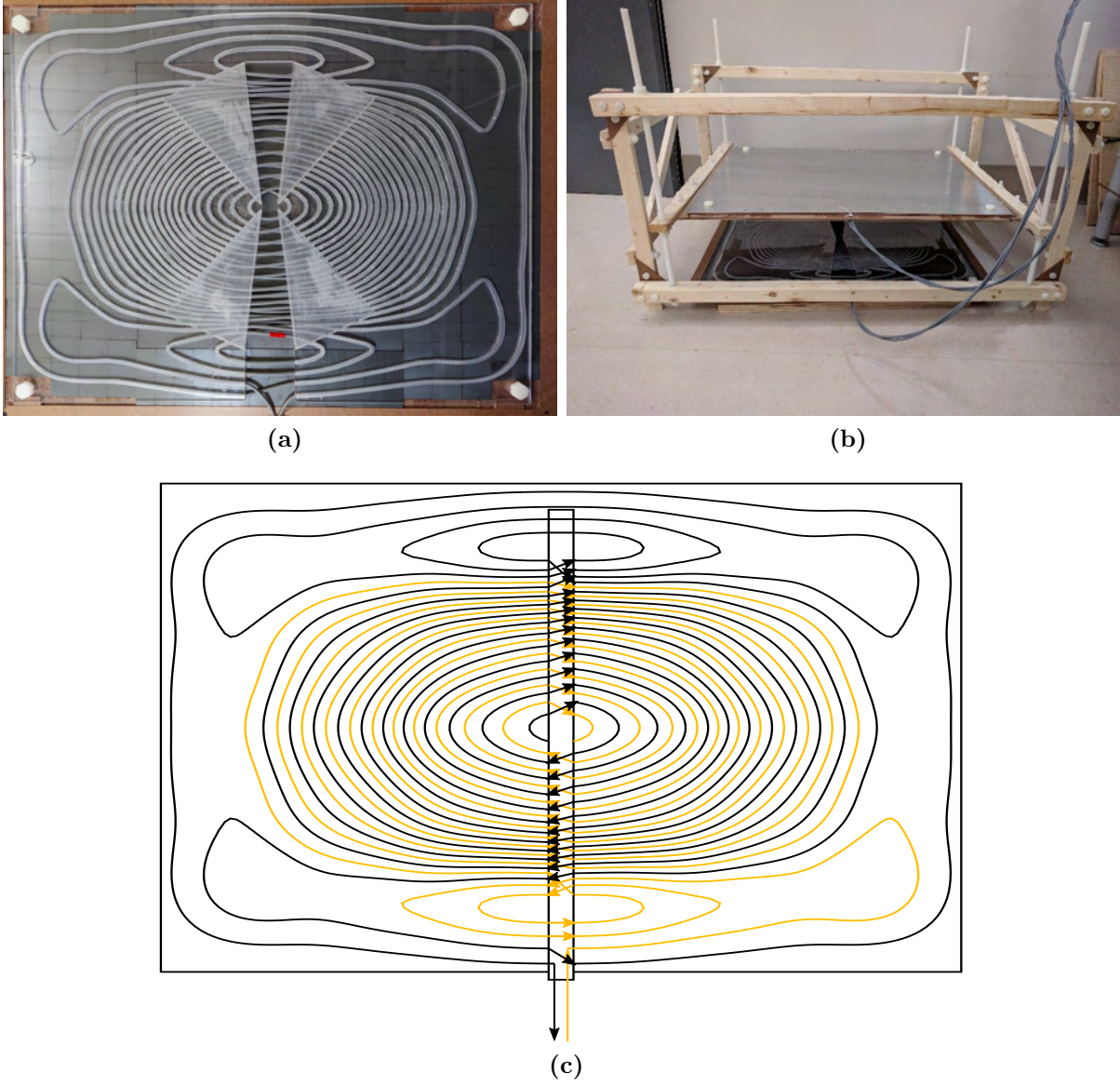
Figure 4.3: 6.6 kW demonstrator construction: (a) Demonstrator 6.6 kW coil. (b) Airgap holder used to set varying airgap and misalignments. (c) Winding pattern of the coil. Here the orange turns go into the coil and the black turns go out of the structure.
