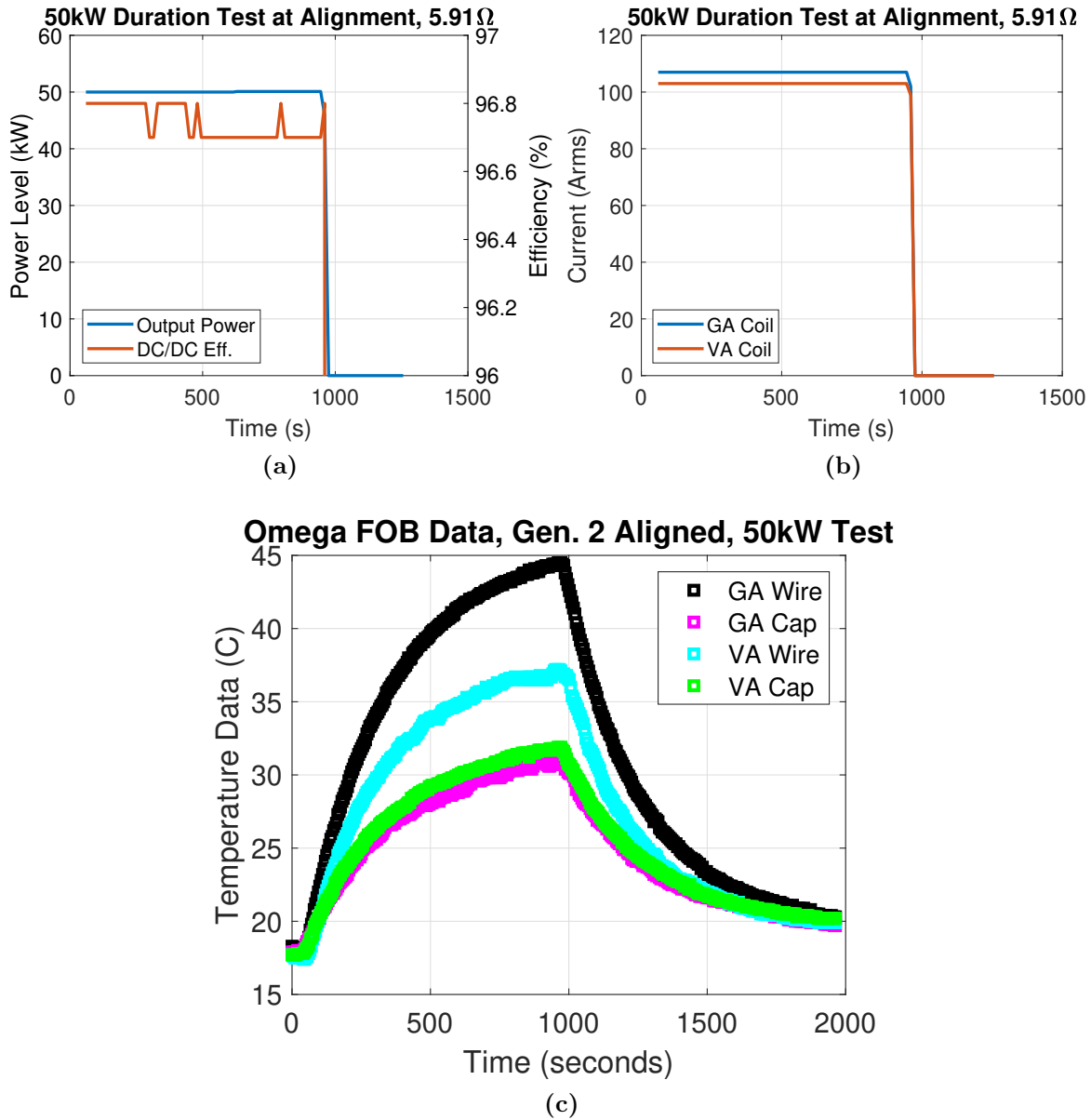
Figure 5.46: Measurements of the Gen. 2 demonstrator from the 50 kW, 15-minute duration test. Power transfer starts at the 60 second mark. (a) Measured output power and DC/DC efficiency during the test. (b) Measured GA and VA currents during the test. (c) Measured temperatures.
