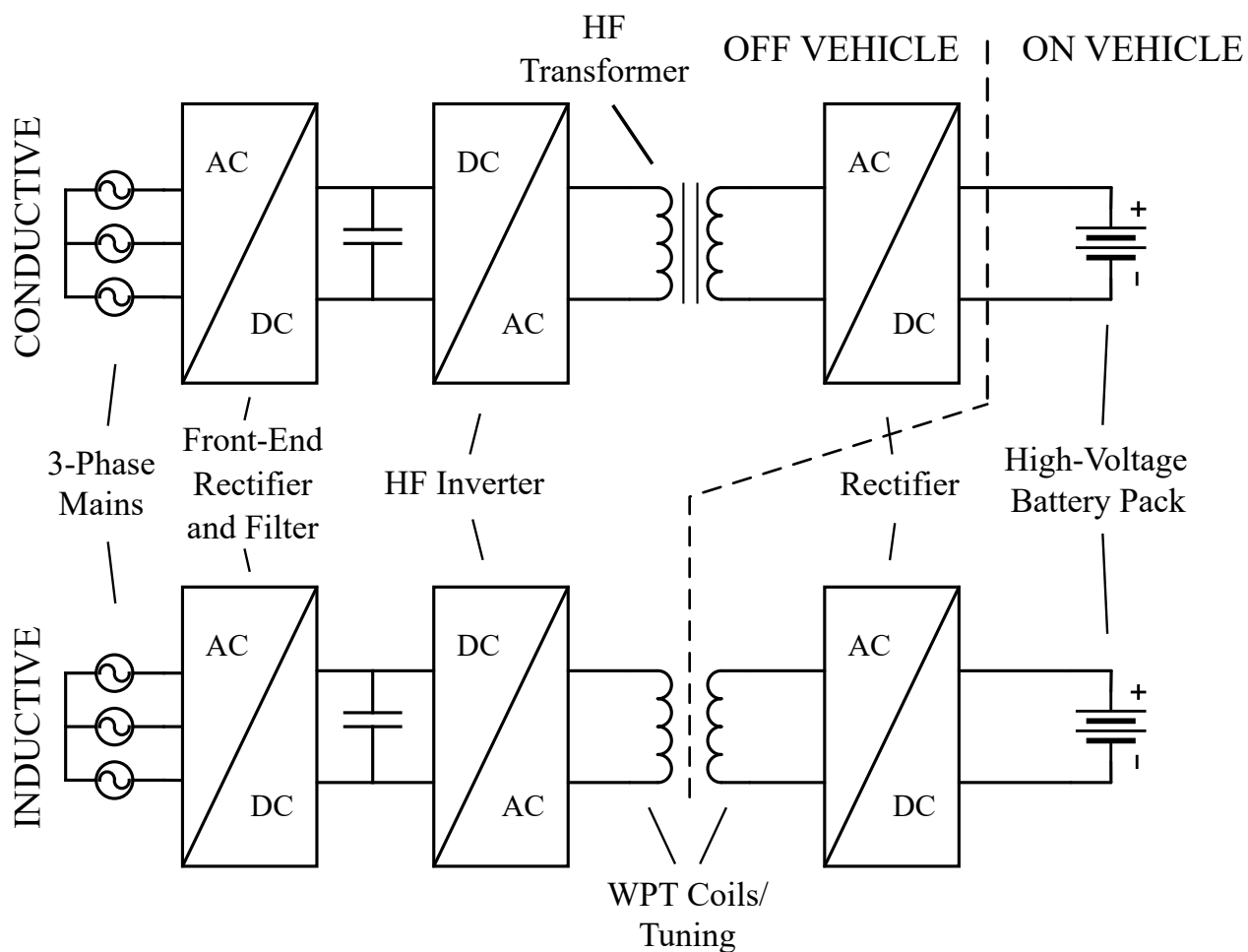
Figure 1.3: Block diagram of a typical conductive DC-fast charging system vs. a high-power inductive WPT system. As seen, the inductive WPT stage replaces the isolated DC/DC converter used in the conductive charger.
