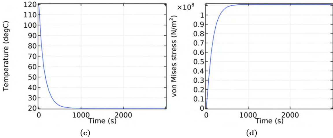
Figure 5.17: FEA simulation of the small-scale coil for the compression effect test. (a) Peak flux density in the coil with 20 A(rms) of coil current. (b) Stresses induced by thermal contraction of the materials from 120°C to 20°C. (c) Temperature at the center of the 2.7 mm ferrite sheet over time. (d) Stress in the center of the 2.7 mm ferrite sheet over time.
