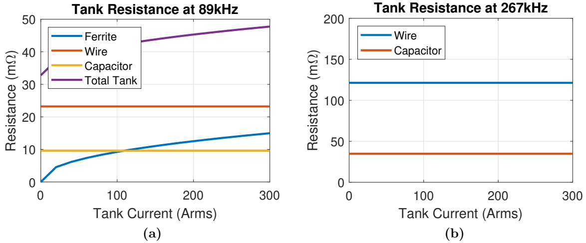
Figure 5.30: Modeled resistance values used in the PLECS simulations at the first two odd harmonics. (a) The modeled resistance values at 89 kHz and (b) 267 kHz.
