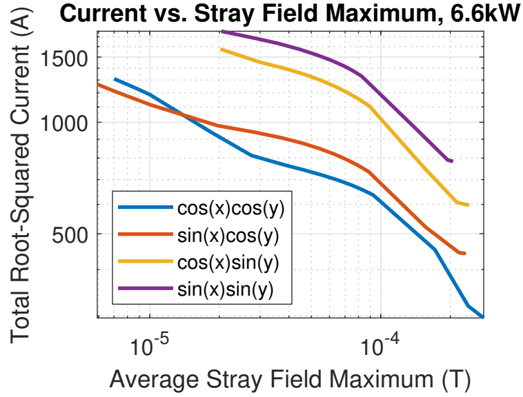
Figure 3.6: The maximum average stray field magnitude for the optimized coils vs. the square root of the integral of the current magnitude squared over a range of B_{str,lim} of 5 \mu T to 1 mT.
