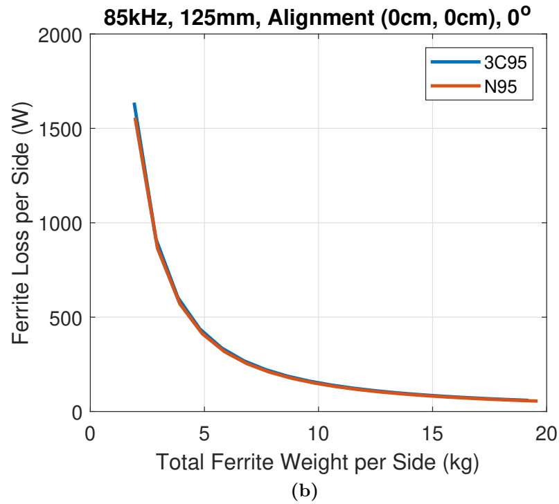
Figure 5.5: Comparison of the ideal ferrite losses per manufacturer Steinmetz equation coefficient and the weight of Ferroxcube 3C95 material and N95 material. (a) Comparison of the cost of the material vs. loss. (b) Comparison of the losses of the materials as a function of weight.
