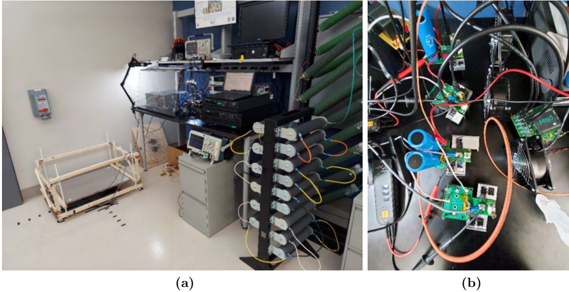
Figure 4.2: Test bench setup for the 6.6 kW demonstrator. (a) Overall test bench with WPT coils, compensation capacitors, inverters and rectifiers, multimeters, power supplies, an electronic load, and wirewound resistors from left to right. (b) Closeup of inverter and rectifier half-bridge modules and control board.
