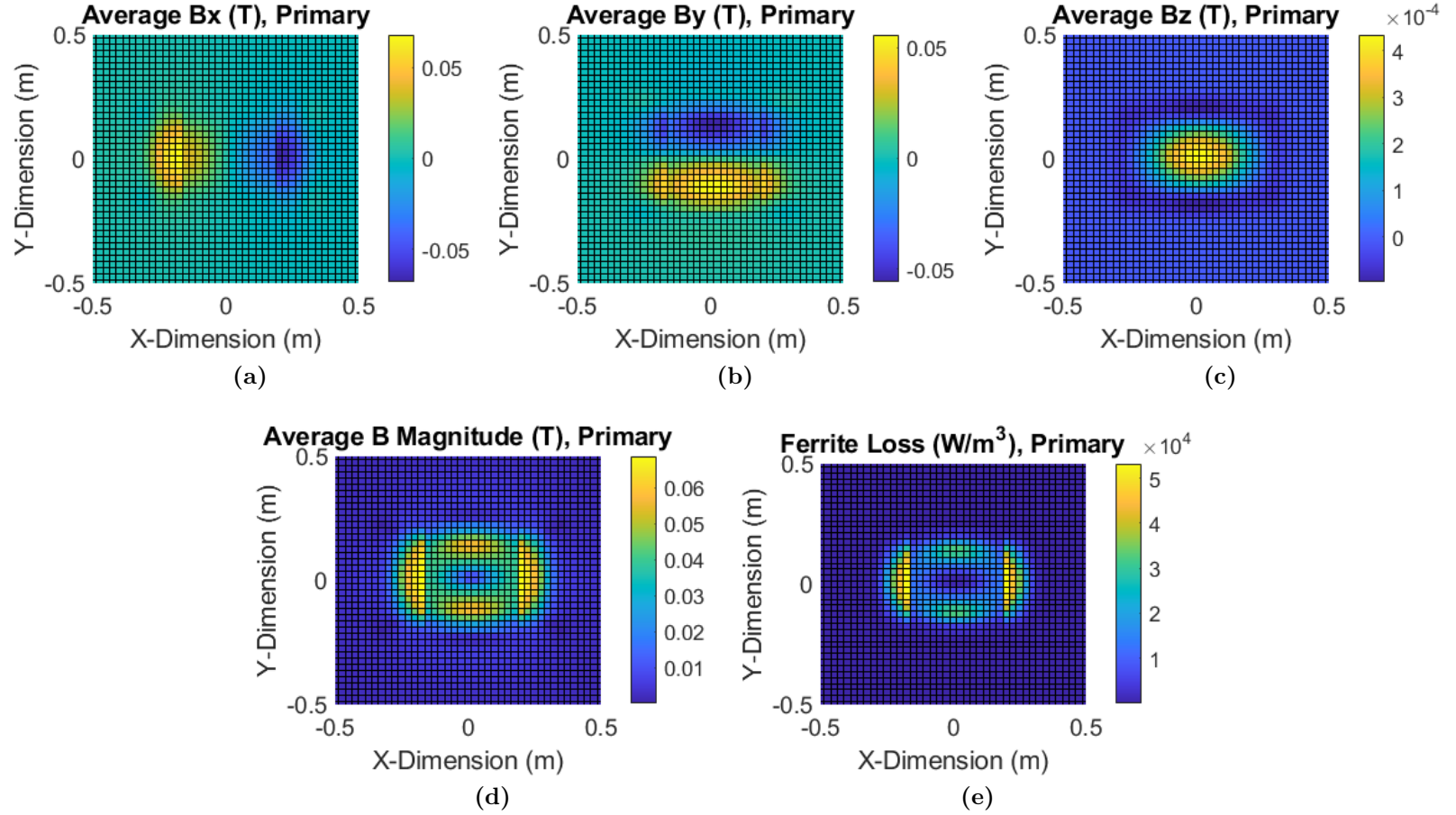
Figure 3.11: Ferrite flux of the 6.6 kW coil derived in FAM: Average RMS fields in primary ferrite coil with a current of 17.3 A in the (a) x -direction, (b) y -direction, and (c) z -direction. (d) The RMS magnitude of the ferrite flux. (e) The spatial specific power loss of the primary coil ferrite at 85 kHz for C_m = 92.66\text{e-}3 , \alpha = 1.045 , and \beta = 2.440 at T_{fer} = 20^\circ\text{C} . Here the inner ferrite is 5 mm and the outer ferrite is 2.7 mm, leading to lower peak fields and lower specific power loss in the middle section.
