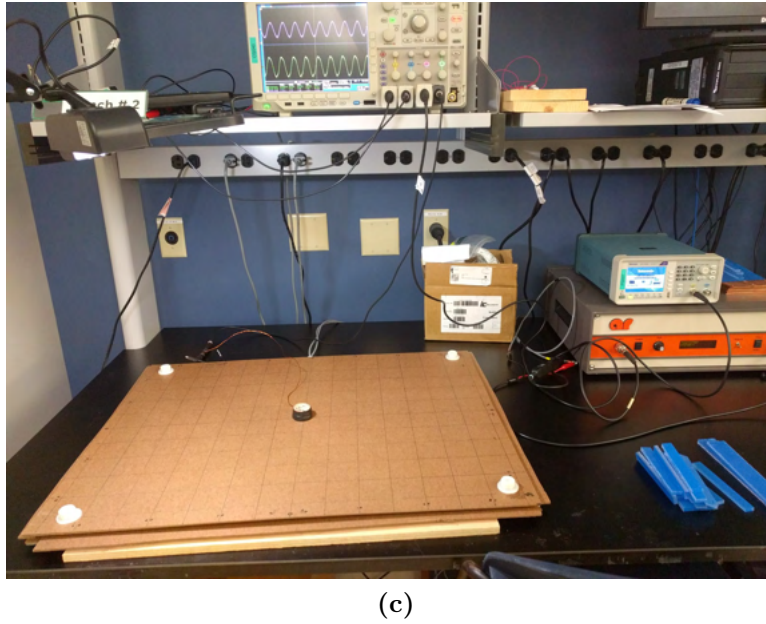
Figure 4.7: Surface field measurement of 6.6 kW coil: (a) Predicted surface B_z of coil. (b) Scaled measured surface B_z of coil. (c) Measurement setup with power amplifier.
