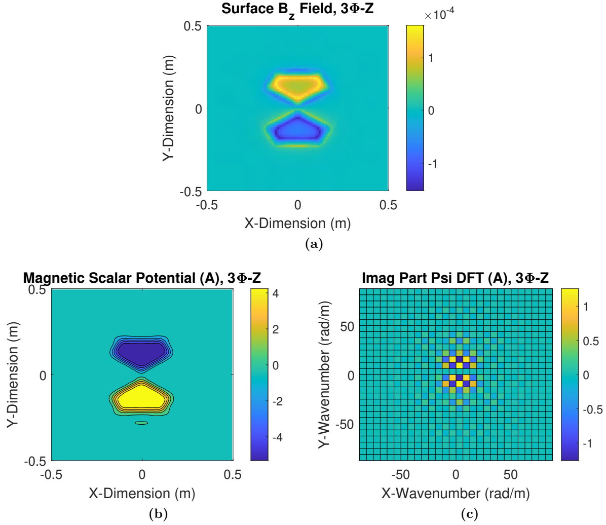
Figure 6.19: Importation of the Z-winding of the 3\Phi coil into Fourier components. (a) The surface B_z field of the Z-winding with 1 A. The resulting (b) magnetic scalar potential and (c) discrete Fourier components.
