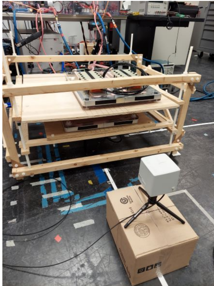
Figure 5.54: Field measurement setup of the Gen. 2 demonstrator. Here a box was used to elevate the probe to the middle of the airgap and tape was placed with markings at distances of 60 cm, 80 cm, and 100 cm on the X and Y axes.
