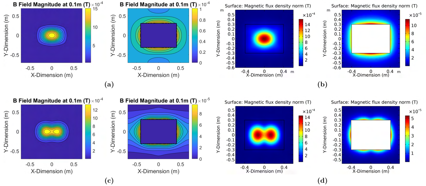
Figure 3.8: Fields calculated in FAM and simulated in FEA for the \cos x \cos y coil: (a) Calculated field magnitude at z = 0.1 m for the \cos x \cos y coil. (b) Fields from FEA simulation with one coil energized for the \cos x \cos y coil. (c) Calculated stray field at z = 0.1 m for the \sin x \cos y coil. (d) Fields from FEA simulation with one coil energized for the \sin x \cos y coil.
