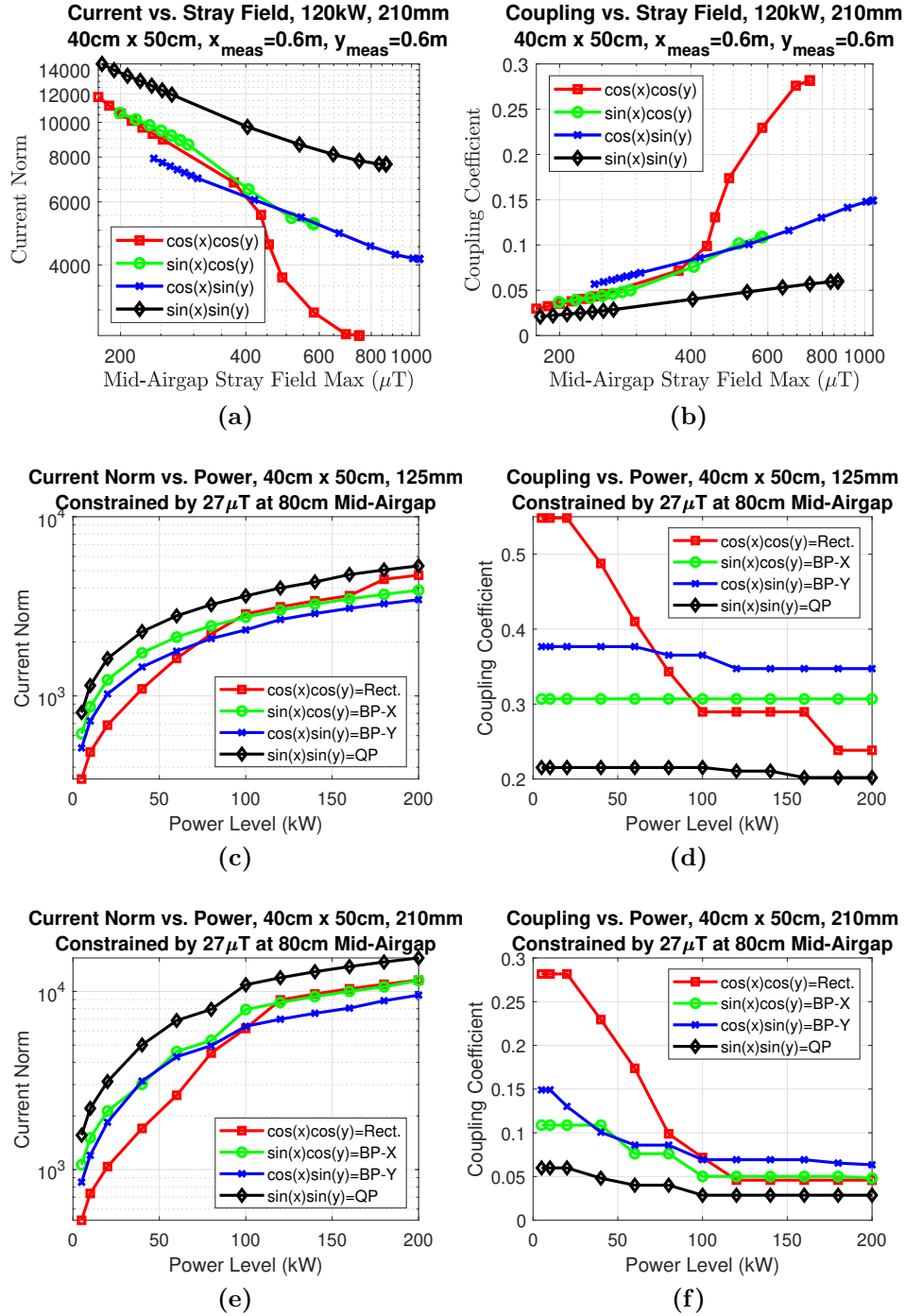
Figure 7.2: Tradeoff analysis of the 40 cm x 50 cm single-phase geometries as a function of power level when constrained by a constant stray field at 80 cm. (a) Current vs. stray field and (b) coupling vs. stray field at mid-airgap at x_{ext} = y_{ext} = 60 cm at 120 kW and 210 mm. (c) Current norm and (d) coupling vs. power level at a 125 mm airgap. (e) Current norm and (f) coupling vs. power level at a 210 mm airgap.
